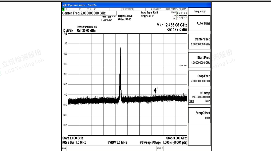
Band2_10MHz_16QAM_18900_1RB#0_1000~3000_1000~3000
