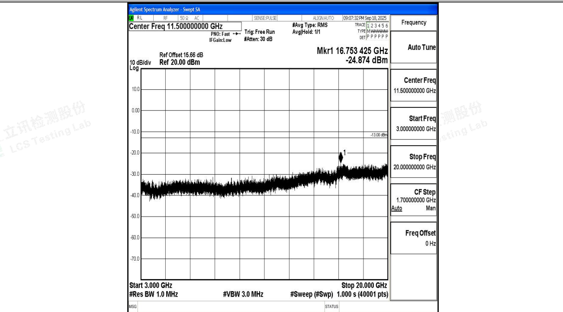
Band2_5MHz_QPSK_18900_1RB#0_3000~20000_3000~20000
