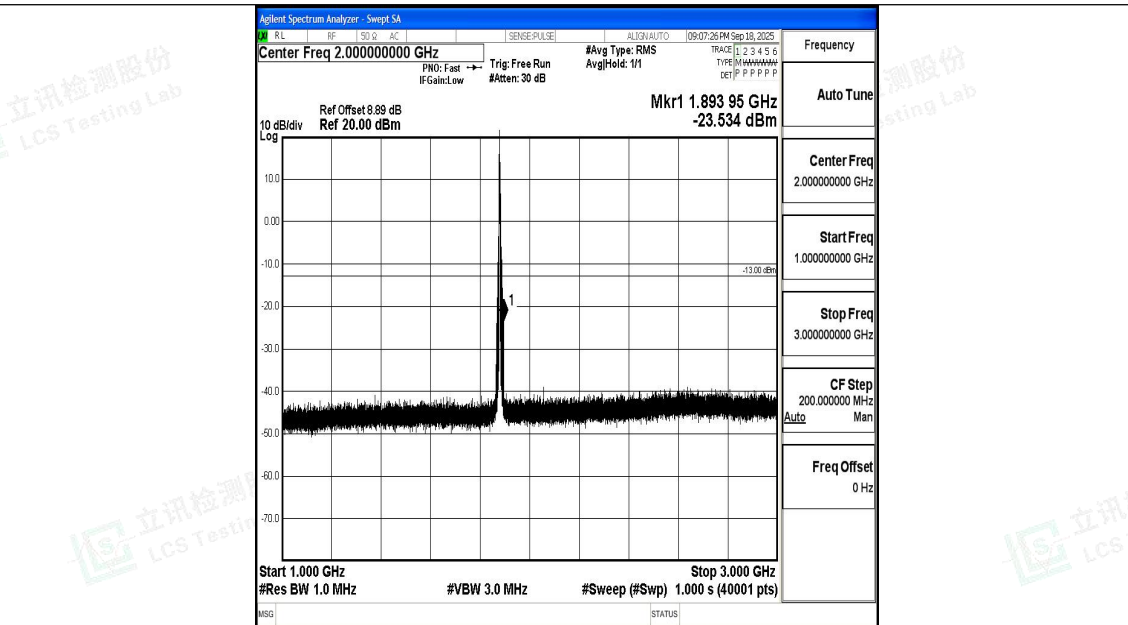
Band2_5MHz_QPSK_18900_1RB#0_1000~3000_1000~3000
