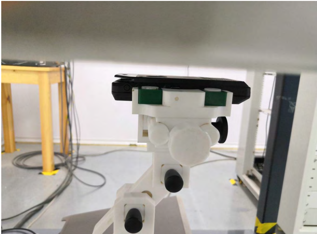
10mm body-worn Front Side Setup Photo (hotspot)
