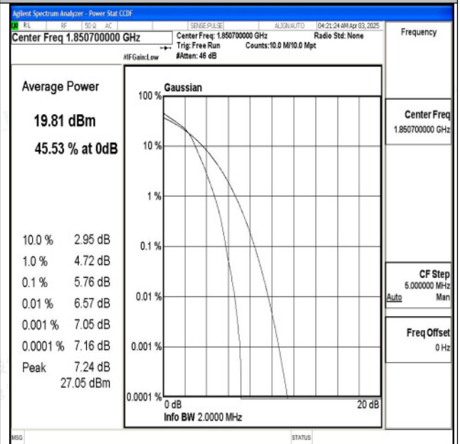
Band2-1.4MHz-16QAM-18607-6RB#0-PASS
