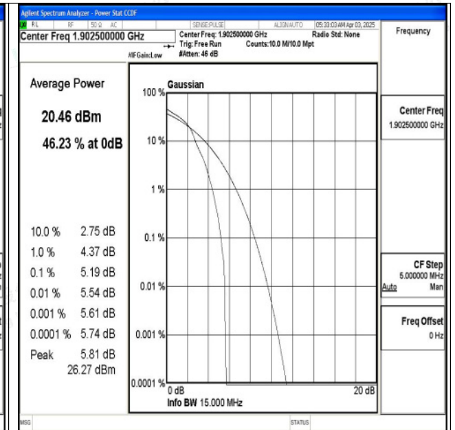
Band2-15MHz-16QAM-19125-1RB#0-PASS
