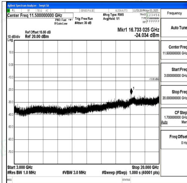
Band2_1.4MHz_QPSK_18607_1RB#0_3000~20000_300 0~20000
