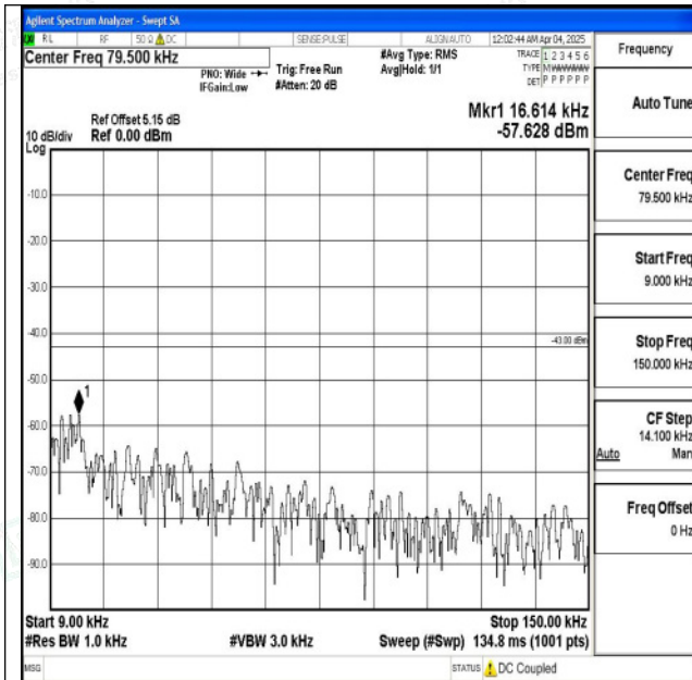
Band2_5MHz_QPSK_18625_1RB#0_0.009~0.15_0.009~0.15
