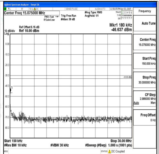
Band2_1.4MHz_QPSK_19193_1RB#0_0.15~30_0.15~30
