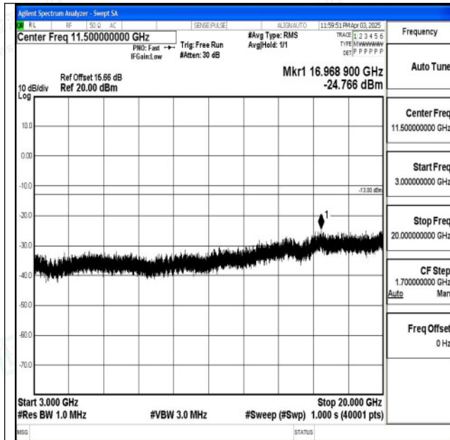
Band2_3MHz_QPSK_18900_1RB#0_3000~20000_3000 ~20000
