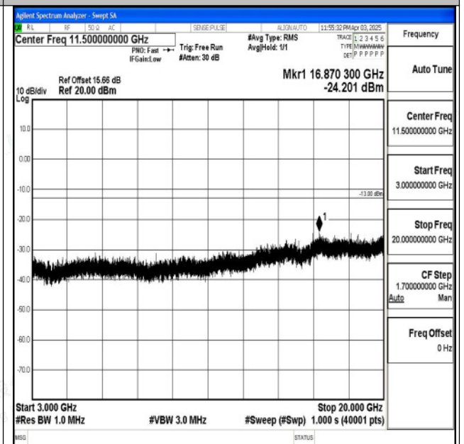
Band2_1.4MHz_16QAM_18900_1RB#0_3000~20000_3000~20000
