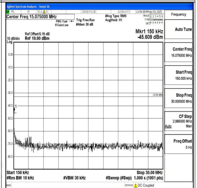
Band2_1.4MHz_QPSK_18900_1RB#0_0.15~30_0.15~30
