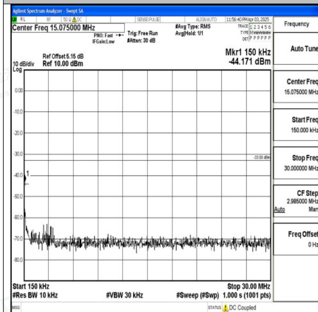
Band2_1.4MHz_16QAM_19193_1RB#0_0.15~30_0.15~ 30
