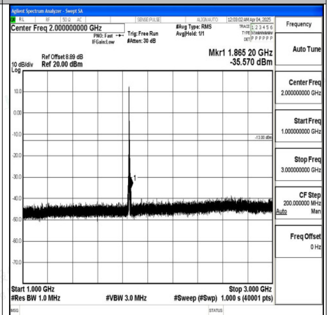
Band2_5MHz_QPSK_18625_1RB#0_1000~3000_1000~3000
