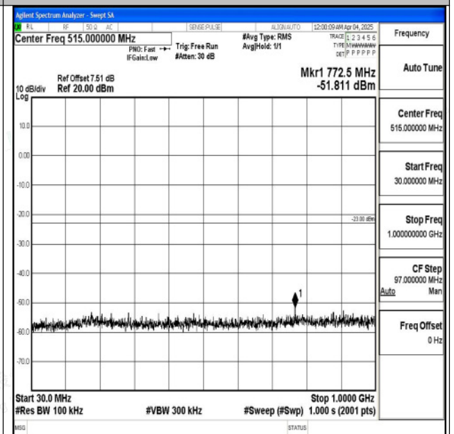
Band2_3MHz_16QAM_18900_1RB#0_30~1000_30~100 0
