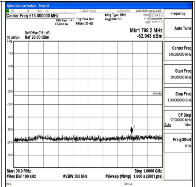
Band2_3MHz_16QAM_18615_1RB#0_30~1000_30~1000 0
