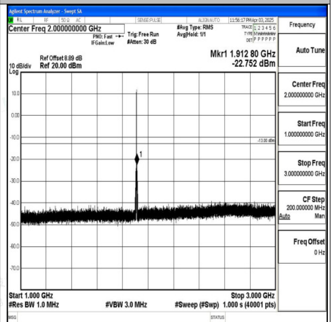
Band2_1.4MHz_QPSK_19193_1RB#0_1000~3000_1000 ~3000
