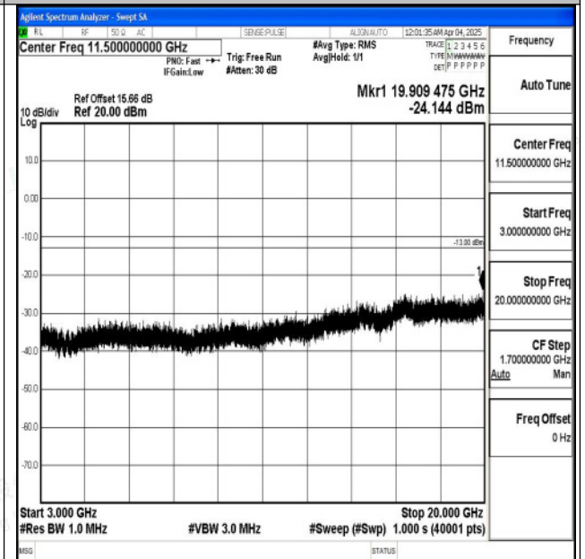
Band2_3MHz_16QAM_19185_1RB#0_3000~20000_3000 0~20000
