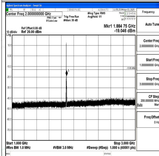
Band2_1.4MHz_16QAM_18900_1RB#0_1000~3000_1000~3000
