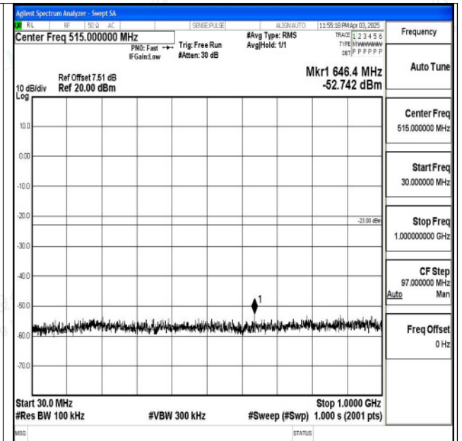
Band2_1.4MHz_16QAM_18900_1RB#0_30~1000_30~1000
