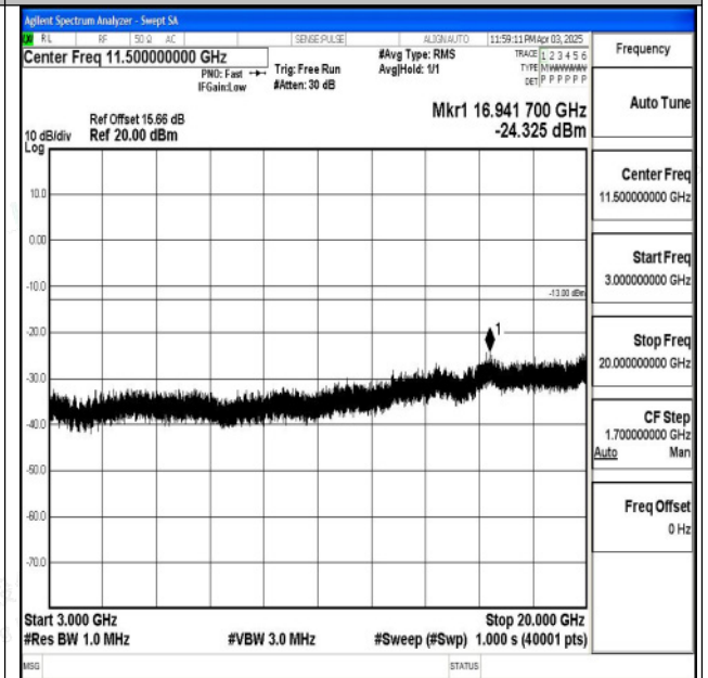
Band2_3MHz_16QAM_18615_1RB#0_3000~20000_3000 0~20000
