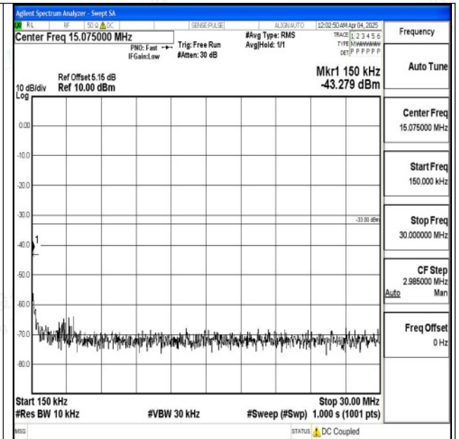
Band2_5MHz_QPSK_18625_1RB#0_0.15~30_0.15~30
