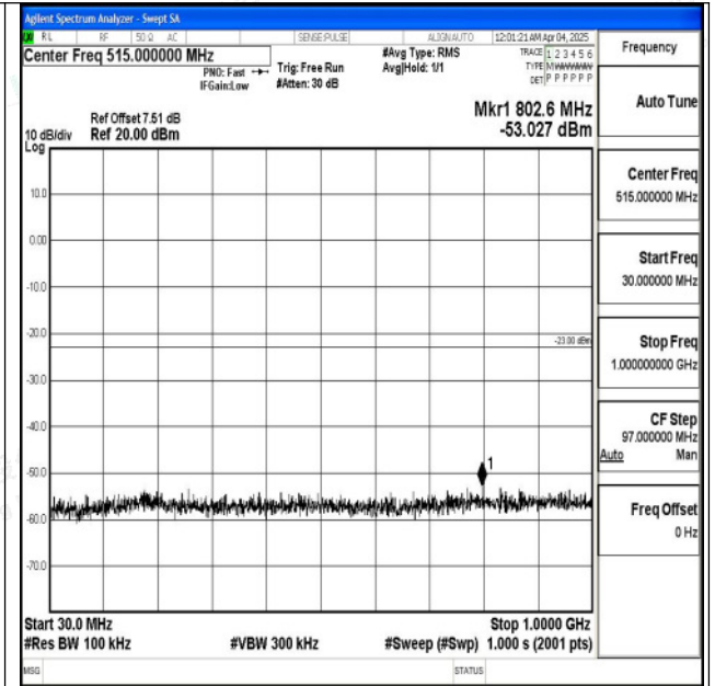
Band2_3MHz_16QAM_19185_1RB#0_30~1000_30~1000 0
