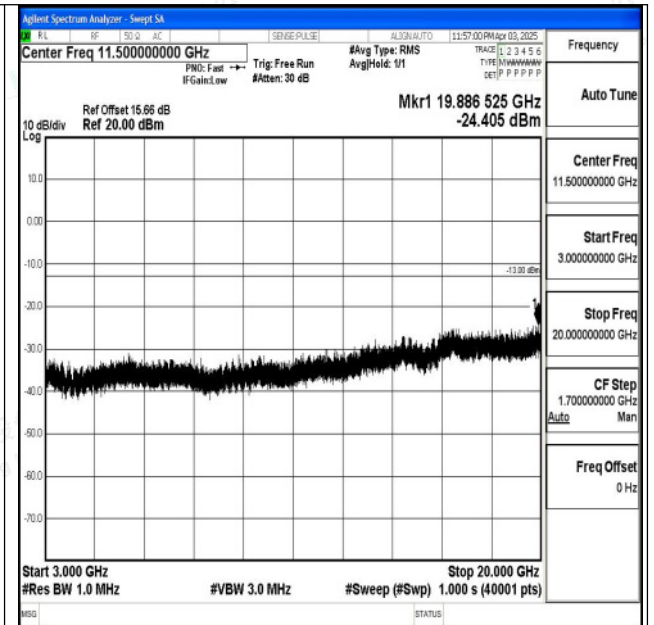
Band2_1.4MHz_16QAM_19193_1RB#0_3000~20000_3 000~20000
