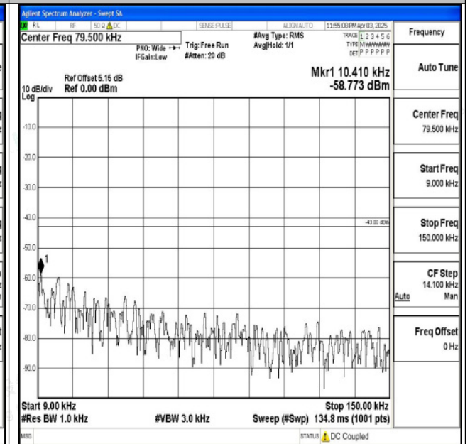
Band2_1.4MHz_16QAM_18900_1RB#0_0.009~0.15_0.0 09~0.15
