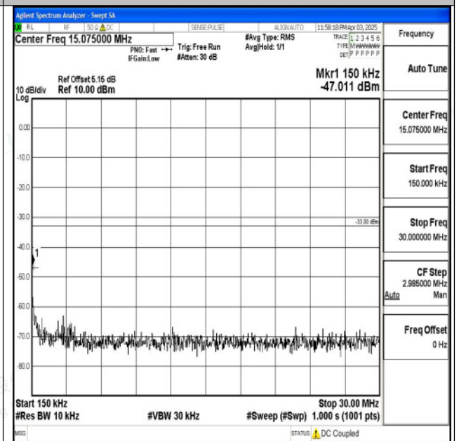
Band2_3MHz_QPSK_18615_1RB#0_0.15~30_0.15~30
