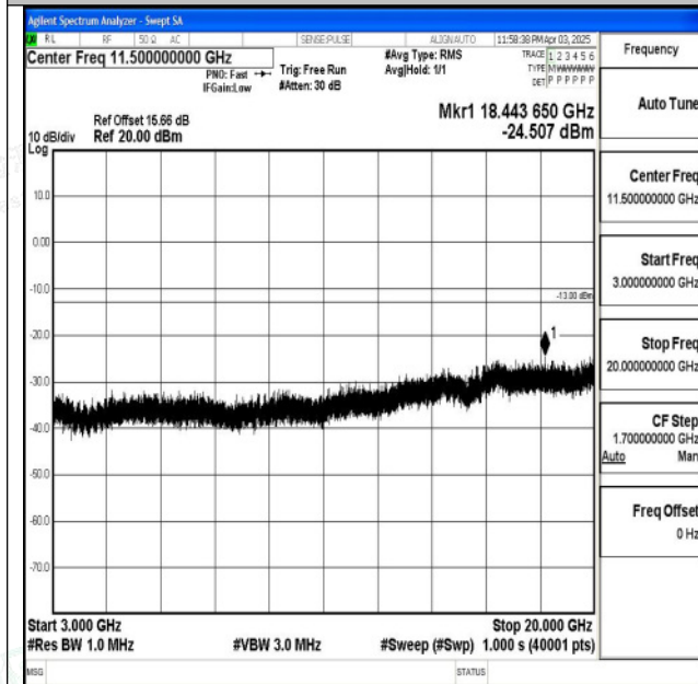
Band2_3MHz_QPSK_18615_1RB#0_3000~20000_3000~20000
