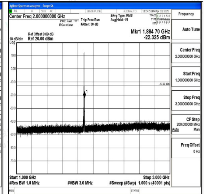
Band2_1.4MHz_QPSK_18900_1RB#0_1000~3000_1000 ~3000
