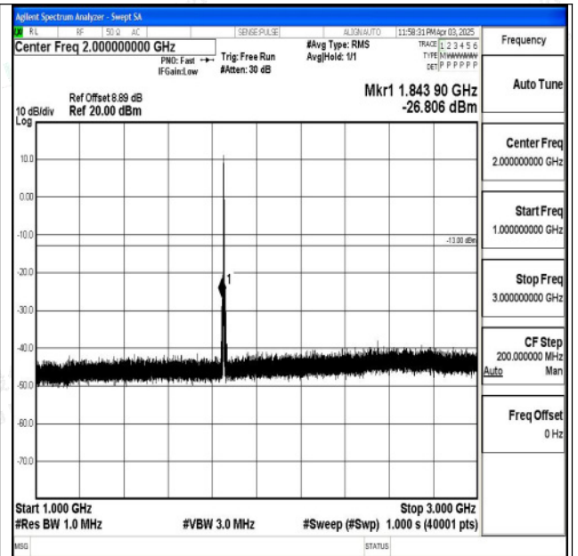
Band2_3MHz_QPSK_18615_1RB#0_1000~3000_1000~3000
