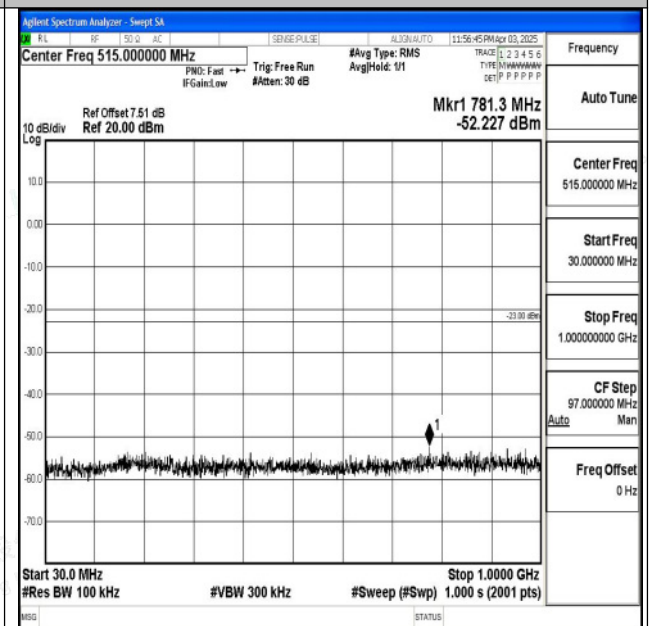
Band2_1.4MHz_16QAM_19193_1RB#0_30~1000_30~1 000
