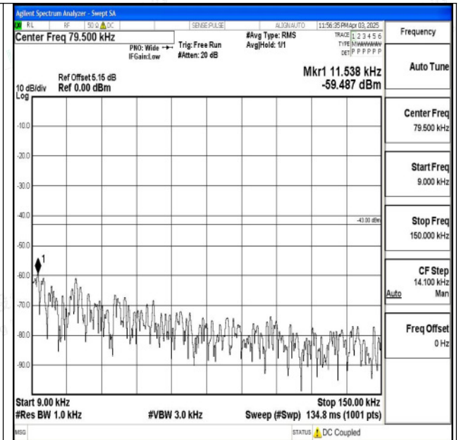
Band2_1.4MHz_16QAM_19193_1RB#0_0.009~0.15_0.0 09~0.15
