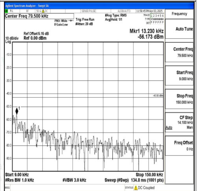
Band2_3MHz_16QAM_18615_1RB#0_0.009~0.15_0.009~0.15
