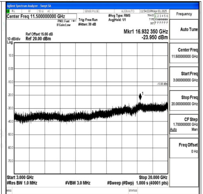
Band2_1.4MHz_16QAM_18607_1RB#0_3000~20000_3 000~20000
