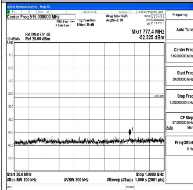
Band2_1.4MHz_QPSK_19193_1RB#0_30~1000_30~100 0
