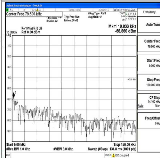
Band2_3MHz_QPSK_18615_1RB#0_0.009~0.15_0.009~ 0.15
