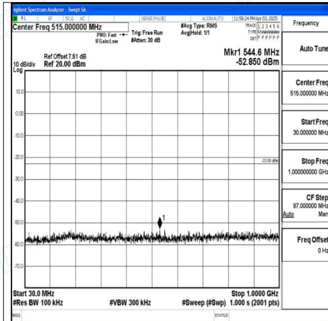
Band2_3MHz_QPSK_18615_1RB#0_30~1000_30~1000
