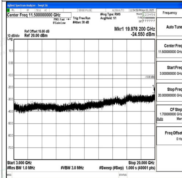
Band2_1.4MHz_QPSK_18900_1RB#0_3000~20000_300 0~20000
