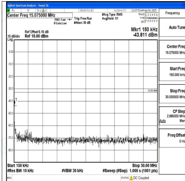
Band2_10MHz_16QAM_18650_1RB#0_0.15~30_0.15~3
