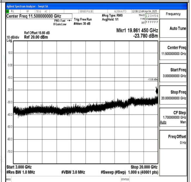
Band2_10MHz_16QAM_18650_1RB#0_3000~20000_30
