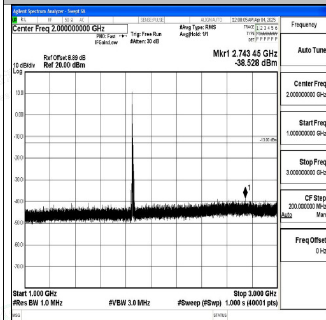
Band2_10MHz_16QAM_18650_1RB#0_1000~3000_100
