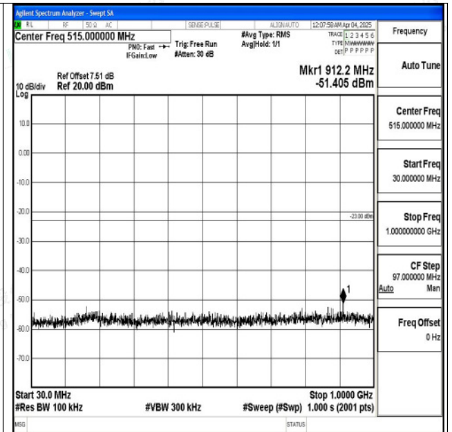
Band2_10MHz_16QAM_18650_1RB#0_30~1000_30~10
