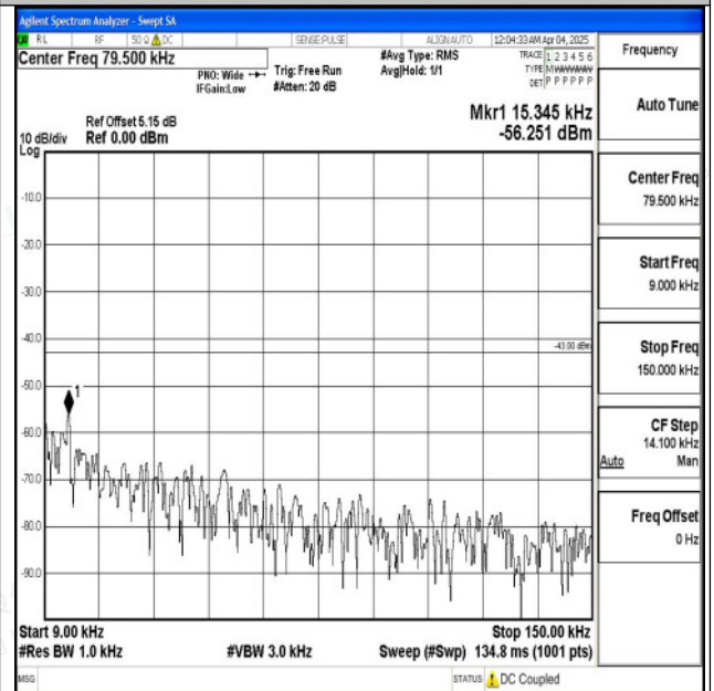
Band2_5MHz_16QAM_18900_1RB#0_0.009~0.15_0.00~0.15
