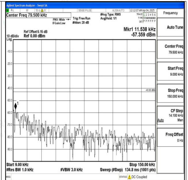
Band2_15MHz_16QAM_18675_1RB#0_0.009~0.15_0.0 09~0.15
