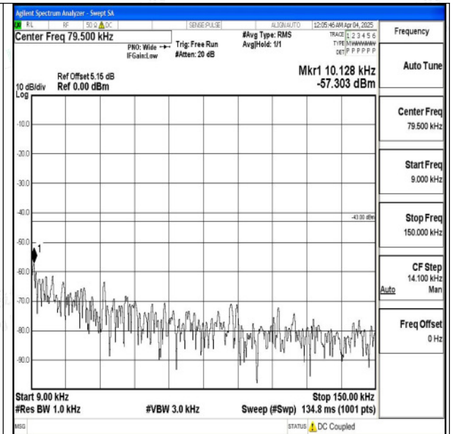
Band2_5MHz_16QAM_19175_1RB#0_0.009~0.15_0.00 9~0.15
