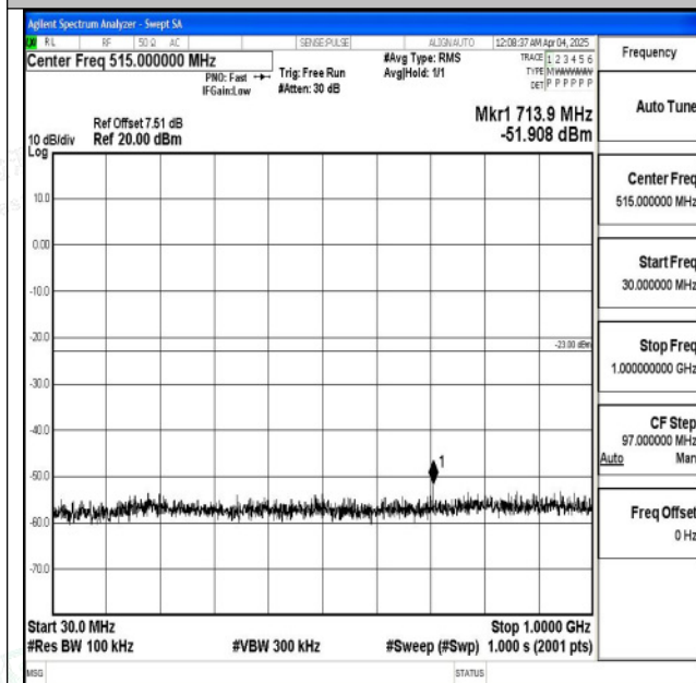
Band2_10MHz_QPSK_18900_1RB#0_30~1000_30~1000 0
