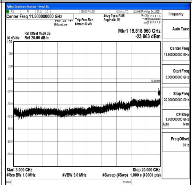
Band2_5MHz_16QAM_18900_1RB#0_3000~20000_3000 0~20000
