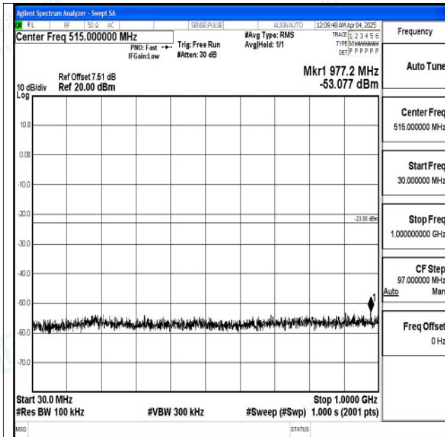
Band2_10MHz_QPSK_19150_1RB#0_30~1000_30~1000 0
