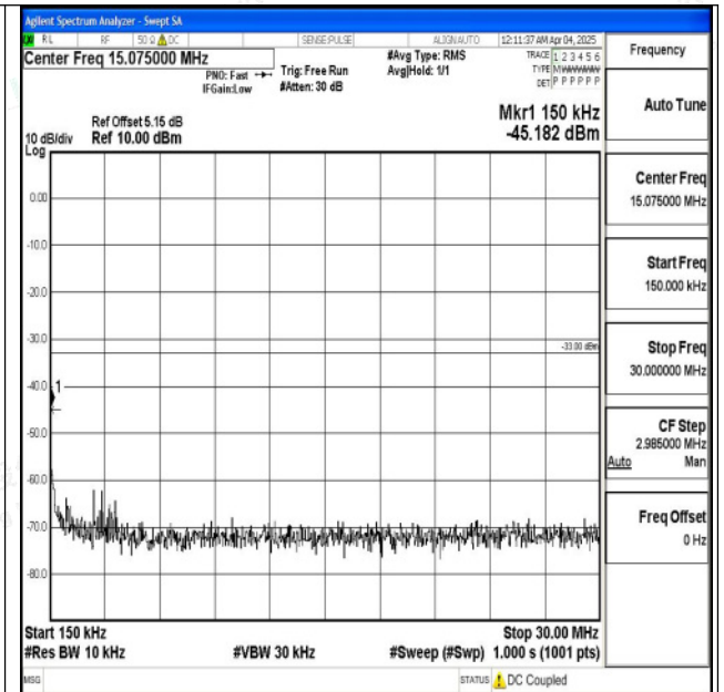
Band2_15MHz_QPSK_18675_1RB#0_0.15~30_0.15~30
