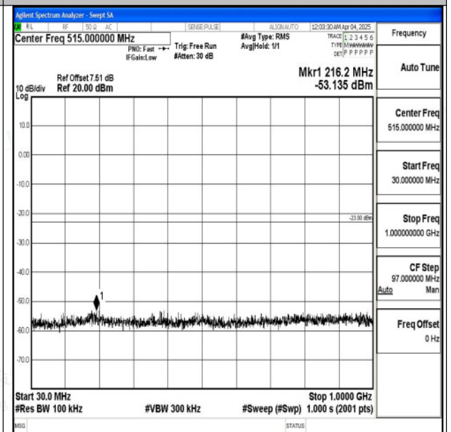
Band2_5MHz_16QAM_18625_1RB#0_30~1000_30~100 0
