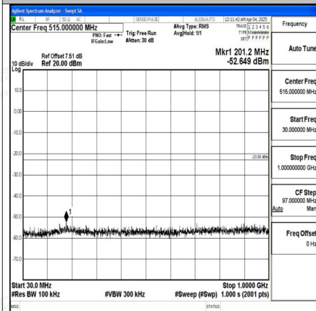
Band2_15MHz_QPSK_18675_1RB#0_30~1000_30~1000 0
