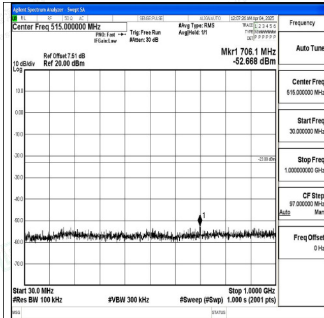
Band2_10MHz_QPSK_18650_1RB#0_30~1000_30~100 0
