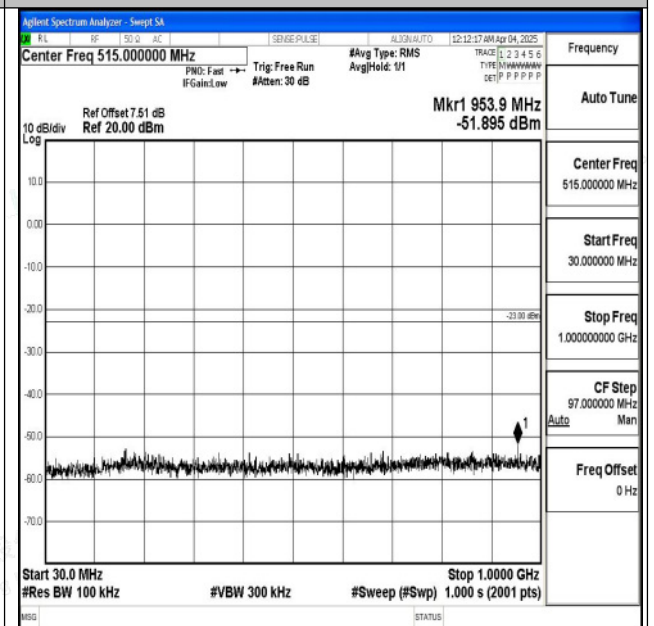
Band2_15MHz_16QAM_18675_1RB#0_30~1000_30~10 00
