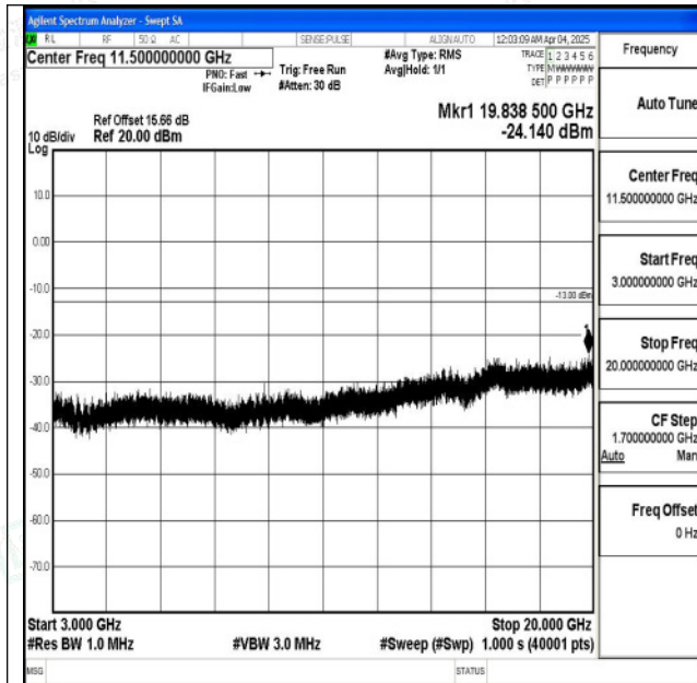
Band2_5MHz_QPSK_18625_1RB#0_3000~20000_3000 ~20000
