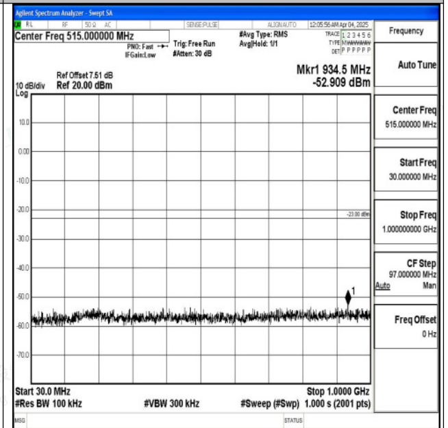
Band2_5MHz_16QAM_19175_1RB#0_30~1000_30~1000 0
