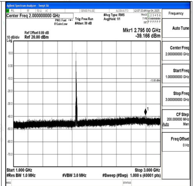
Band2_10MHz_QPSK_18650_1RB#0_1000~3000_1000 ~3000
