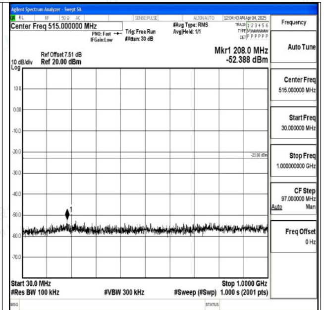
Band2_5MHz_16QAM_18900_1RB#0_30~1000_30~1000 0
