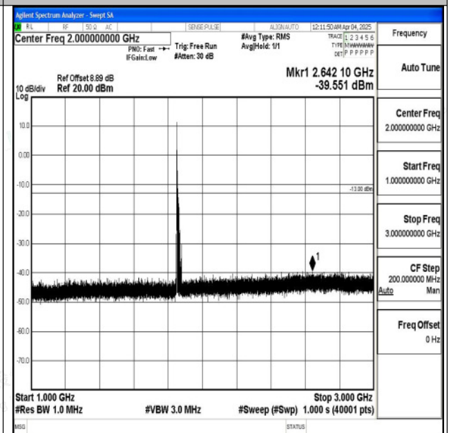
Band2_15MHz_QPSK_18675_1RB#0_1000~3000_1000~3000
