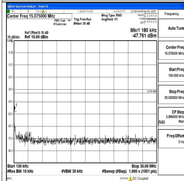
Band2_10MHz_16QAM_18900_1RB#0_0.15~30_0.15~3 0
