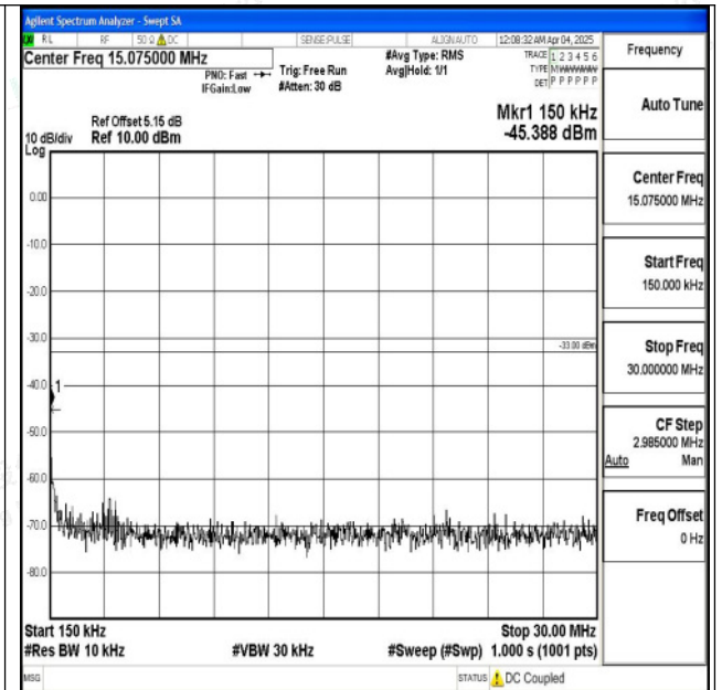
Band2_10MHz_QPSK_18900_1RB#0_0.15~30_0.15~30
