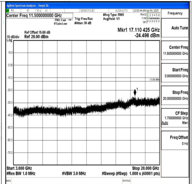
Band2_5MHz_16QAM_18625_1RB#0_3000~20000_300 0~20000
