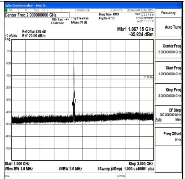
Band2_5MHz_QPSK_18900_1RB#0_1000~3000_1000~3000
