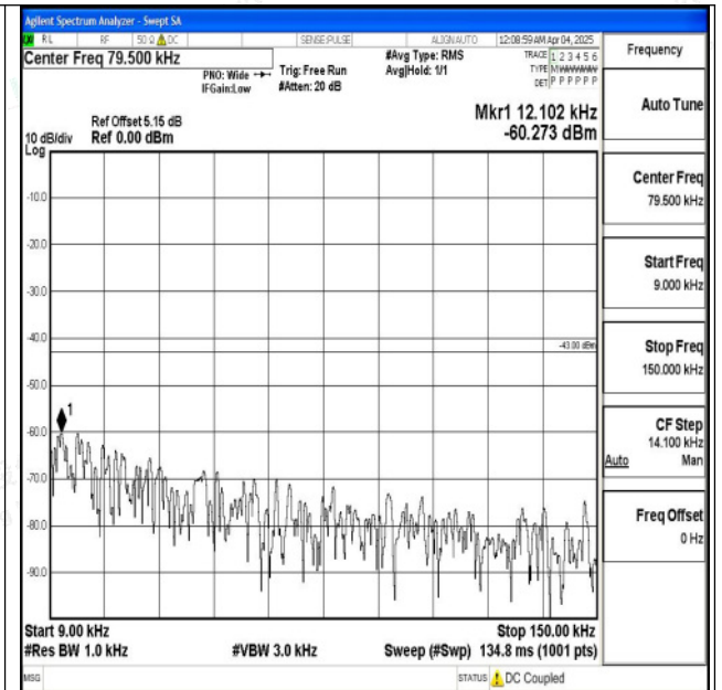
Band2_10MHz_16QAM_18900_1RB#0_0.009~0.15_0.0 09~0.15
