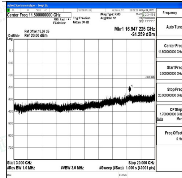
Band2_10MHz_QPSK_18900_1RB#0_3000~20000_300 0~20000
