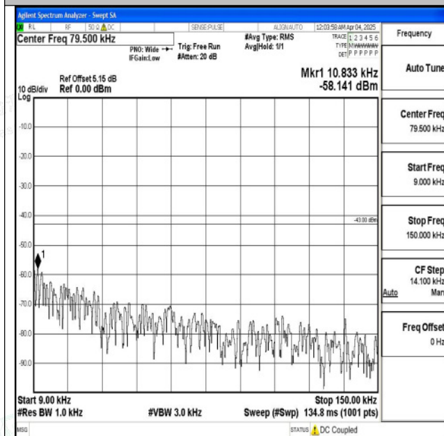
Band2_5MHz_QPSK_18900_1RB#0_0.009~0.15_0.009~ 0.15
