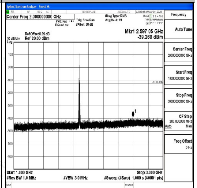
Band2_10MHz_QPSK_18900_1RB#0_1000~3000_1000~3000
