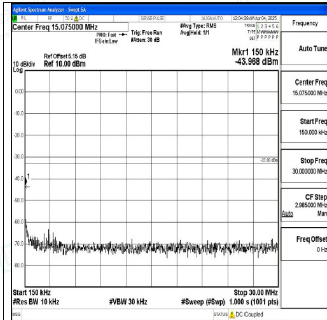
Band2_5MHz_16QAM_18900_1RB#0_0.15~30_0.15~30
