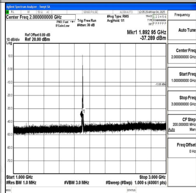
Band2_5MHz_QPSK_19175_1RB#0_1000~3000_1000~3000
