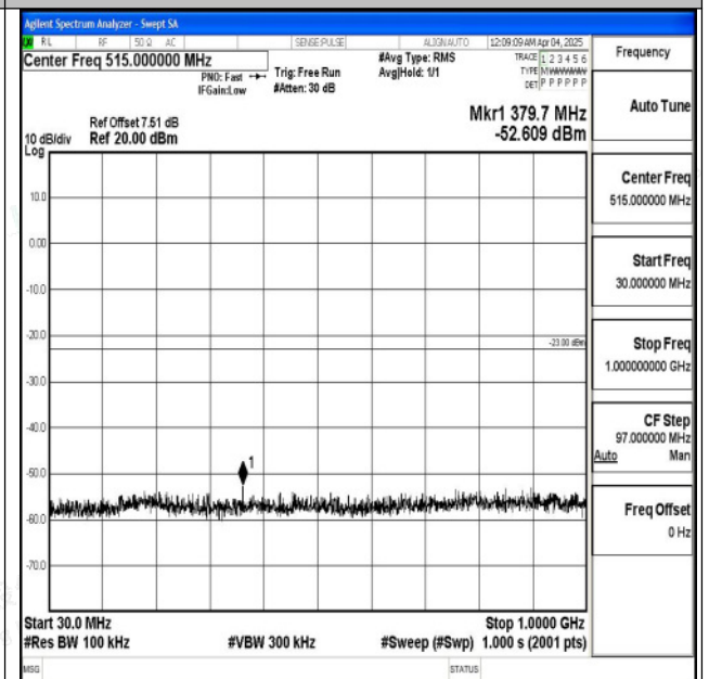
Band2_10MHz_16QAM_18900_1RB#0_30~1000_30~10 00
