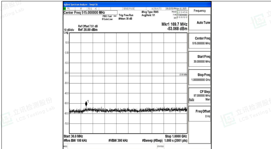
Band4_3MHz_QPSK_20175_1RB#0_30~1000_30~1000
