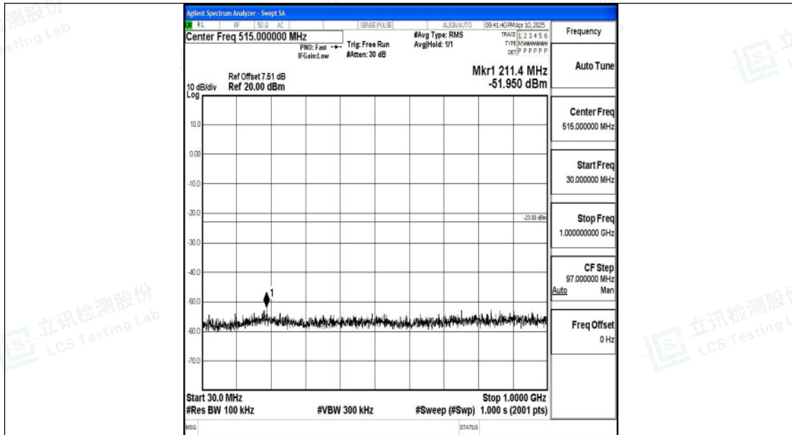
Band4_5MHz_QPSK_19975_1RB#0_30~1000_30~1000
