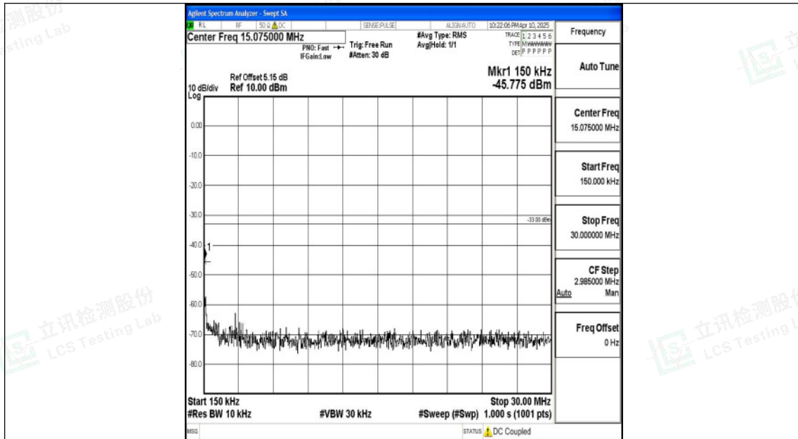
Band4_15MHz_16QAM_20025_1RB#0_0.15~30_0.15~30
