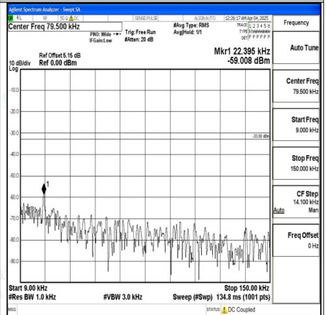
Band5_3MHz_16QAM_20415_1RB#0_0.009~0.15_0.009~0.15
