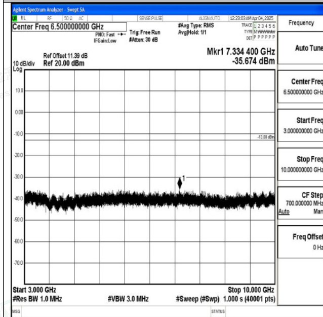
Band5_1.4MHz_QPSK_20525_1RB#0_3000~10000_300~10000 0~10000
