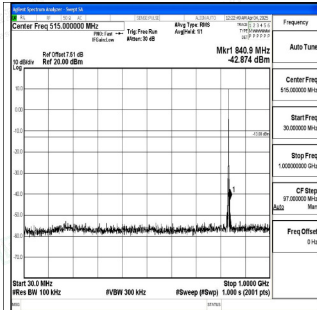
Band5_1.4MHz_QPSK_20525_1RB#0_30~1000_30~1000 0
