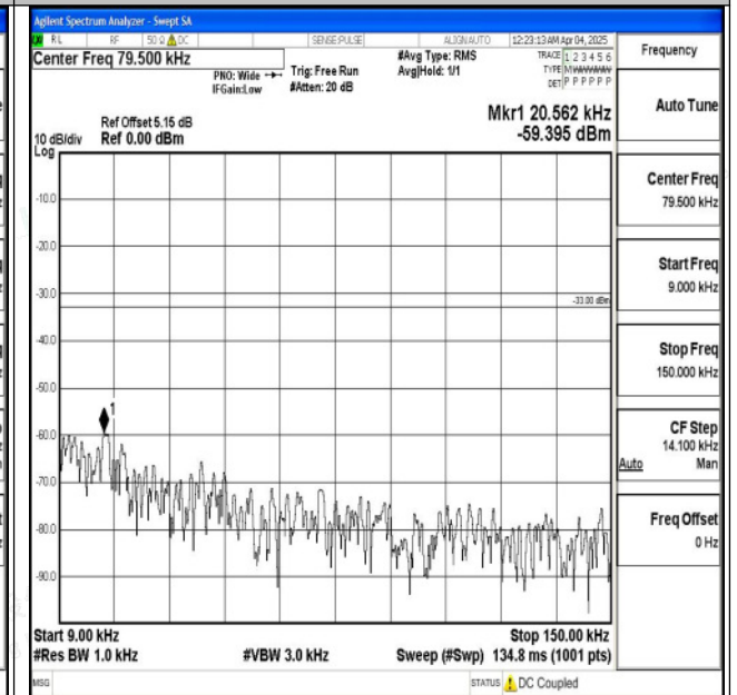
Band5_1.4MHz_16QAM_20525_1RB#0_0.009~0.15_0.09~0.15 09~0.15
