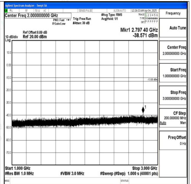
Band5_3MHz_QPSK_20415_1RB#0_1000~3000_1000~3000
