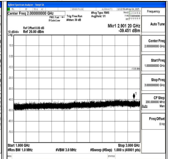
Band5_1.4MHz_QPSK_20525_1RB#0_1000~3000_1000~3000 ~3000
