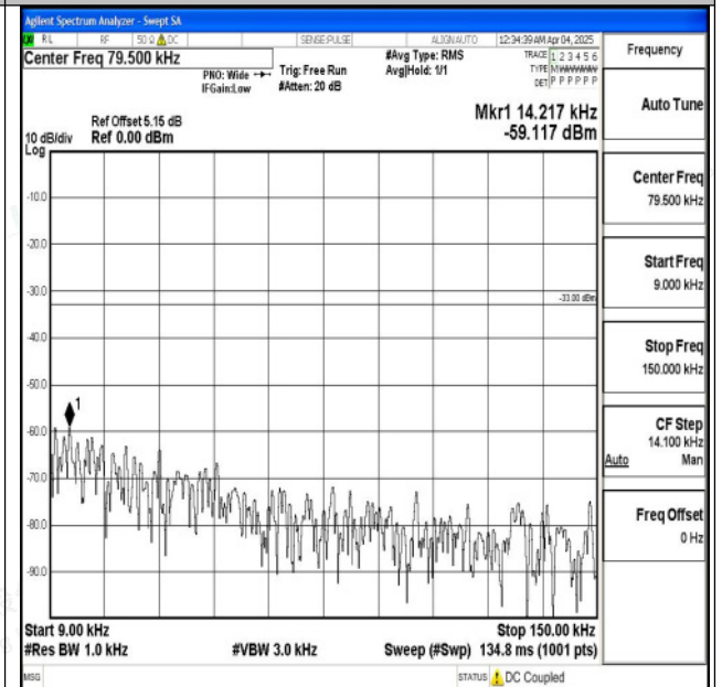
Band5_10MHz_16QAM_20450_1RB#0_0.009~0.15_0.0 09~0.15
