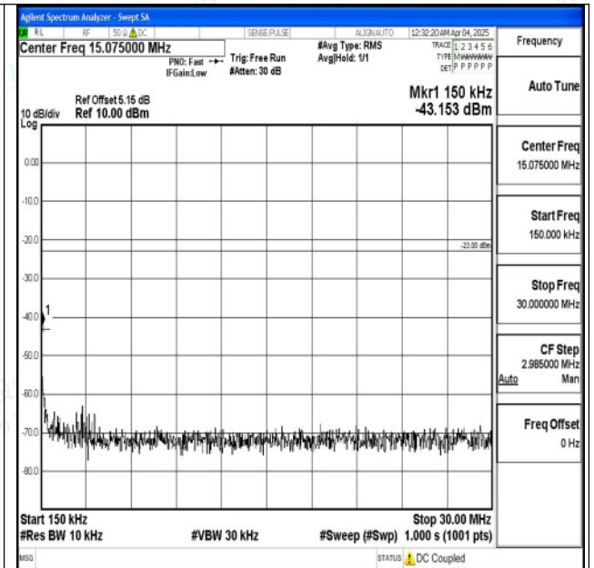
Band5_5MHz_QPSK_20625_1RB#0_0.15~30_0.15~30
