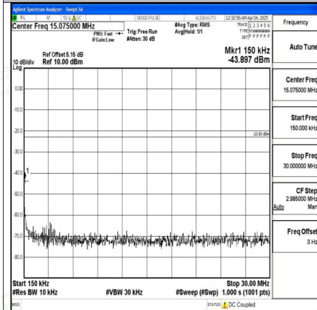
Band5_5MHz_16QAM_20625_1RB#0_0.15~30_0.15~30
