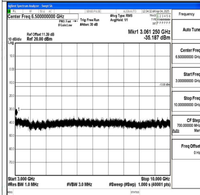
Band5_10MHz_QPSK_20450_1RB#0_3000~10000_300 0~10000
