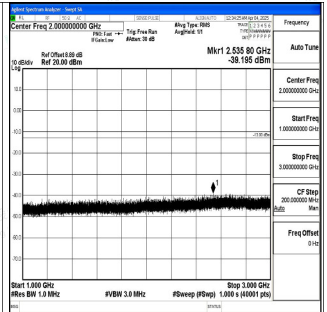
Band5_10MHz_QPSK_20450_1RB#0_1000~3000_1000 ~3000
