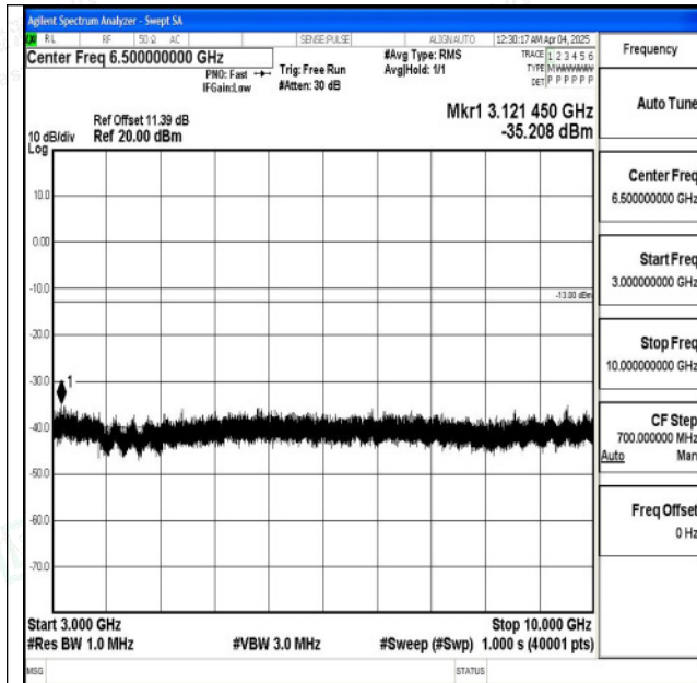
Band5_5MHz_QPSK_20425_1RB#0_3000~10000_3000~10000
