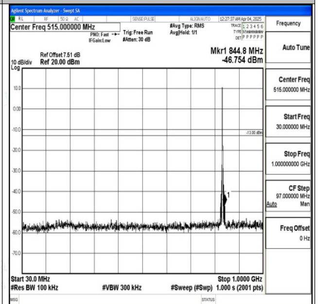
Band5_3MHz_16QAM_20525_1RB#0_30~1000_30~100 0
