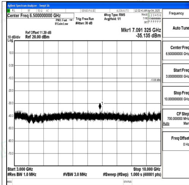
Band5_5MHz_QPSK_20625_1RB#0_3000~10000_3000~10000
