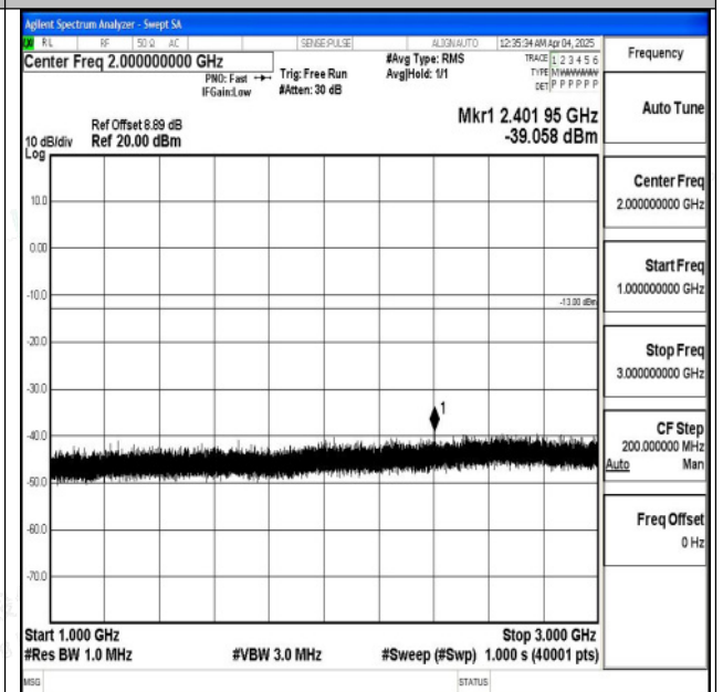
Band5_10MHz_QPSK_20525_1RB#0_1000~3000_1000~3000
