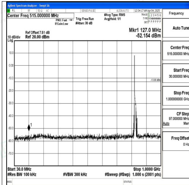
Band5_10MHz_QPSK_20450_1RB#0_30~1000_30~1000 0
