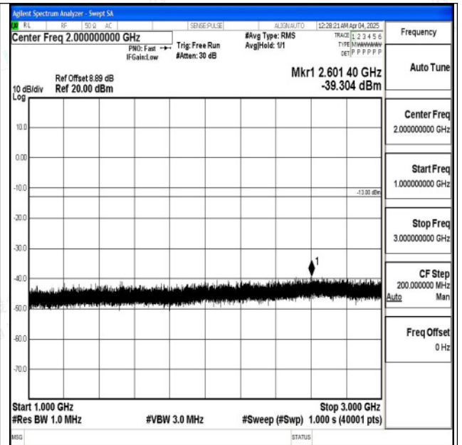
Band5_3MHz_QPSK_20635_1RB#0_1000~3000_1000~3000
