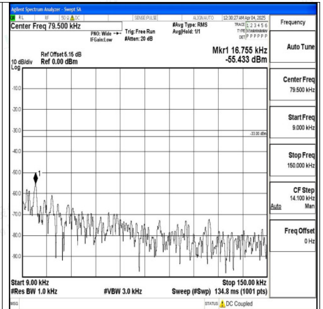
Band5_5MHz_16QAM_20425_1RB#0_0.009~0.15_0.009~0.15
