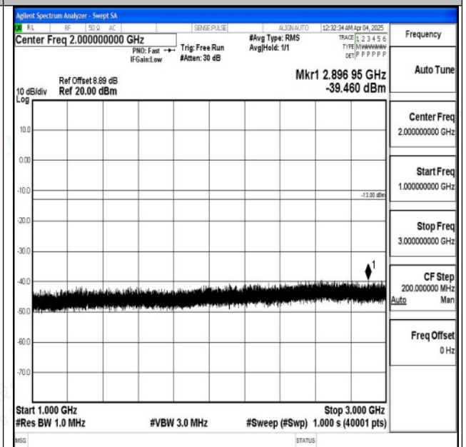
Band5_5MHz_QPSK_20625_1RB#0_1000~3000_1000~3000
