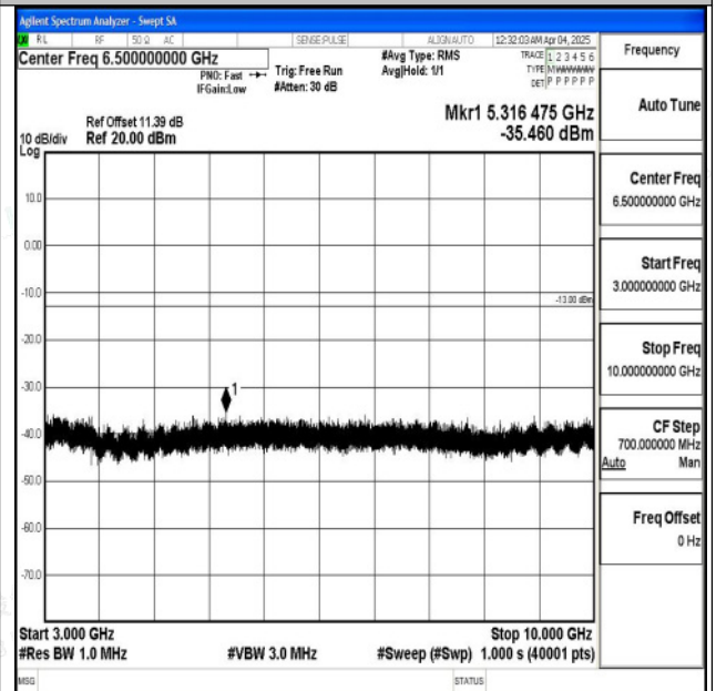
Band5_5MHz_16QAM_20525_1RB#0_3000~10000_3000 0~10000
