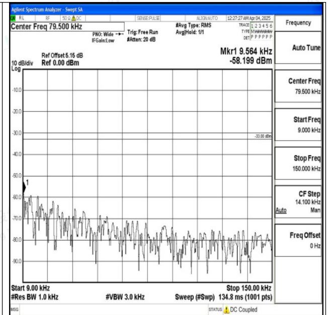
Band5_3MHz_16QAM_20525_1RB#0_0.009~0.15_0.00 9~0.15
