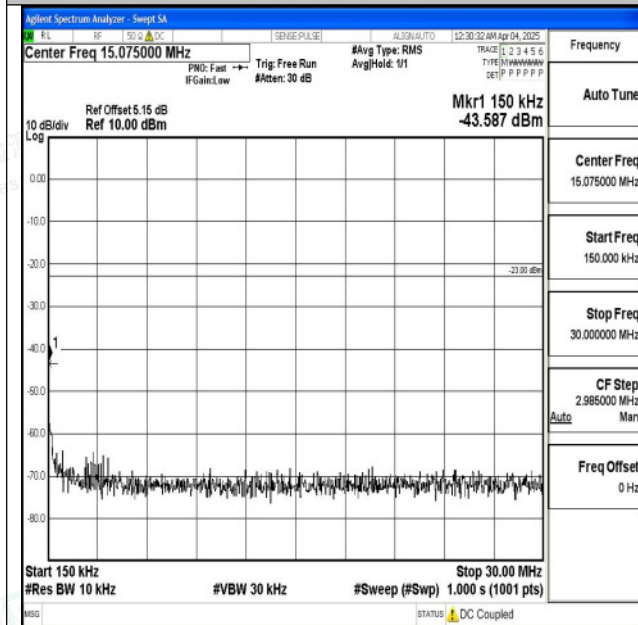
Band5_5MHz_16QAM_20425_1RB#0_0.15~30_0.15~30
