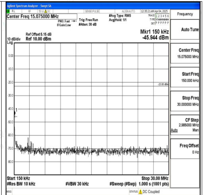
Band5_10MHz_QPSK_20525_1RB#0_0.15~30_0.15~30
