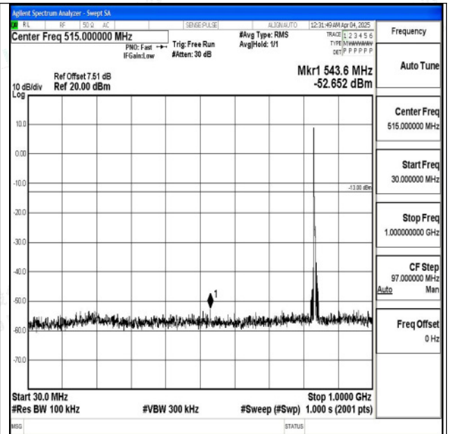
Band5_5MHz_16QAM_20525_1RB#0_30~1000_30~1000 0
