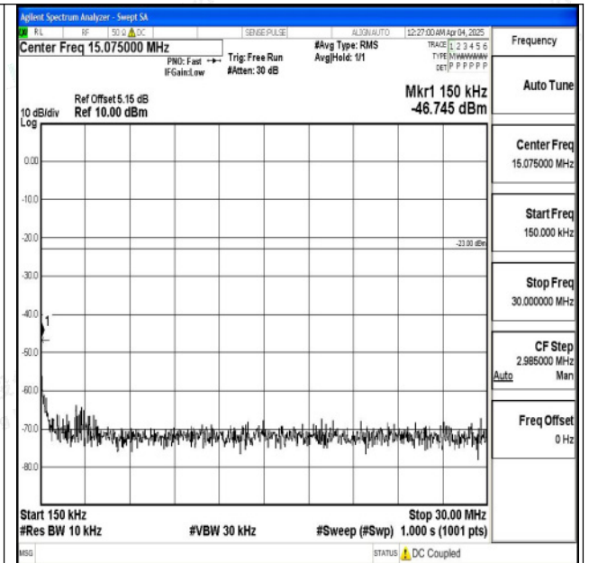
Band5_3MHz_QPSK_20525_1RB#0_0.15~30_0.15~30
