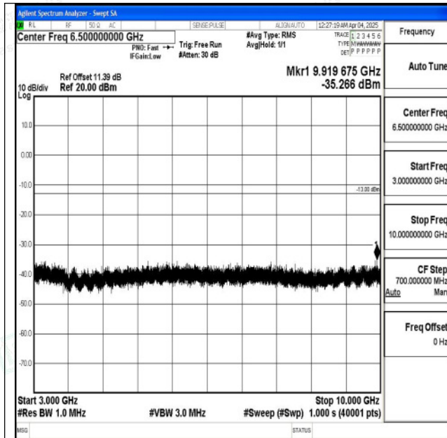
Band5_3MHz_QPSK_20525_1RB#0_3000~10000_3000 ~10000
