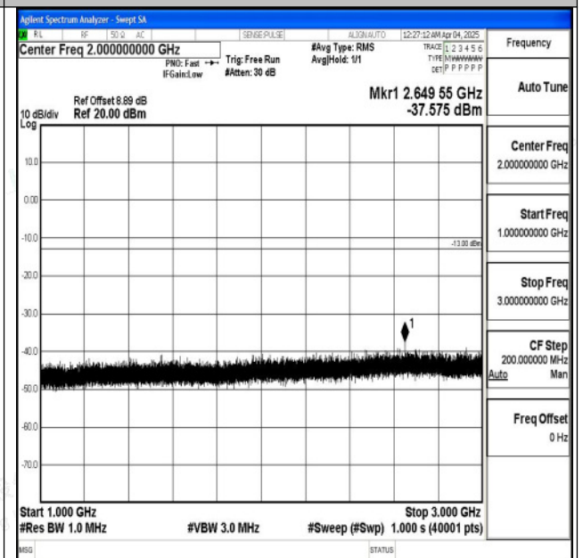
Band5_3MHz_QPSK_20525_1RB#0_1000~3000_1000~3000
