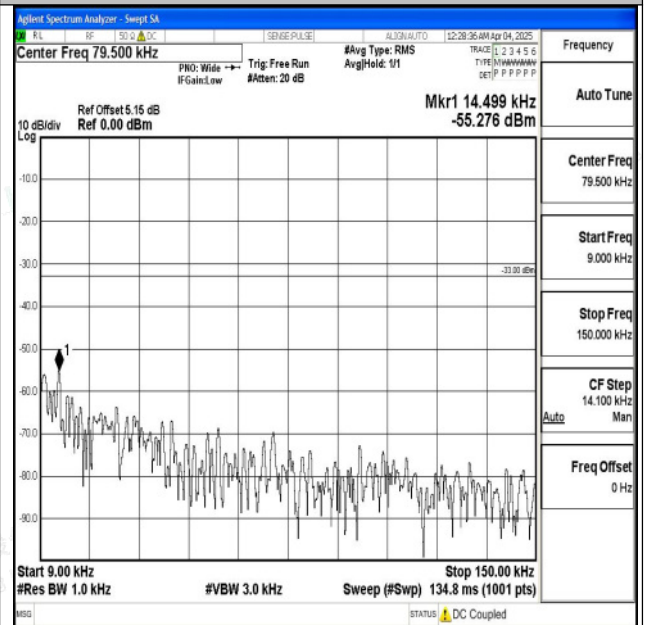
Band5_3MHz_16QAM_20635_1RB#0_0.009~0.15_0.009~0.15
