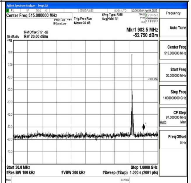
Band5_5MHz_16QAM_20425_1RB#0_30~1000_30~1000
