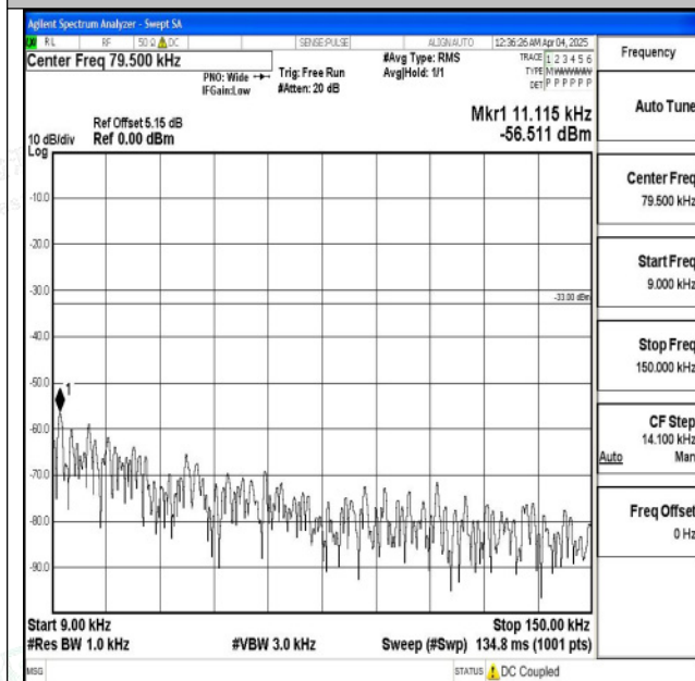
Band5_10MHz_QPSK_20600_1RB#0_0.009~0.15_0.009 ~0.15
