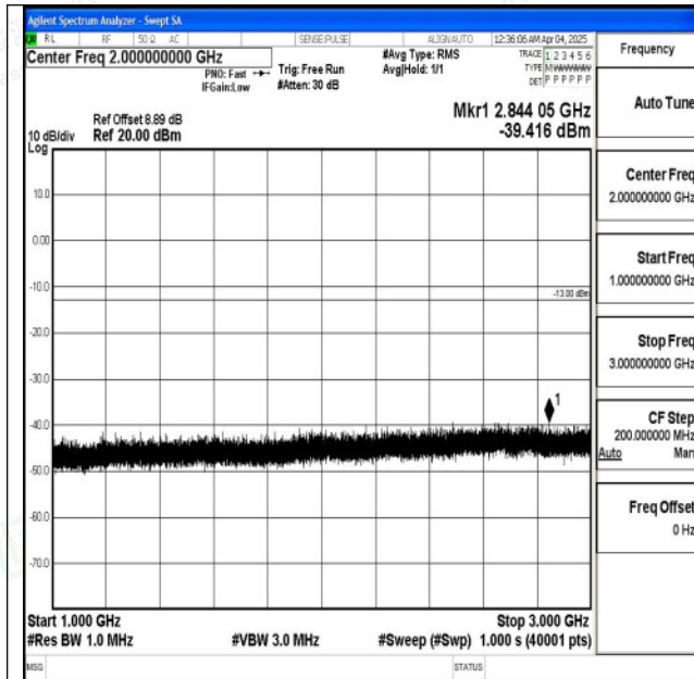
Band5_10MHz_16QAM_20525_1RB#0_1000~3000_100 0~3000
