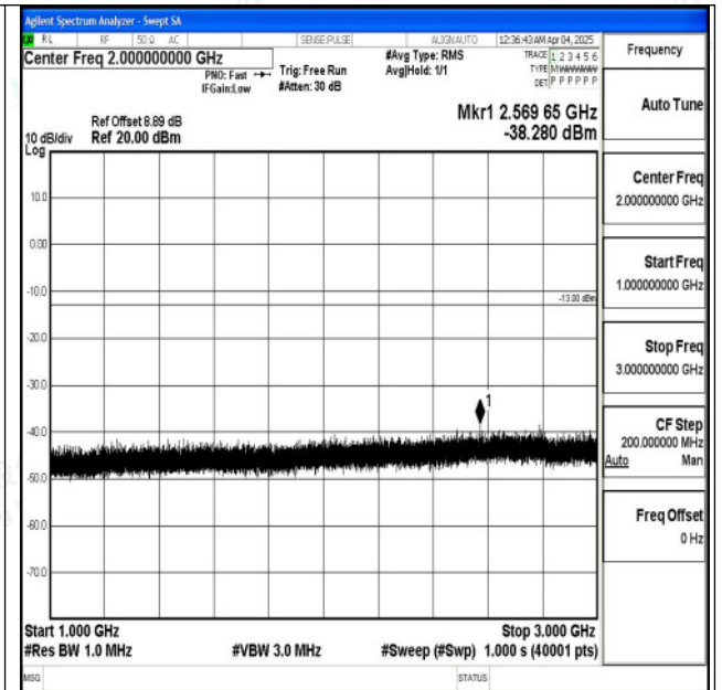
Band5_10MHz_QPSK_20600_1RB#0_1000~3000_1000 ~3000
