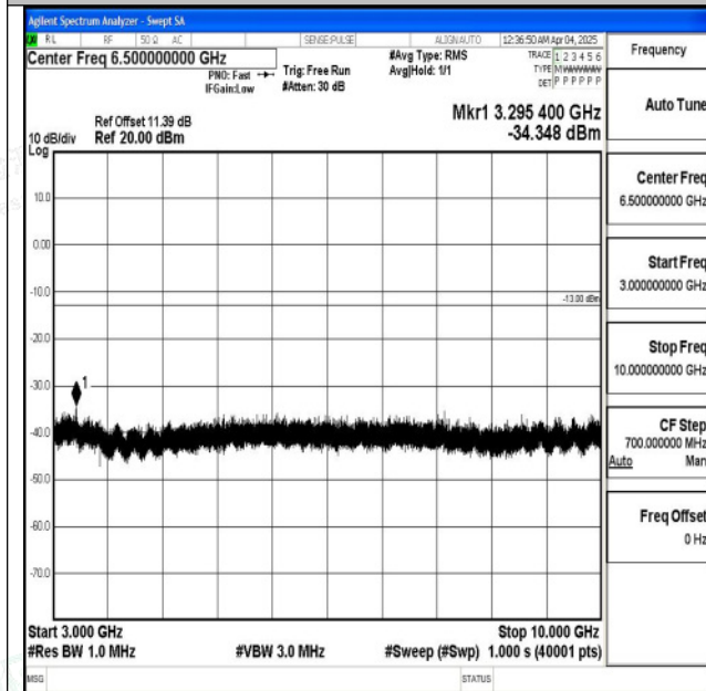
Band5_10MHz_QPSK_20600_1RB#0_3000~10000_300 0~10000
