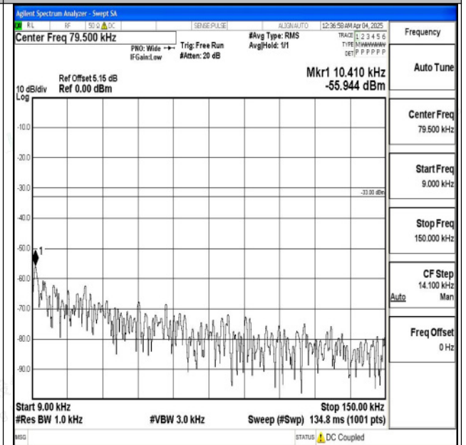
Band5_10MHz_16QAM_20600_1RB#0_0.009~0.15_0.0 09~0.15
