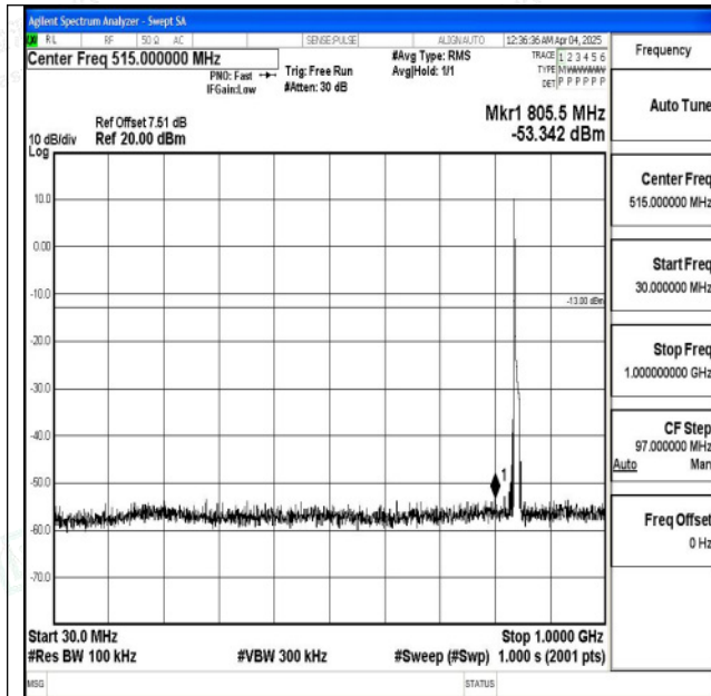
Band5_10MHz_QPSK_20600_1RB#0_30~1000_30~1000 0
