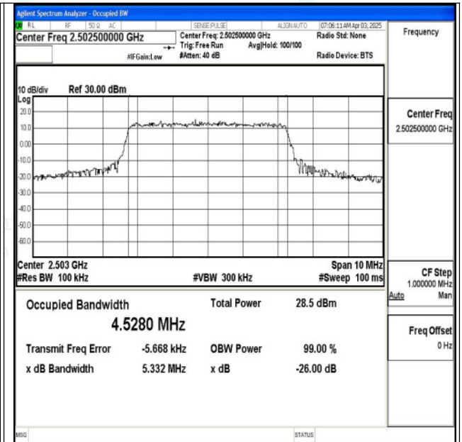
Band7-5MHz-16QAM-20775-25RB#0-PASS
