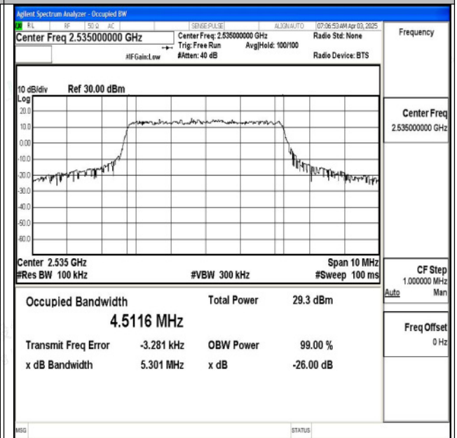
Band7-5MHz-16QAM-21100-25RB#0-PASS
