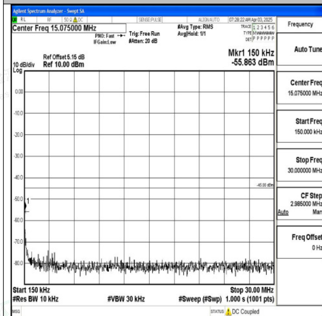
Band7_10MHz_16QAM_21400_1RB#0_0.15~30_0.15~30
