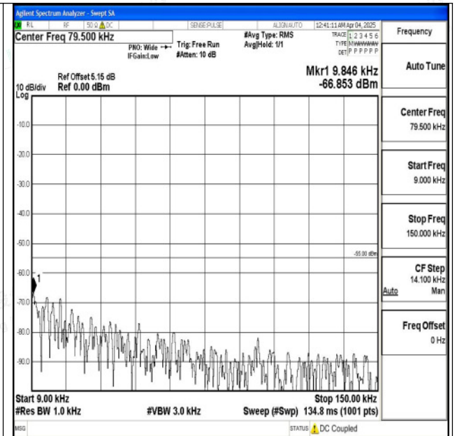
Band7_5MHz_16QAM_21100_1RB#0_0.009~0.15_0.009~0.15
