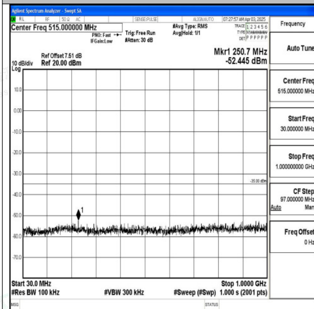
Band7_10MHz_QPSK_21400_1RB#0_30~1000_30~1000
