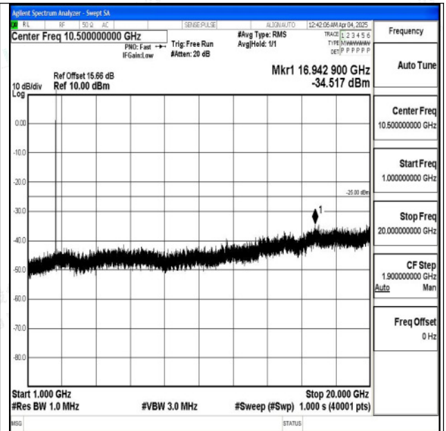
Band7_5MHz_QPSK_21425_1RB#0_1000~20000_1000~20000
