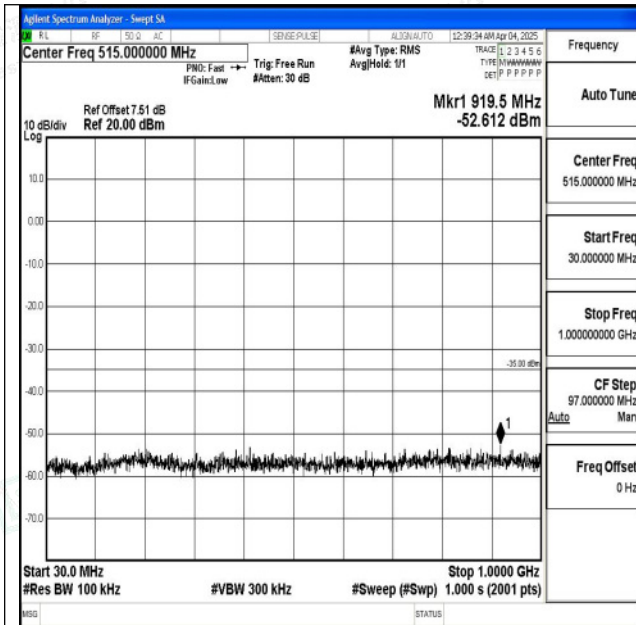
Band7_5MHz_QPSK_20775_1RB#0_30~1000_30~1000
