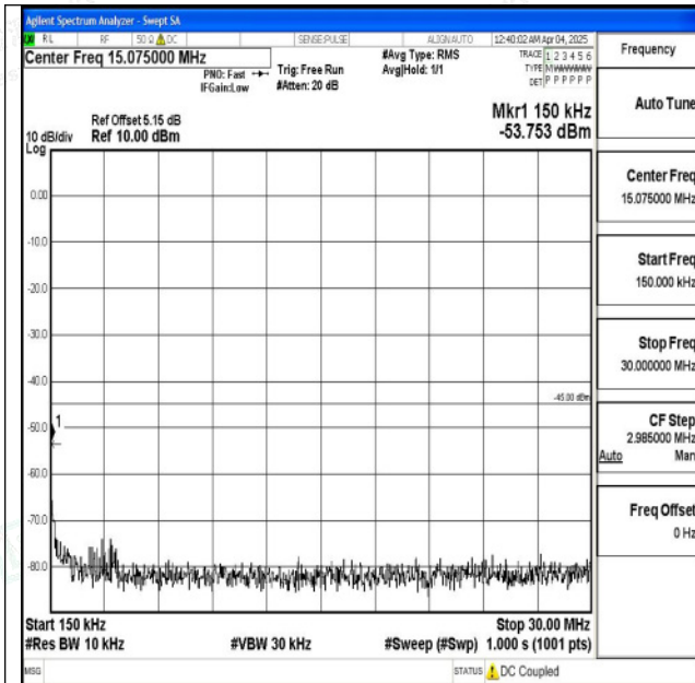
Band7_5MHz_16QAM_20775_1RB#0_0.15~30_0.15~30
