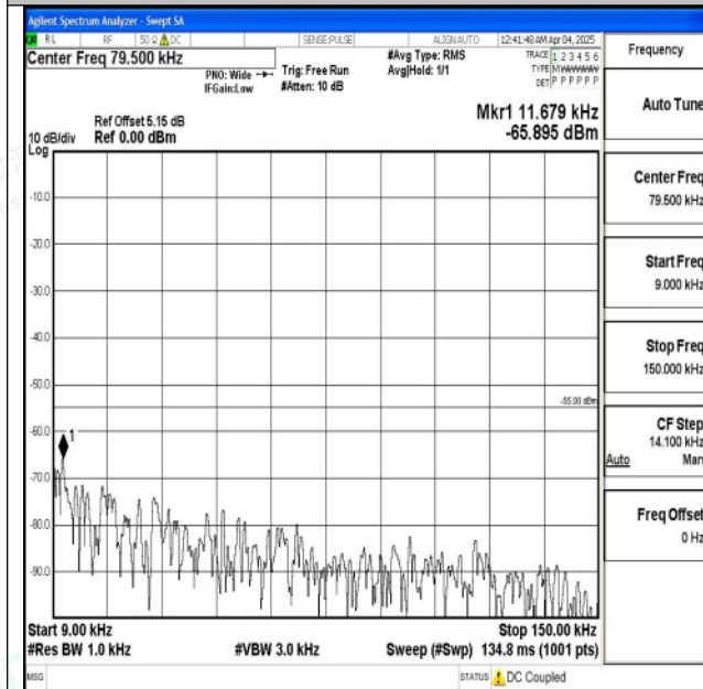
Band7_5MHz_QPSK_21425_1RB#0_0.009~0.15_0.009~ 0.15
