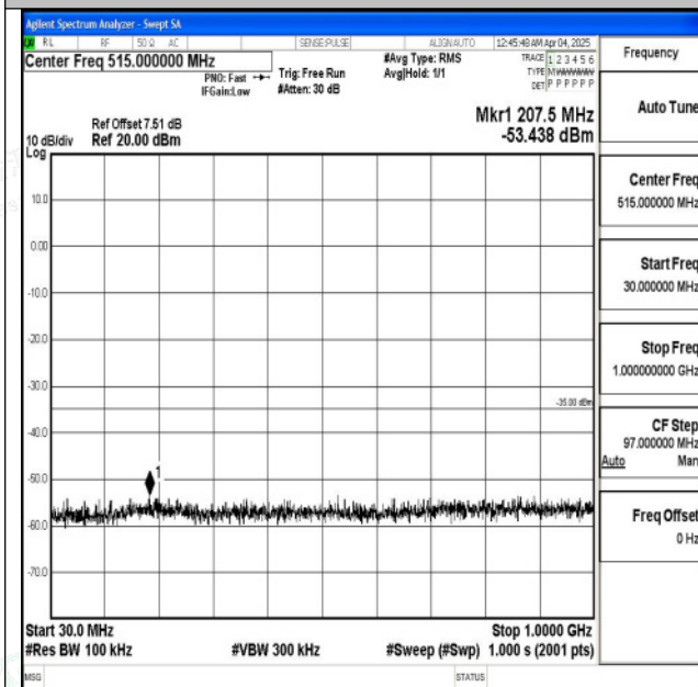
Band7_15MHz_QPSK_20825_1RB#0_30~1000_30~1000
