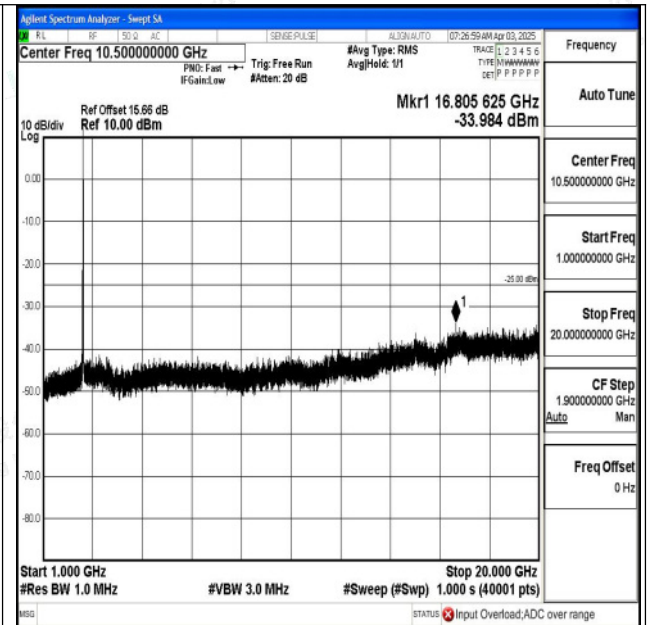
Band7_10MHz_QPSK_21100_1RB#0_1000~20000_1000~20000 0~20000
