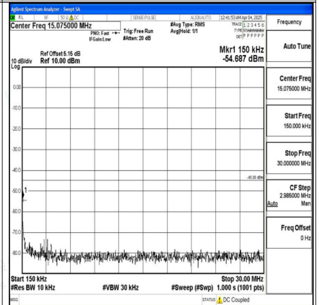
Band7_5MHz_QPSK_21425_1RB#0_0.15~30_0.15~30
