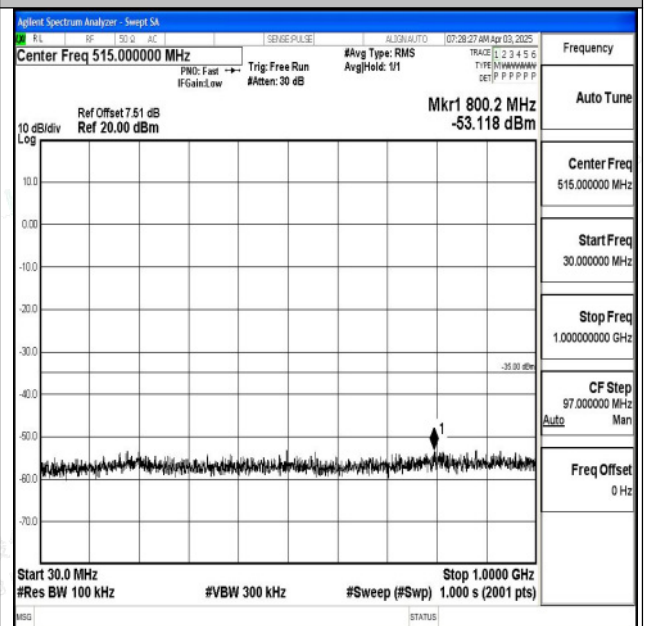
Band7_10MHz_16QAM_21400_1RB#0_30~1000_30~1000
