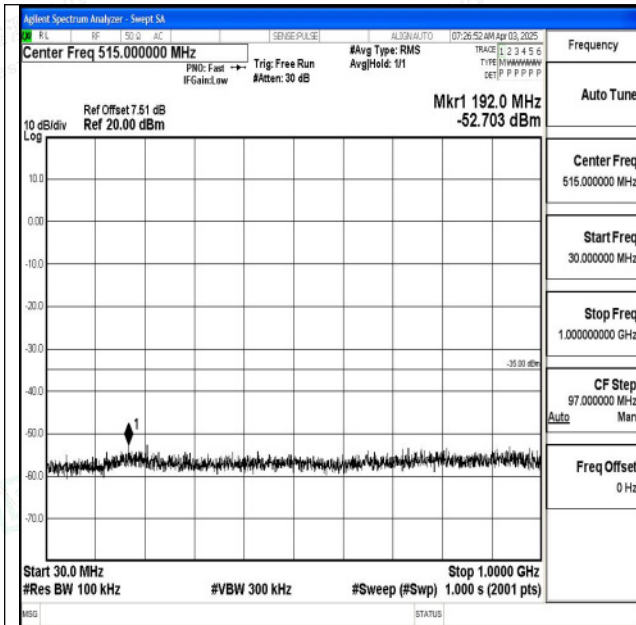
Band7_10MHz_QPSK_21100_1RB#0_30~1000_30~1000 0
