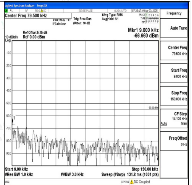
Band7_10MHz_16QAM_21400_1RB#0_0.009~0.15_0.009~0.15
