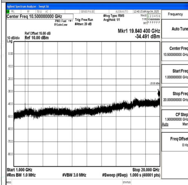
Band7_5MHz_16QAM_20775_1RB#0_1000~20000_1000~20000
