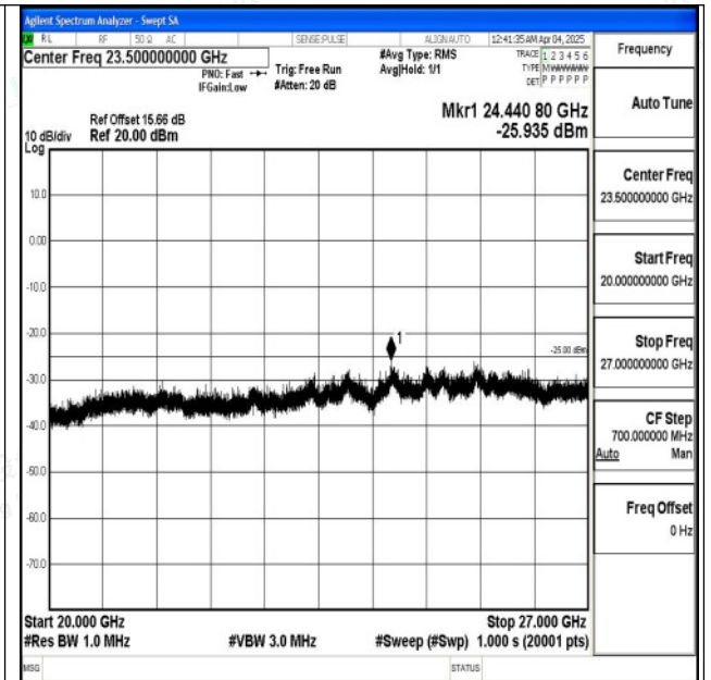
Band7_5MHz_16QAM_21100_1RB#0_20000~27000_20 000~27000
