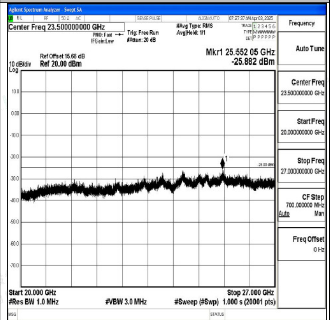
Band7_10MHz_16QAM_21100_1RB#0_20000~27000_2 0000~27000
