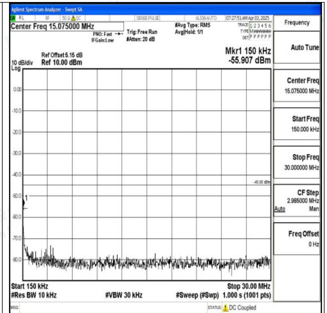
Band7_10MHz_QPSK_21400_1RB#0_0.15~30_0.15~30
