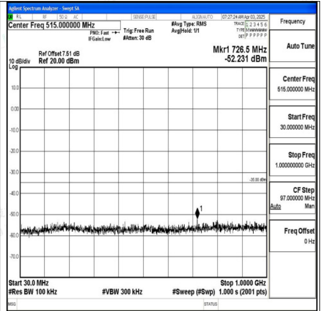
Band7_10MHz_16QAM_21100_1RB#0_30~1000_30~10 00
