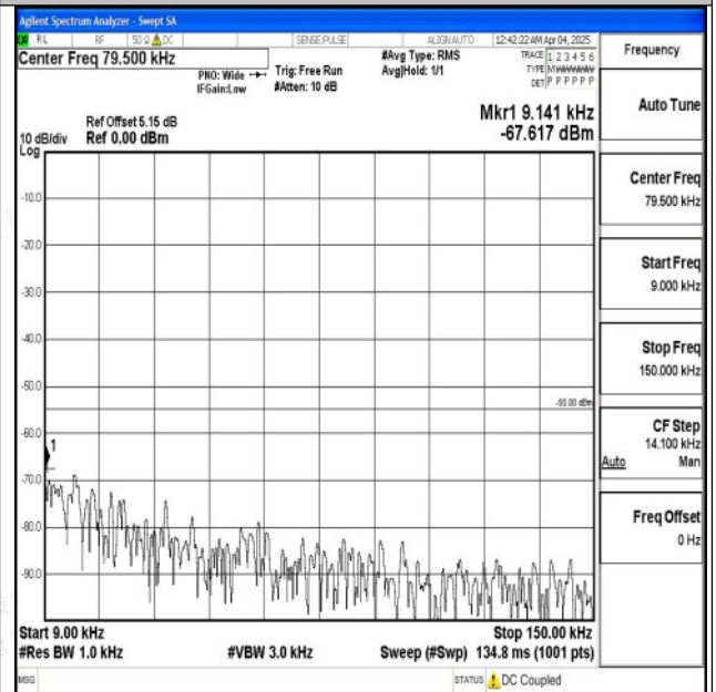
Band7_5MHz_16QAM_21425_1RB#0_0.009~0.15_0.009~0.15
