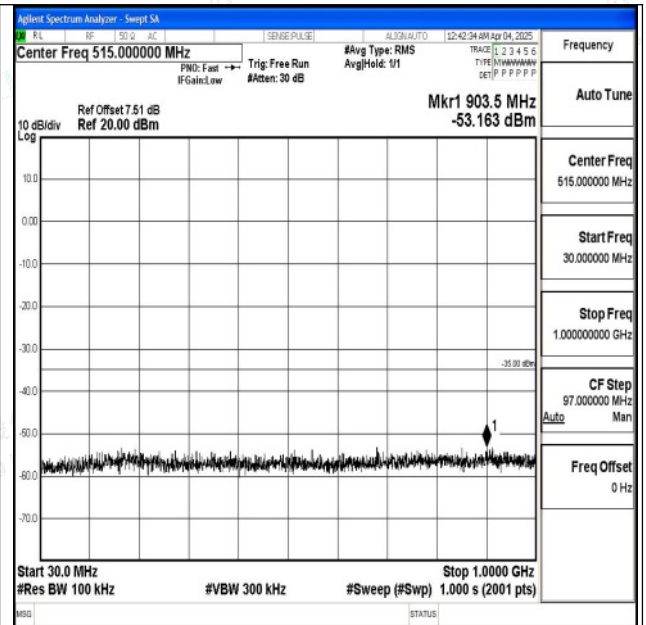
Band7_5MHz_16QAM_21425_1RB#0_30~1000_30~1000
