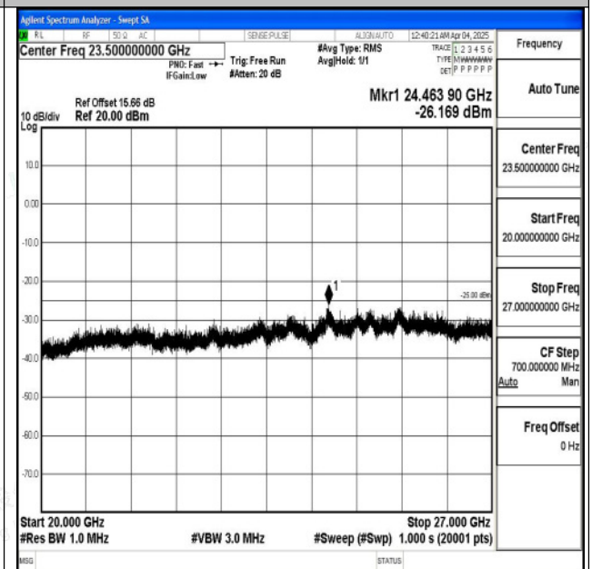
Band7_5MHz_16QAM_20775_1RB#0_20000~27000_20000~27000
