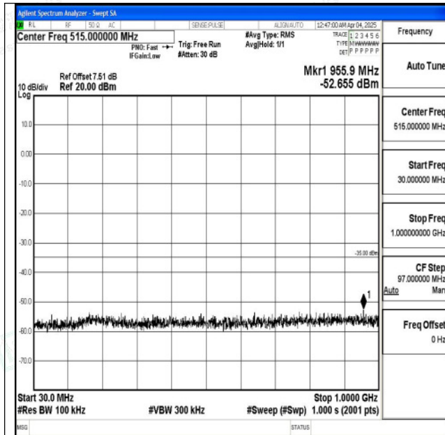
Band7_15MHz_QPSK_21100_1RB#0_30~1000_30~1000 0
