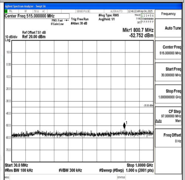
Band7_15MHz_16QAM_20825_1RB#0_30~1000_30~1000
