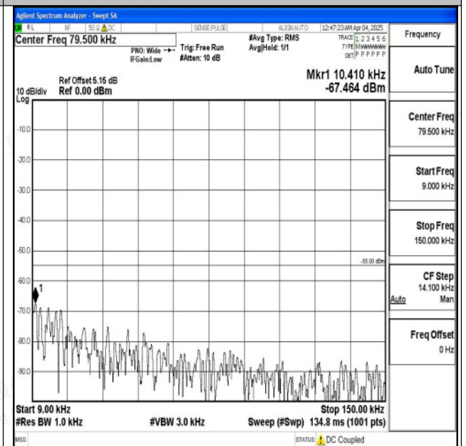
Band7_15MHz_16QAM_21100_1RB#0_0.009~0.15_0.009~0.15 9~0.15
