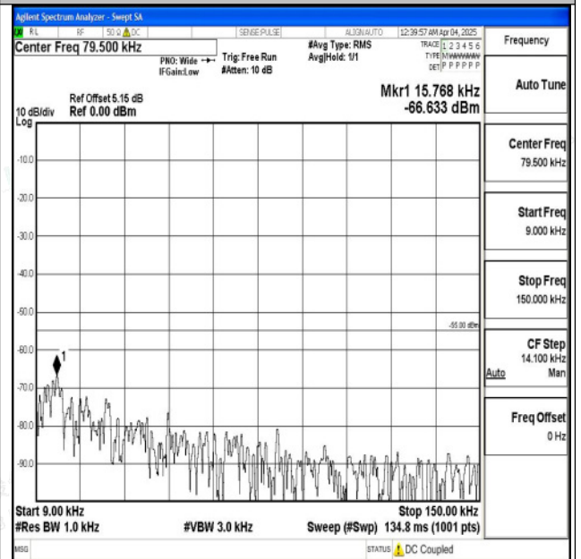
Band7_5MHz_16QAM_20775_1RB#0_0.009~0.15_0.009~0.15
