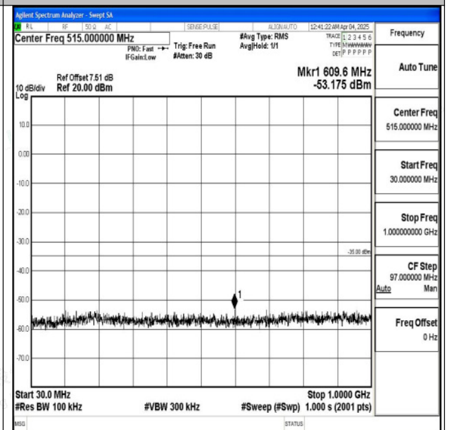
Band7_5MHz_16QAM_21100_1RB#0_30~1000_30~1000
