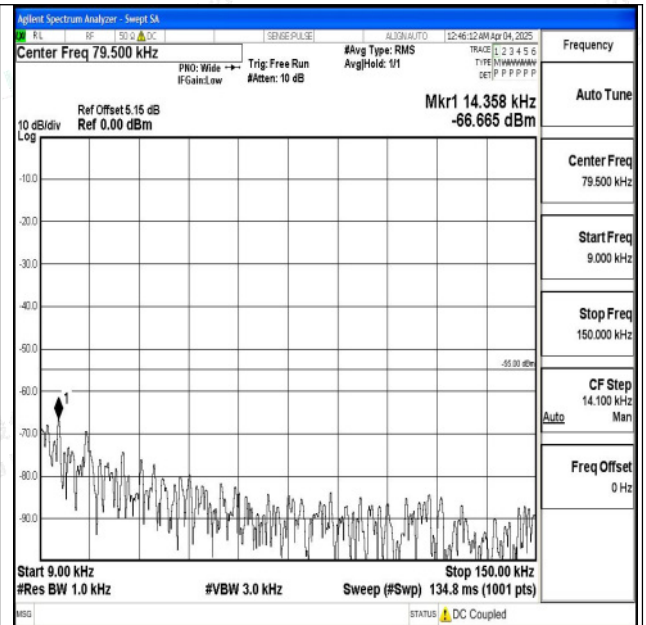
Band7_15MHz_16QAM_20825_1RB#0_0.009~0.15_0.009~0.15
