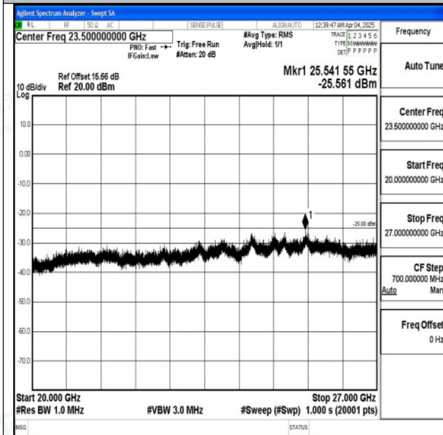
Band7_5MHz_QPSK_20775_1RB#0_20000~27000_20000~27000
