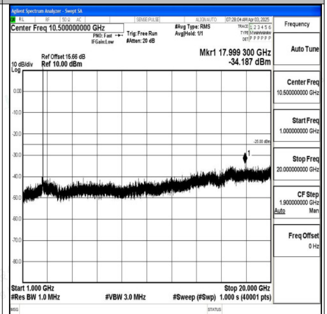
Band7_10MHz_QPSK_21400_1RB#0_1000~20000_1000~20000
