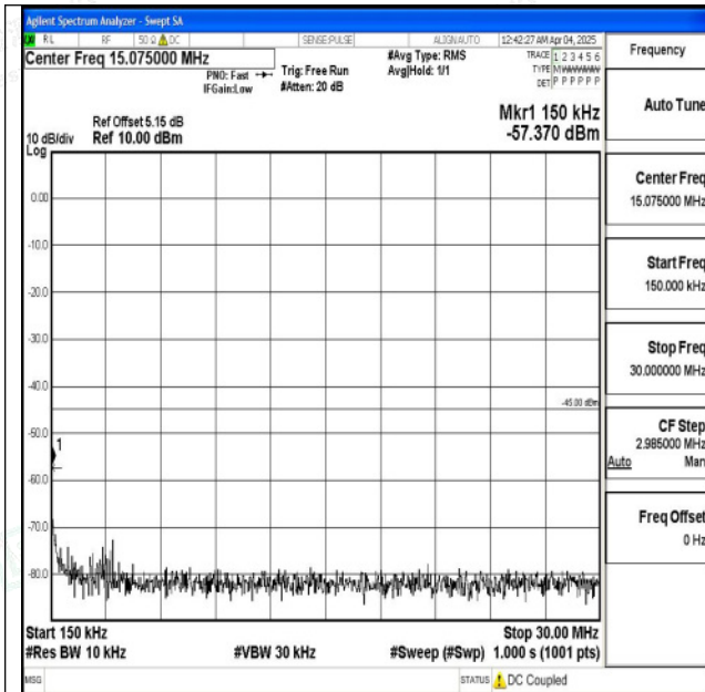
Band7_5MHz_16QAM_21425_1RB#0_0.15~30_0.15~30
