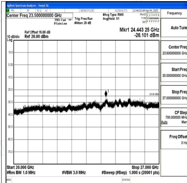
Band7_15MHz_QPSK_20825_1RB#0_20000~27000_2000~27000
