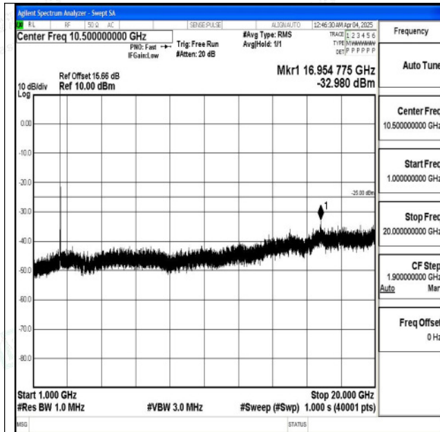
Band7_15MHz_16QAM_20825_1RB#0_1000~20000_10 00~20000
