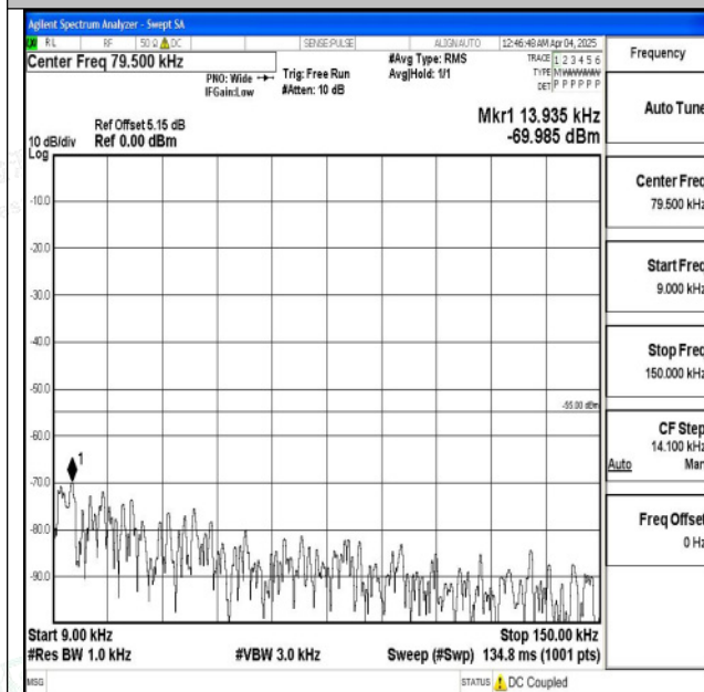
Band7_15MHz_QPSK_21100_1RB#0_0.009~0.15_0.009 ~0.15
