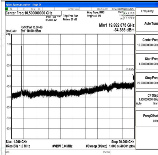
Band7_10MHz_16QAM_21100_1RB#0_1000~20000_10 00~20000
