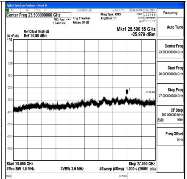
Band7_15MHz_16QAM_20825_1RB#0_20000~27000_2 0000~27000
