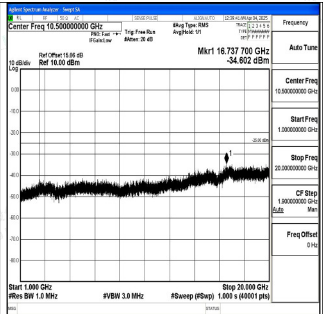
Band7_5MHz_QPSK_20775_1RB#0_1000~20000_1000~20000
