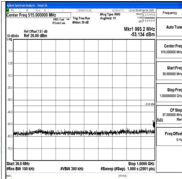
Band7_5MHz_QPSK_21425_1RB#0_30~1000_30~1000
