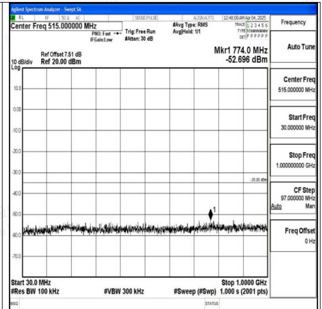
Band7_5MHz_16QAM_20775_1RB#0_30~1000_30~1000 0
