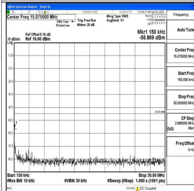
Band7_15MHz_16QAM_20825_1RB#0_0.15~30_0.15~30
