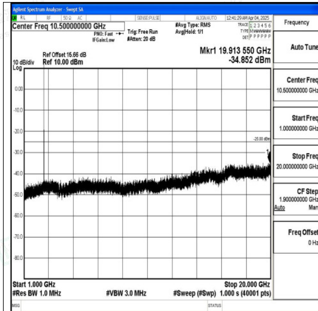
Band7_5MHz_16QAM_21100_1RB#0_1000~20000_100 0~20000
