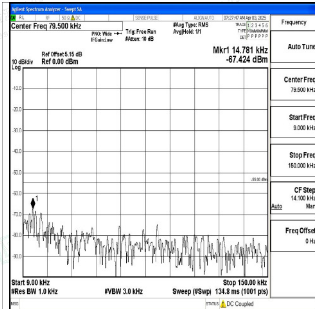
Band7_10MHz_QPSK_21400_1RB#0_0.009~0.15_0.009~0.15
