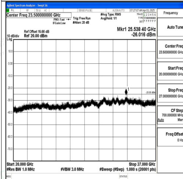
Band7_10MHz_QPSK_21100_1RB#0_20000~27000_20000~27000 000~27000
