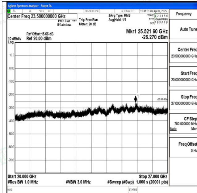
Band7_5MHz_QPSK_21100_1RB#0_20000~27000_20000~27000
