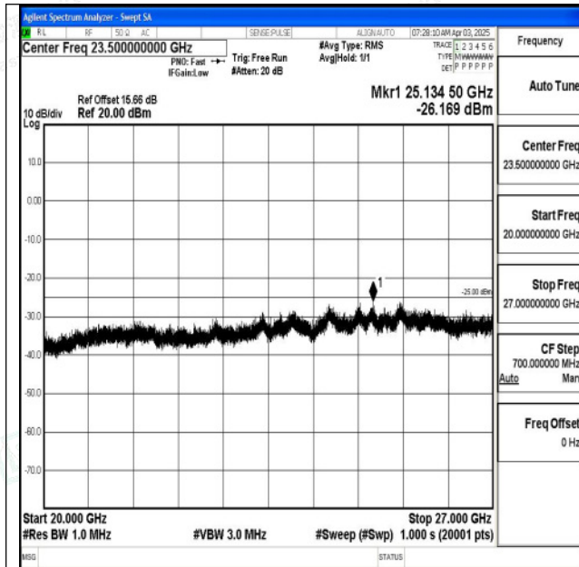
Band7_10MHz_QPSK_21400_1RB#0_20000~27000_2000~27000
