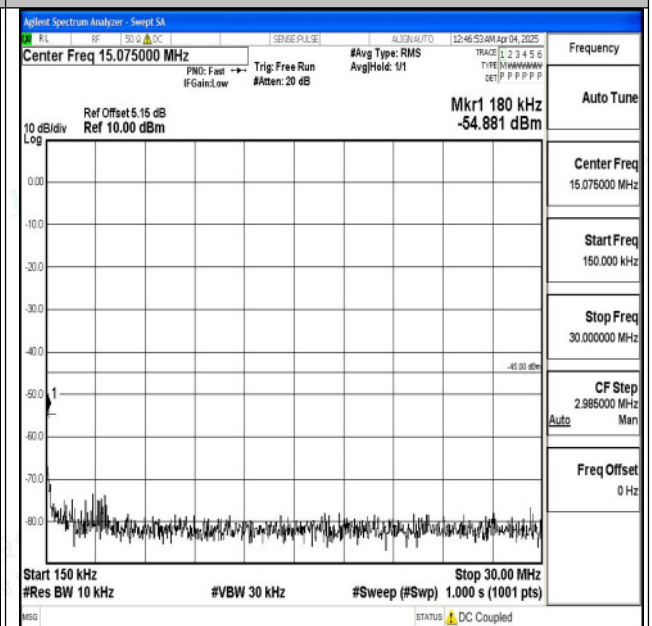
Band7_15MHz_QPSK_21100_1RB#0_0.15~30_0.15~30
