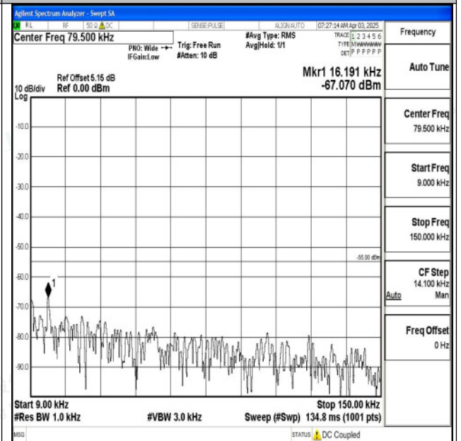
Band7_10MHz_16QAM_21100_1RB#0_0.009~0.15_0.009~0.15 9~0.15
