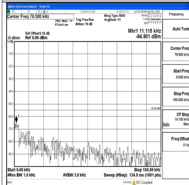
Band7_20MHz_QPSK_20850_1RB#0_0.009~0.15_0.009 ~0.15
