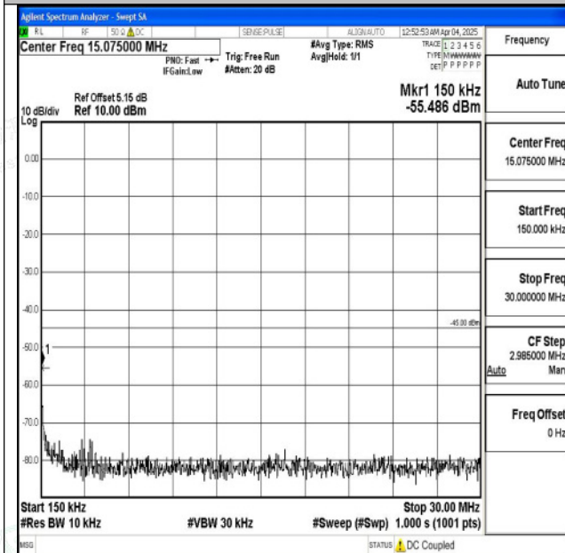
Band7_20MHz_16QAM_21100_1RB#0_0.15~30_0.15~30
