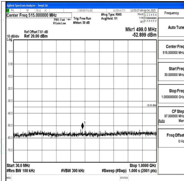
Band7_20MHz_QPSK_21350_1RB#0_30~1000_30~1000 0
