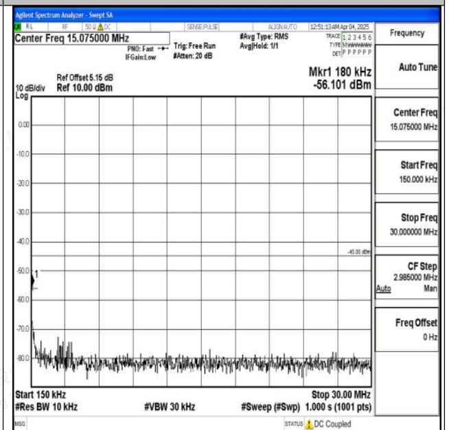
Band7_20MHz_QPSK_20850_1RB#0_0.15~30_0.15~30
