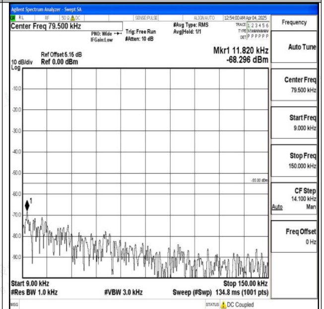
Band7_20MHz_16QAM_21350_1RB#0_0.009~0.15_0.009~0.15 09~0.15
