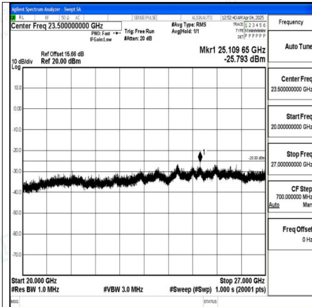
Band7_20MHz_QPSK_21100_1RB#0_20000~27000_2000~27000
