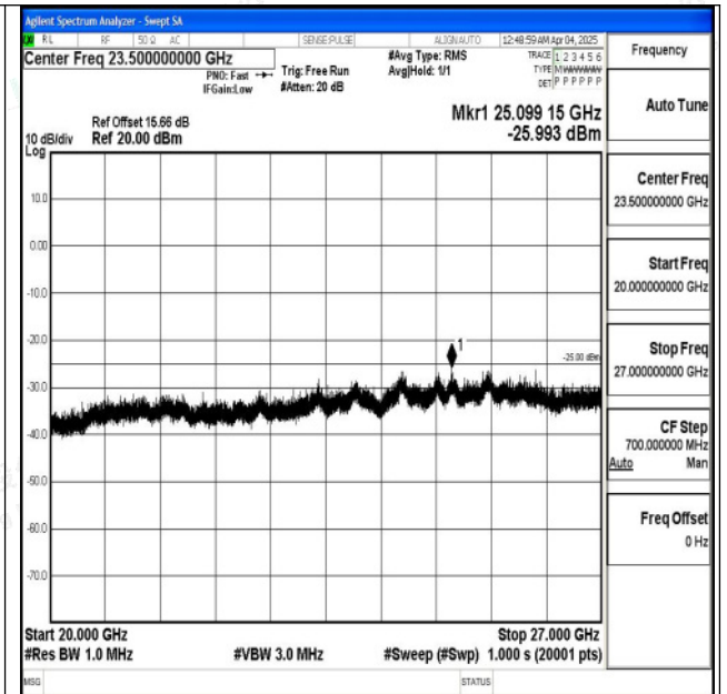
Band7_15MHz_16QAM_21375_1RB#0_20000~27000_2 0000~27000
