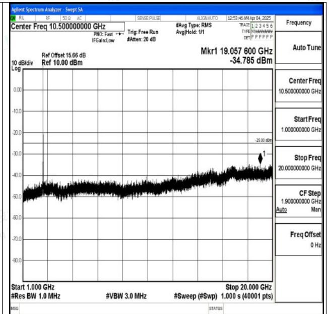
Band7_20MHz_QPSK_21350_1RB#0_1000~20000_1000~20000 0~20000
