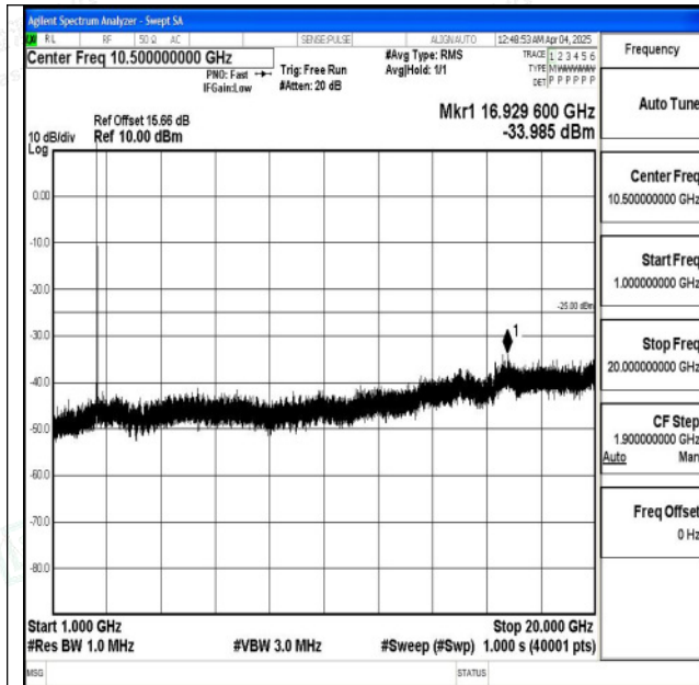
Band7_15MHz_16QAM_21375_1RB#0_1000~20000_10 00~20000
