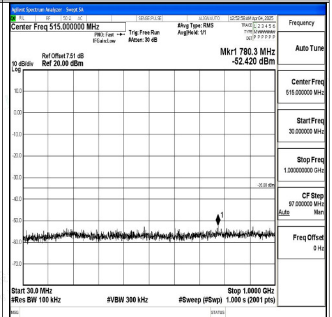
Band7_20MHz_16QAM_21100_1RB#0_30~1000_30~1000
