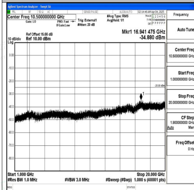
Band38_5MHz_16QAM_38000_1RB#0_1000~20000_10
