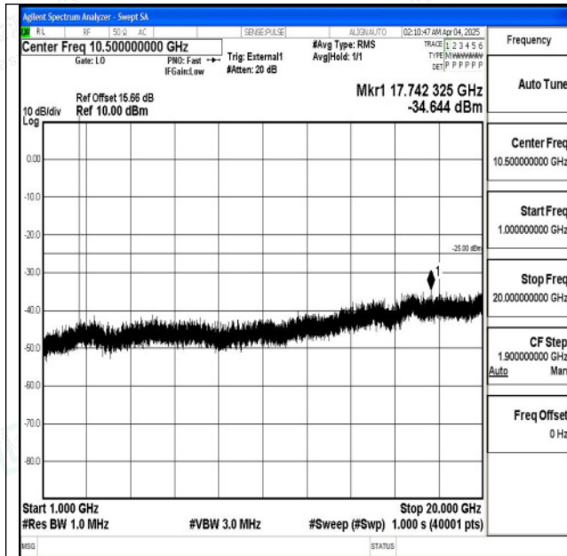
Band38_5MHz_16QAM_37775_1RB#0_1000~20000_10 00~20000
