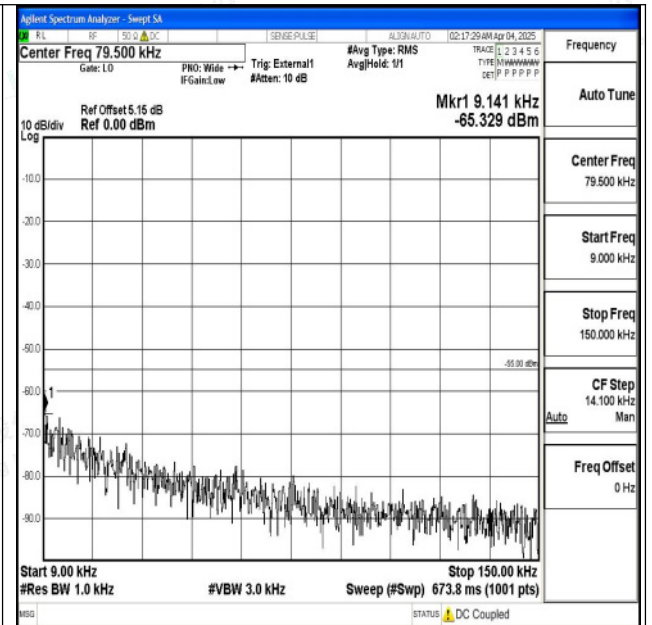
Band38_5MHz_16QAM_38225_1RB#0_0.009~0.15_0.0 09~0.15
