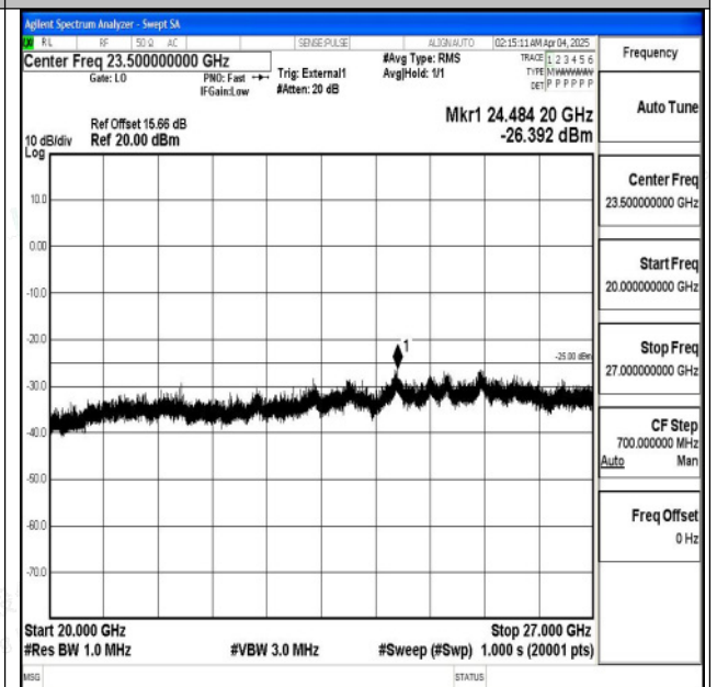
Band38_5MHz_16QAM_38000_1RB#0_20000~27000_2
