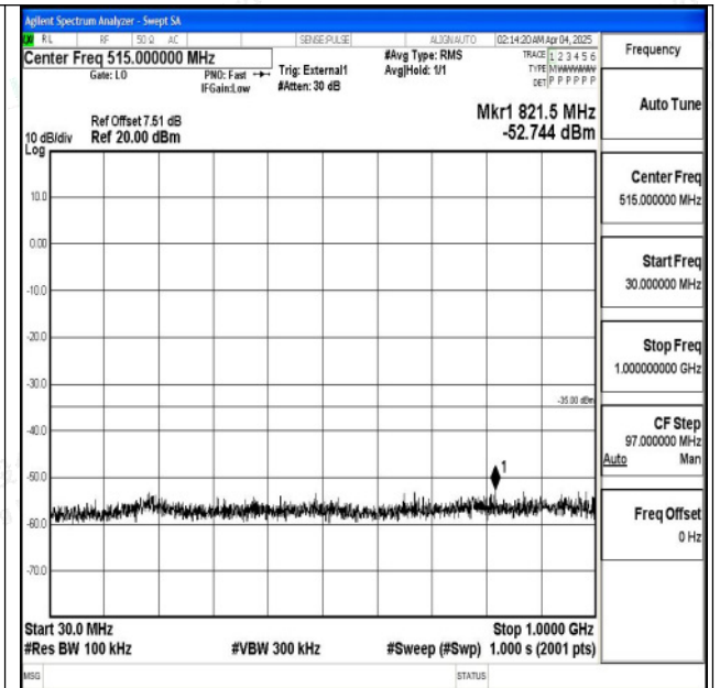
Band38_5MHz_16QAM_38000_1RB#0_30~1000_30~10
