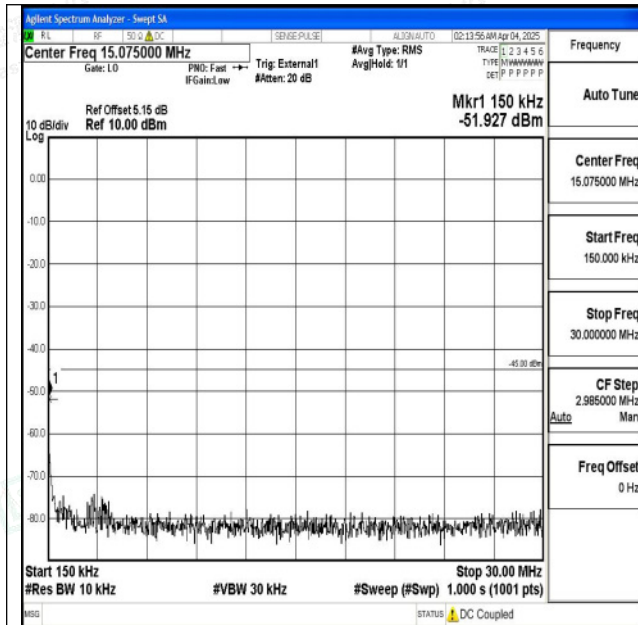
Band38_5MHz_16QAM_38000_1RB#0_0.15~30_0.15~3
