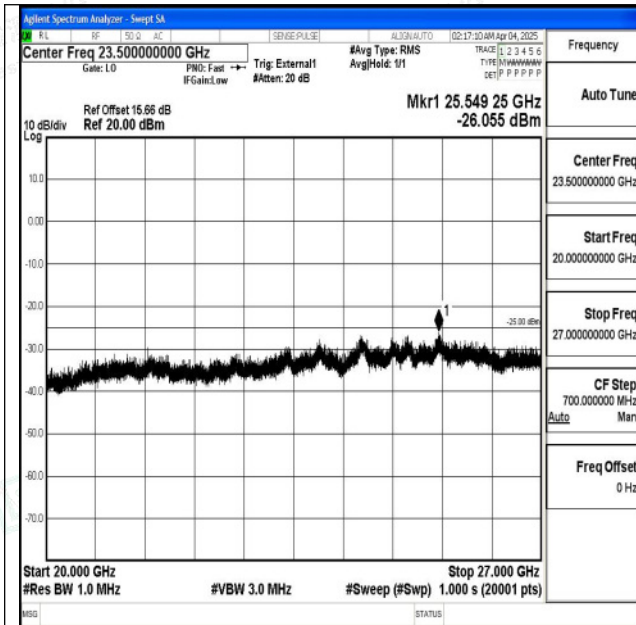
Band38_5MHz_QPSK_38225_1RB#0_20000~27000_20 000~27000
