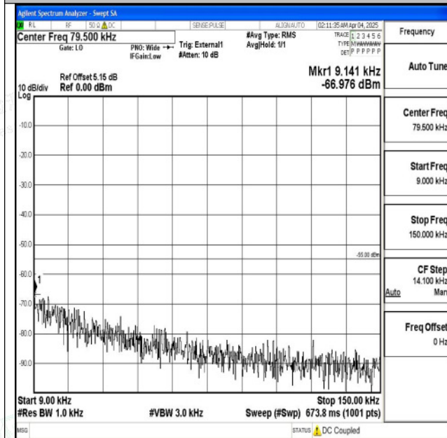
Band38_5MHz_QPSK_38000_1RB#0_0.009~0.15_0.009 ~0.15
