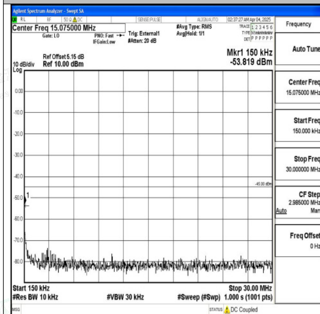
Band38_15MHz_16QAM_37825_1RB#0_0.15~30_0.15~30 30
