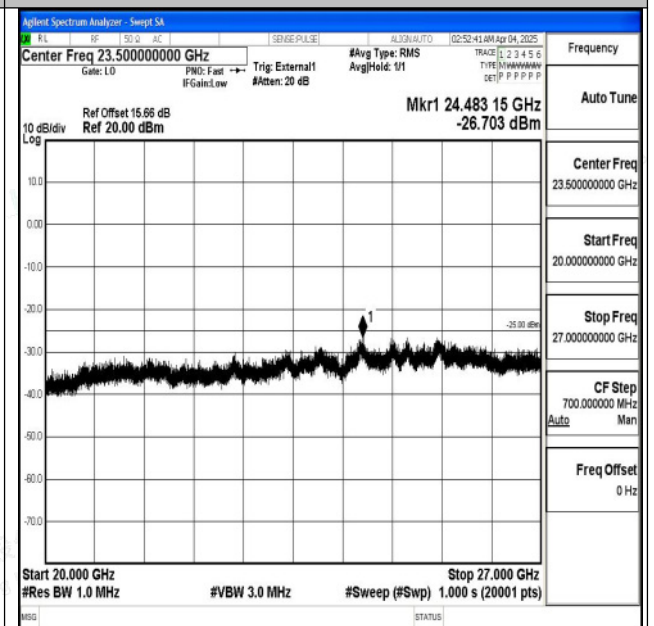
Band38_20MHz_16QAM_37850_1RB#0_20000~27000_20000~27000
