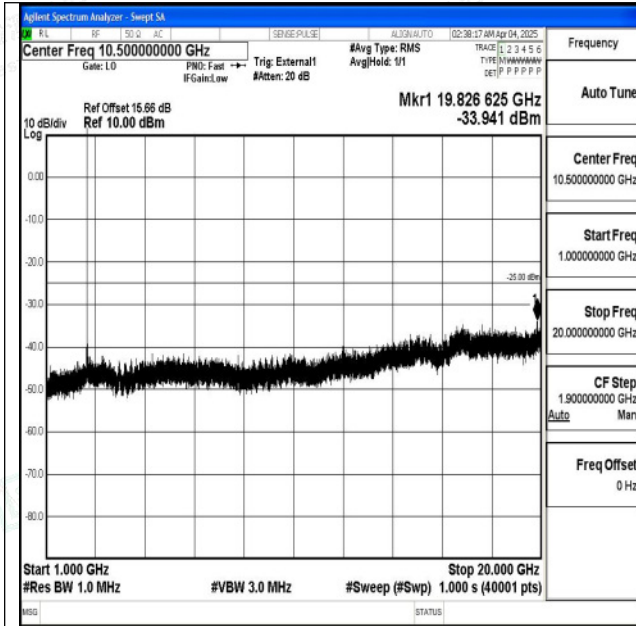
Band38_15MHz_16QAM_37825_1RB#0_1000~20000_1 000~20000
