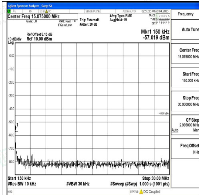
Band38_20MHz_16QAM_37850_1RB#0_0.15~30_0.15~30
