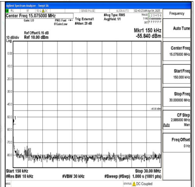
Band38_15MHz_QPSK_38175_1RB#0_0.15~30_0.15~3 0
