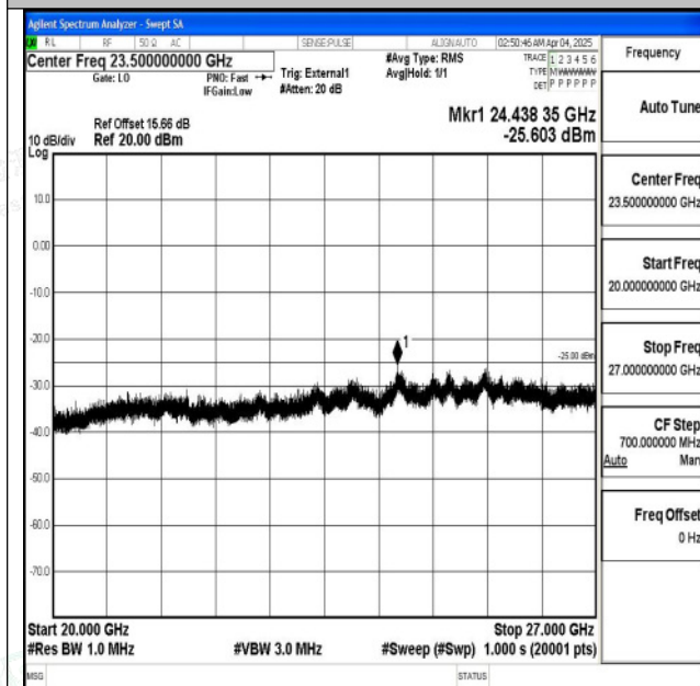
Band38_20MHz_QPSK_37850_1RB#0_20000~27000_20000~27000
