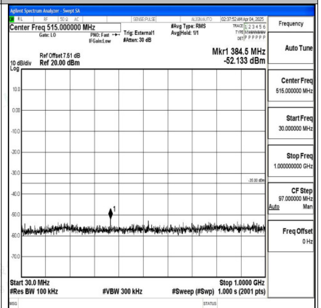
Band38_15MHz_16QAM_37825_1RB#0_30~1000_30~1000 000
