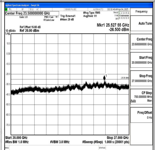
Band38_10MHz_16QAM_38200_1RB#0_20000~27000_20000~27000
