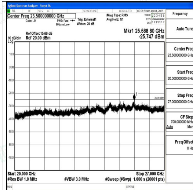
Band38_10MHz_QPSK_38000_1RB#0_20000~27000_2 0000~27000
