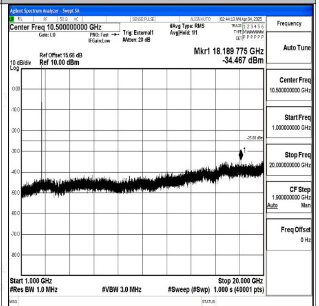
Band38_15MHz_QPSK_38175_1RB#0_1000~20000_10 00~20000
