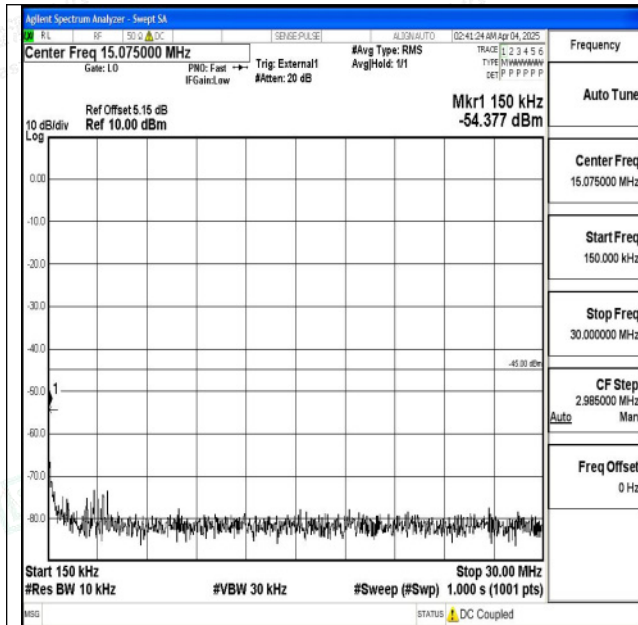
Band38_15MHz_16QAM_38000_1RB#0_0.15~30_0.15~30
