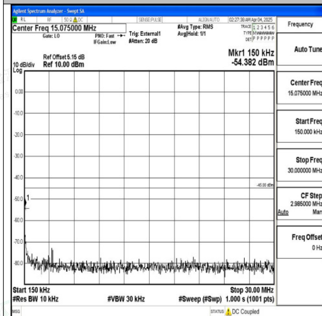
Band38_10MHz_16QAM_38000_1RB#0_0.15~30_0.15~30 30
