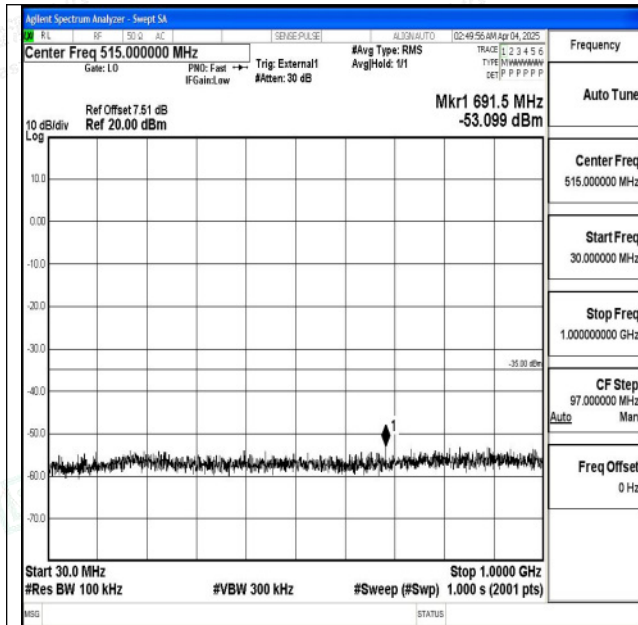
Band38_20MHz_QPSK_37850_1RB#0_30~1000_30~1000
