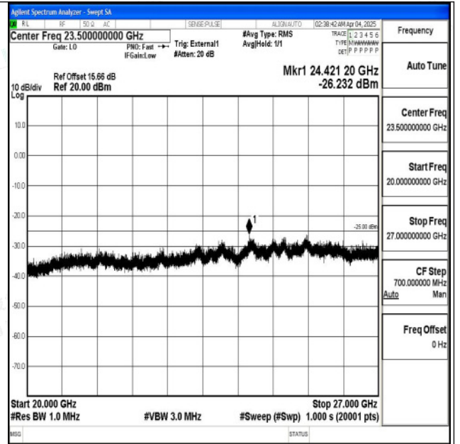
Band38_15MHz_16QAM_37825_1RB#0_20000~27000_ 20000~27000
