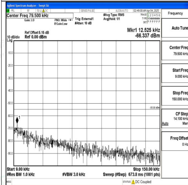
Band38_20MHz_QPSK_37850_1RB#0_0.009~0.15_0.00 9~0.15
