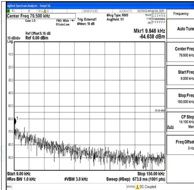
Band38_20MHz_QPSK_38000_1RB#0_0.009~0.15_0.00 9~0.15
