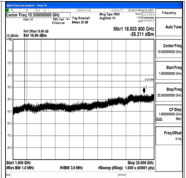
Band38_15MHz_QPSK_38000_1RB#0_1000~20000_1000~20000
