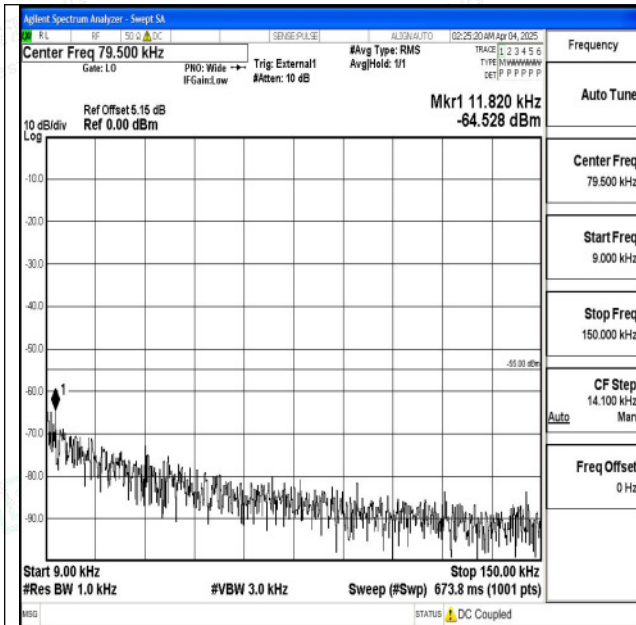
Band38_10MHz_QPSK_38000_1RB#0_0.009~0.15_0.00 9~0.15
