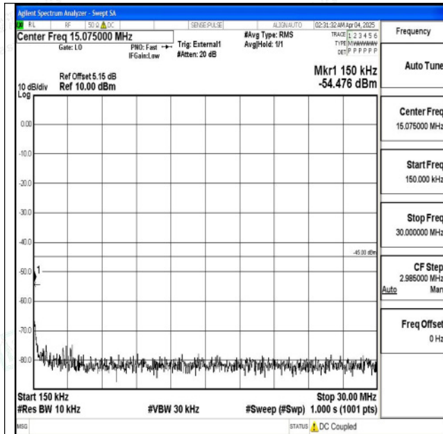
Band38_10MHz_16QAM_38200_1RB#0_0.15~30_0.15~30
