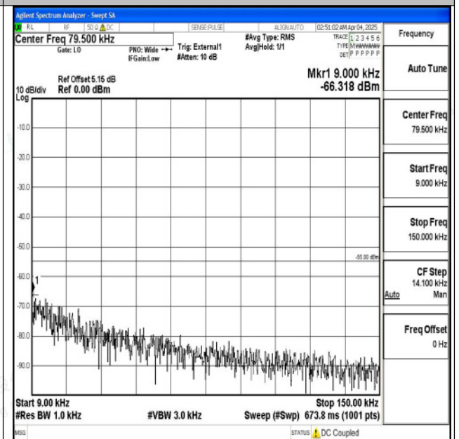
Band38_20MHz_16QAM_37850_1RB#0_0.009~0.15_0.009~0.15
