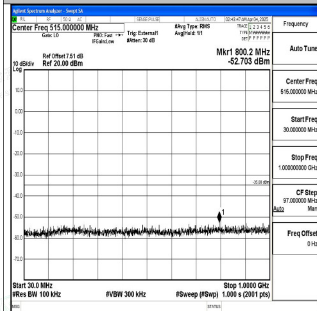
Band38_15MHz_QPSK_38175_1RB#0_30~1000_30~10 00
