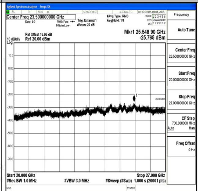
Band38_15MHz_16QAM_38000_1RB#0_20000~27000_20000~27000
