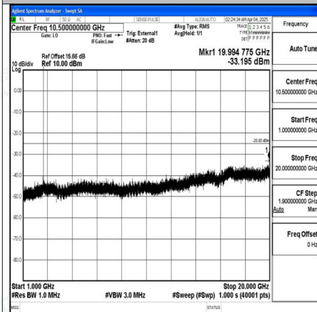
Band38_10MHz_16QAM_37800_1RB#0_1000~20000_1000~20000
