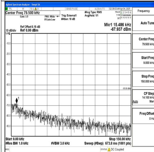
Band38_15MHz_QPSK_38000_1RB#0_0.009~0.15_0.00 9~0.15
