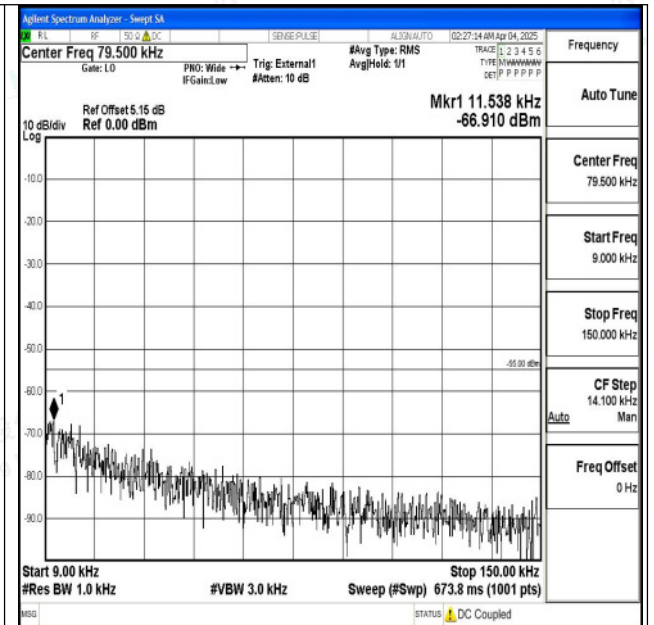
Band38_10MHz_16QAM_38000_1RB#0_0.009~0.15_0. 009~0.15
