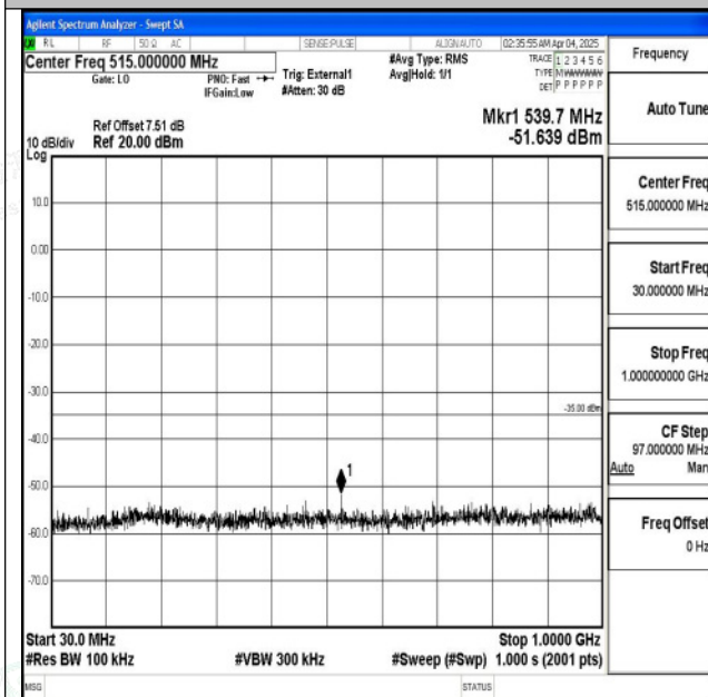
Band38_15MHz_QPSK_37825_1RB#0_30~1000_30~10 00
