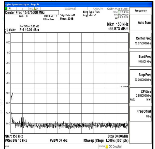
Band38_10MHz_QPSK_38000_1RB#0_0.15~30_0.15~3 0
