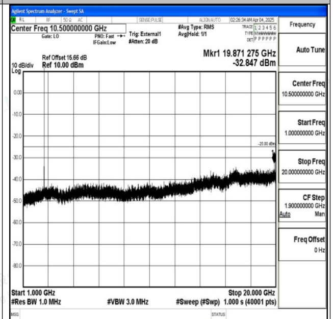
Band38_10MHz_QPSK_38000_1RB#0_1000~20000_10 00~20000
