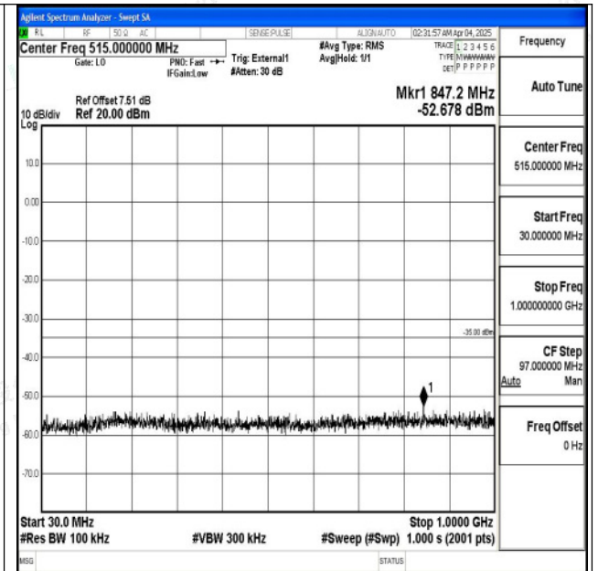
Band38_10MHz_16QAM_38200_1RB#0_30~1000_30~1000
