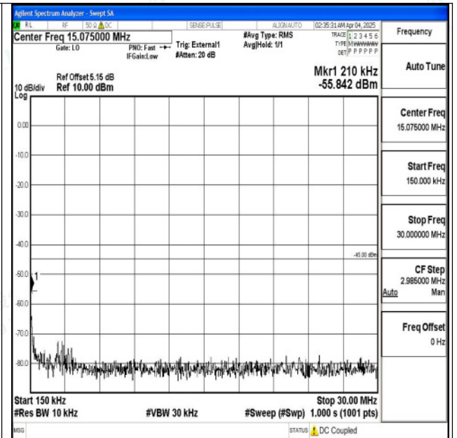
Band38_15MHz_QPSK_37825_1RB#0_0.15~30_0.15~3 0
