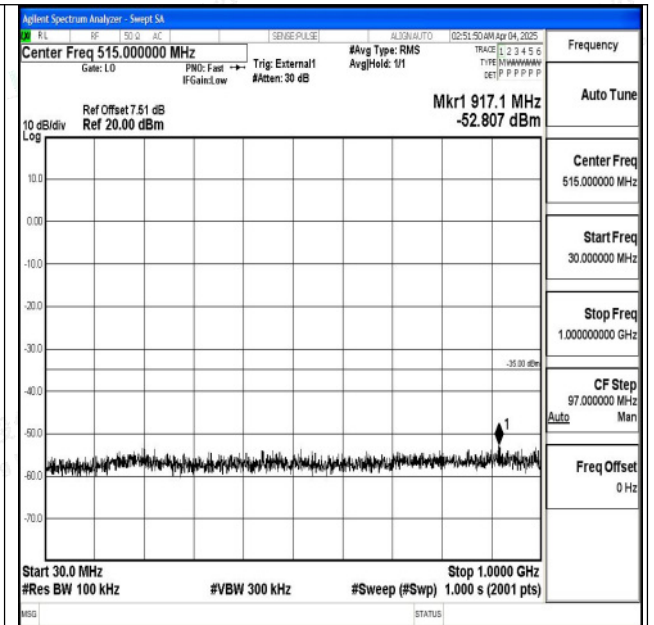
Band38_20MHz_16QAM_37850_1RB#0_30~1000_30~1000
