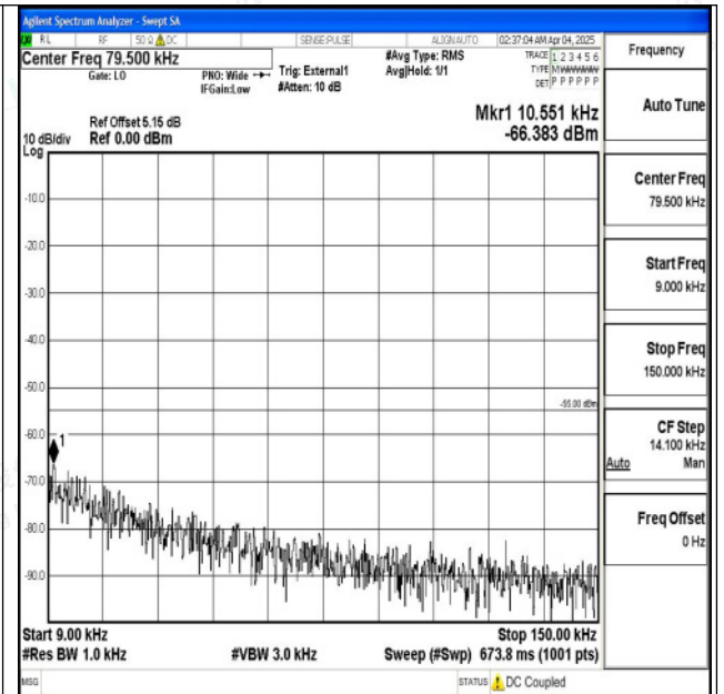
Band38_15MHz_16QAM_37825_1RB#0_0.009~0.15_0. 009~0.15
