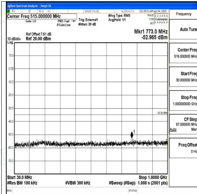
Band38_15MHz_QPSK_38000_1RB#0_30~1000_30~1000
