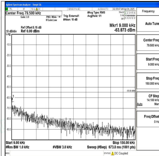
Band38_15MHz_QPSK_37825_1RB#0_0.009~0.15_0.00 9~0.15
