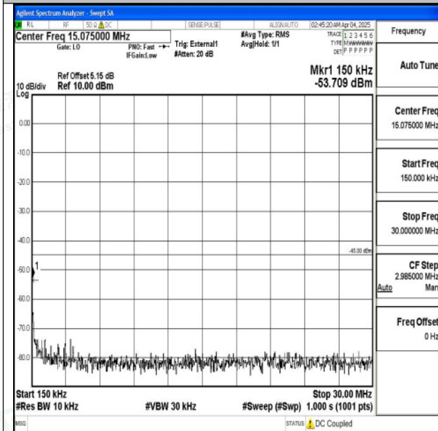
Band38_15MHz_16QAM_38175_1RB#0_0.15~30_0.15~30 30
