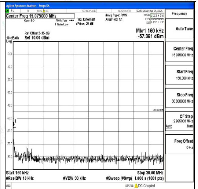
Band38_20MHz_QPSK_38000_1RB#0_0.15~30_0.15~3 0
