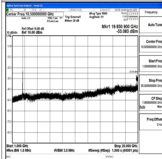
Band38_20MHz_16QAM_37850_1RB#0_1000~20000_1000~20000
