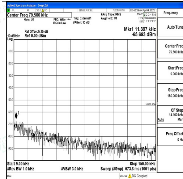
Band38_15MHz_QPSK_38175_1RB#0_0.009~0.15_0.00 9~0.15
