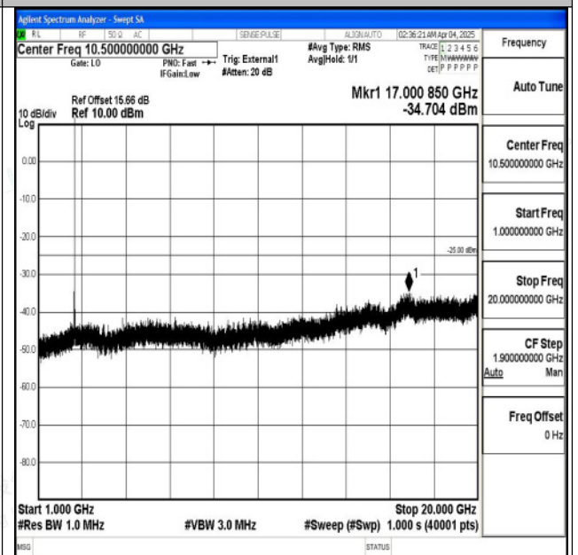
Band38_15MHz_QPSK_37825_1RB#0_1000~20000_10 00~20000
