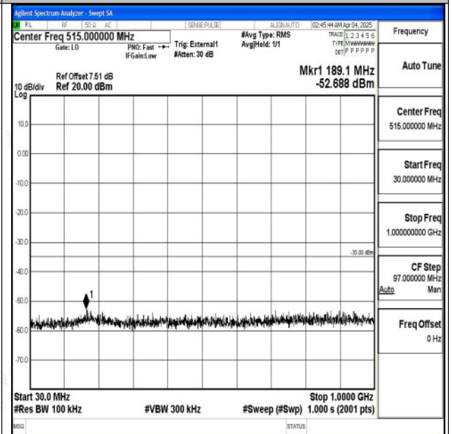
Band38_15MHz_16QAM_38175_1RB#0_30~1000_30~1000 000
