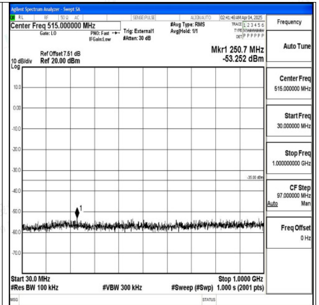
Band38_15MHz_16QAM_38000_1RB#0_30~1000_30~1000
