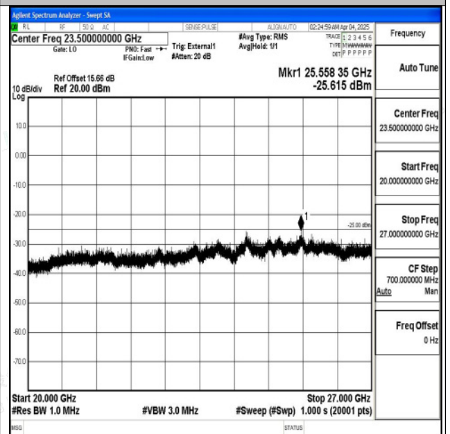
Band38_10MHz_16QAM_37800_1RB#0_20000~27000_20000~27000
