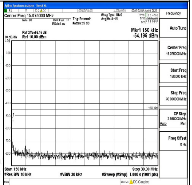
Band38_20MHz_QPSK_37850_1RB#0_0.15~30_0.15~3 0
