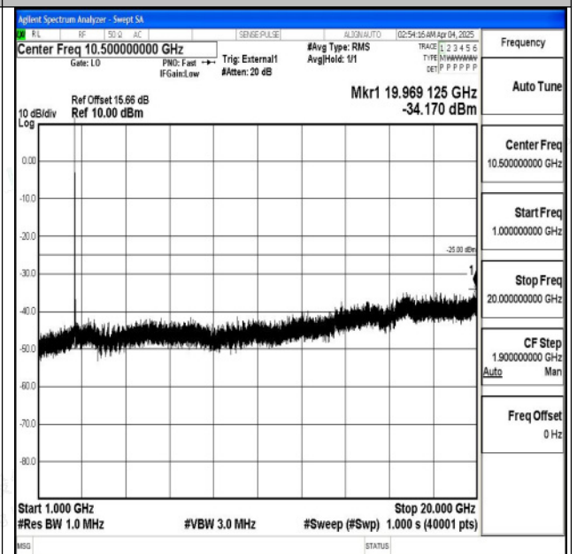
Band38_20MHz_QPSK_38000_1RB#0_1000~20000_10 00~20000
