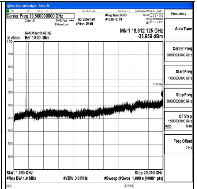
Band38_20MHz_QPSK_37850_1RB#0_1000~20000_1000~20000
