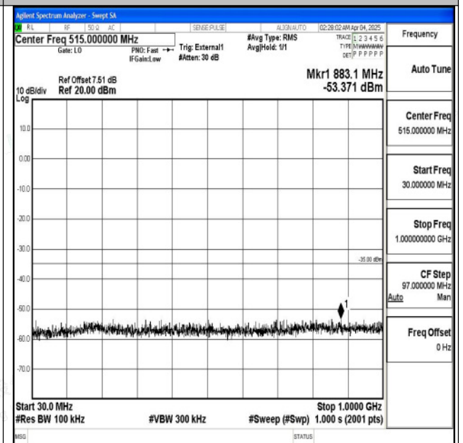
Band38_10MHz_16QAM_38000_1RB#0_30~1000_30~1000 000
