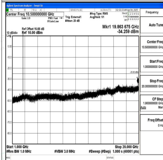
Band38_10MHz_16QAM_38200_1RB#0_1000~20000_1000~20000
