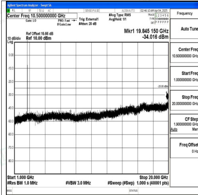
Band38_15MHz_16QAM_38175_1RB#0_1000~20000_1 000~20000
