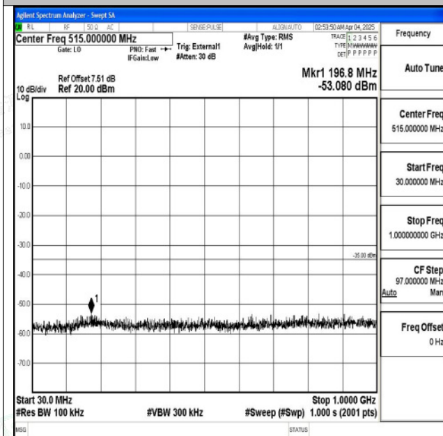
Band38_20MHz_QPSK_38000_1RB#0_30~1000_30~10 00
