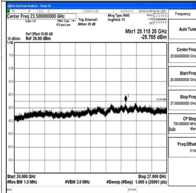
Band38_15MHz_QPSK_38000_1RB#0_20000~27000_20000~27000
