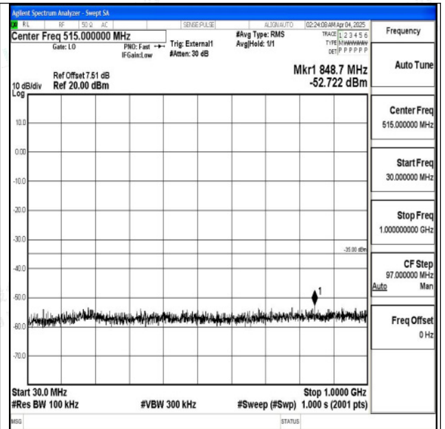
Band38_10MHz_16QAM_37800_1RB#0_30~1000_30~1000
