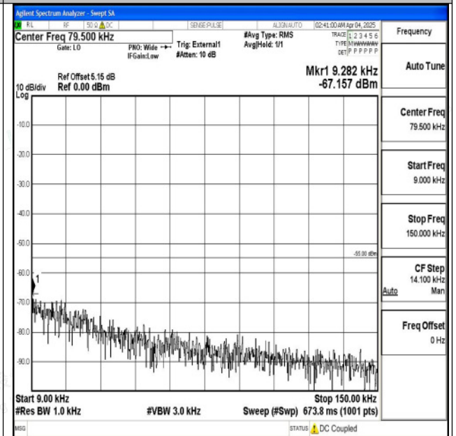
Band38_15MHz_16QAM_38000_1RB#0_0.009~0.15_0.009~0.15
