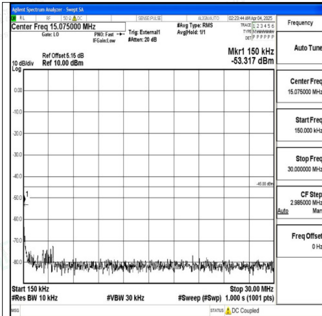
Band38_10MHz_16QAM_37800_1RB#0_0.15~30_0.15~30
