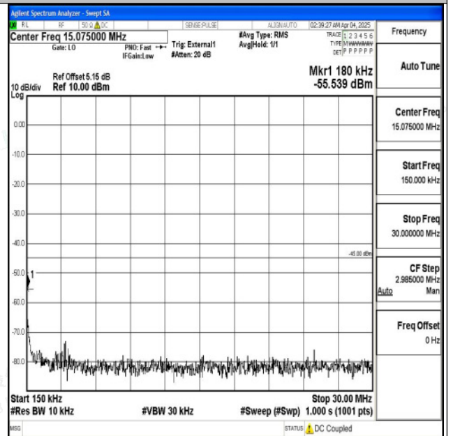
Band38_15MHz_QPSK_38000_1RB#0_0.15~30_0.15~3 0
