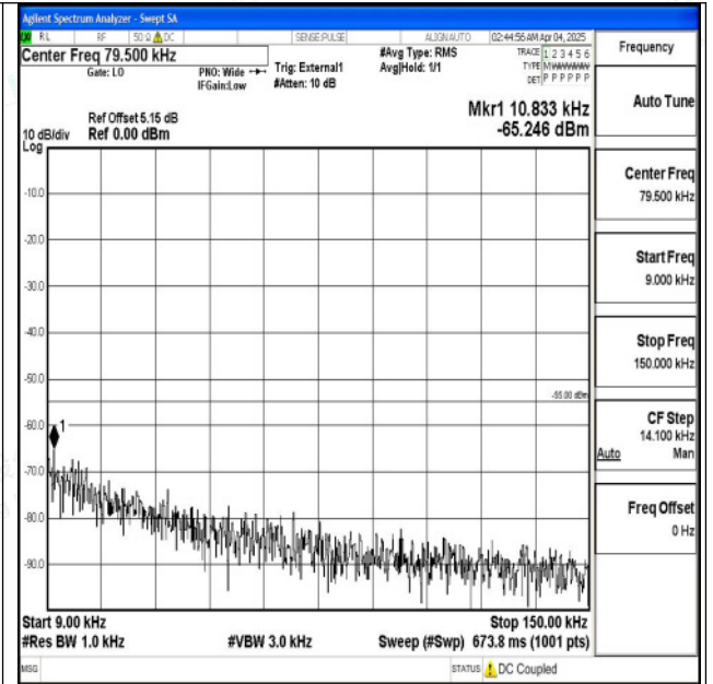
Band38_15MHz_16QAM_38175_1RB#0_0.009~0.15_0. 009~0.15
