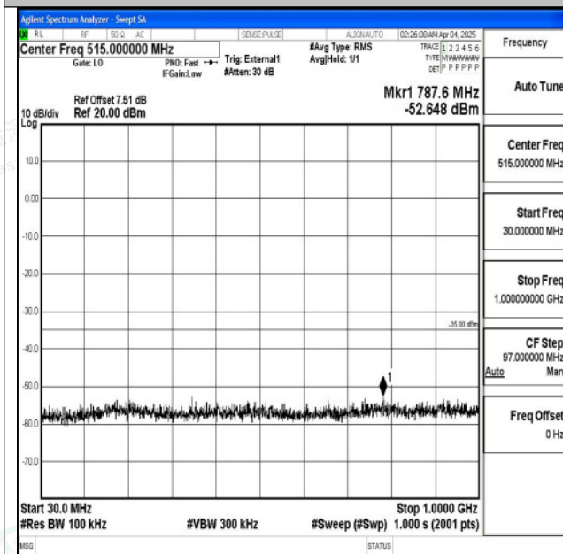
Band38_10MHz_QPSK_38000_1RB#0_30~1000_30~10 00
