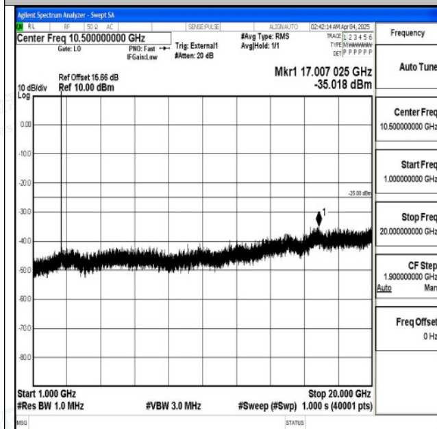
Band38_15MHz_16QAM_38000_1RB#0_1000~20000_1000~20000
