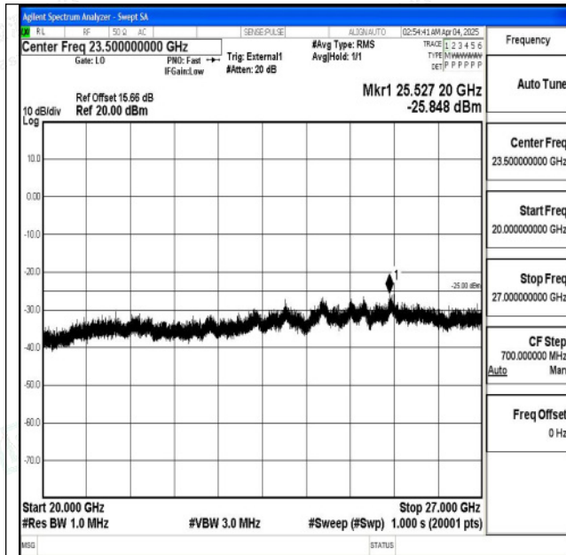
Band38_20MHz_QPSK_38000_1RB#0_20000~27000_2 0000~27000
