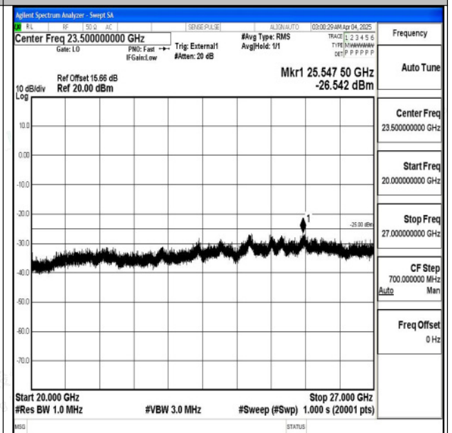
Band38_20MHz_16QAM_38150_1RB#0_20000~27000_20000~27000
