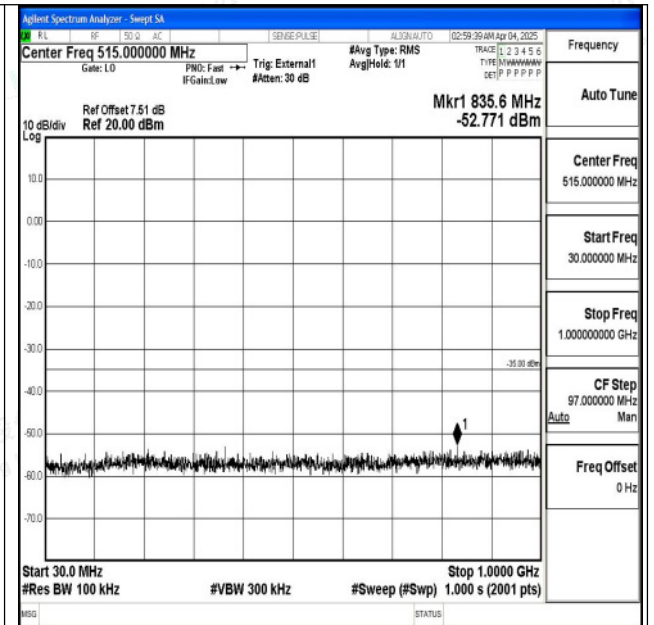
Band38_20MHz_16QAM_38150_1RB#0_30~1000_30~1000
