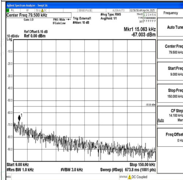
Band38_20MHz_QPSK_38150_1RB#0_0.009~0.15_0.009~0.15
