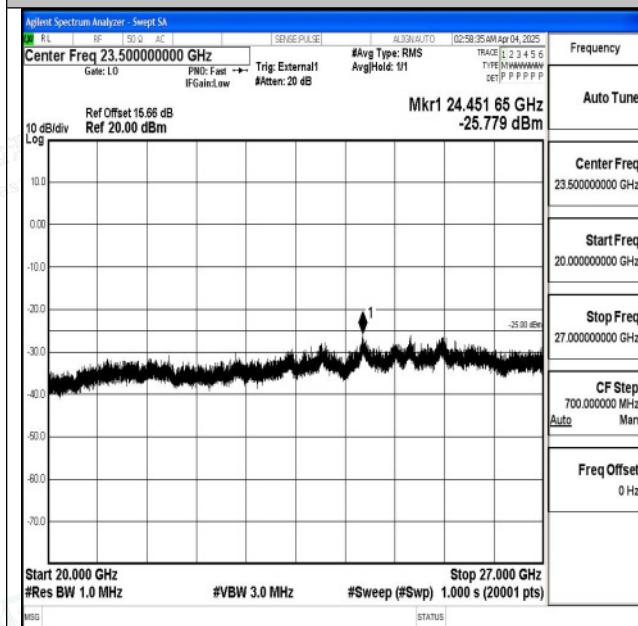
Band38_20MHz_QPSK_38150_1RB#0_20000~27000_20000~27000
