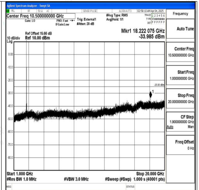
Band38_20MHz_QPSK_38150_1RB#0_1000~20000_1000~20000
