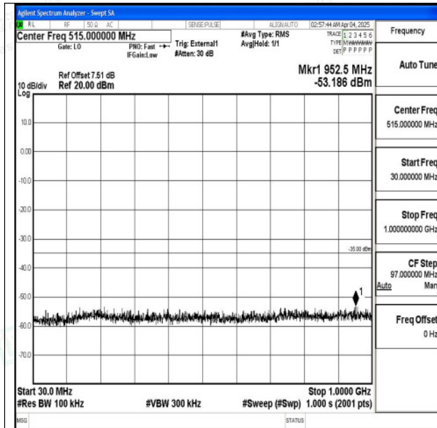
Band38_20MHz_QPSK_38150_1RB#0_30~1000_30~1000
