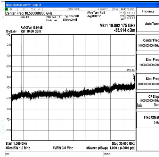
Band38_20MHz_16QAM_38000_1RB#0_1000~20000_1000~20000
