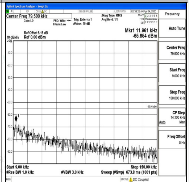
Band38_20MHz_16QAM_38150_1RB#0_0.009~0.15_0.009~0.15
