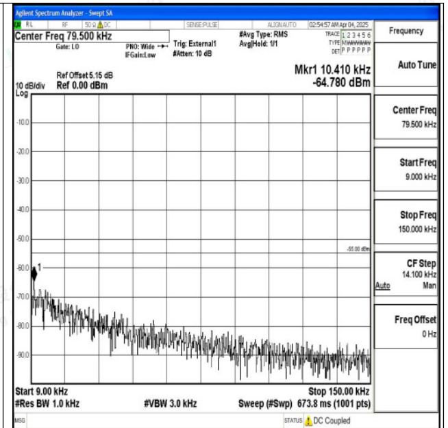
Band38_20MHz_16QAM_38000_1RB#0_0.009~0.15_0. 009~0.15
