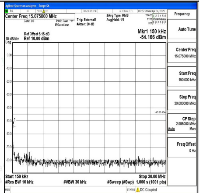
Band38_20MHz_QPSK_38150_1RB#0_0.15~30_0.15~30
