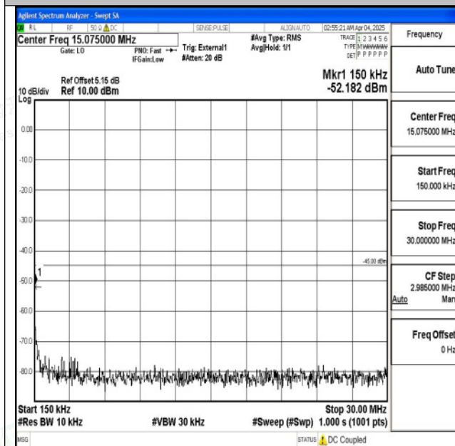
Band38_20MHz_16QAM_38000_1RB#0_0.15~30_0.15~ 30
