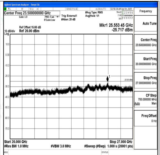
Band38_20MHz_16QAM_38000_1RB#0_20000~27000_20000~27000
