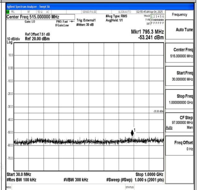
Band38_20MHz_16QAM_38000_1RB#0_30~1000_30~1 000
