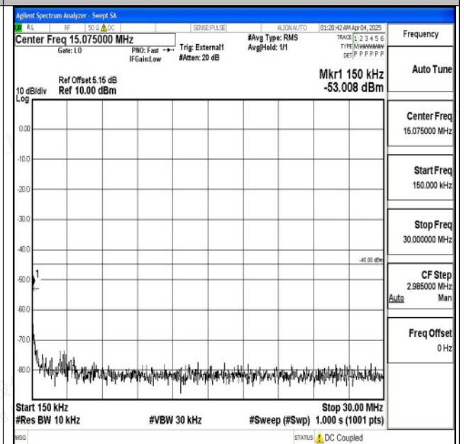
Band41_10MHz_QPSK_41540_1RB#0_0.15~30_0.15~30
