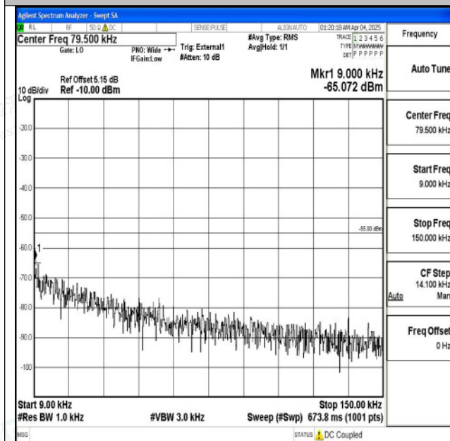
Band41_10MHz_QPSK_41540_1RB#0_0.009~0.15_0.009~0.15
