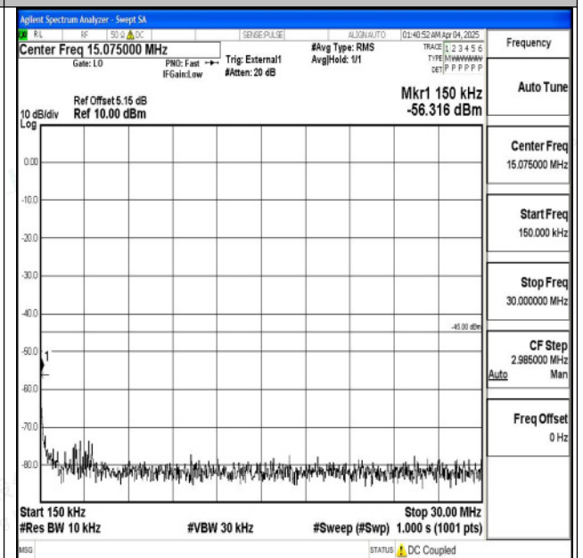
Band41_20MHz_QPSK_39750_1RB#0_0.15~30_0.15~3 0
