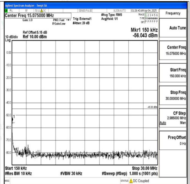
Band41_15MHz_QPSK_39725_1RB#0_0.15~30_0.15~3 0
