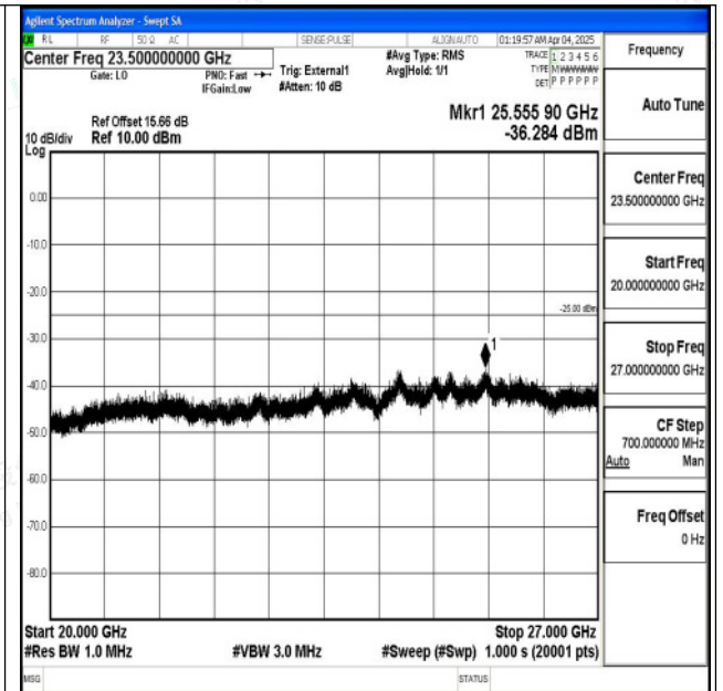
Band41_10MHz_16QAM_40620_1RB#0_20000~27000_20000~27000
