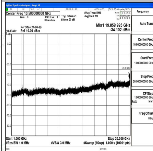
Band41_20MHz_16QAM_41490_1RB#0_1000~20000_1000~20000
