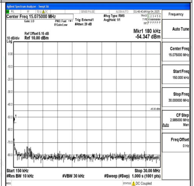
Band41_20MHz_QPSK_41490_1RB#0_0.15~30_0.15~3 0
