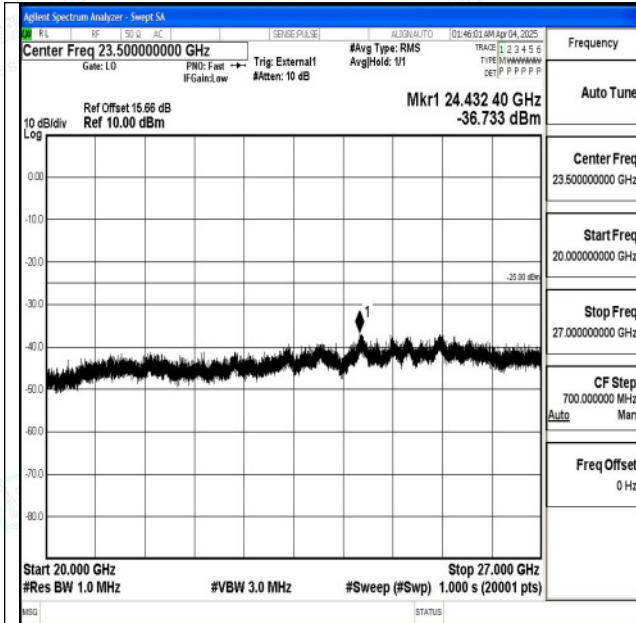
Band41_20MHz_QPSK_40620_1RB#0_20000~27000_2 0000~27000
