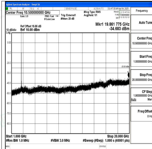
Band41_20MHz_16QAM_40620_1RB#0_1000~20000_1 000~20000
