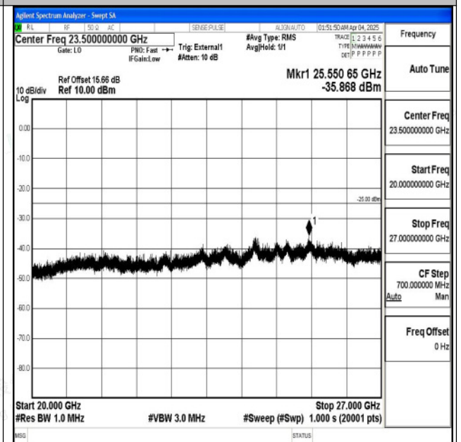
Band41_20MHz_16QAM_41490_1RB#0_20000~27000_20000~27000
