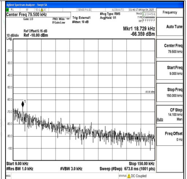
Band41_20MHz_16QAM_40620_1RB#0_0.009~0.15_0. 009~0.15
