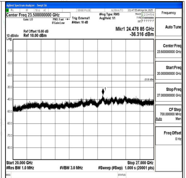
Band41_20MHz_16QAM_40620_1RB#0_20000~27000_ 20000~27000
