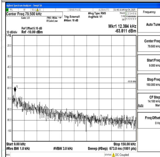
Band41_20MHz_QPSK_41490_1RB#0_0.009~0.15_0.00 9~0.15
