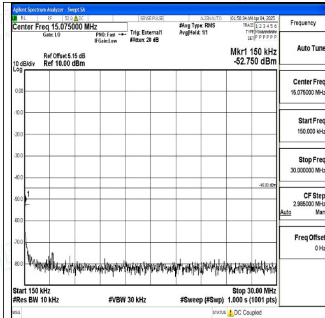
Band41_20MHz_16QAM_41490_1RB#0_0.15~30_0.15~30
