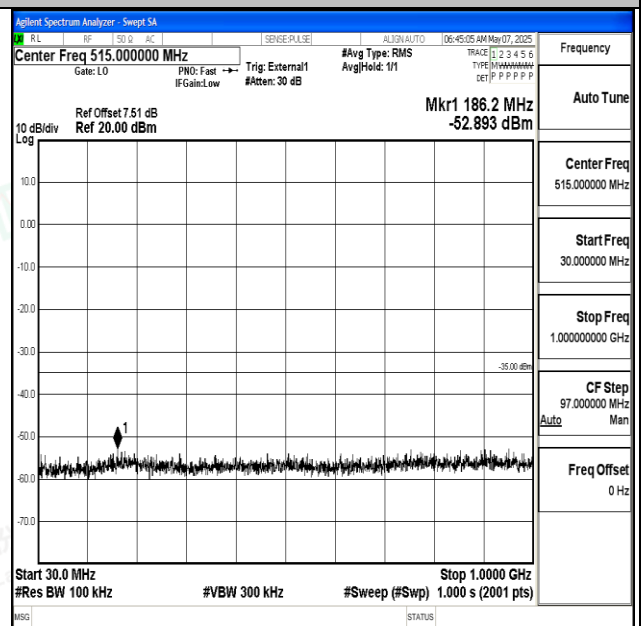
Band38_15MHz_16QAM_37825_1RB#0_30~1000_30~1 000
