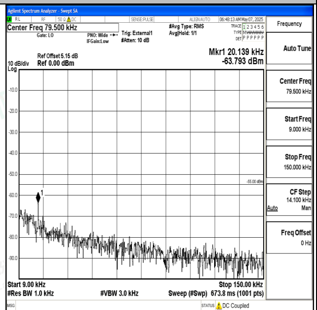
Band38_15MHz_16QAM_38000_1RB#0_0.009~0.15_0. 009~0.15
