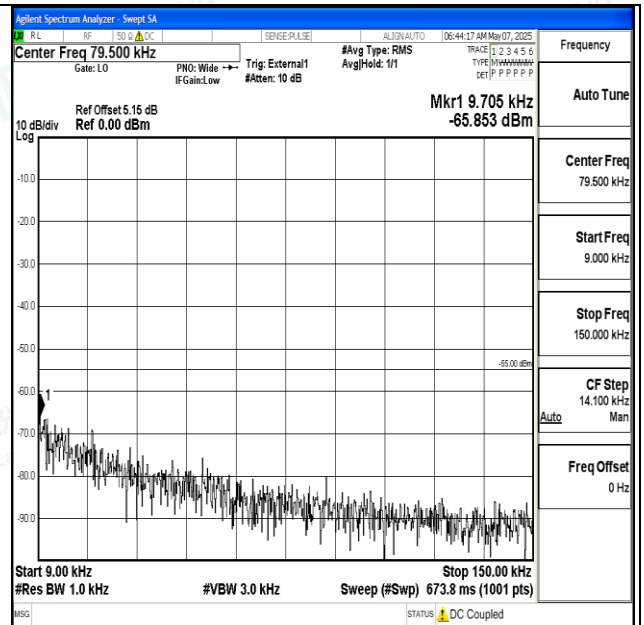
Band38_15MHz_16QAM_37825_1RB#0_0.009~0.15_0. 009~0.15
