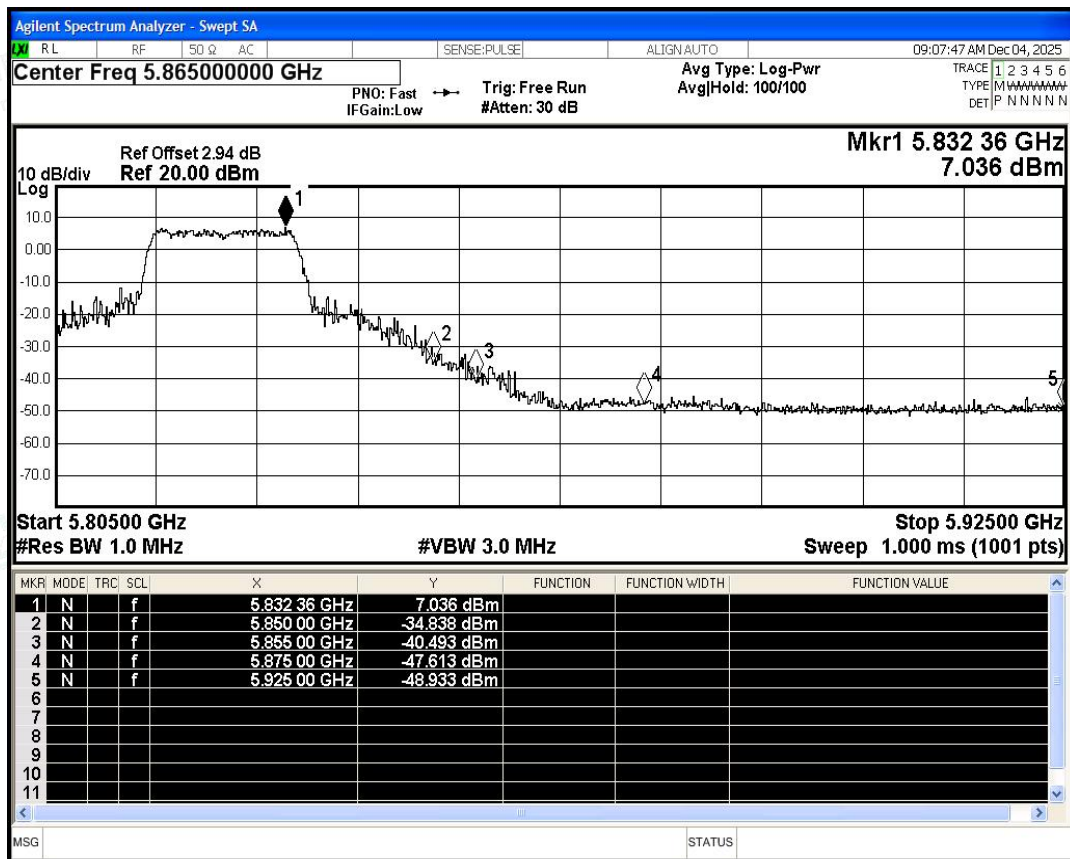
Restrict Band NVNT ac20 5825MHz Ant1 Peak
