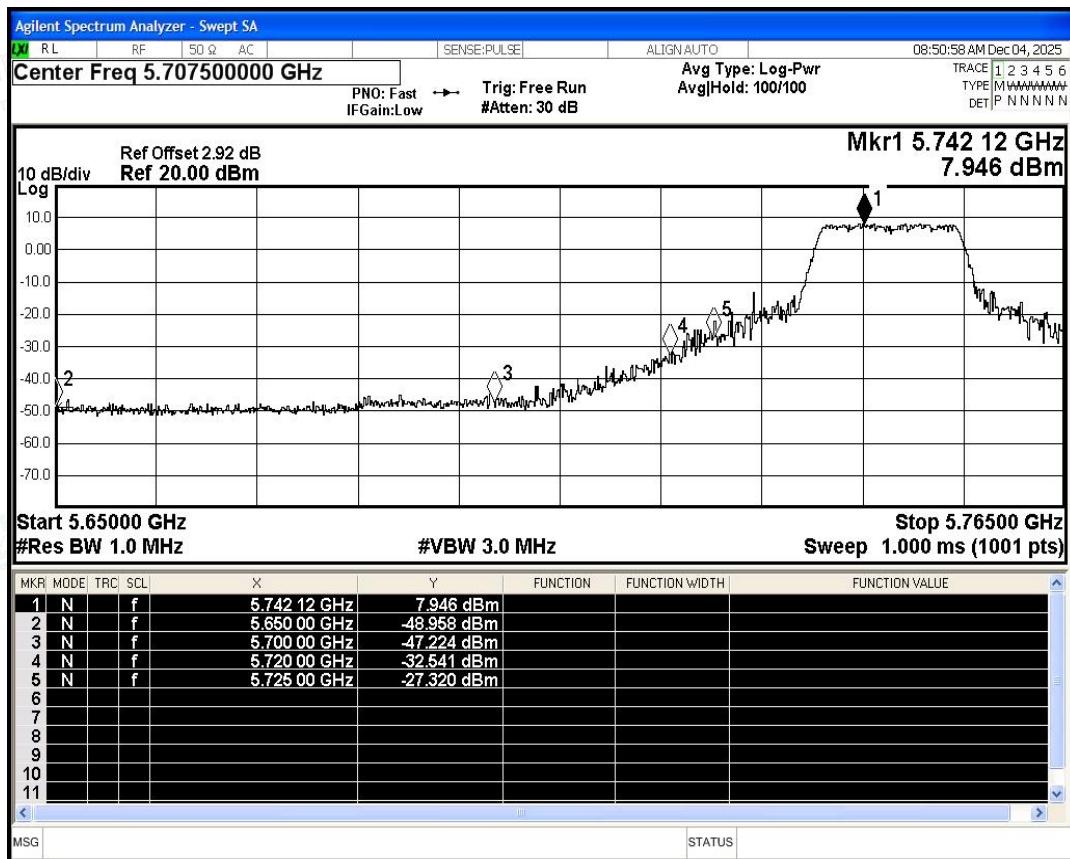
Restrict Band NVNT a 5745MHz Ant1 Peak
