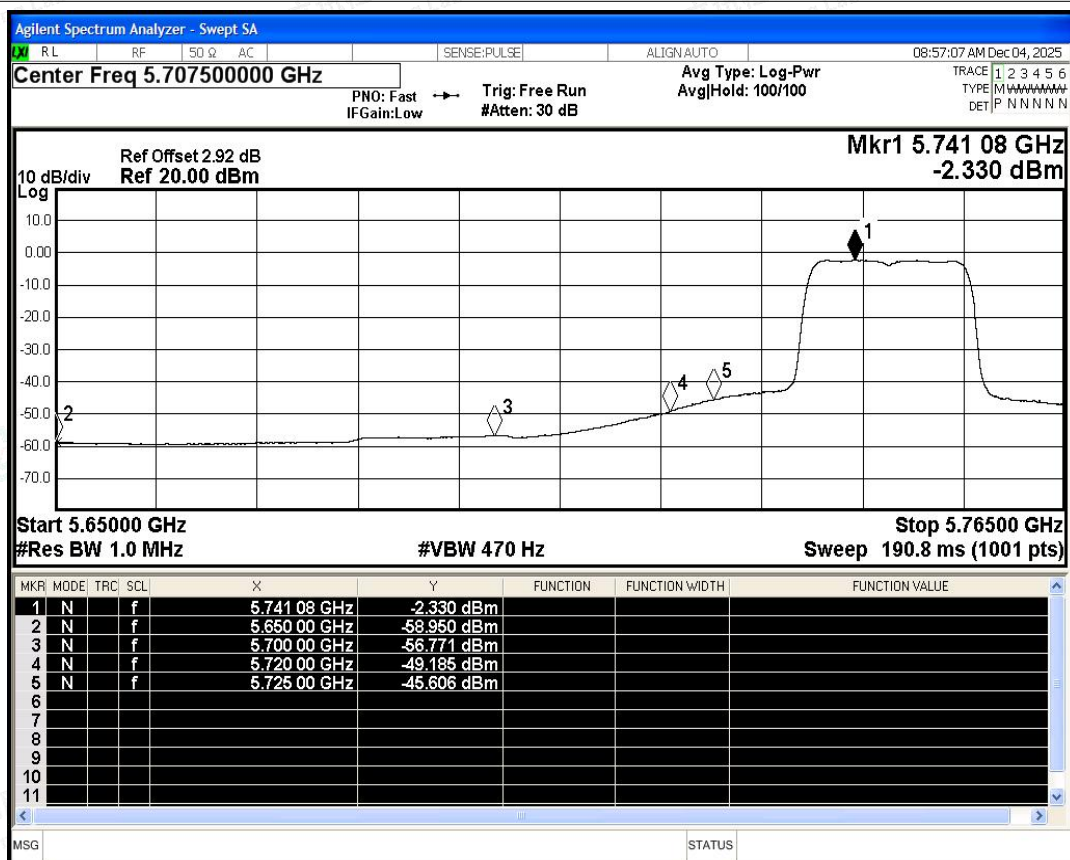
Restrict Band NVNT n20 5745MHz Ant1 Average
