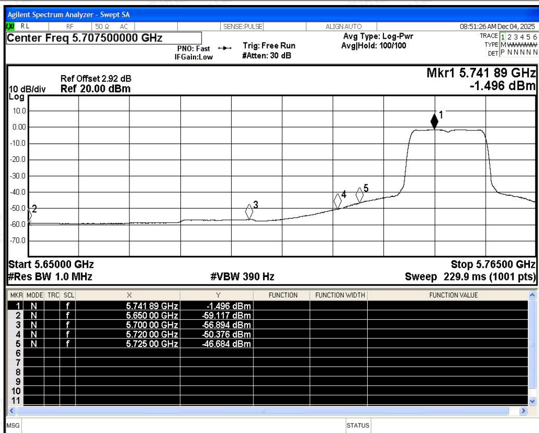
Restrict Band NVNT a 5745MHz Ant1 Average
