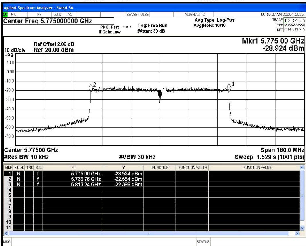
Freq. Stability NVNT ac80 5775MHz Ant1
