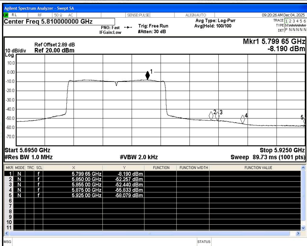
Restrict Band NVNT ac80 5775MHz Ant1 Average
