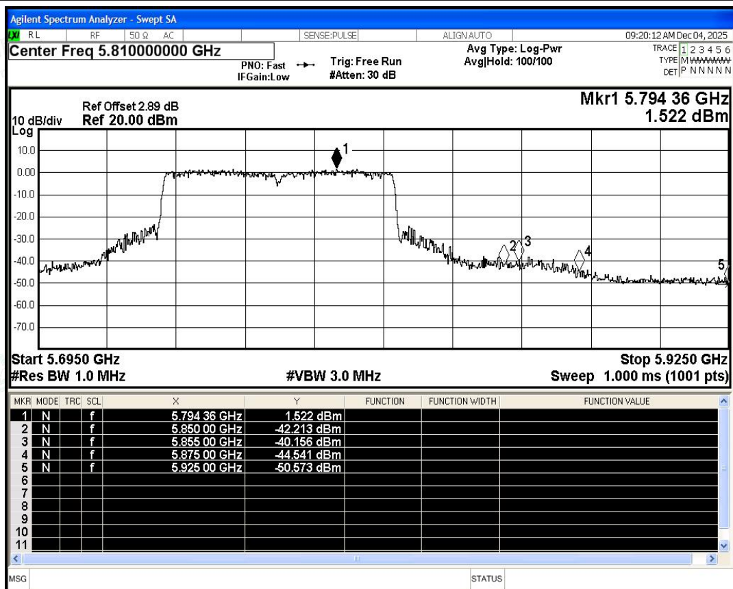
Restrict Band NVNT ac80 5775MHz Ant1 Peak
