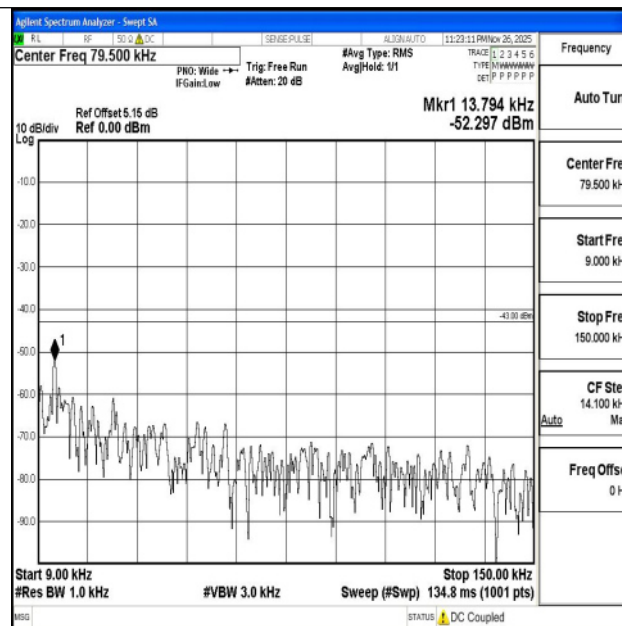
Band2_3MHz_16QAM_19185_1RB#0_0.009~0.15_0.009~0.15
