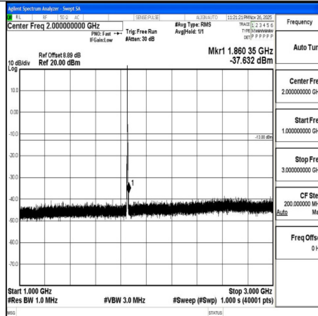
Band2_3MHz_16QAM_18615_1RB#0_1000~3000_1000~3000
