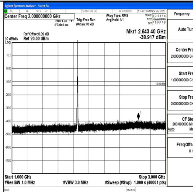
Band2_5MHz_16QAM_18625_1RB#0_1000~3000_1000~3000
