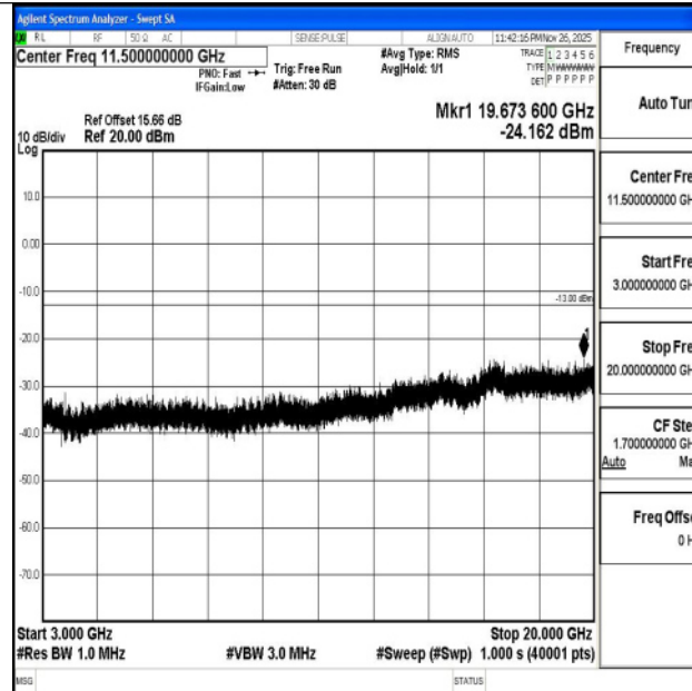
Band2_5MHz_16QAM_18625_1RB#0_3000~20000_3000~20000
