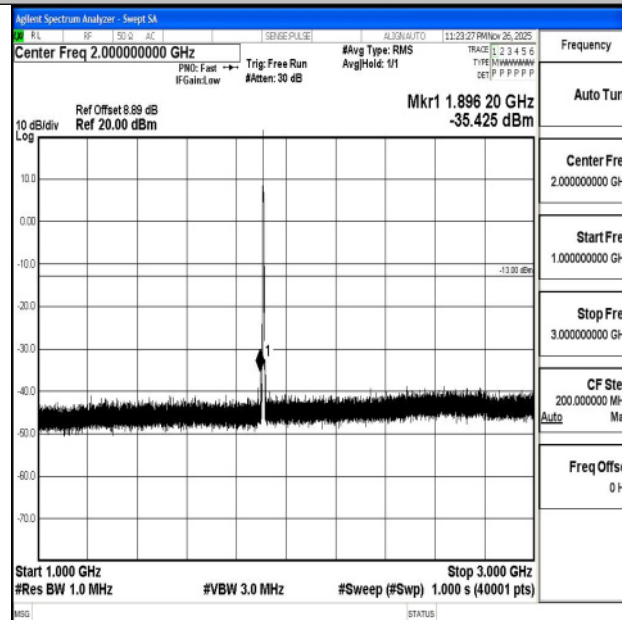
Band2_3MHz_16QAM_19185_1RB#0_1000~3000_1000~3000
