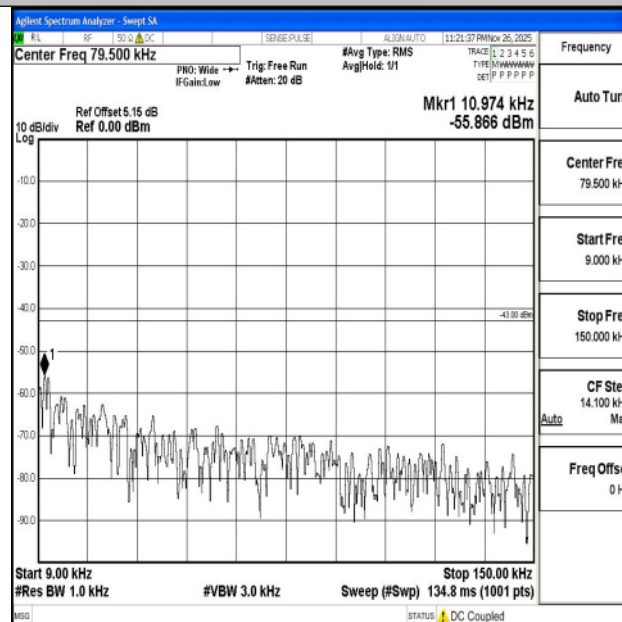
Band2_3MHz_QPSK_18900_1RB#0_0.009~0.15_0.009~0.15
