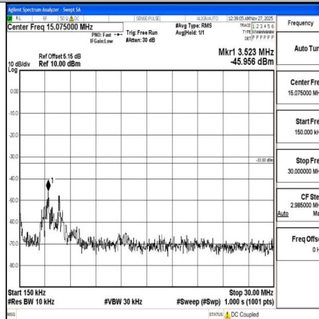
Band2_20MHz_16QAM_19100_1RB#0_0.15~30_0.15~30
