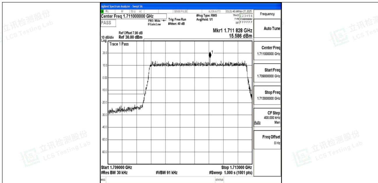
Band4_3MHz_QPSK_19965_15RB#0
