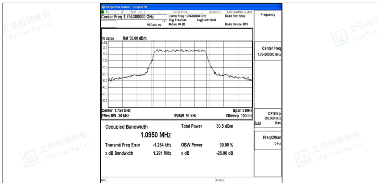
Band4-1.4MHz-QPSK-20393-6RB#0-PASS
