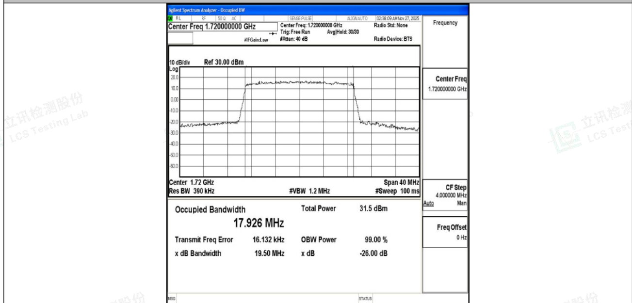
Band4-20MHz-16QAM-20050-100RB#0-PASS
