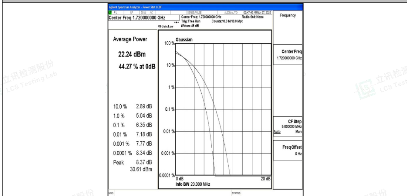
Band4-20MHz-16QAM-20050-100RB#0-PASS
