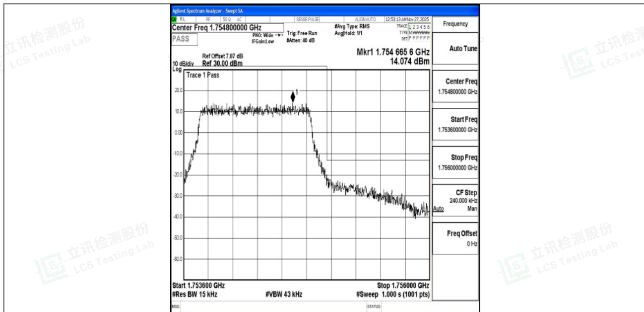
Band4_1.4MHz_QPSK_20393_6RB#0
