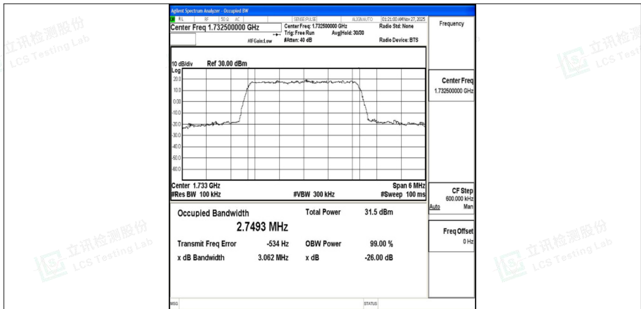
Band4-3MHz-QPSK-20175-15RB#0-PASS
