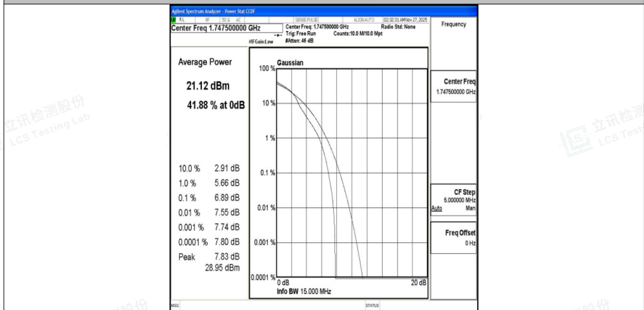
Band4-15MHz-16QAM-20325-1RB#0-PASS
