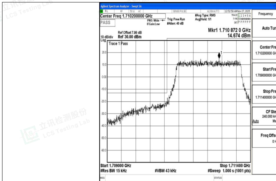
Band4_1.4MHz_QPSK_19957_6RB#0
