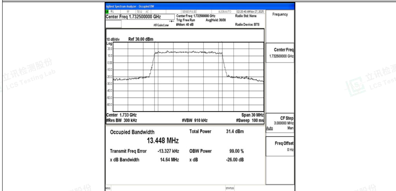
Band4-15MHz-16QAM-20175-75RB#0-PASS
