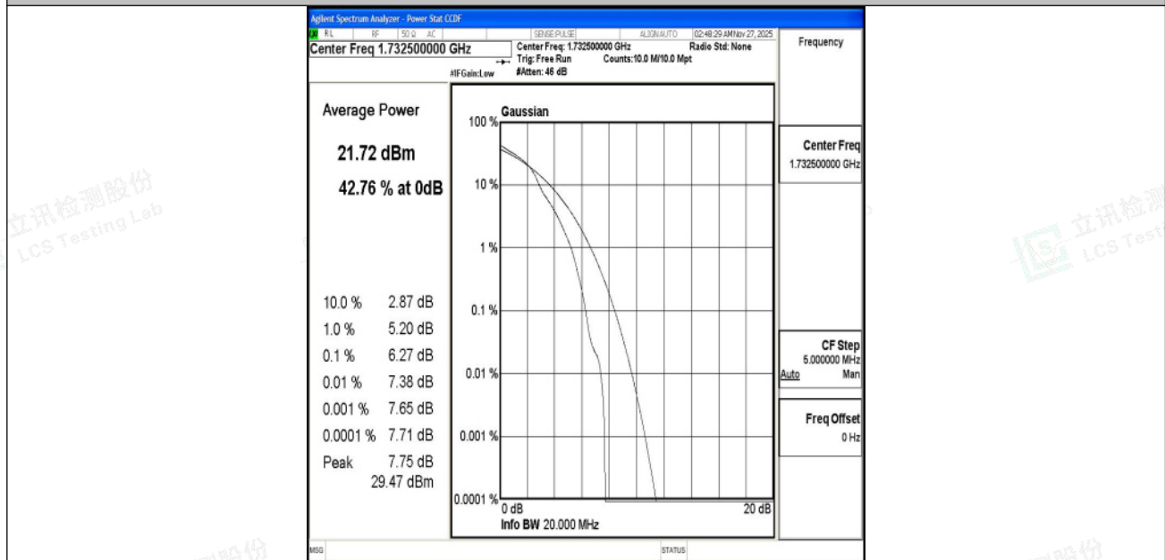
Band4-20MHz-16QAM-20175-1RB#0-PASS
