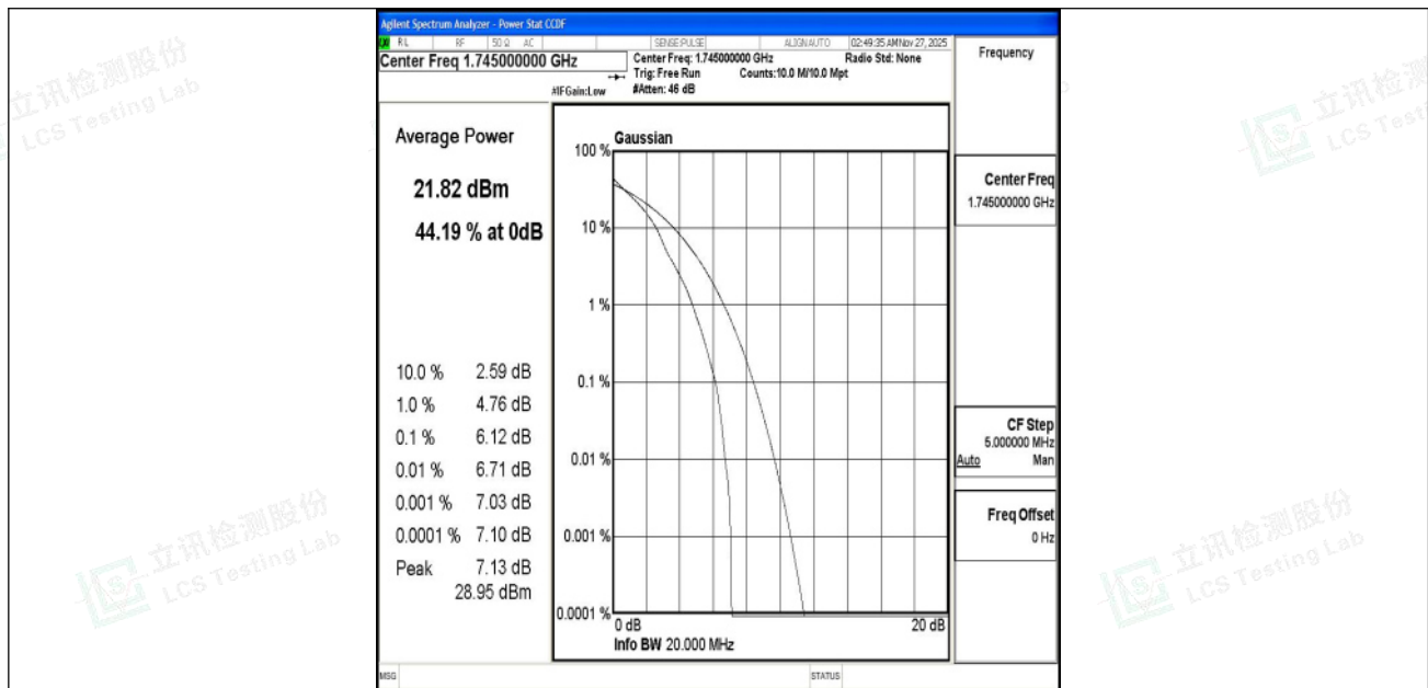
Band4-20MHz-QPSK-20300-1RB#0-PASS
