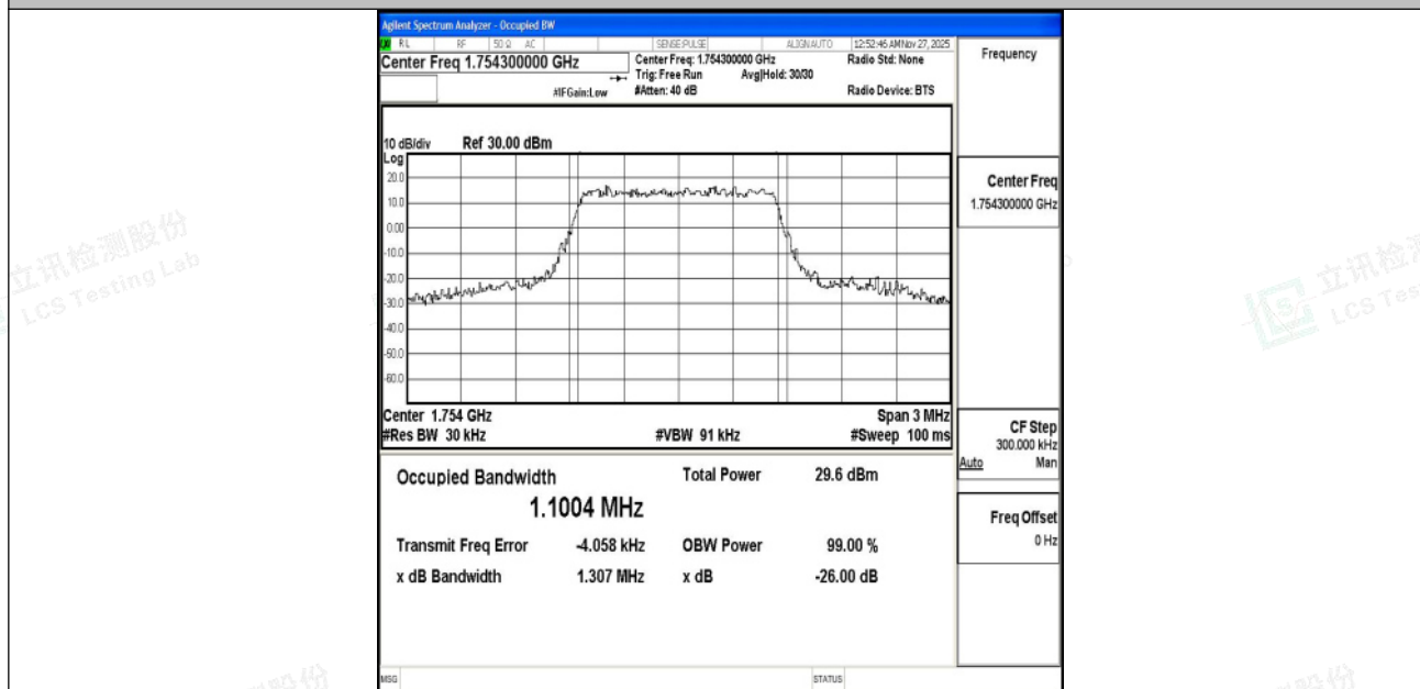
Band4-1.4MHz-16QAM-20393-6RB#0-PASS
