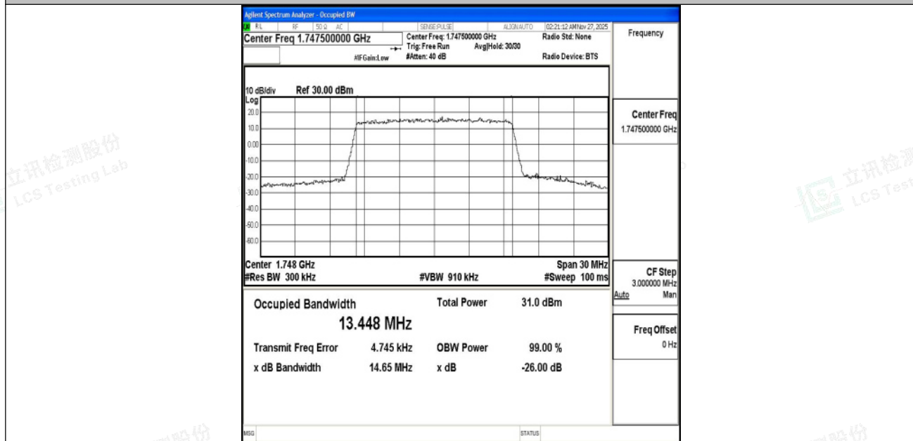
Band4-15MHz-16QAM-20325-75RB#0-PASS
