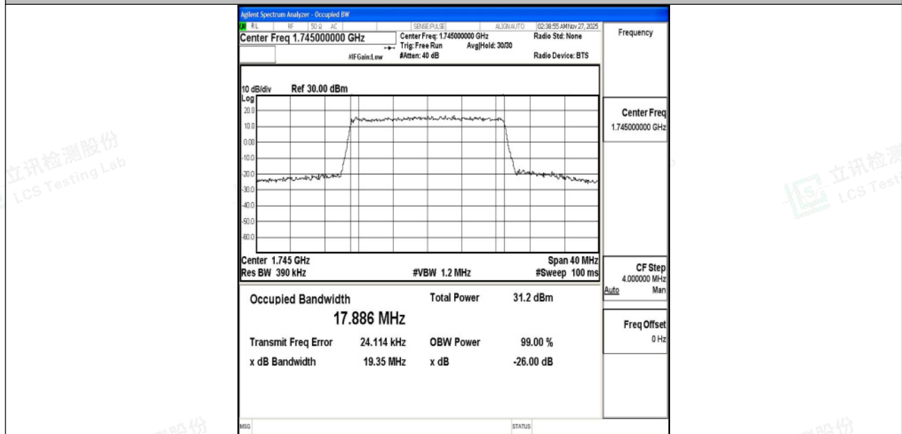
Band4-20MHz-16QAM-20300-100RB#0-PASS
