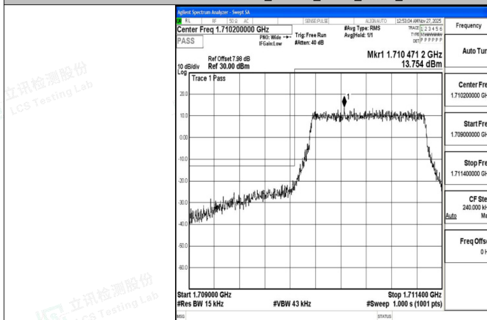
Band4_1.4MHz_16QAM_19957_6RB#0
