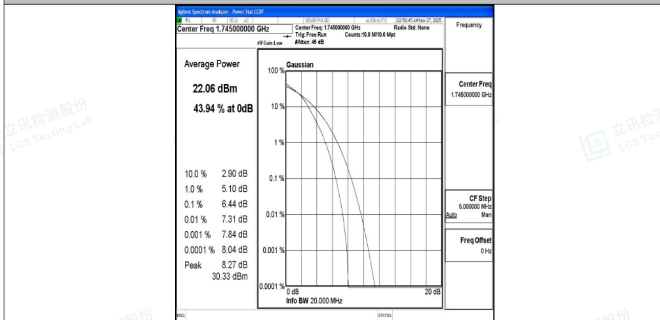
Band4-20MHz-16QAM-20300-100RB#0-PASS
