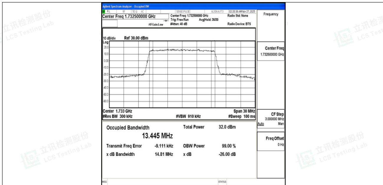
Band4-15MHz-QPSK-20175-75RB#0-PASS
