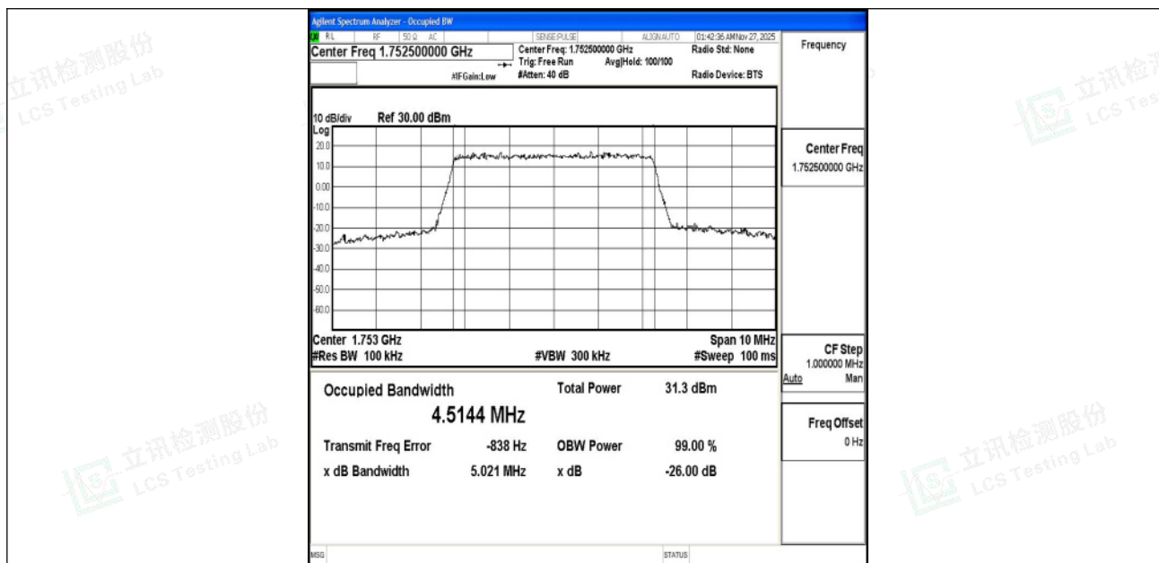
Band4-5MHz-QPSK-20375-25RB#0-PASS
