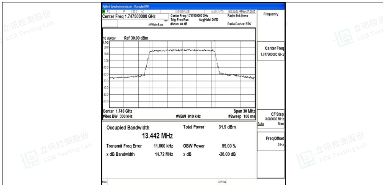
Band4-15MHz-QPSK-20325-75RB#0-PASS
