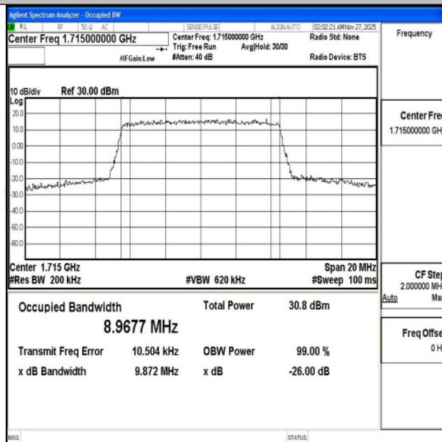
Band4-10MHz-16QAM-20000-50RB#0-PASS
