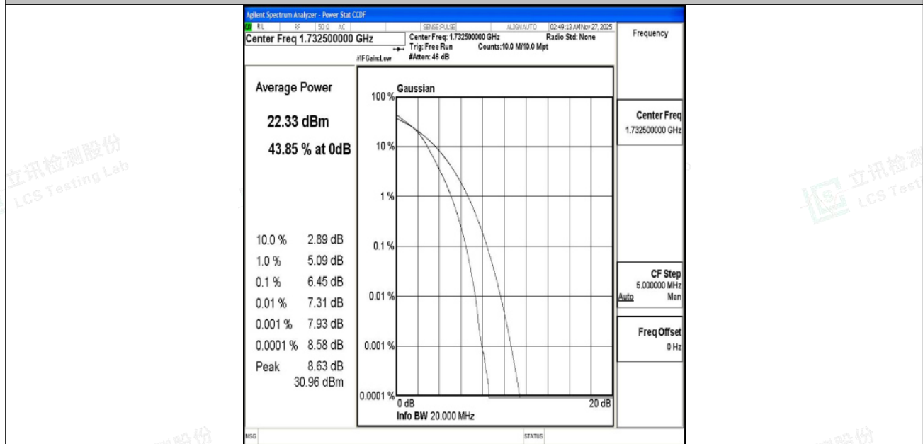
Band4-20MHz-16QAM-20175-100RB#0-PASS
