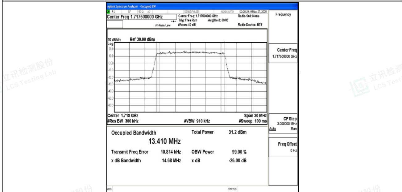
Band4-15MHz-16QAM-20025-75RB#0-PASS
