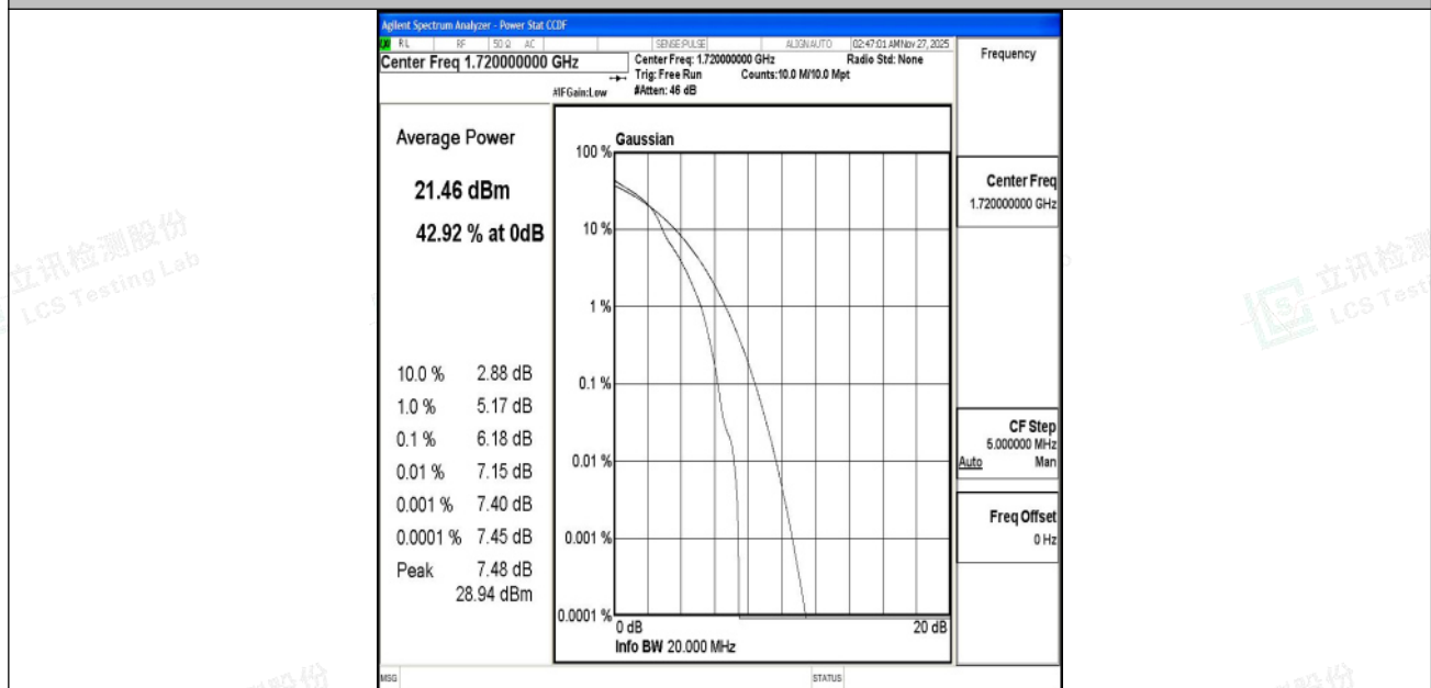
Band4-20MHz-16QAM-20050-1RB#0-PASS
