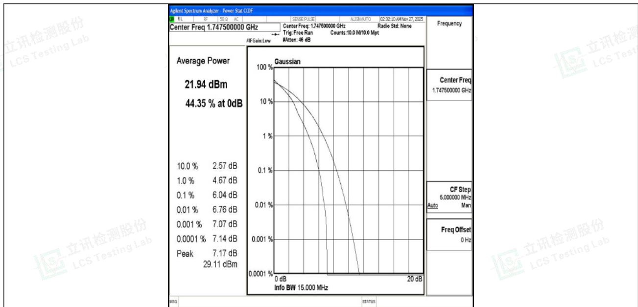
Band4-15MHz-QPSK-20325-1RB#0-PASS
