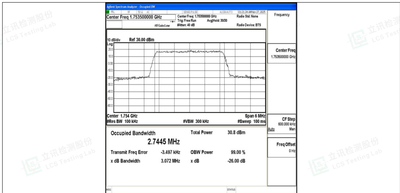
Band4-3MHz-QPSK-20385-15RB#0-PASS
