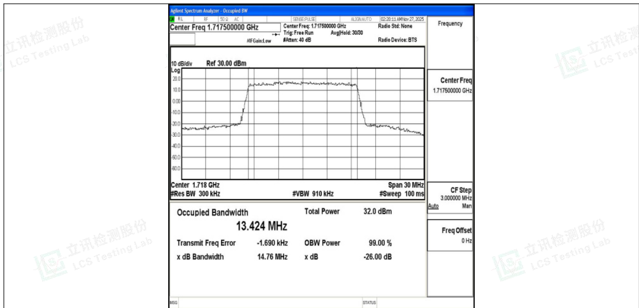
Band4-15MHz-QPSK-20025-75RB#0-PASS
