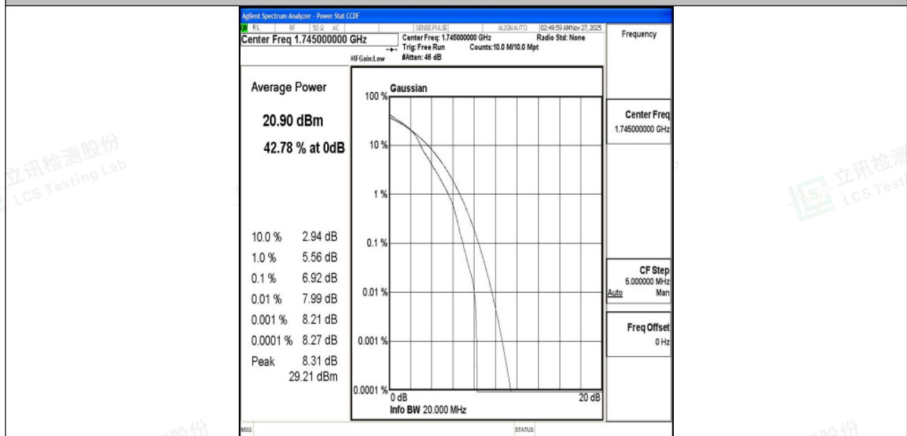
Band4-20MHz-16QAM-20300-1RB#0-PASS
