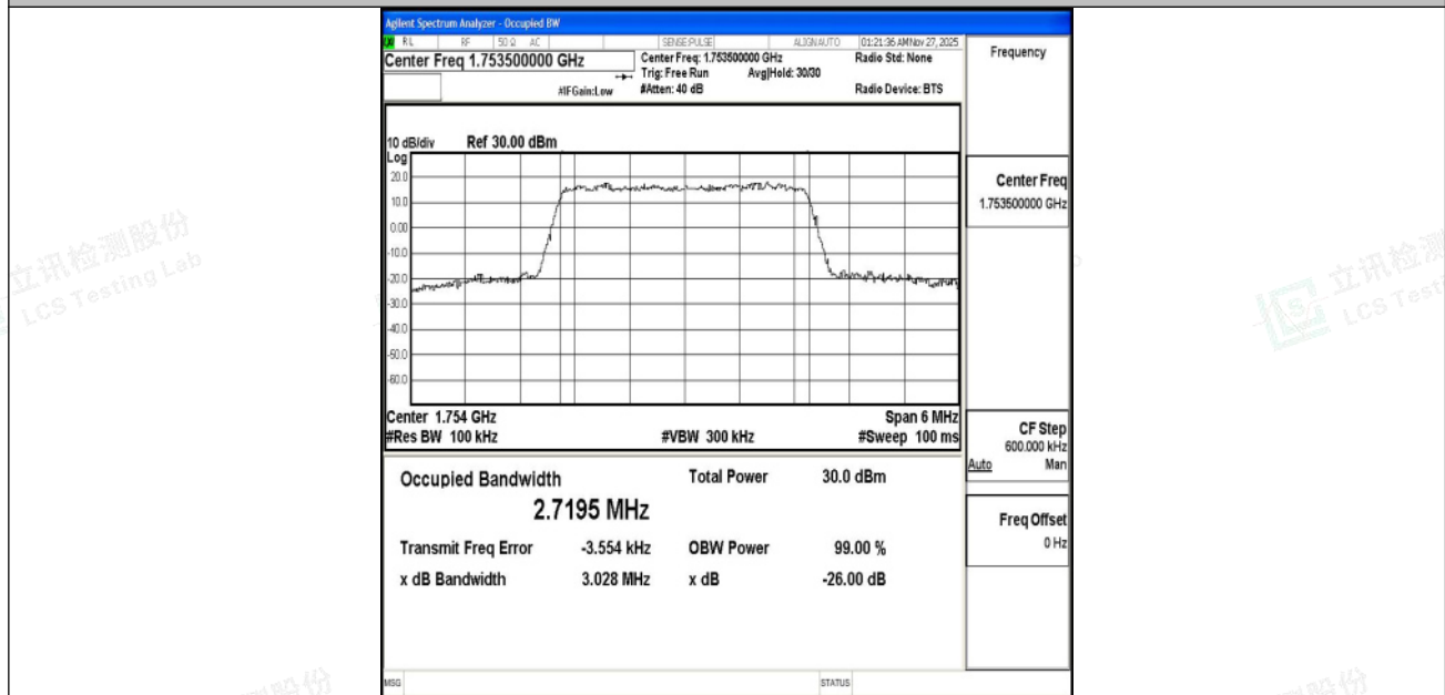
Band4-3MHz-16QAM-20385-15RB#0-PASS
