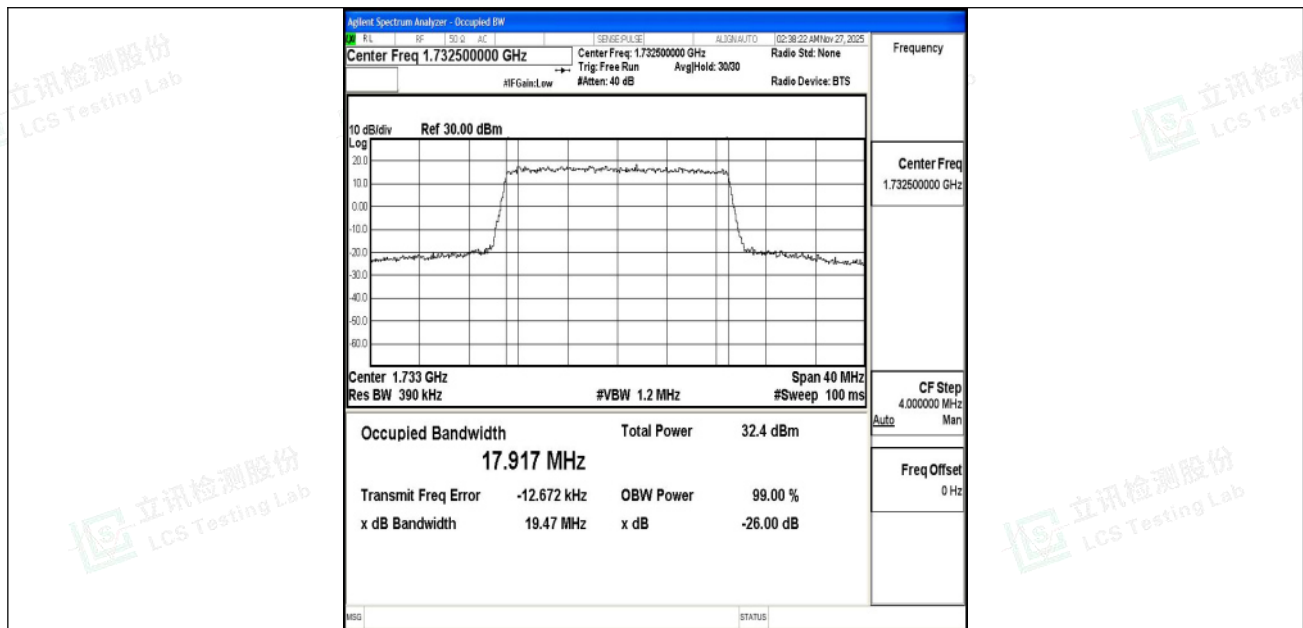
Band4-20MHz-QPSK-20175-100RB#0-PASS
