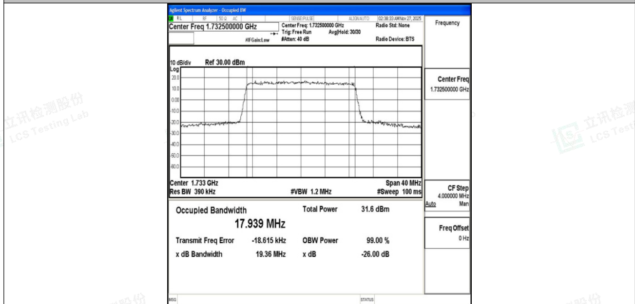
Band4-20MHz-16QAM-20175-100RB#0-PASS
