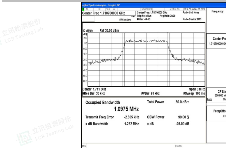
Band4-1.4MHz-16QAM-19957-6RB#0-PASS
