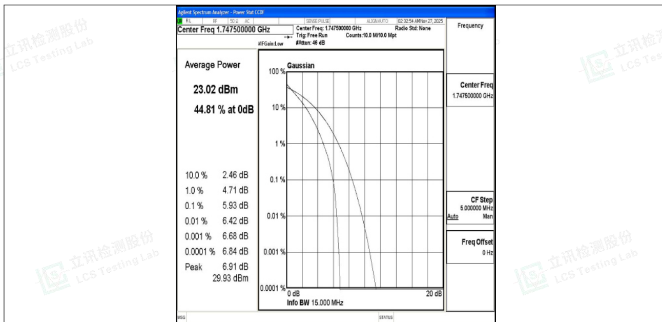
Band4-15MHz-QPSK-20325-75RB#0-PASS
