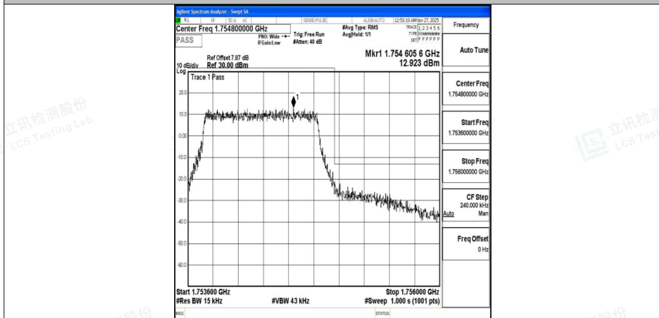
Band4_1.4MHz_16QAM_20393_6RB#0
