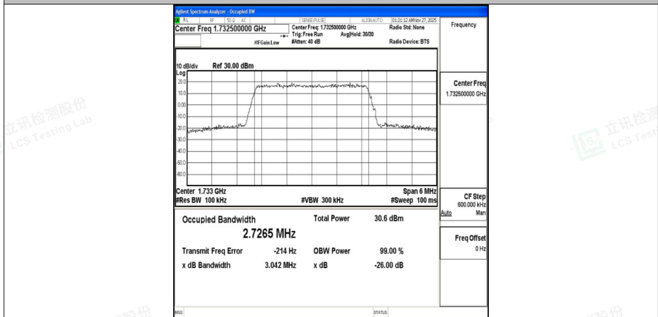
Band4-3MHz-16QAM-20175-15RB#0-PASS
