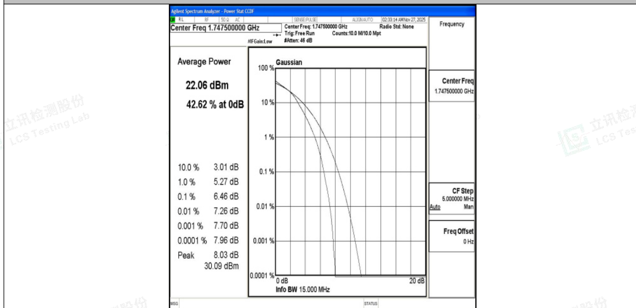
Band4-15MHz-16QAM-20325-75RB#0-PASS
