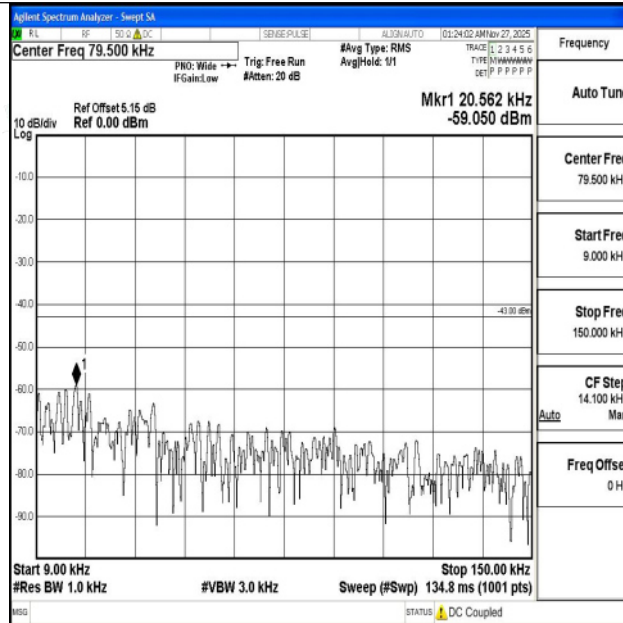
Band4_3MHz_16QAM_20175_1RB#0_0.009~0.15_0.009~0.15
