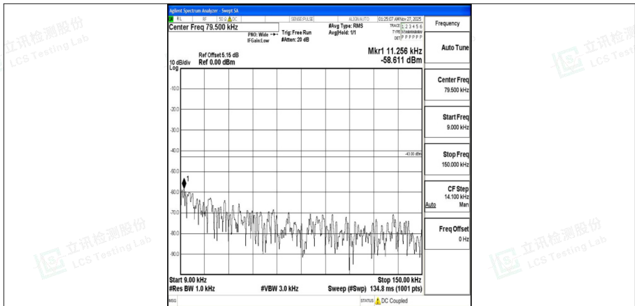
Band4_3MHz_16QAM_20385_1RB#0_0.009~0.15_0.009~0.15
