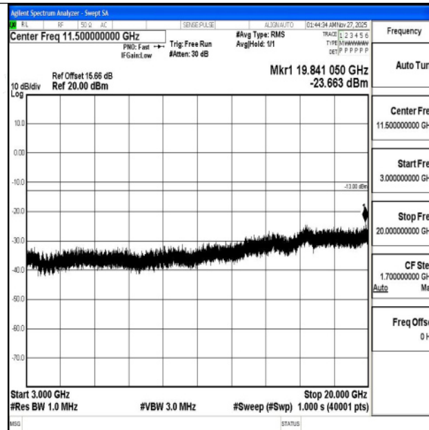
Band4_5MHz_16QAM_19975_1RB#0_3000~20000_3000~20000
