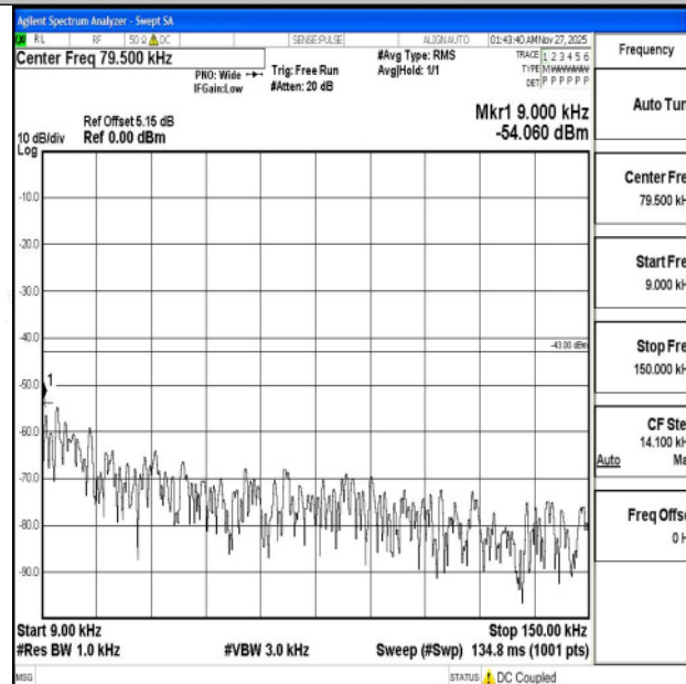
Band4_5MHz_QPSK_19975_1RB#0_0.009~0.15_0.009~0.15
