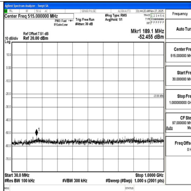
Band4_5MHz_16QAM_19975_1RB#0_30~1000_30~1000
