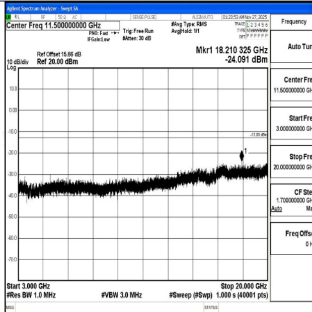
Band4_3MHz_QPSK_20175_1RB#0_3000~20000_3000~20000
