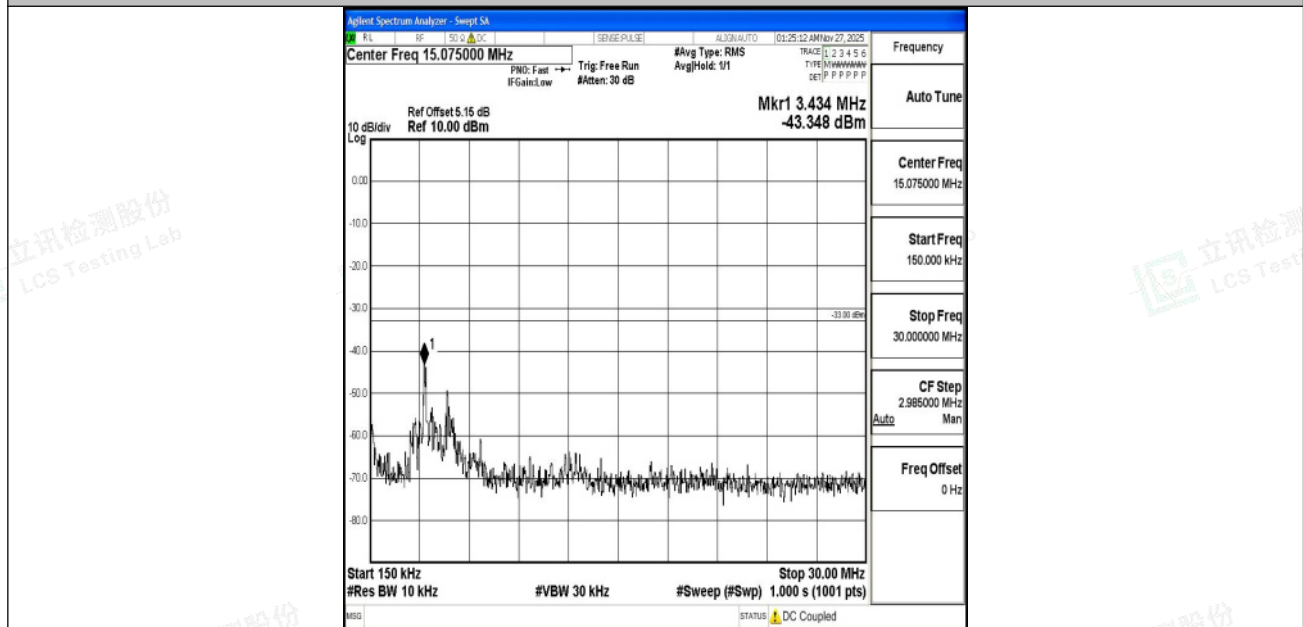
Band4_3MHz_16QAM_20385_1RB#0_0.15~30_0.15~30
