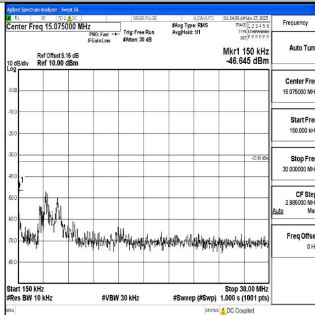
Band4_3MHz_16QAM_20175_1RB#0_0.15~30_0.15~30
