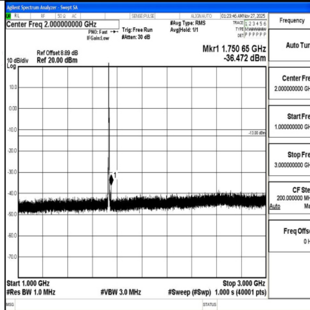
Band4_3MHz_QPSK_20175_1RB#0_1000~3000_1000~3000
