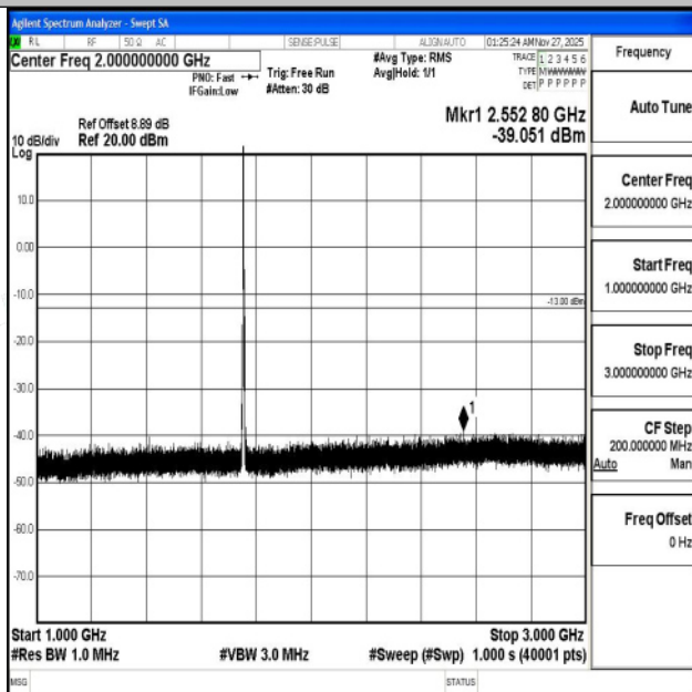
Band4_3MHz_16QAM_20385_1RB#0_1000~3000_1000~3000
