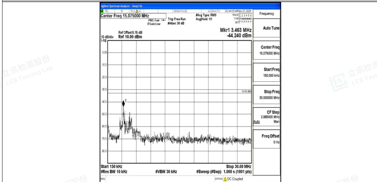
Band4_5MHz_16QAM_19975_1RB#0_0.15~30_0.15~30
