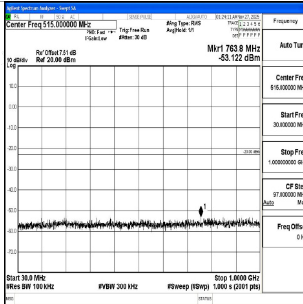
Band4_3MHz_16QAM_20175_1RB#0_30~1000_30~1000
