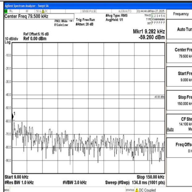
Band4_5MHz_QPSK_20175_1RB#0_0.009~0.15_0.009~0.15
