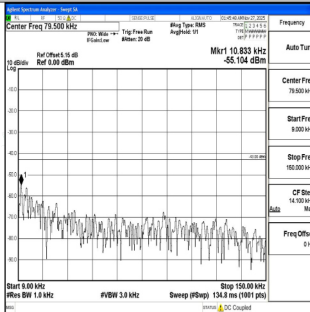
Band4_5MHz_QPSK_20375_1RB#0_0.009~0.15_0.009~0.15
