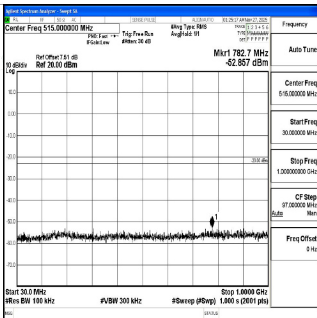
Band4_3MHz_16QAM_20385_1RB#0_30~1000_30~1000
