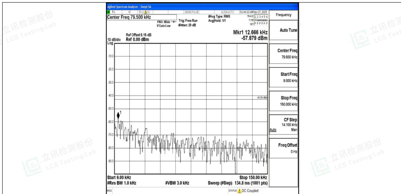
Band4_5MHz_16QAM_19975_1RB#0_0.009~0.15_0.009~0.15
