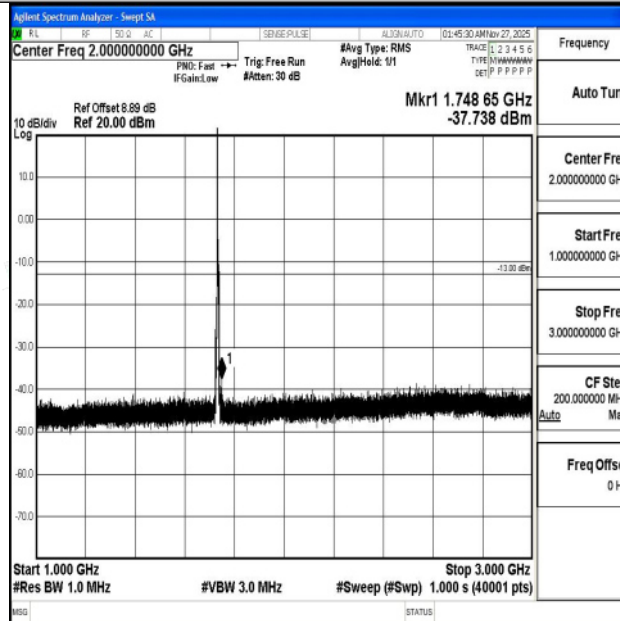
Band4_5MHz_16QAM_20175_1RB#0_1000~3000_1000~3000
