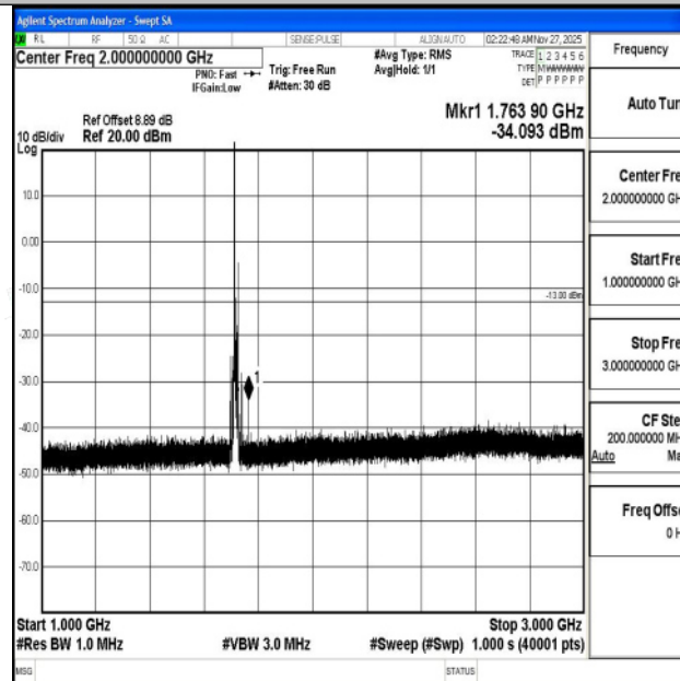
Band4_15MHz_16QAM_20025_1RB#0_1000~3000_1000~3000
