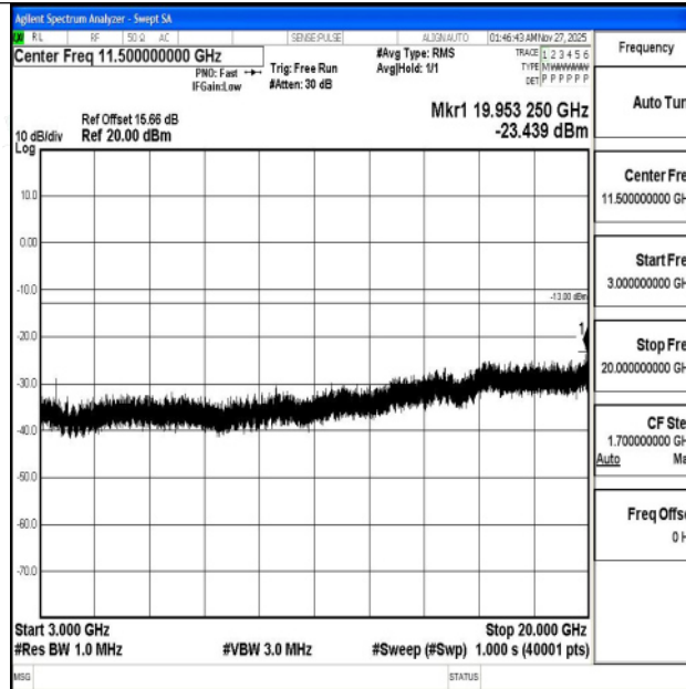
Band4_5MHz_16QAM_20375_1RB#0_3000~20000_3000~20000
