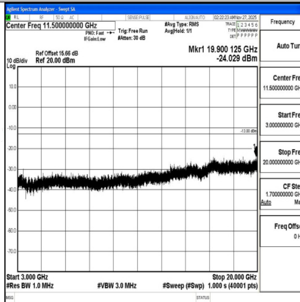
Band4_15MHz_QPSK_20025_1RB#0_3000~20000_3000~20000
