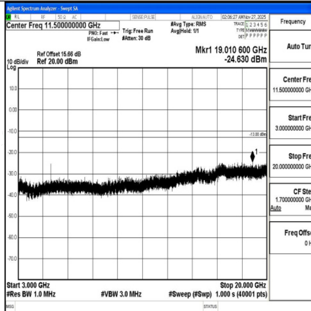
Band4_10MHz_QPSK_20350_1RB#0_3000~20000_3000~20000
