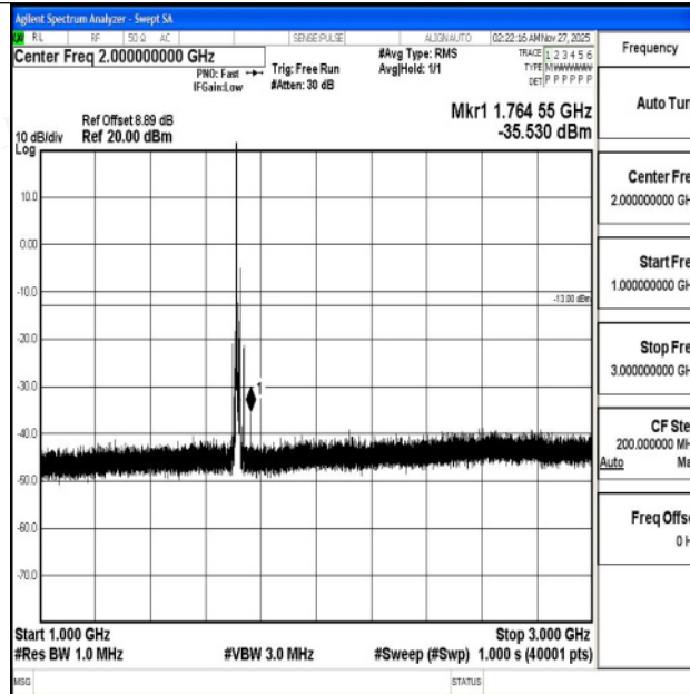
Band4_15MHz_QPSK_20025_1RB#0_1000~3000_1000~3000
