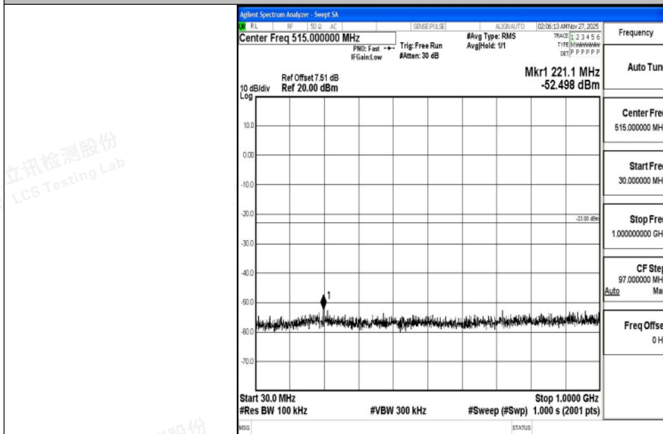
Band4_10MHz_QPSK_20350_1RB#0_30~1000_30~1000
