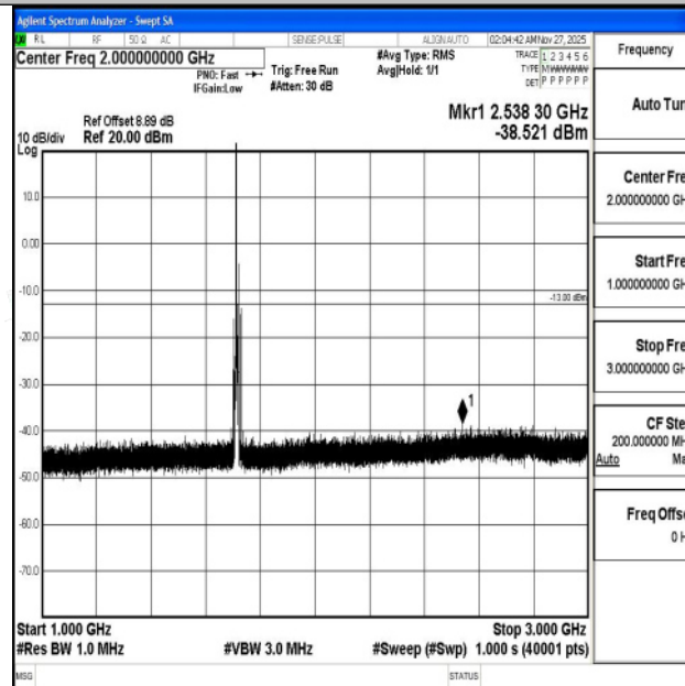
Band4_10MHz_16QAM_20000_1RB#0_1000~3000_1000~3000
