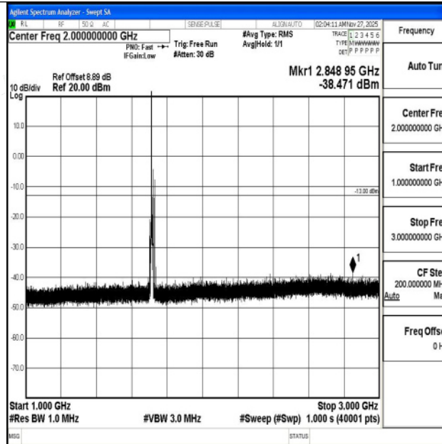
Band4_10MHz_QPSK_20000_1RB#0_1000~3000_1000~3000
