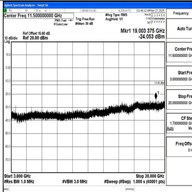
Band4_5MHz_QPSK_20375_1RB#0_3000~20000_3000~20000
