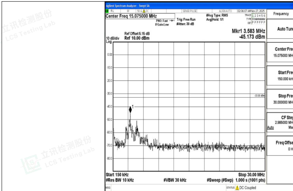
Band4_10MHz_QPSK_20350_1RB#0_0.15~30_0.15~30
