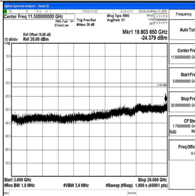
Band4_10MHz_QPSK_20000_1RB#0_3000~20000_3000~20000
