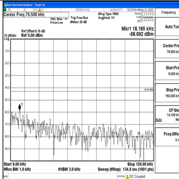
Band4_10MHz_QPSK_20000_1RB#0_0.009~0.15_0.009~0.15
