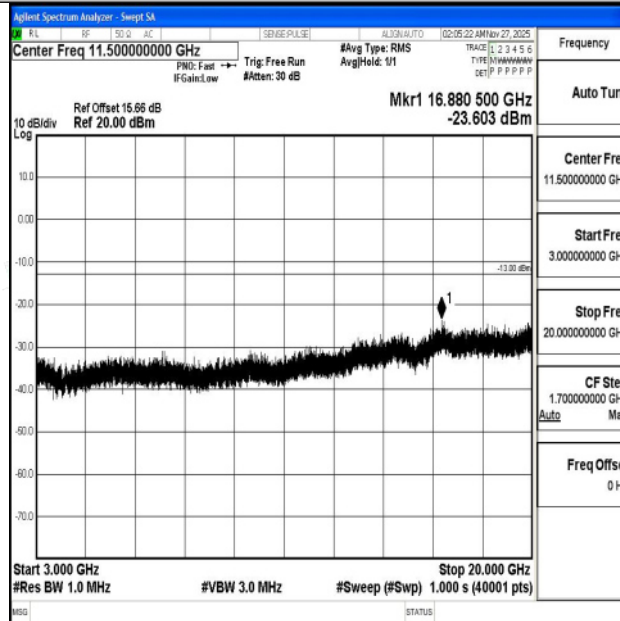
Band4_10MHz_QPSK_20175_1RB#0_3000~20000_3000~20000
