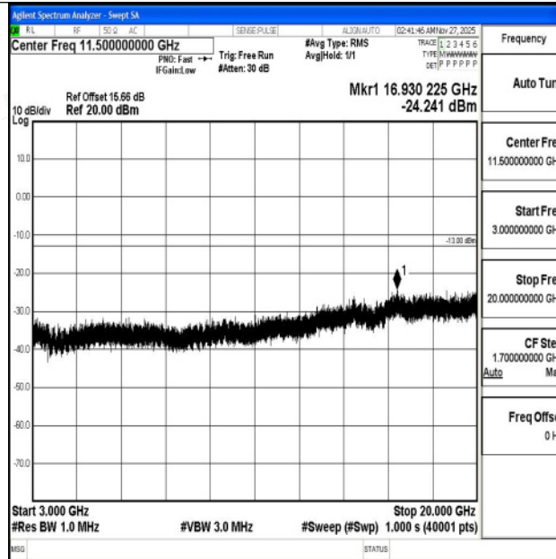
Band4_20MHz_16QAM_20175_1RB#0_3000~20000_3000~20000
