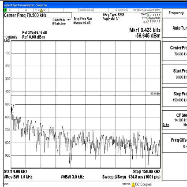
Band4_20MHz_QPSK_20050_1RB#0_0.009~0.15_0.009~0.15
