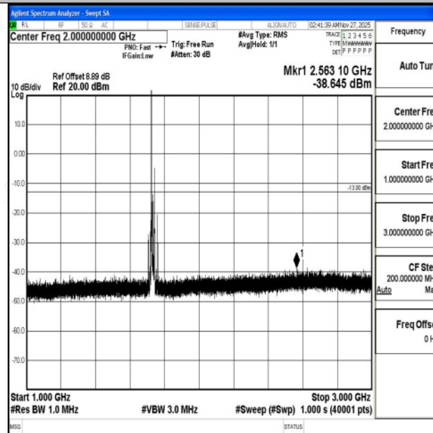
Band4_20MHz_16QAM_20175_1RB#0_1000~3000_1000~3000
