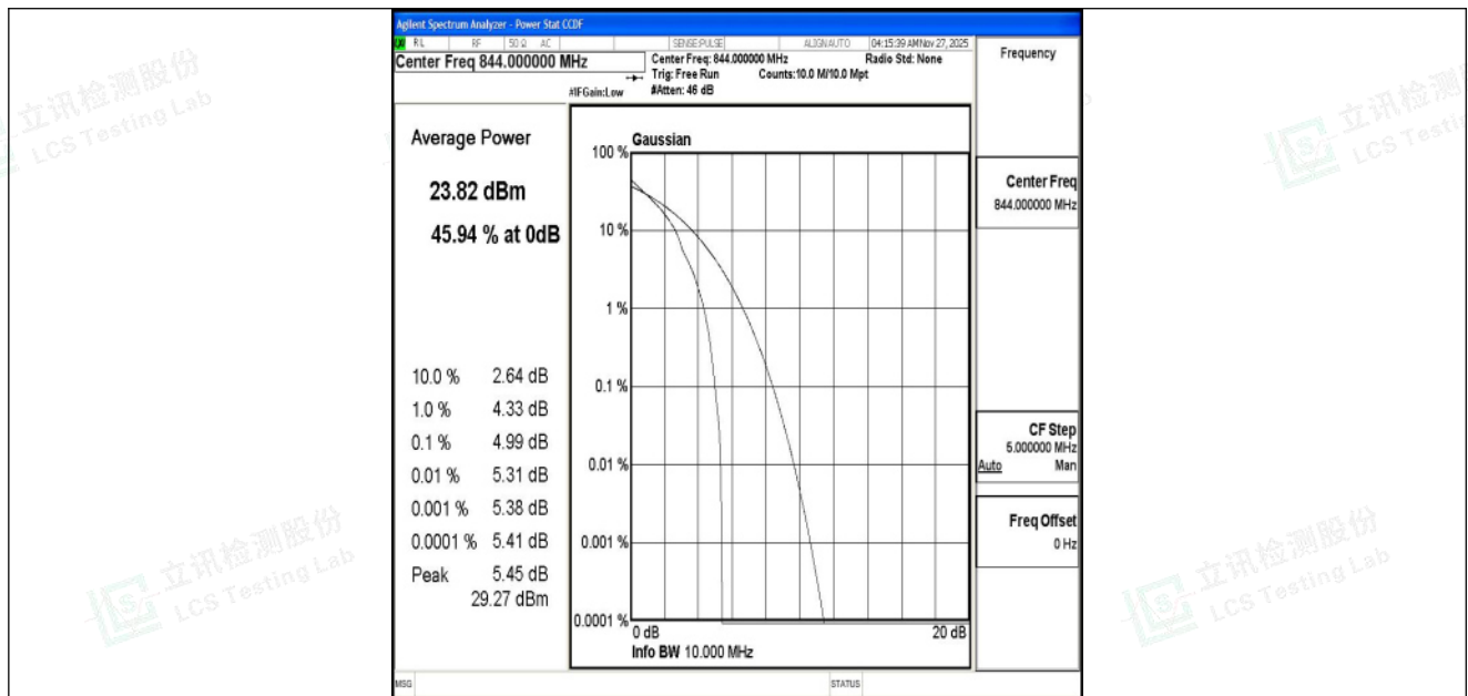
Band5-10MHz-QPSK-20600-1RB#0-PASS
