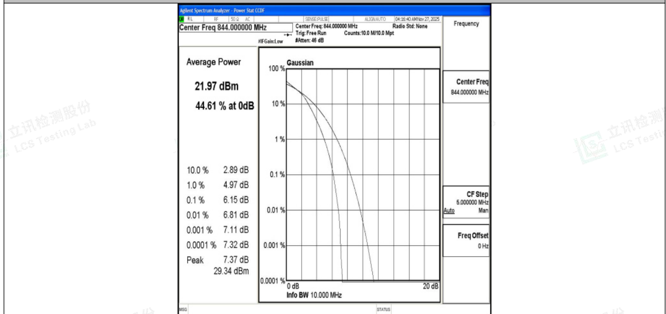
Band5-10MHz-16QAM-20600-50RB#0-PASS
