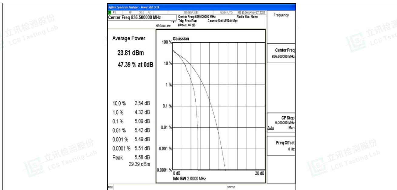
Band5-1.4MHz-QPSK-20525-1RB#0-PASS
