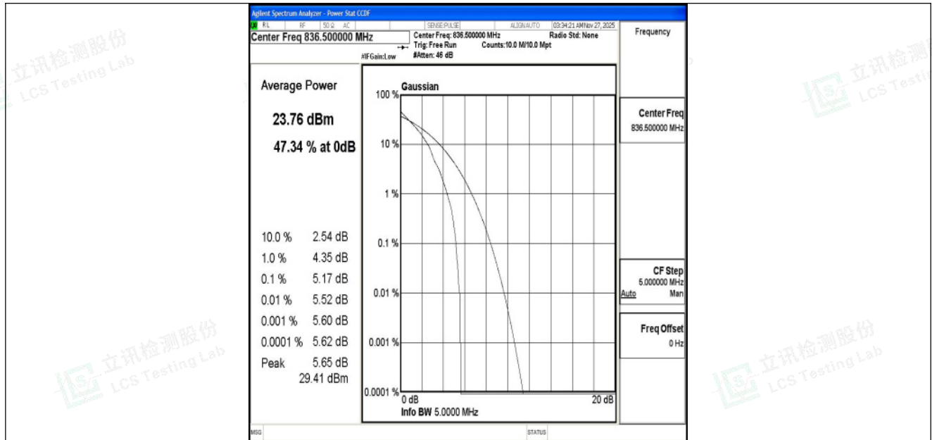
Band5-3MHz-QPSK-20525-1RB#0-PASS
