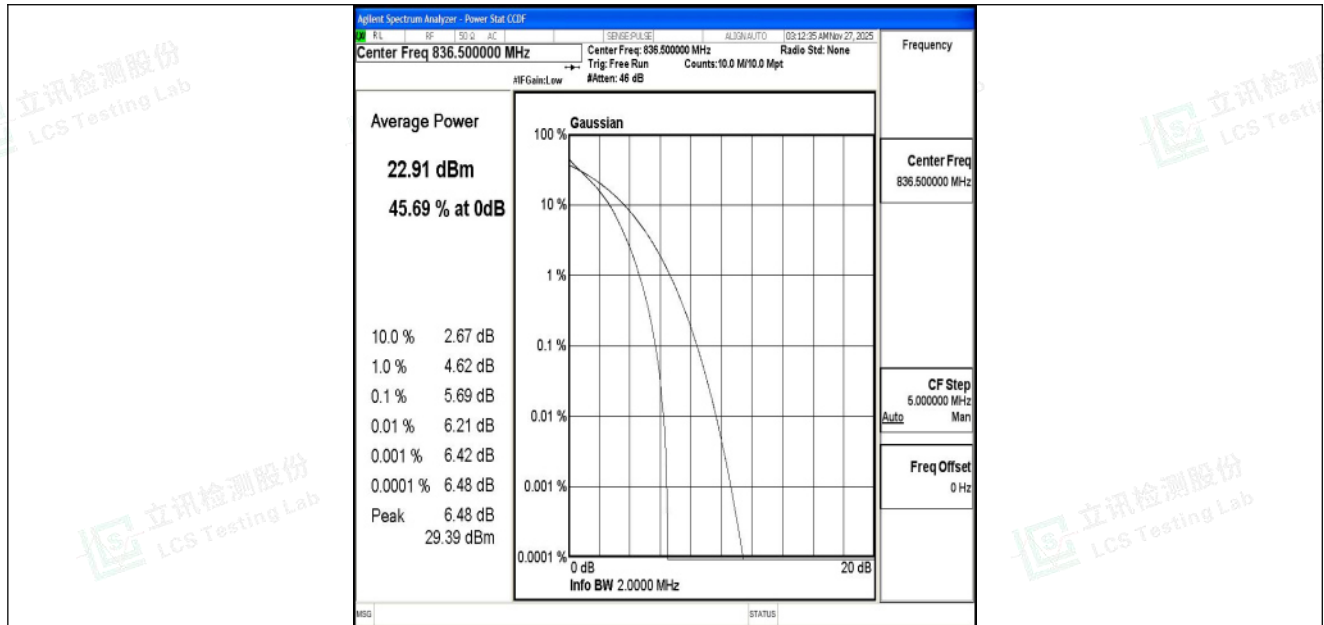
Band5-1.4MHz-QPSK-20525-6RB#0-PASS
