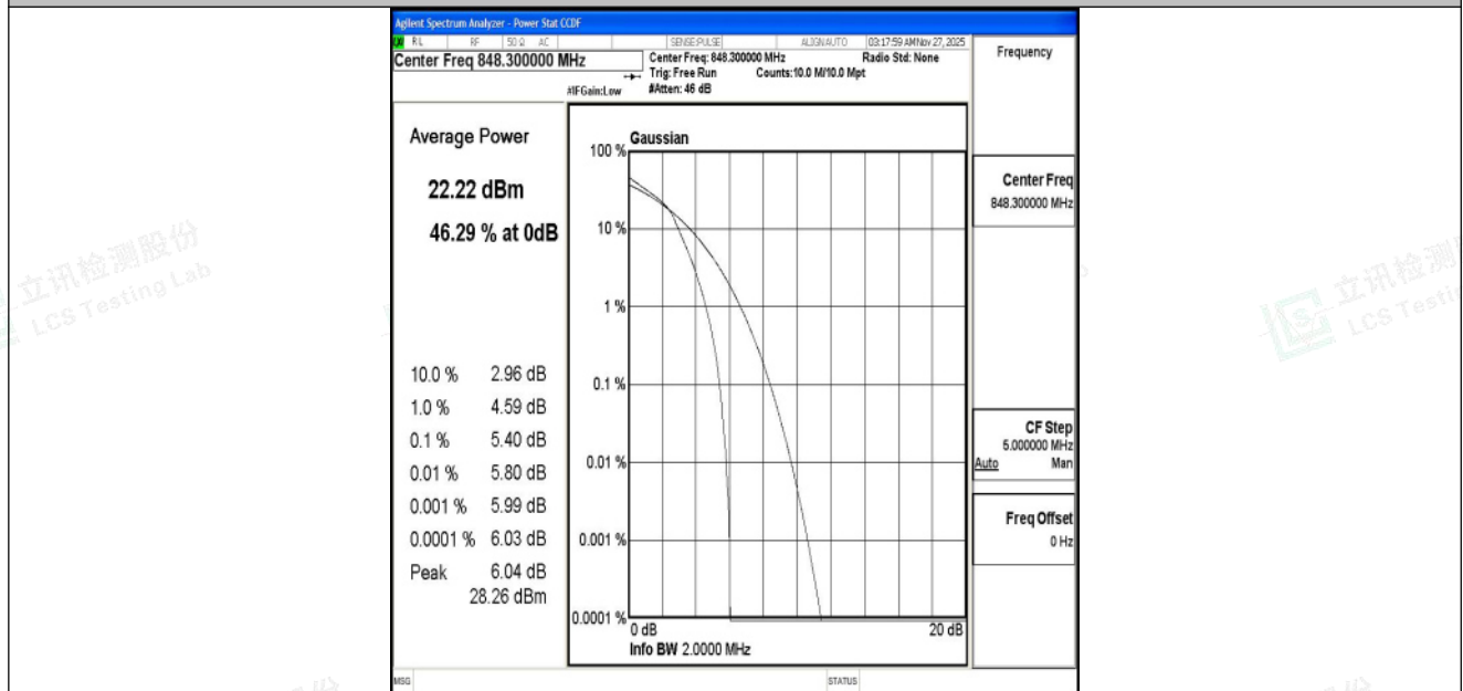
Band5-1.4MHz-16QAM-20643-6RB#0-PASS
