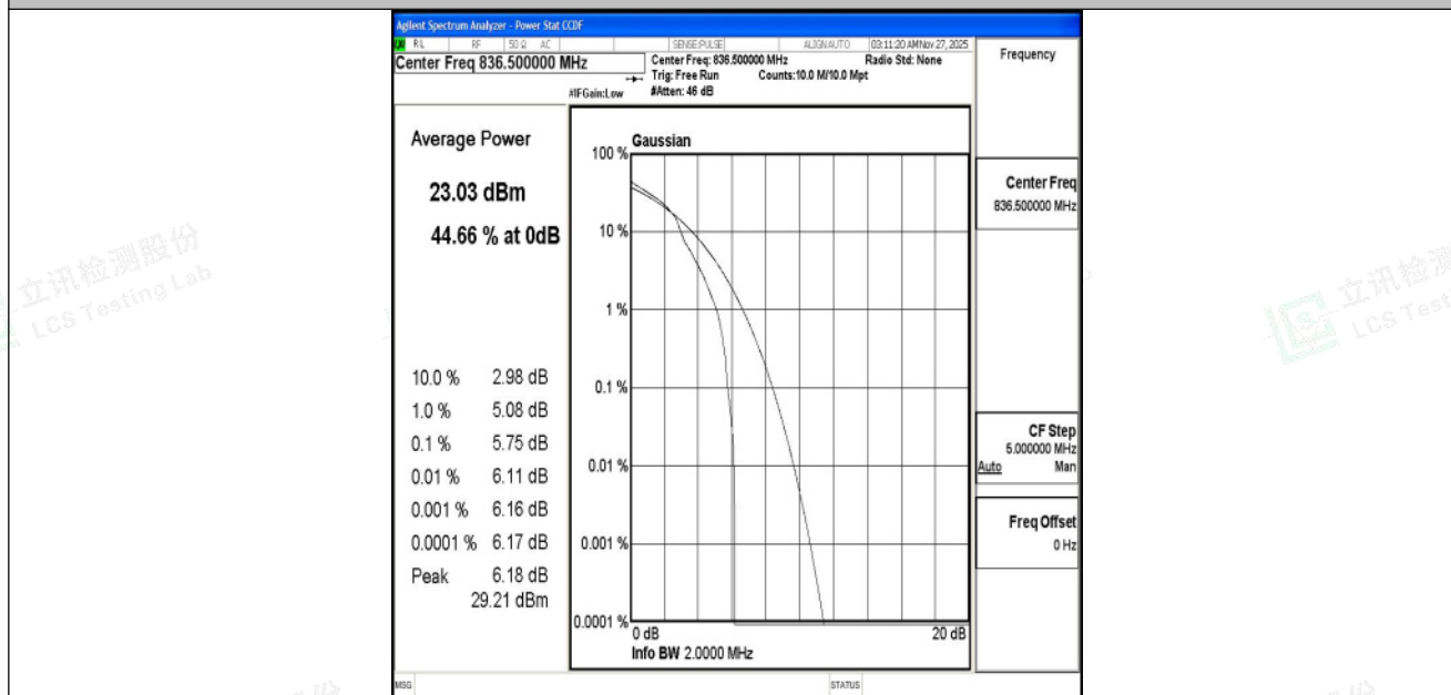
Band5-1.4MHz-16QAM-20525-1RB#0-PASS
