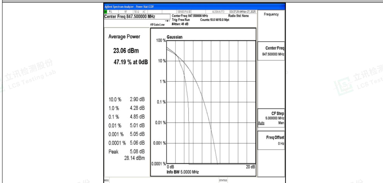
Band5-3MHz-16QAM-20635-1RB#0-PASS
