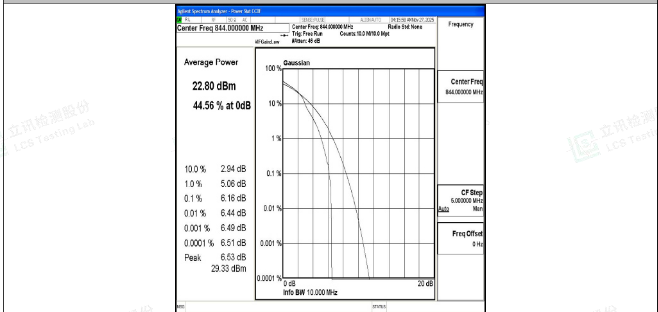
Band5-10MHz-16QAM-20600-1RB#0-PASS
