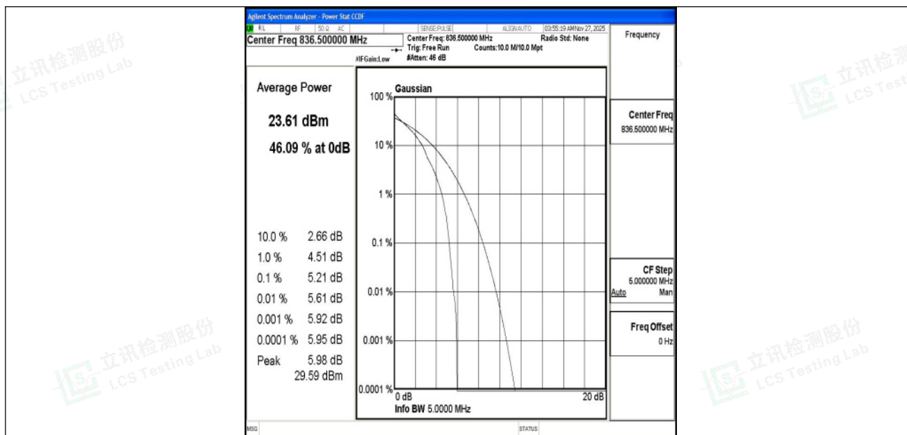
Band5-5MHz-QPSK-20525-1RB#0-PASS
