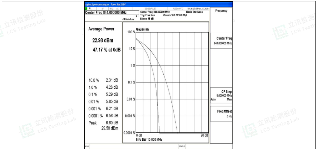
Band5-10MHz-QPSK-20600-50RB#0-PASS
