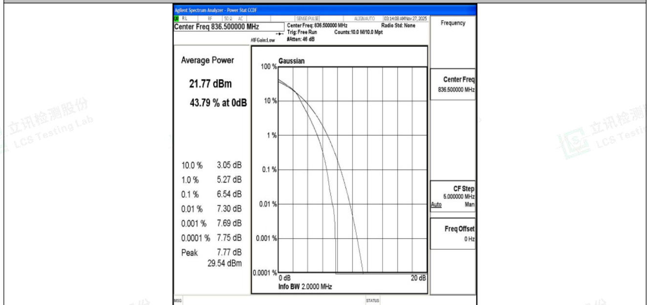
Band5-1.4MHz-16QAM-20525-6RB#0-PASS
