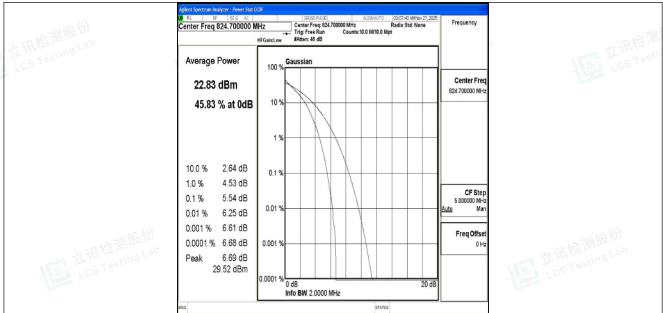
Band5-1.4MHz-QPSK-20407-6RB#0-PASS
