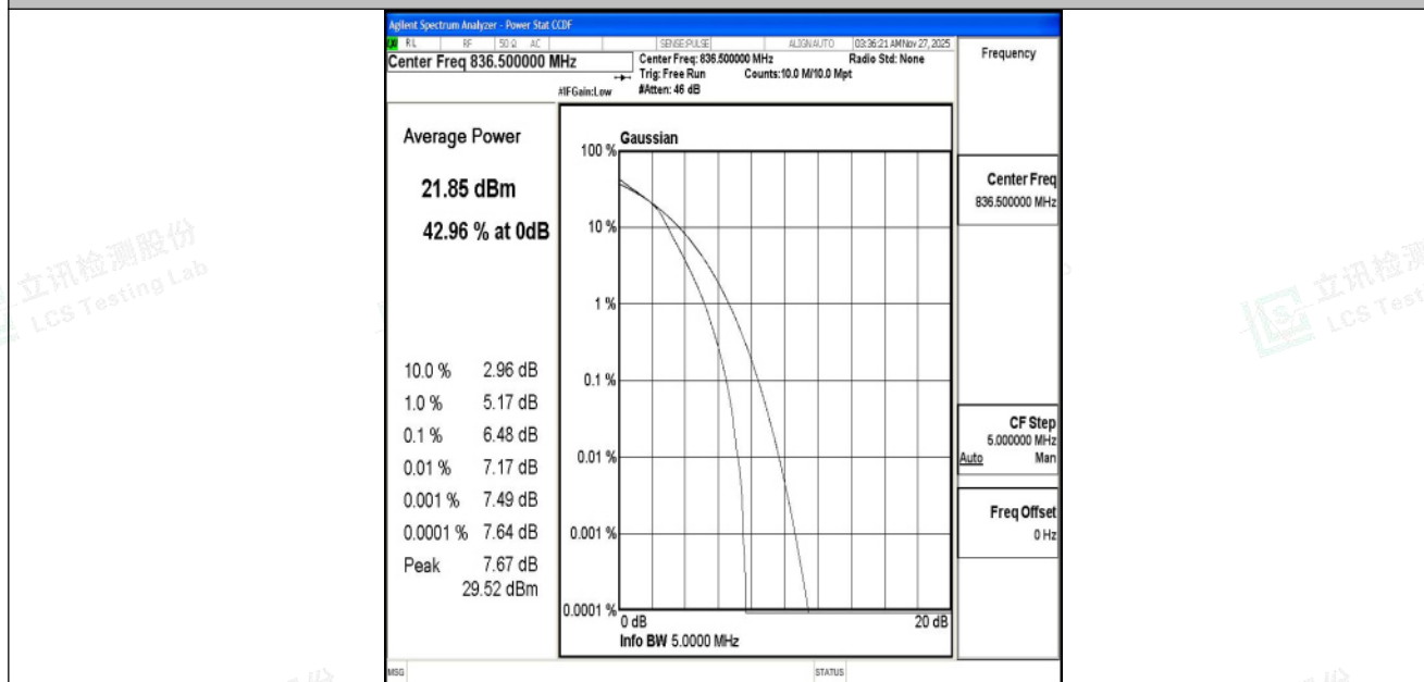
Band5-3MHz-16QAM-20525-15RB#0-PASS
