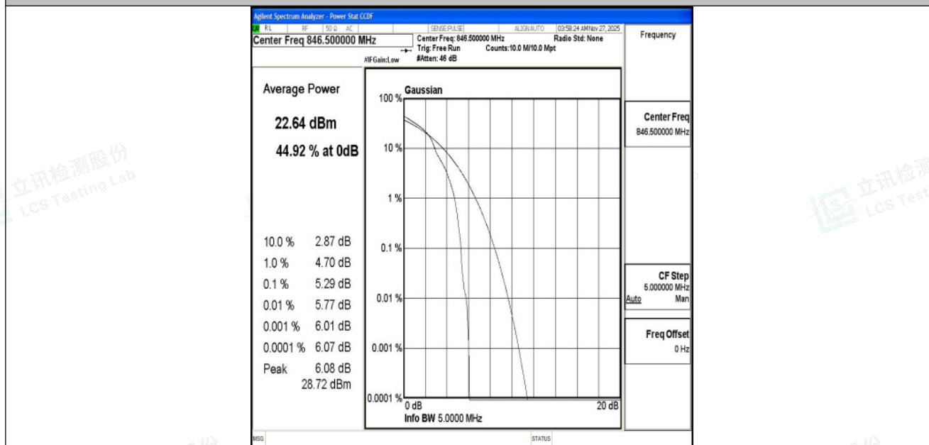
Band5-5MHz-16QAM-20625-1RB#0-PASS
