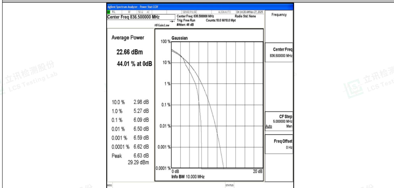
Band5-10MHz-16QAM-20525-1RB#0-PASS
