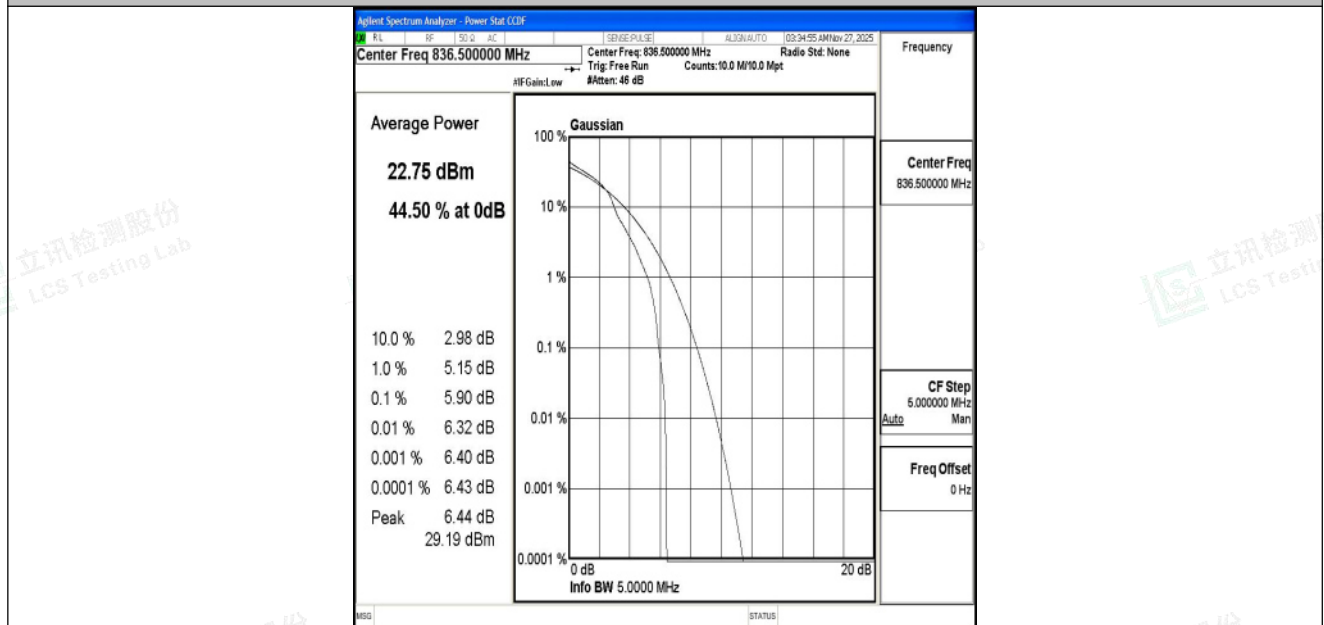
Band5-3MHz-16QAM-20525-1RB#0-PASS
