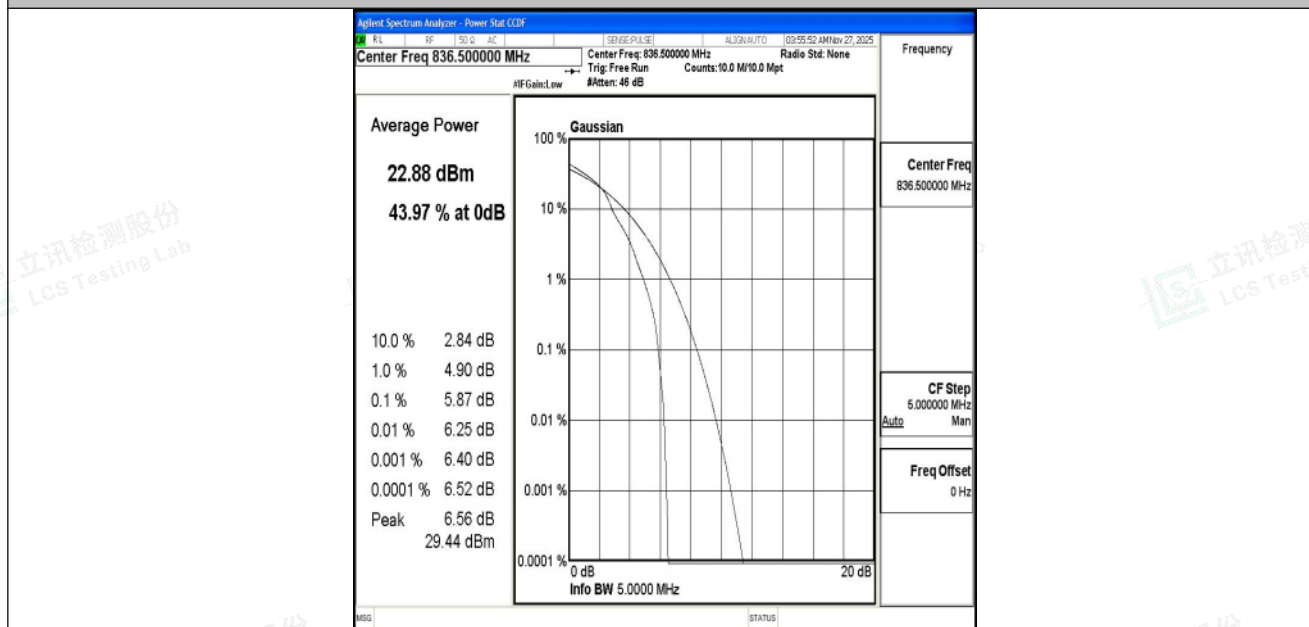
Band5-5MHz-16QAM-20525-1RB#0-PASS
