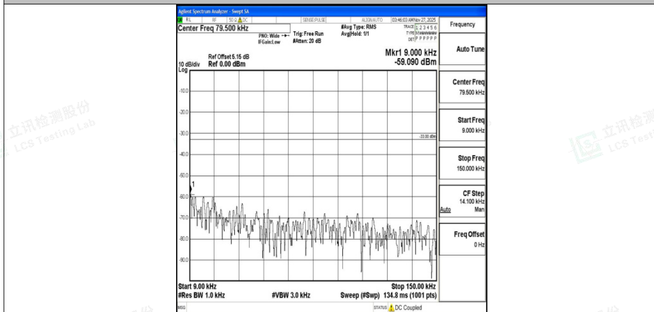
Band5_5MHz_16QAM_20425_1RB#0_0.009~0.15_0.009~0.15
