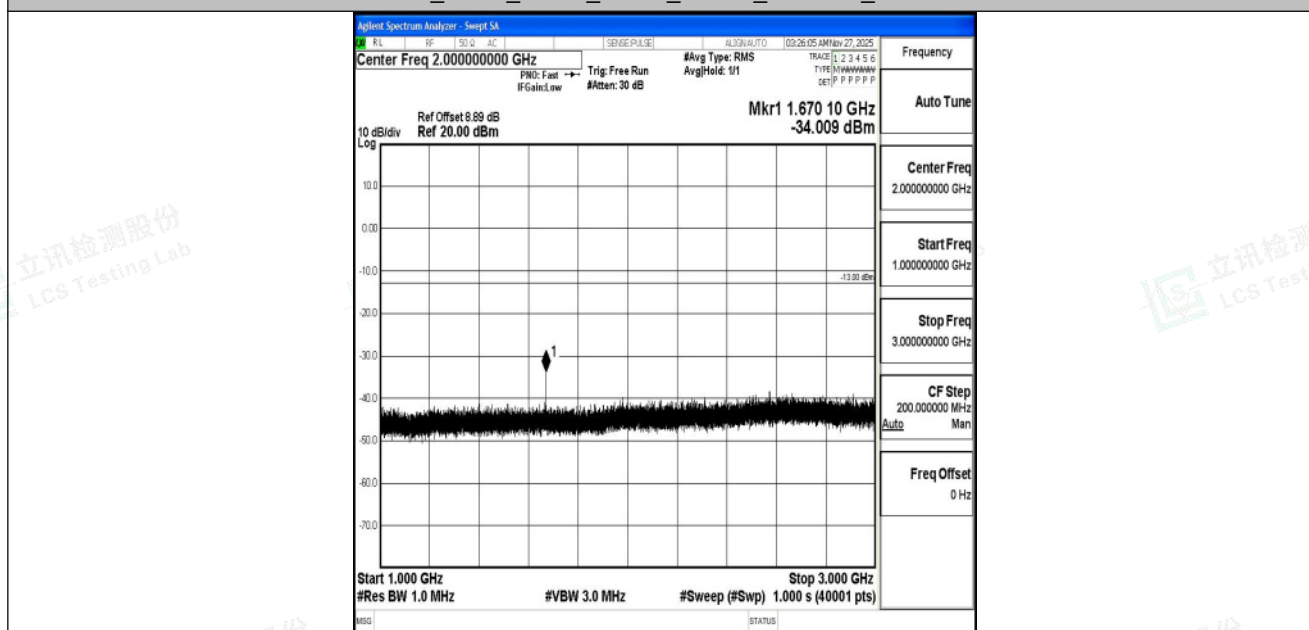
Band5_3MHz_QPSK_20525_1RB#0_1000~3000_1000~3000
