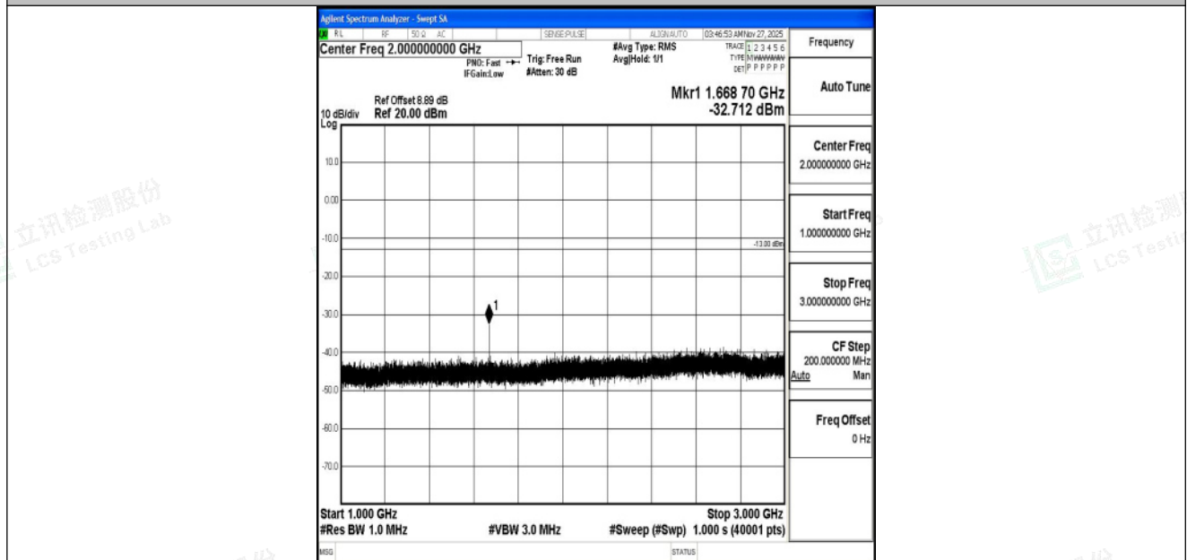
Band5_5MHz_QPSK_20525_1RB#0_1000~3000_1000~3000
