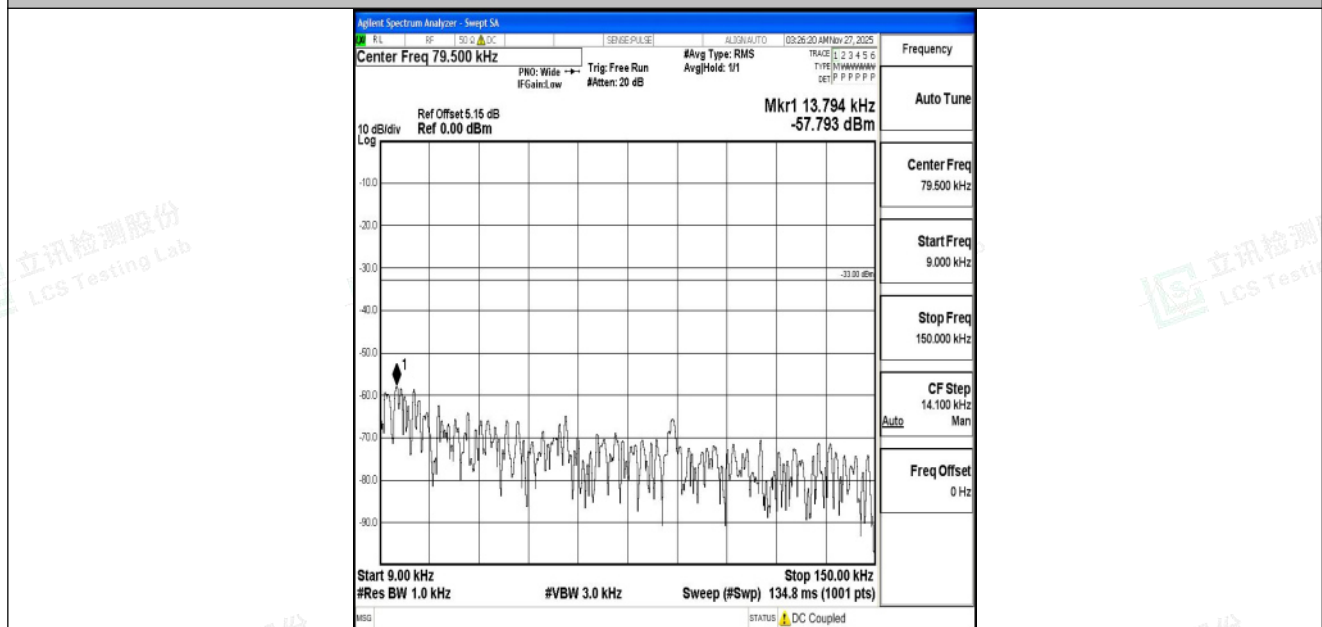
Band5_3MHz_16QAM_20525_1RB#0_0.009~0.15_0.009~0.15
