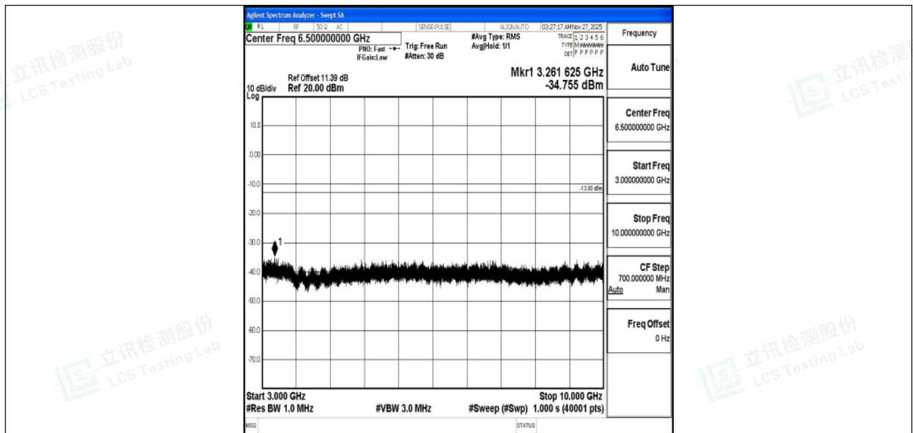
Band5_3MHz_QPSK_20635_1RB#0_3000~10000_3000~10000
