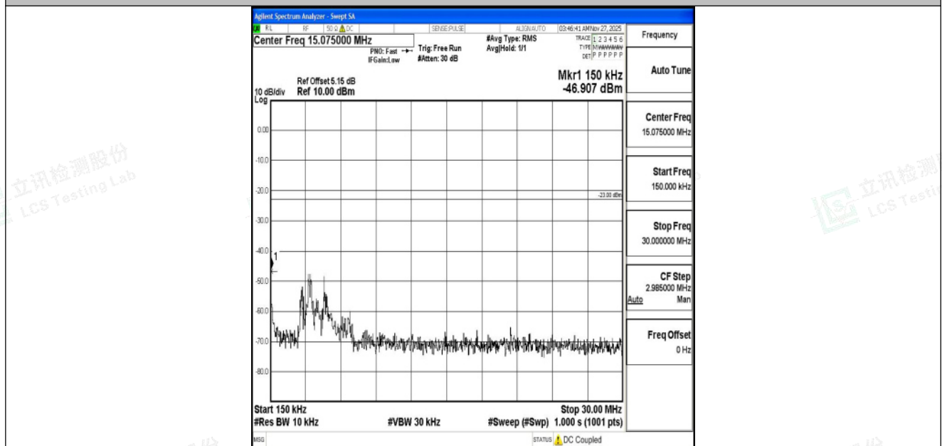
Band5_5MHz_QPSK_20525_1RB#0_0.15~30_0.15~30
