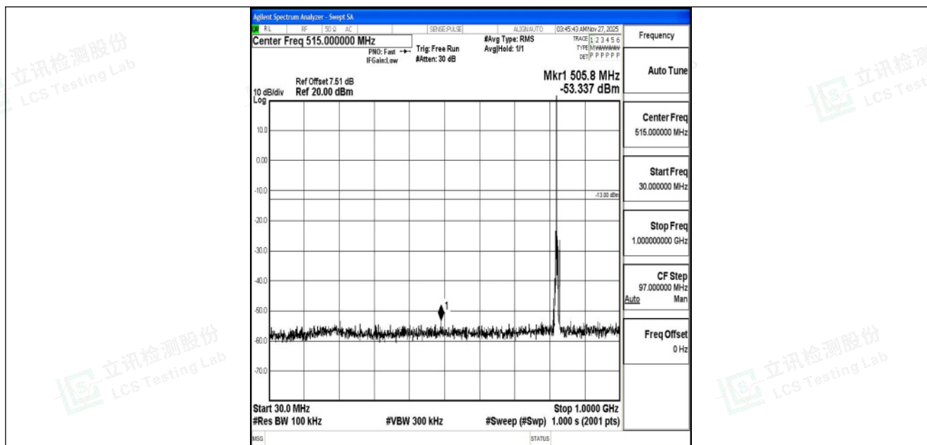
Band5_5MHz_QPSK_20425_1RB#0_30~1000_30~1000
