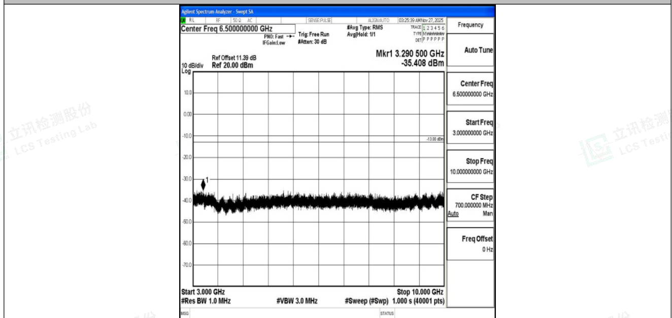
Band5_3MHz_16QAM_20415_1RB#0_3000~10000_3000~10000
