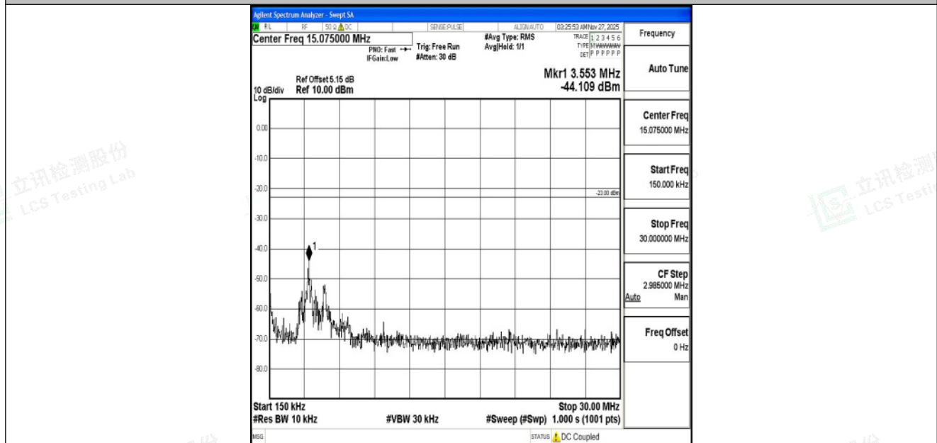
Band5_3MHz_QPSK_20525_1RB#0_0.15~30_0.15~30
