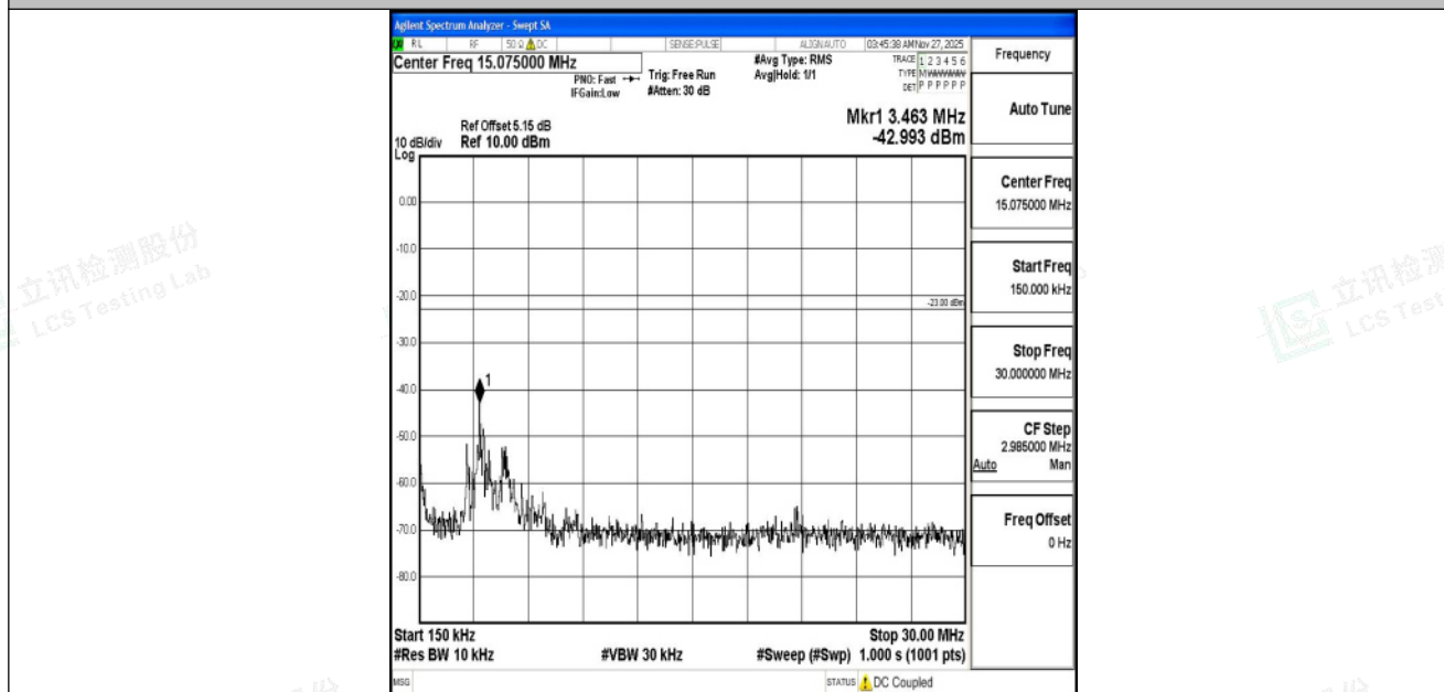
Band5_5MHz_QPSK_20425_1RB#0_0.15~30_0.15~30
