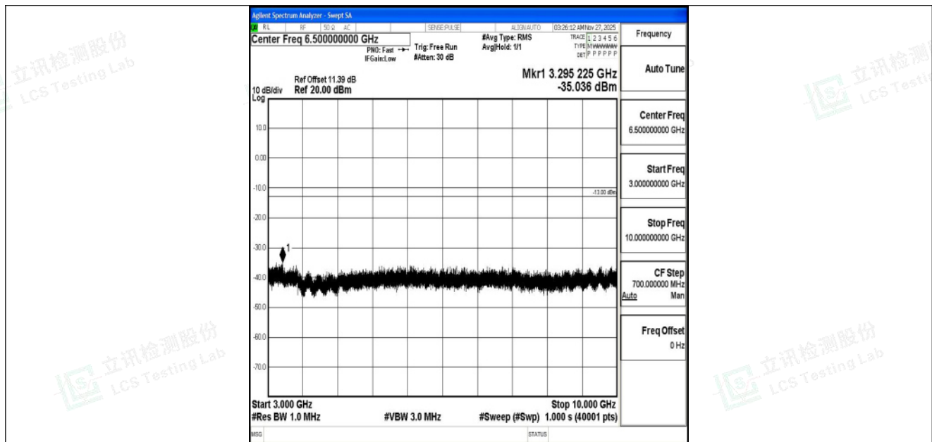
Band5_3MHz_QPSK_20525_1RB#0_3000~10000_3000~10000
