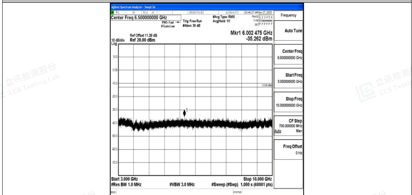
Band5_5MHz_16QAM_20425_1RB#0_3000~10000_3000~10000
