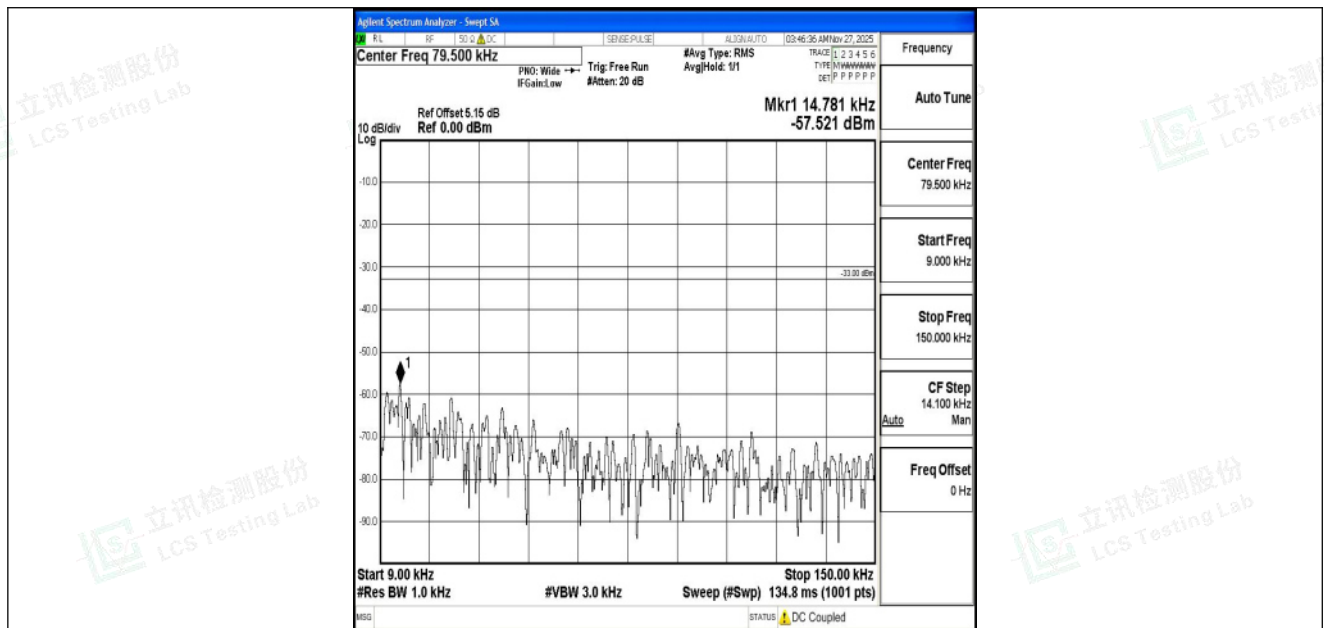
Band5_5MHz_QPSK_20525_1RB#0_0.009~0.15_0.009~0.15
