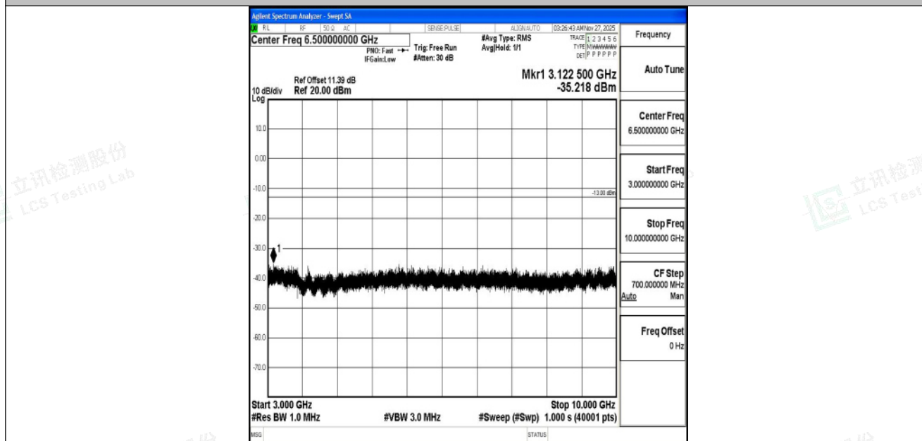
Band5_3MHz_16QAM_20525_1RB#0_3000~10000_3000~10000
