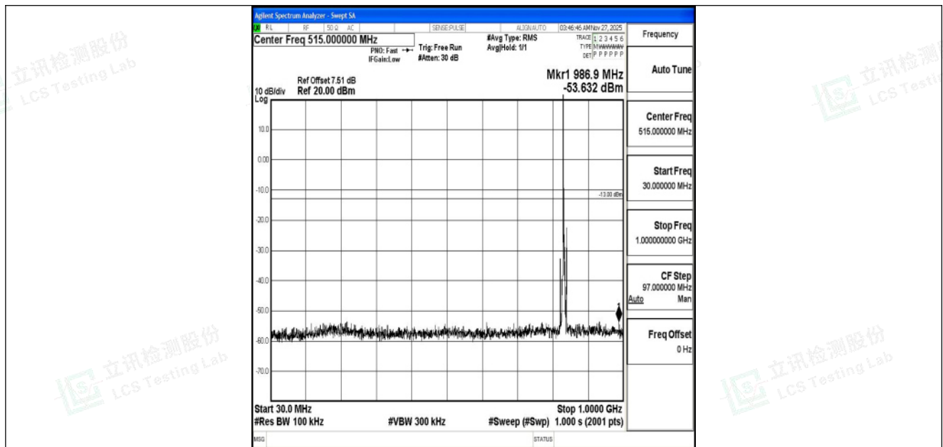
Band5_5MHz_QPSK_20525_1RB#0_30~1000_30~1000
