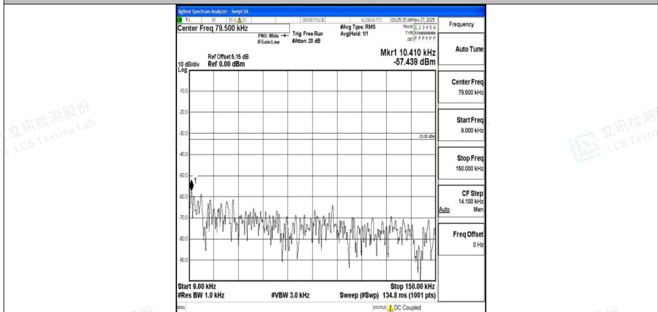
Band5_3MHz_16QAM_20415_1RB#0_0.009~0.15_0.009~0.15
