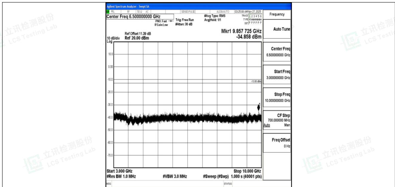
Band5_3MHz_QPSK_20415_1RB#0_3000~10000_3000~10000
