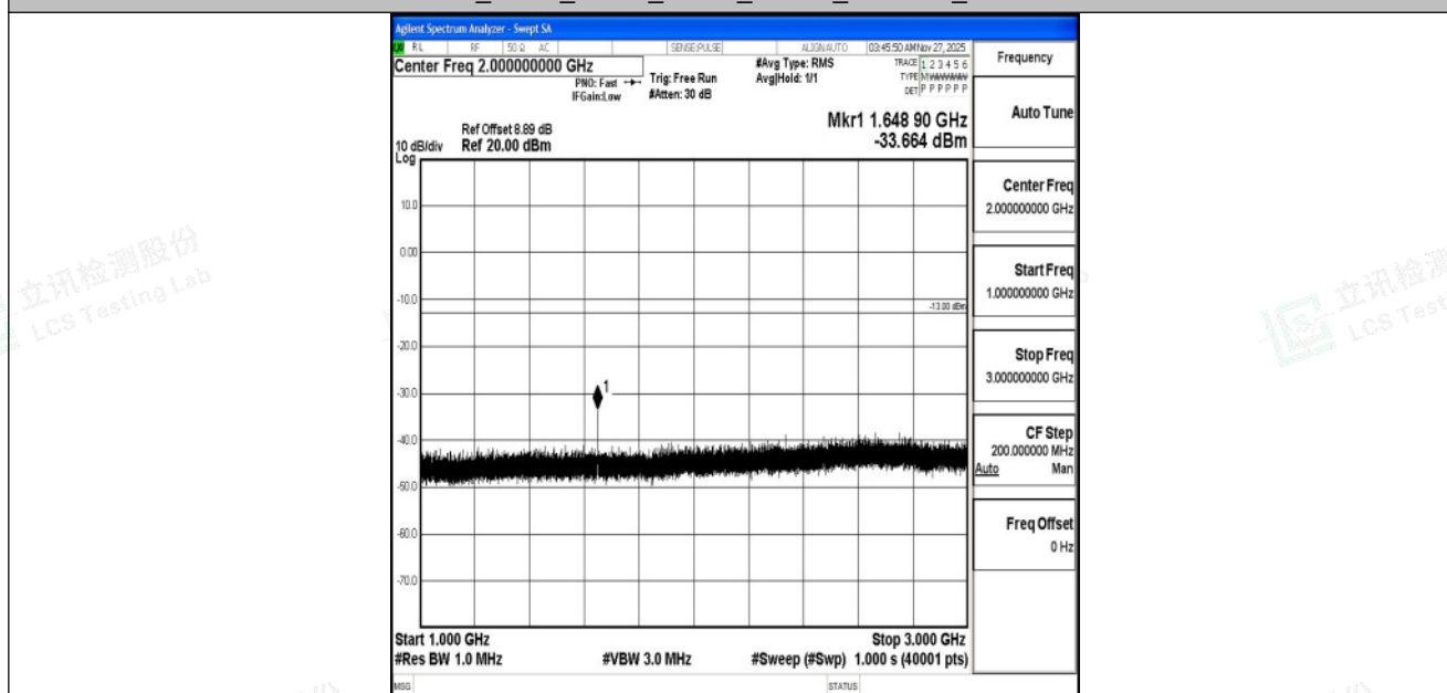
Band5_5MHz_QPSK_20425_1RB#0_1000~3000_1000~3000
