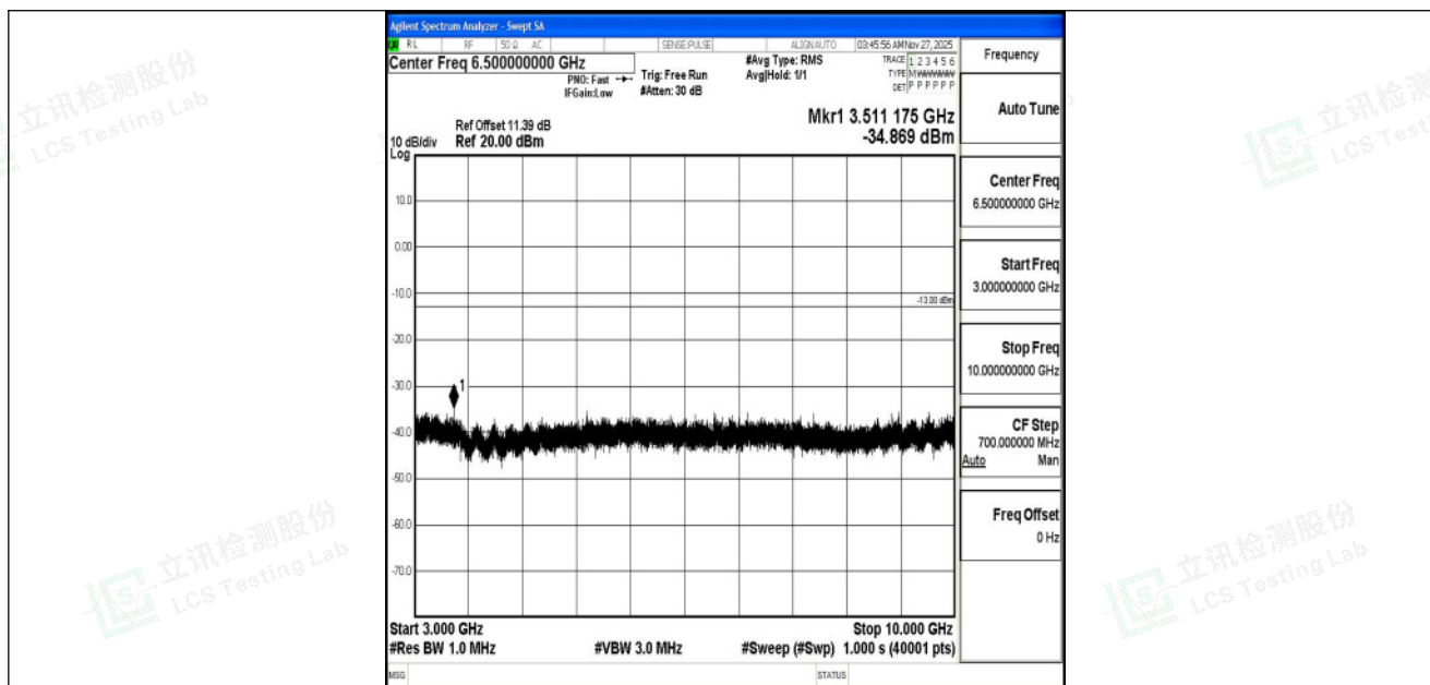
Band5_5MHz_QPSK_20425_1RB#0_3000~10000_3000~10000
