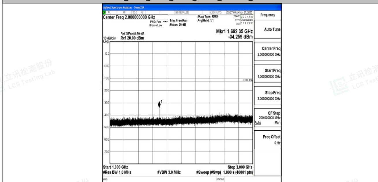
Band5_3MHz_QPSK_20635_1RB#0_1000~3000_1000~3000
