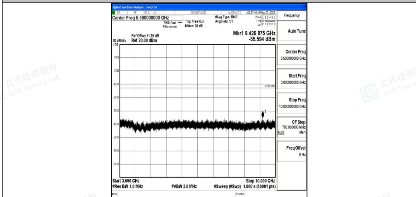
Band5_3MHz_16QAM_20635_1RB#0_3000~10000_3000~10000
