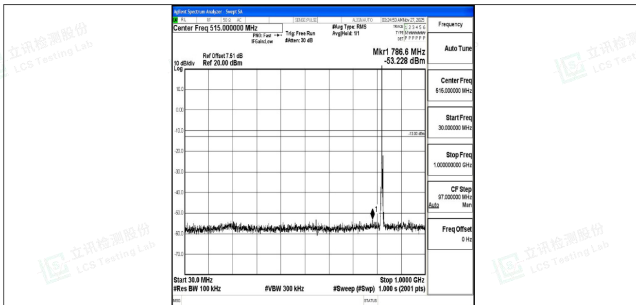
Band5_3MHz_QPSK_20415_1RB#0_30~1000_30~1000
