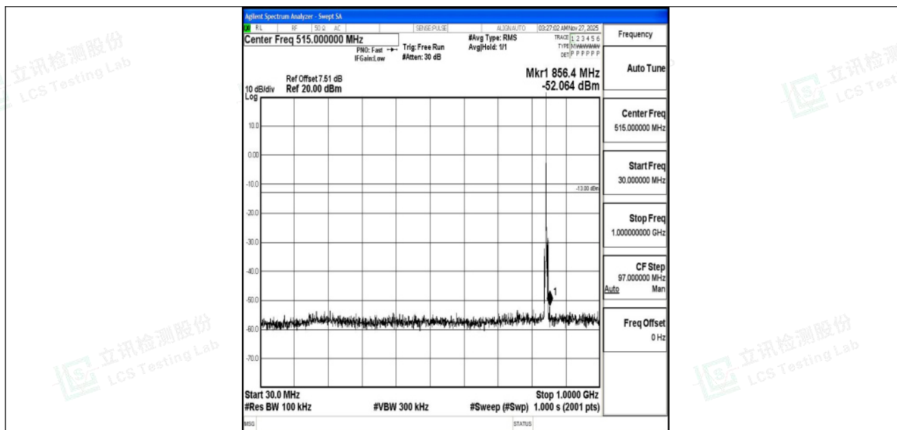
Band5_3MHz_QPSK_20635_1RB#0_30~1000_30~1000
