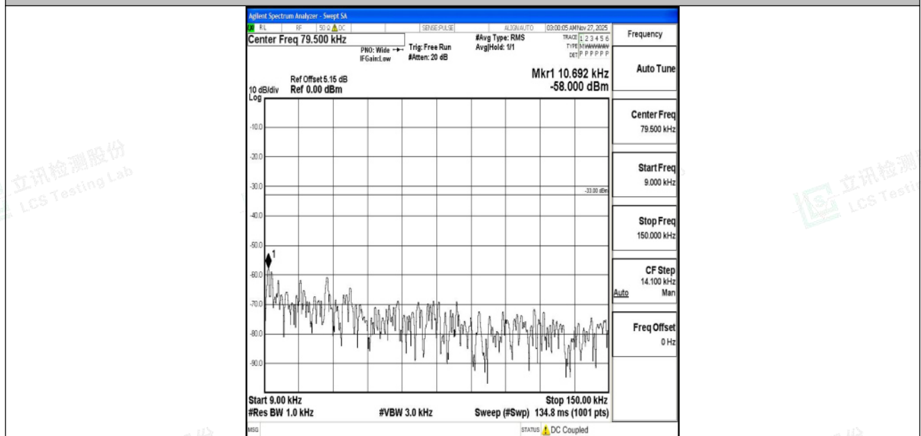
Band5_1.4MHz_16QAM_20643_1RB#0_0.009~0.15_0.009~0.15
