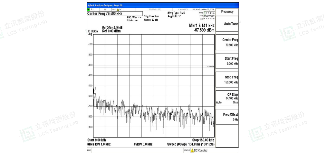
Band5_3MHz_QPSK_20525_1RB#0_0.009~0.15_0.009~0.15
