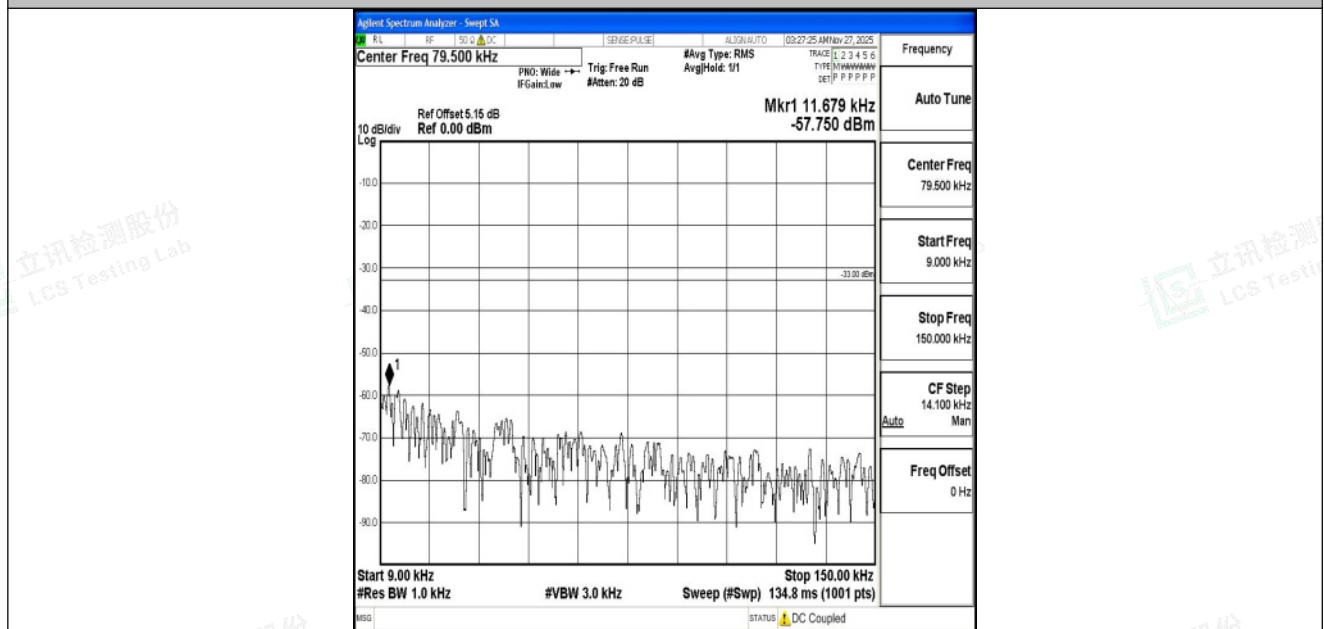
Band5_3MHz_16QAM_20635_1RB#0_0.009~0.15_0.009~0.15
