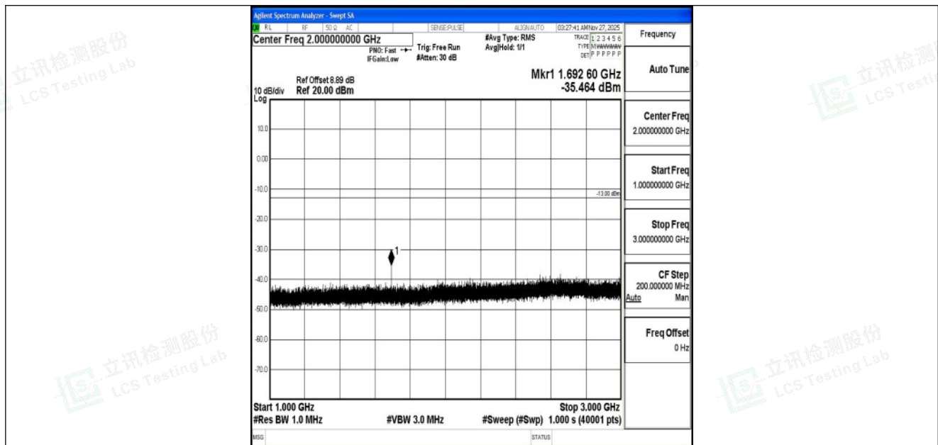
Band5_3MHz_16QAM_20635_1RB#0_1000~3000_1000~3000
