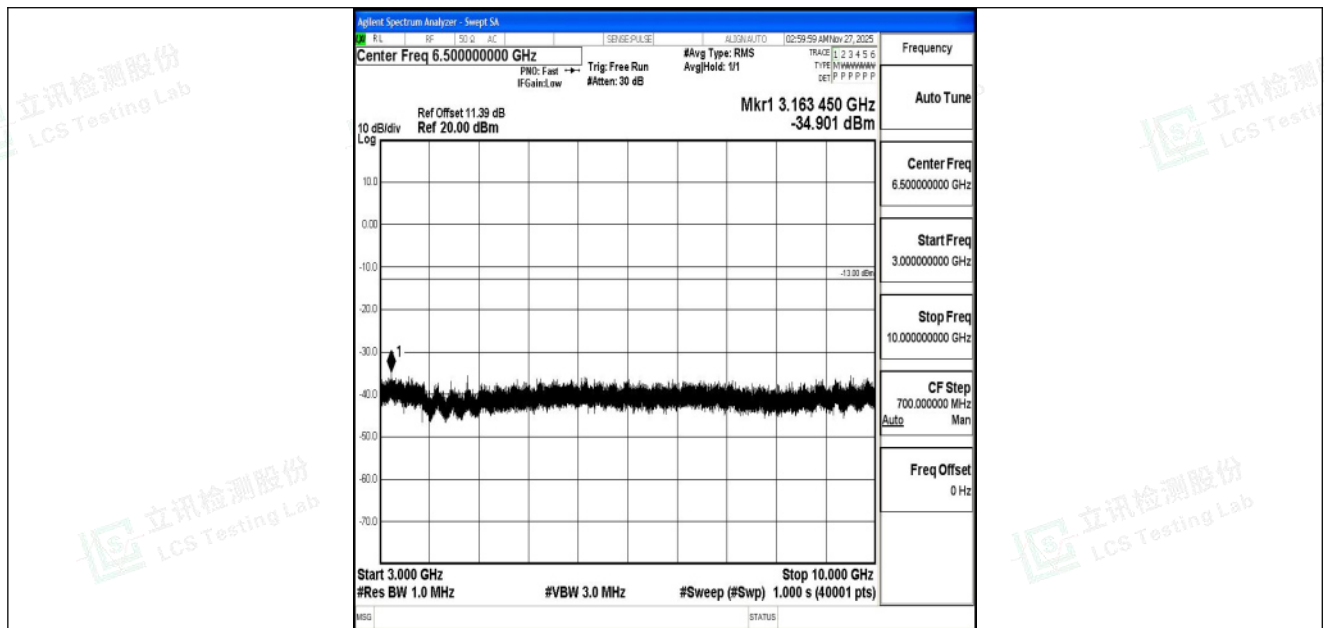
Band5_1.4MHz_QPSK_20643_1RB#0_3000~10000_3000~10000
