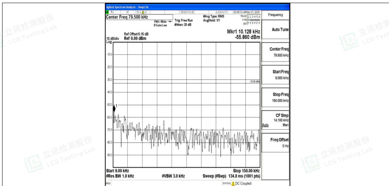
Band5_5MHz_QPSK_20425_1RB#0_0.009~0.15_0.009~0.15
