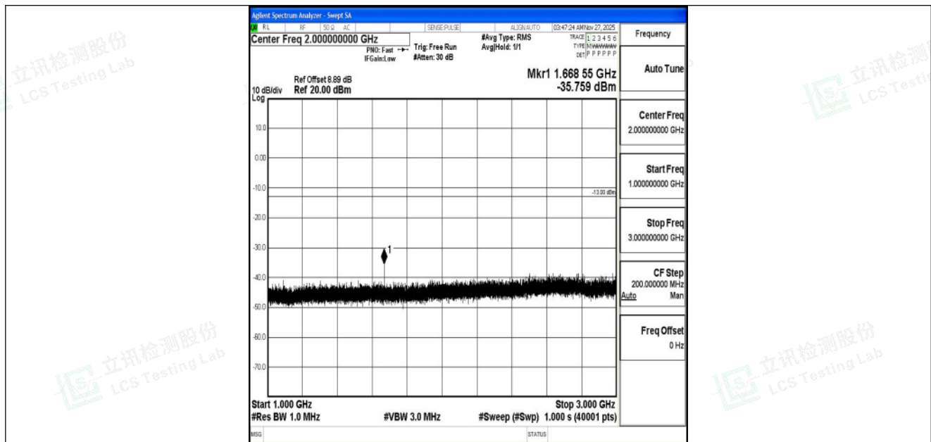
Band5_5MHz_16QAM_20525_1RB#0_1000~3000_1000~3000
