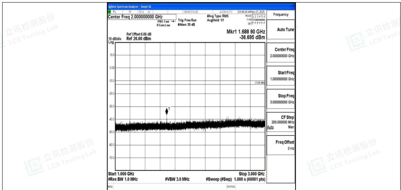
Band5_5MHz_16QAM_20625_1RB#0_1000~3000_1000~3000
