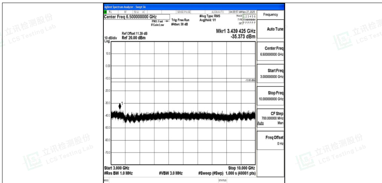
Band5_10MHz_QPSK_20450_1RB#0_3000~10000_3000~10000
