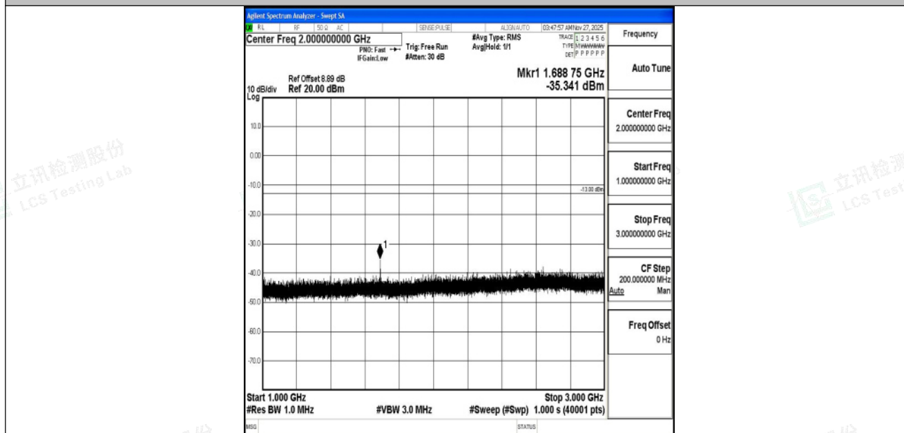
Band5_5MHz_QPSK_20625_1RB#0_1000~3000_1000~3000
