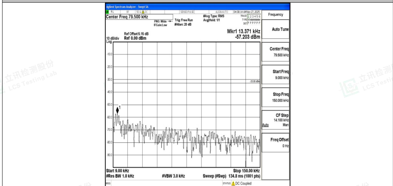
Band5_10MHz_16QAM_20600_1RB#0_0.009~0.15_0.009~0.15
