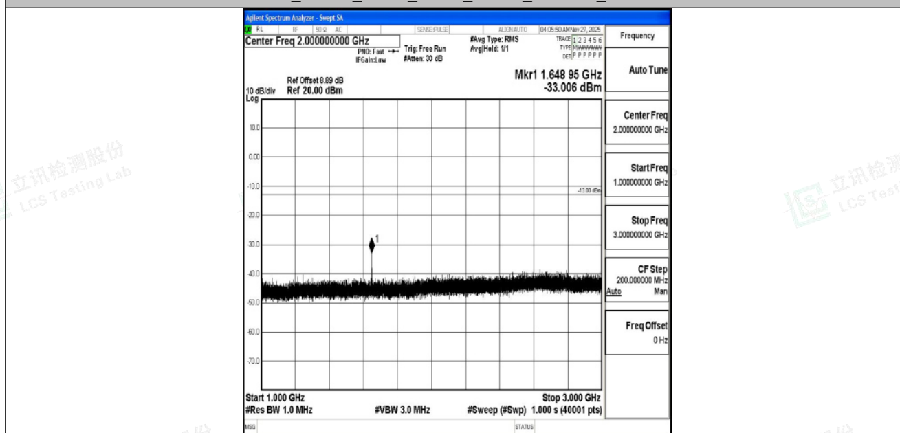
Band5_10MHz_QPSK_20450_1RB#0_1000~3000_1000~3000
