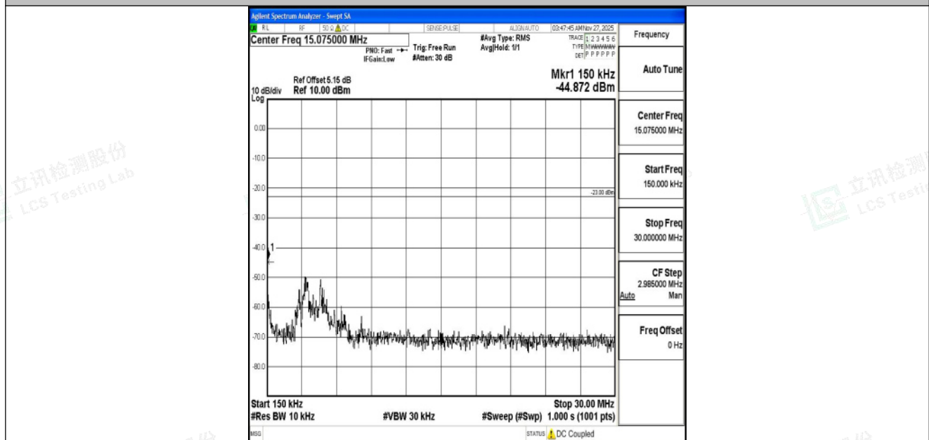
Band5_5MHz_QPSK_20625_1RB#0_0.15~30_0.15~30
