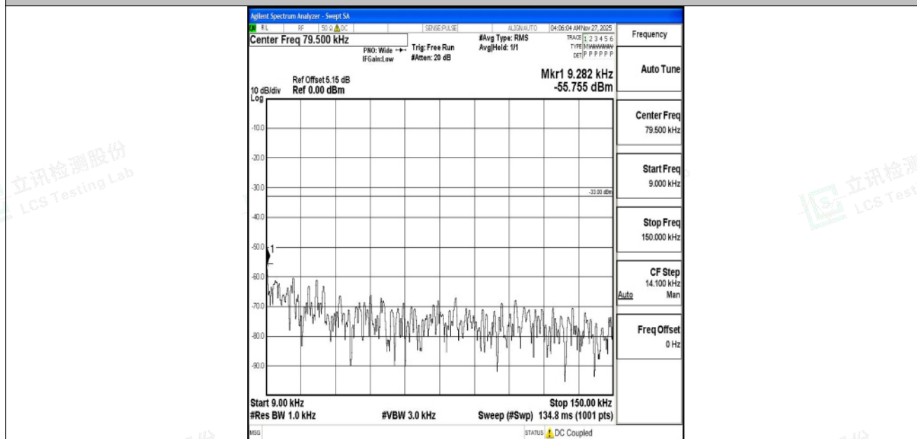
Band5_10MHz_16QAM_20450_1RB#0_0.009~0.15_0.009~0.15
