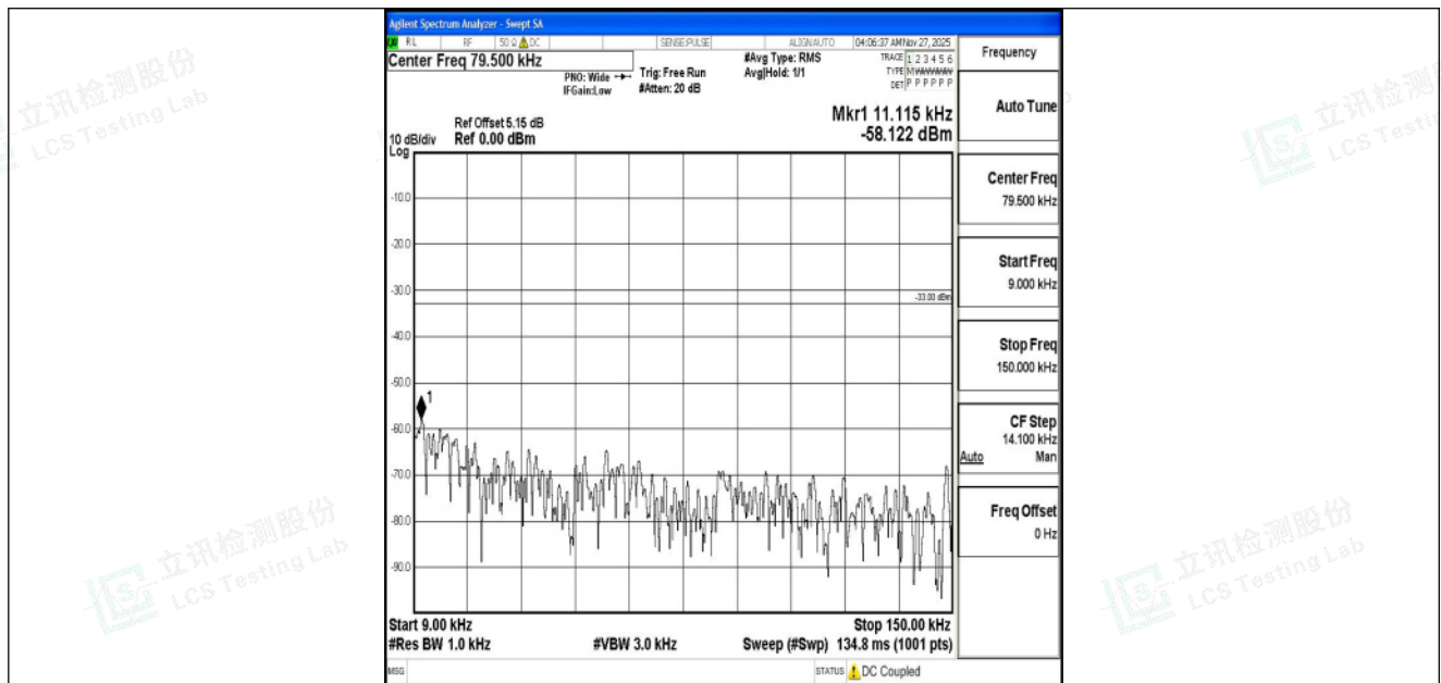
Band5_10MHz_QPSK_20525_1RB#0_0.009~0.15_0.009~0.15
