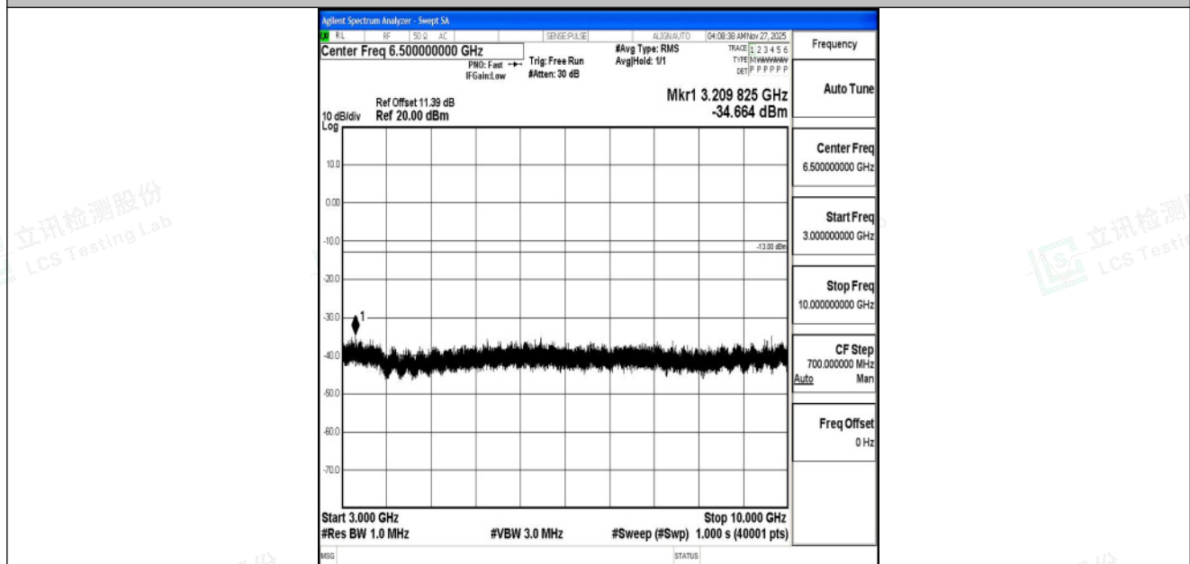
Band5_10MHz_16QAM_20600_1RB#0_3000~10000_3000~10000
