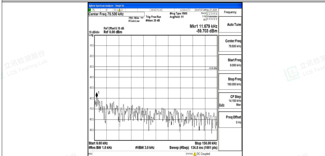
Band5_5MHz_16QAM_20525_1RB#0_0.009~0.15_0.009~0.15
