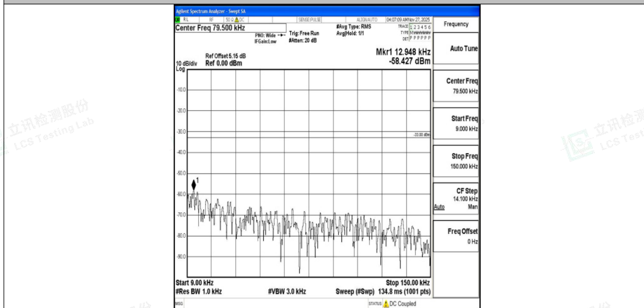
Band5_10MHz_16QAM_20525_1RB#0_0.009~0.15_0.009~0.15
