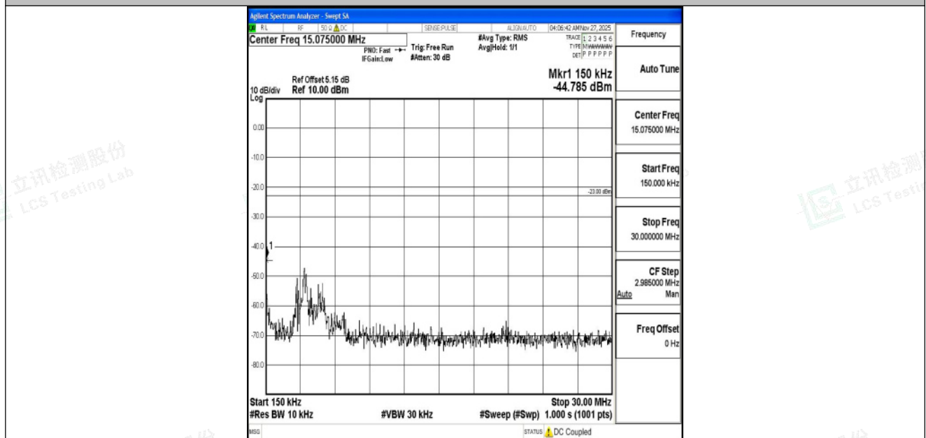
Band5_10MHz_QPSK_20525_1RB#0_0.15~30_0.15~30
