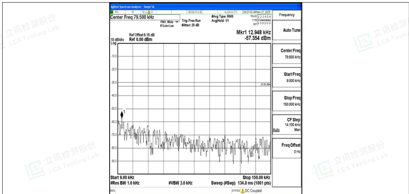
Band5_10MHz_QPSK_20600_1RB#0_0.009~0.15_0.009~0.15
