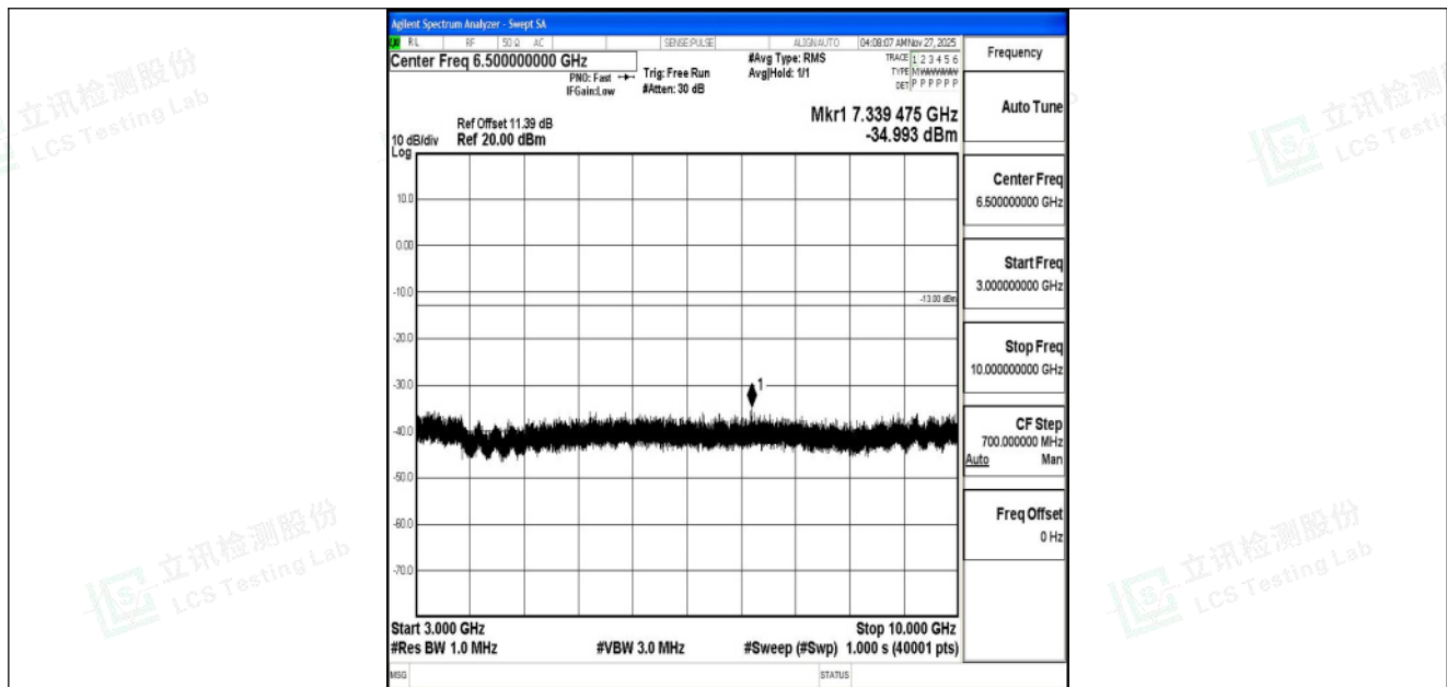
Band5_10MHz_QPSK_20600_1RB#0_3000~10000_3000~10000
