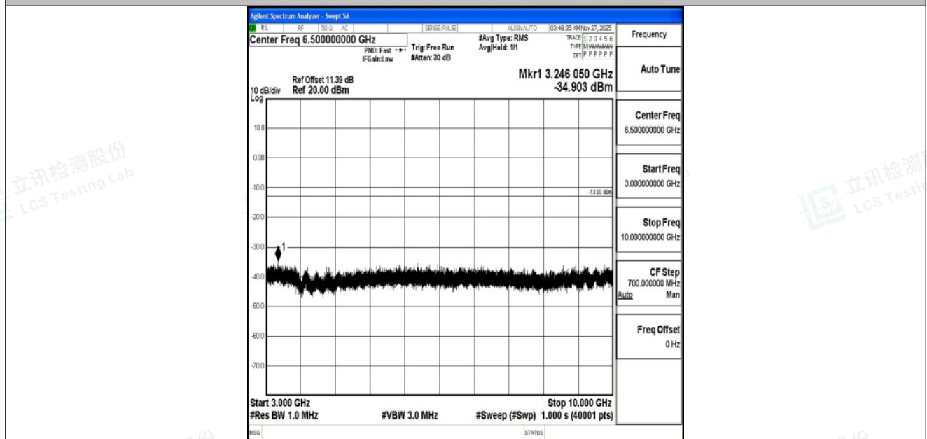
Band5_5MHz_16QAM_20625_1RB#0_3000~10000_3000~10000
