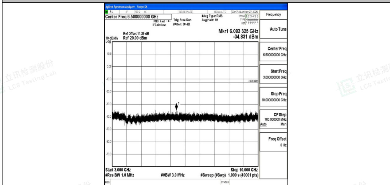
Band5_5MHz_16QAM_20525_1RB#0_3000~10000_3000~10000
