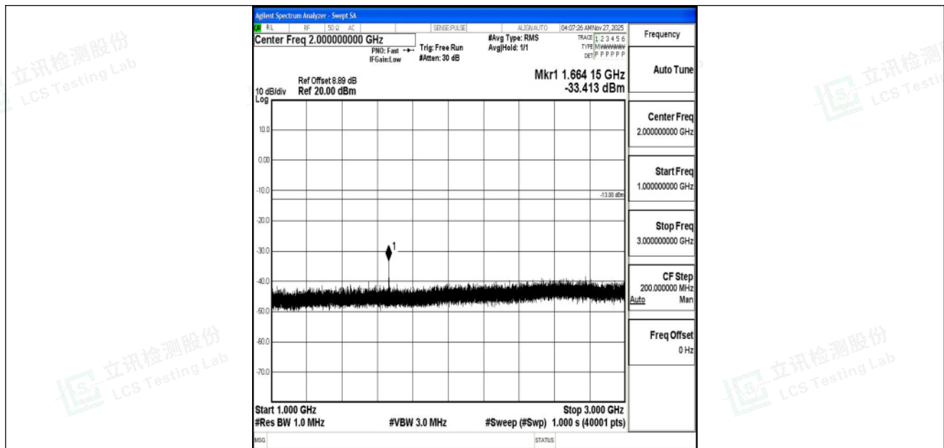
Band5_10MHz_16QAM_20525_1RB#0_1000~3000_1000~3000
