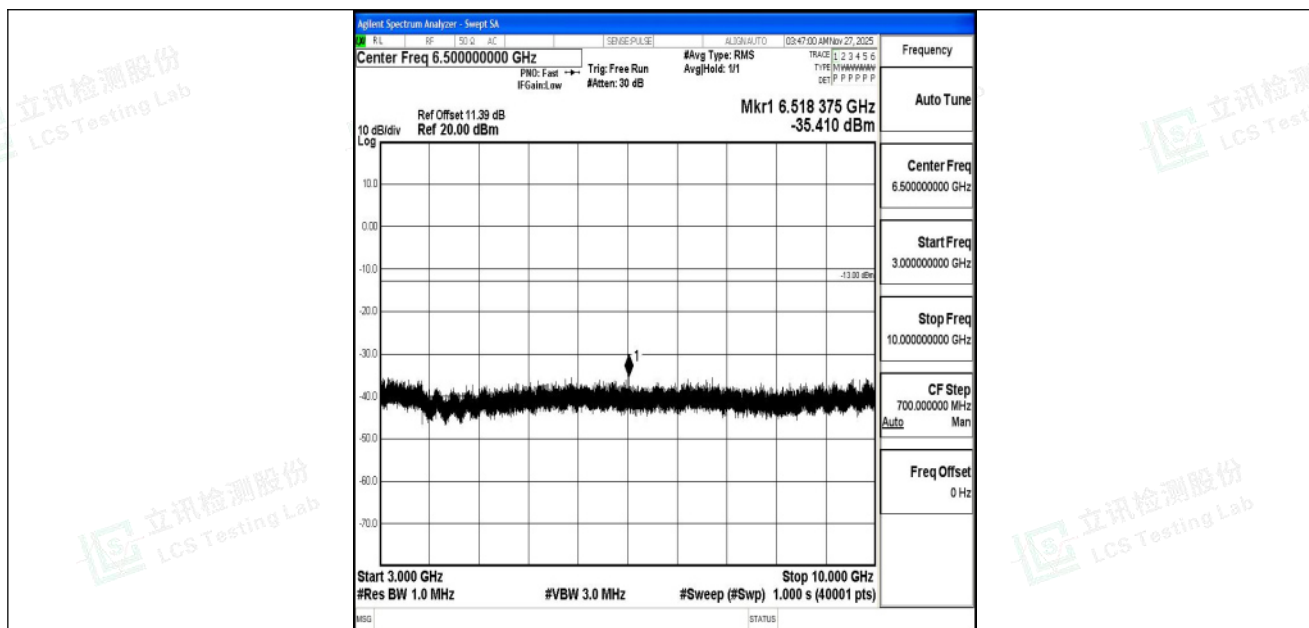
Band5_5MHz_QPSK_20525_1RB#0_3000~10000_3000~10000
