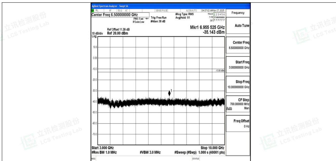
Band5_10MHz_QPSK_20525_1RB#0_3000~10000_3000~10000
