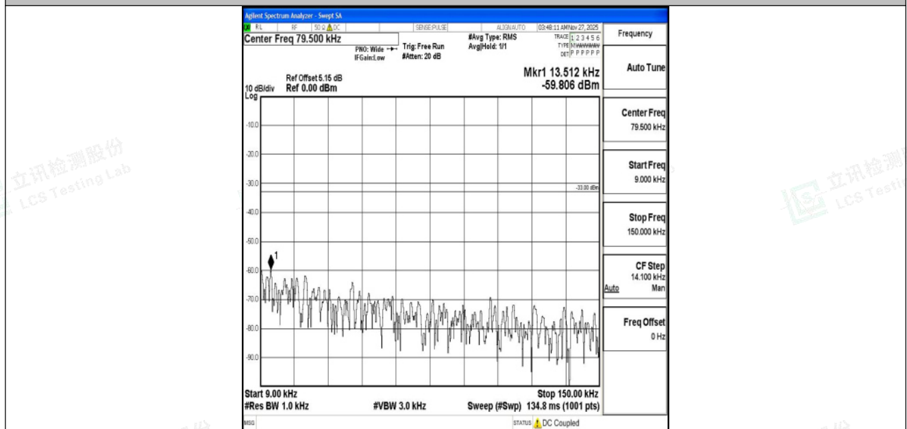
Band5_5MHz_16QAM_20625_1RB#0_0.009~0.15_0.009~0.15
