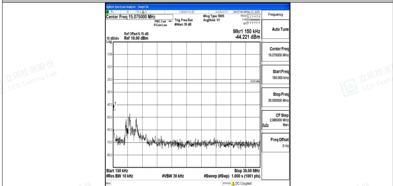
Band5_10MHz_QPSK_20600_1RB#0_0.15~30_0.15~30
