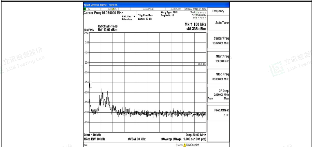
Band5_10MHz_QPSK_20450_1RB#0_0.15~30_0.15~30
