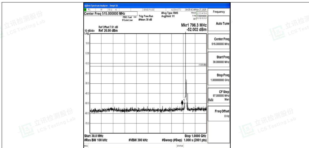
Band5_10MHz_QPSK_20450_1RB#0_30~1000_30~1000
