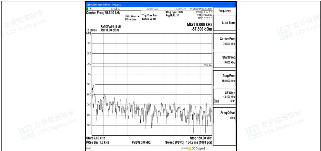
Band5_10MHz_QPSK_20450_1RB#0_0.009~0.15_0.009~0.15
