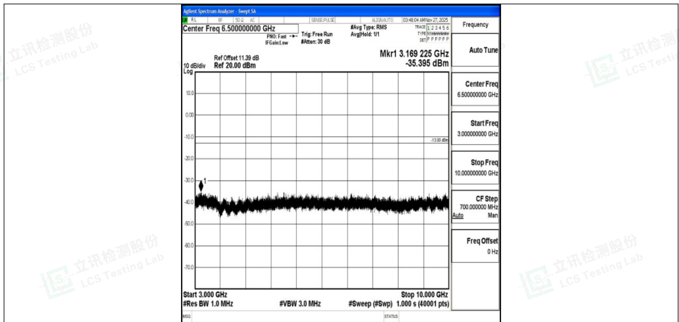
Band5_5MHz_QPSK_20625_1RB#0_3000~10000_3000~10000
