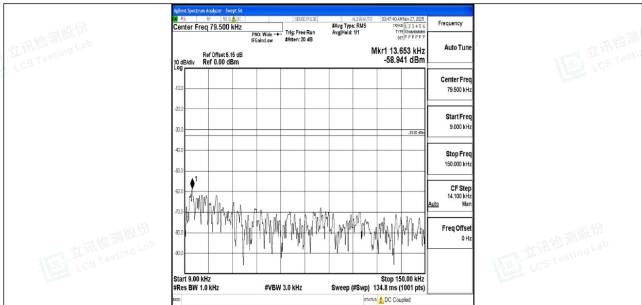
Band5_5MHz_QPSK_20625_1RB#0_0.009~0.15_0.009~0.15
