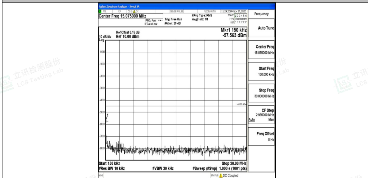
Band7_15MHz_QPSK_21100_1RB#0_0.15~30_0.15~30
