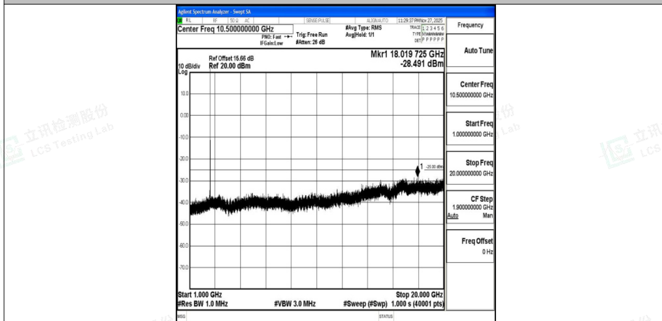
Band7_15MHz_QPSK_21100_1RB#0_1000~20000_1000~20000
