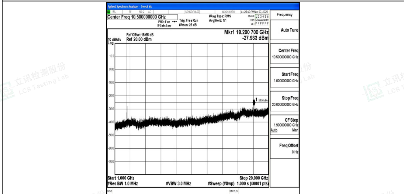
Band7_10MHz_QPSK_20800_1RB#0_1000~20000_1000~20000
