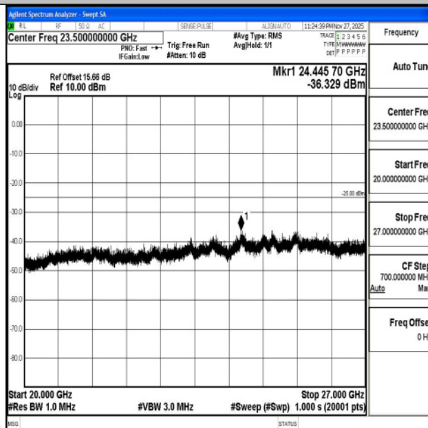
Band7_5MHz_16QAM_21425_1RB#0_20000~27000_20000~27000
