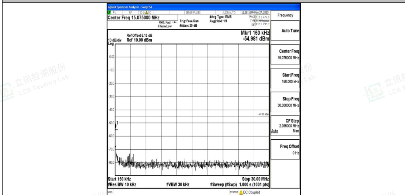
Band7_15MHz_QPSK_20825_1RB#0_0.15~30_0.15~30
