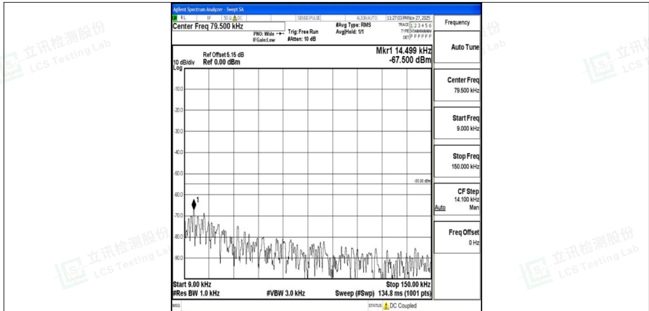
Band7_10MHz_QPSK_21400_1RB#0_0.009~0.15_0.009~0.15
