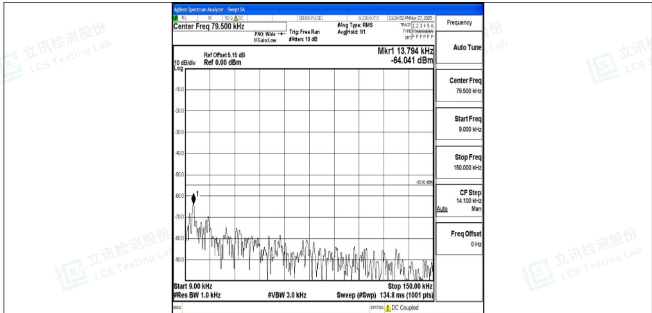
Band7_10MHz_QPSK_20800_1RB#0_0.009~0.15_0.009~0.15
