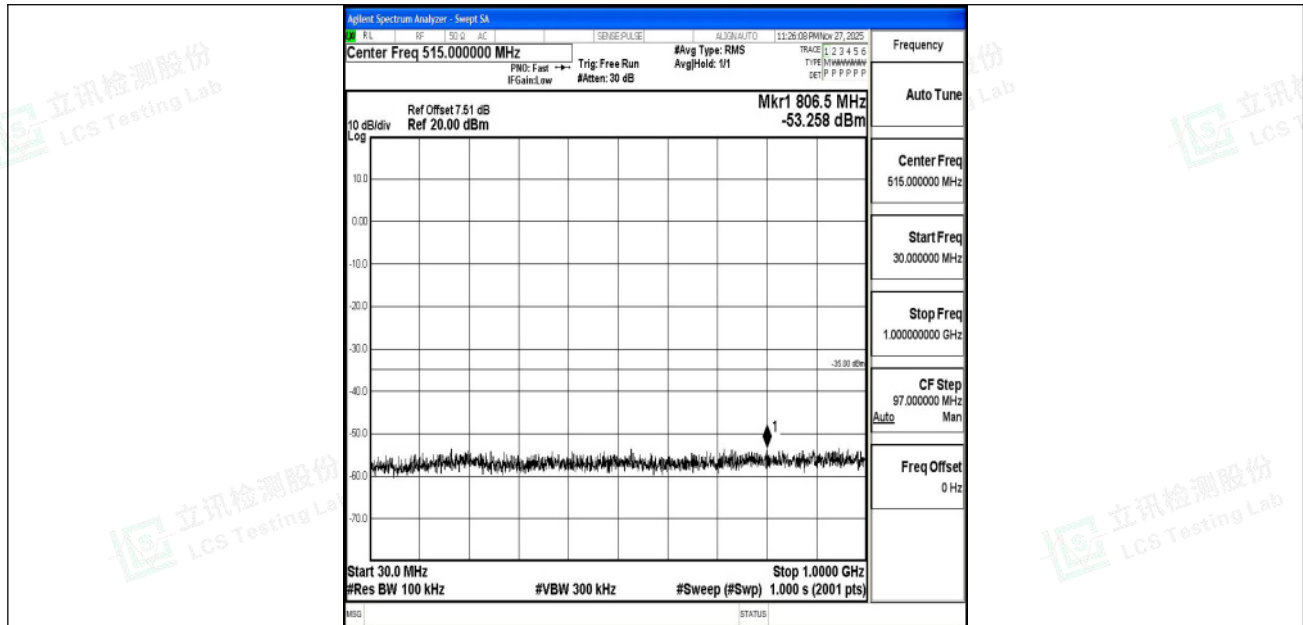
Band7_10MHz_QPSK_21100_1RB#0_30~1000_30~1000
