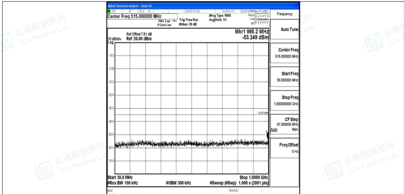
Band7_10MHz_QPSK_21400_1RB#0_30~1000_30~1000
