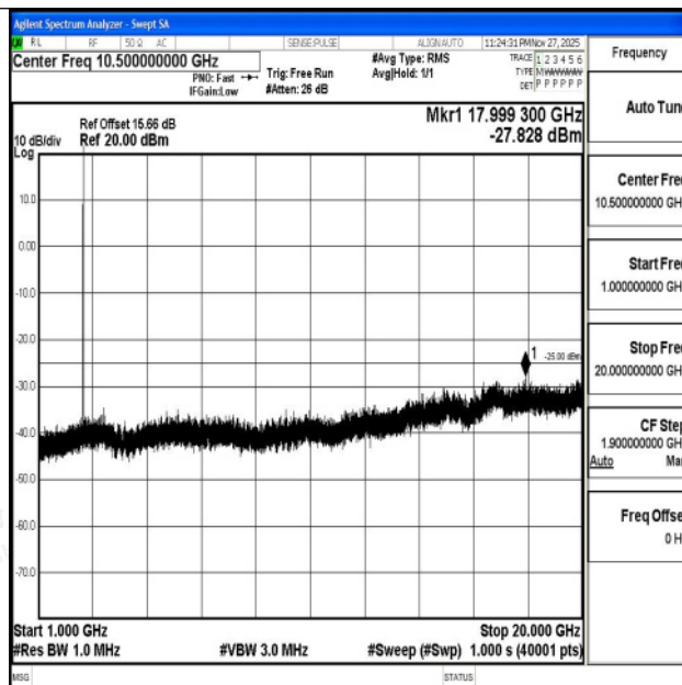
Band7_5MHz_16QAM_21425_1RB#0_1000~20000_1000~20000
