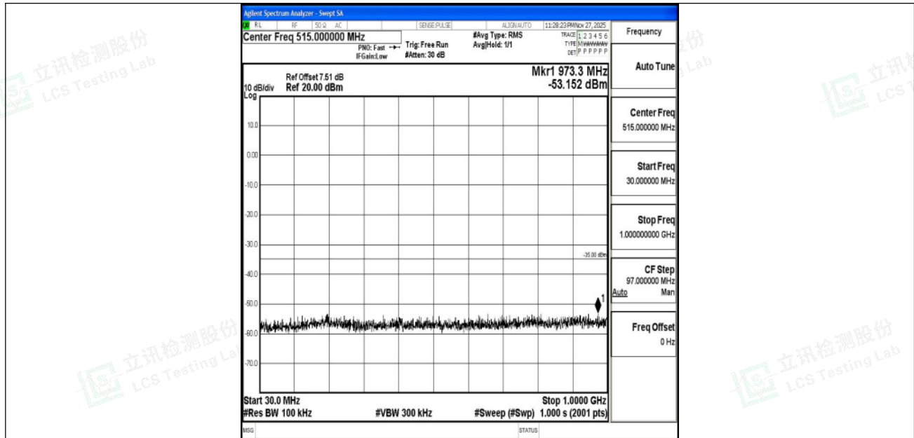
Band7_15MHz_QPSK_20825_1RB#0_30~1000_30~1000
