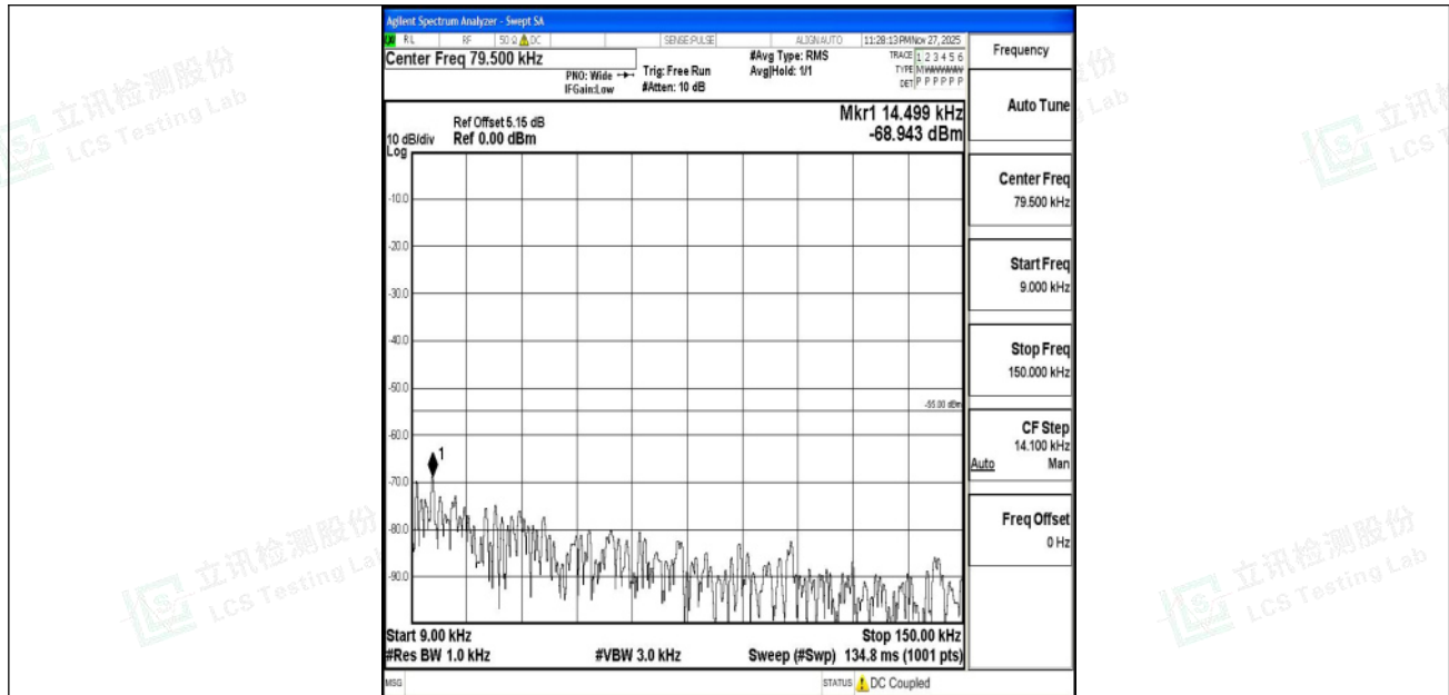
Band7_15MHz_QPSK_20825_1RB#0_0.009~0.15_0.009~0.15
