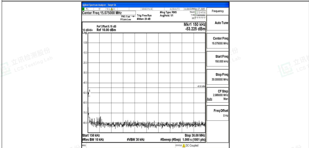
Band7_10MHz_QPSK_21100_1RB#0_0.15~30_0.15~30
