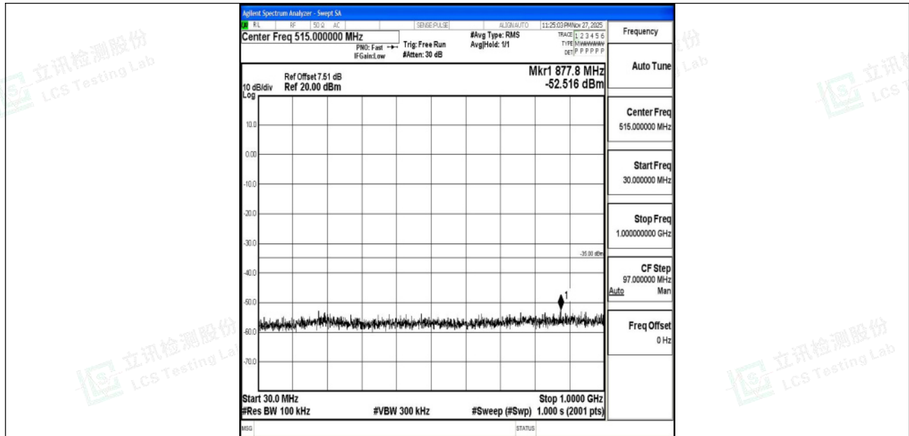
Band7_10MHz_QPSK_20800_1RB#0_30~1000_30~1000
