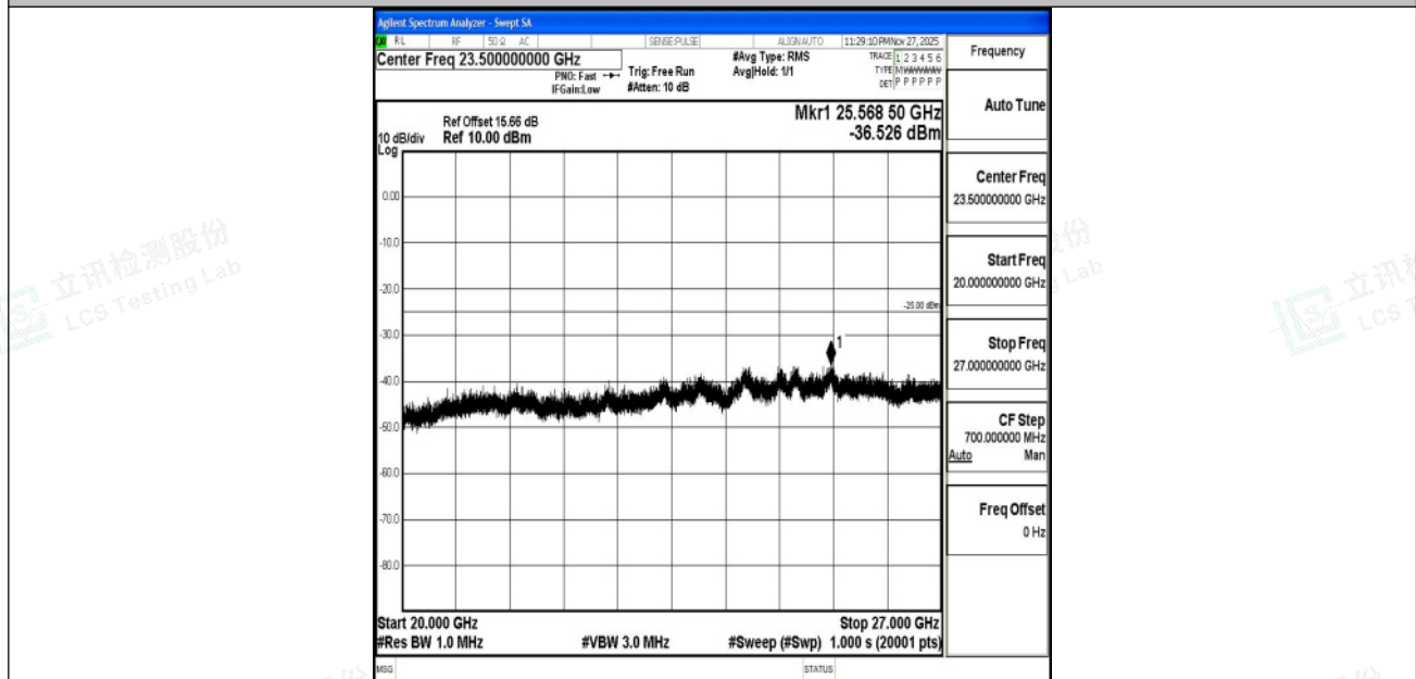
Band7_15MHz_16QAM_20825_1RB#0_20000~27000_20000~27000
