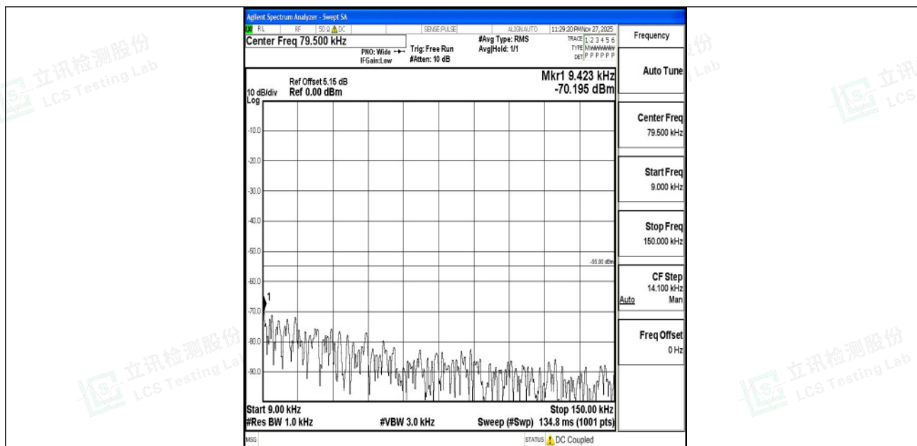
Band7_15MHz_QPSK_21100_1RB#0_0.009~0.15_0.009~0.15
