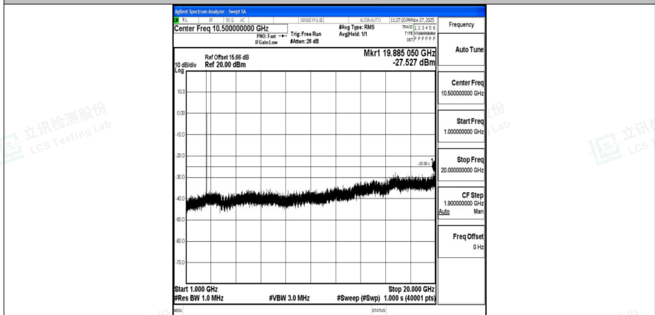
Band7_10MHz_QPSK_21400_1RB#0_1000~20000_1000~20000
