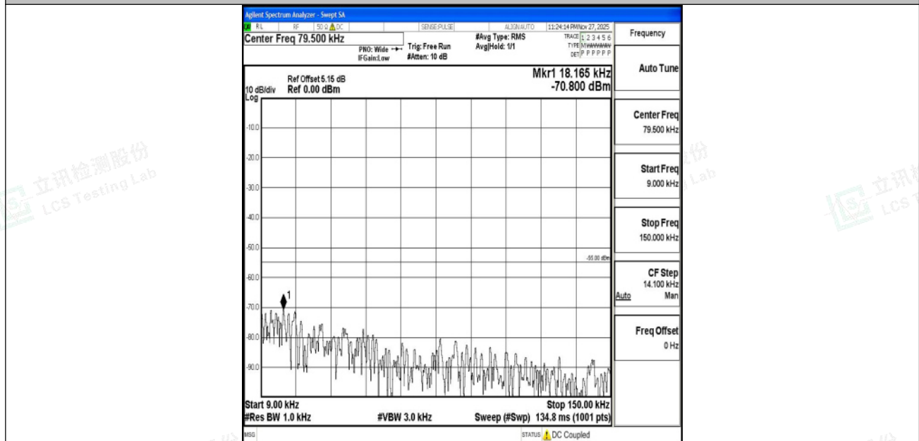
Band7_5MHz_16QAM_21425_1RB#0_0.009~0.15_0.009~0.15
