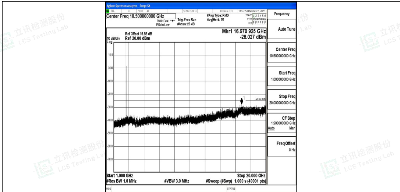
Band7_10MHz_16QAM_21400_1RB#0_1000~20000_1000~20000
