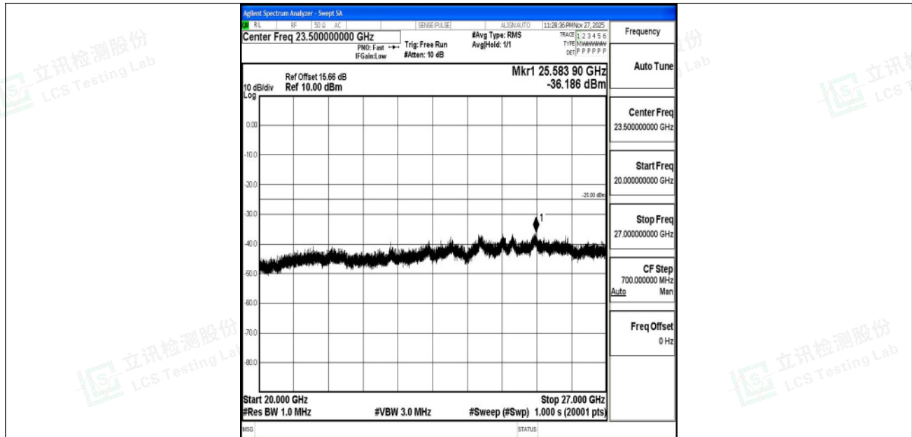
Band7_15MHz_QPSK_20825_1RB#0_20000~27000_20000~27000
