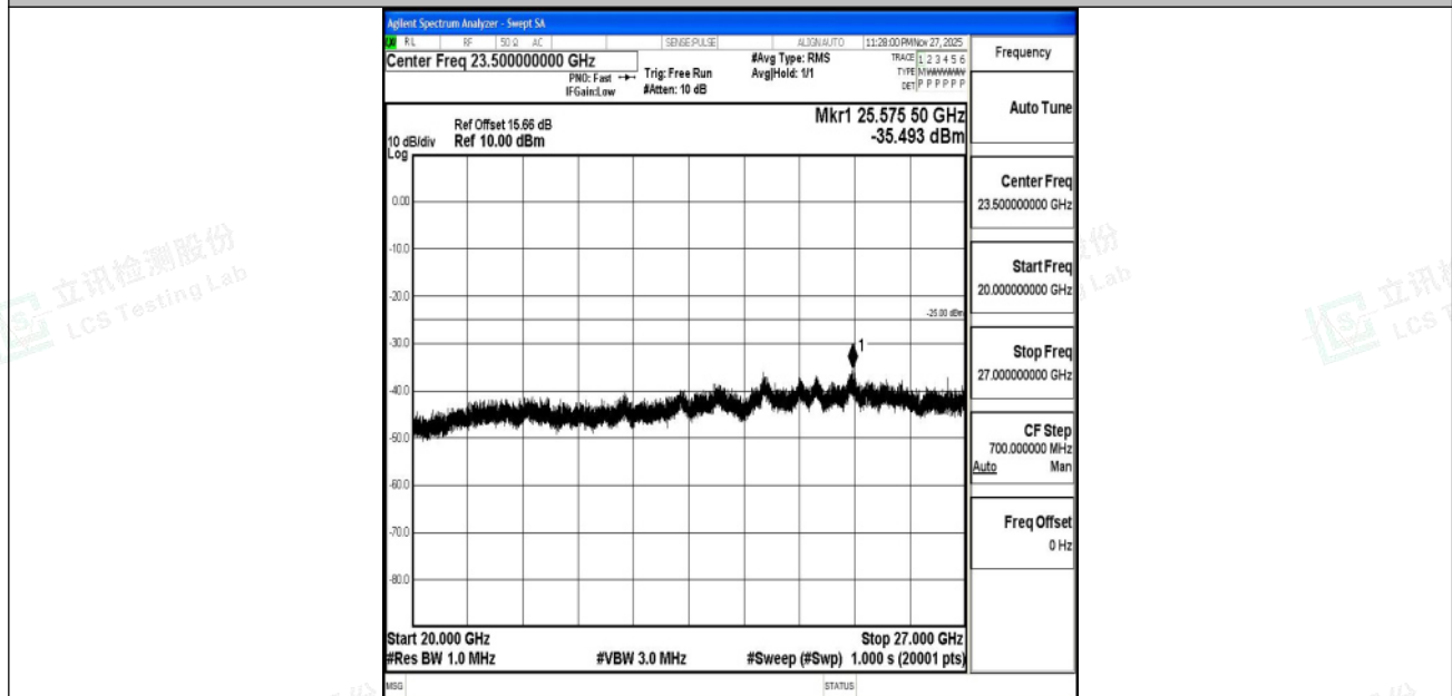
Band7_10MHz_16QAM_21400_1RB#0_20000~27000_20000~27000
