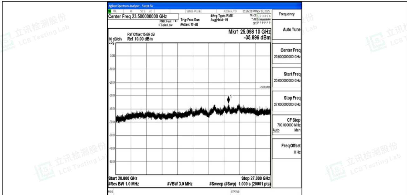
Band7_10MHz_QPSK_21100_1RB#0_20000~27000_20000~27000
