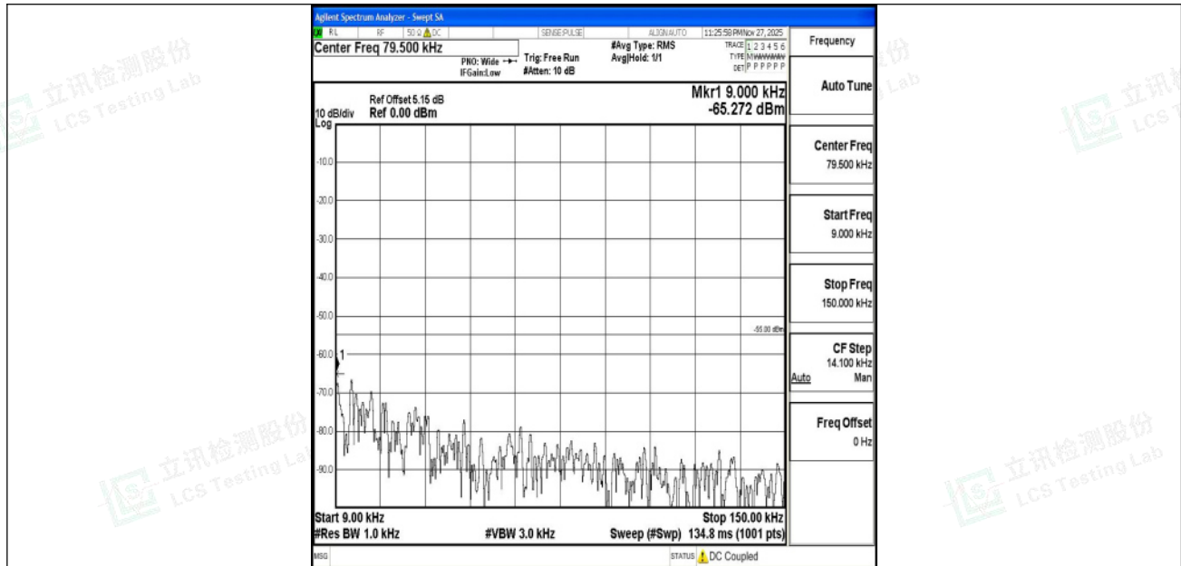
Band7_10MHz_QPSK_21100_1RB#0_0.009~0.15_0.009~0.15
