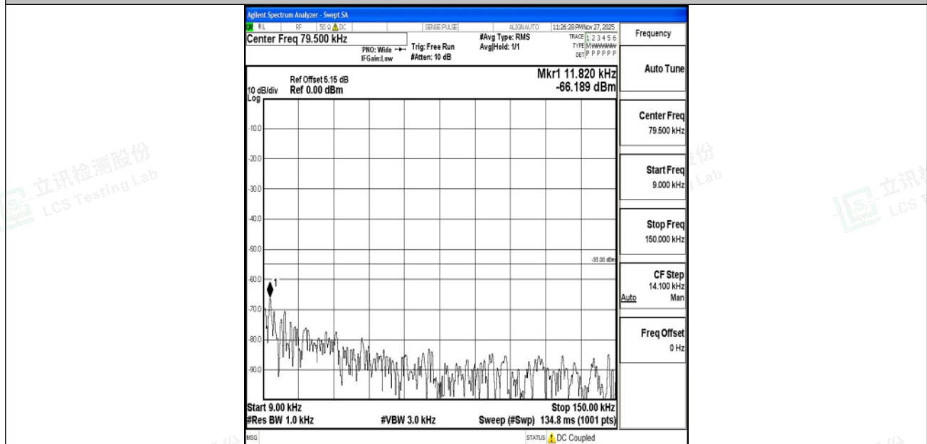
Band7_10MHz_16QAM_21100_1RB#0_0.009~0.15_0.009~0.15
