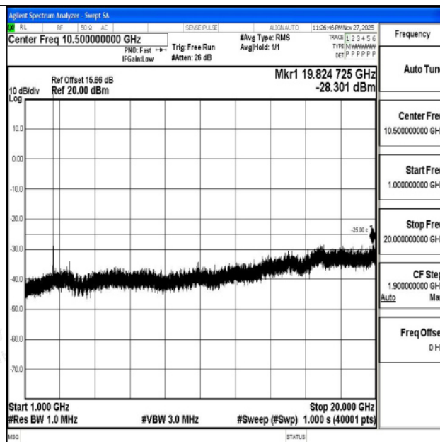
Band7_10MHz_16QAM_21100_1RB#0_1000~20000_1000~20000
