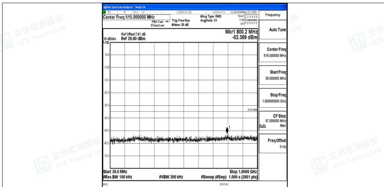
Band7_15MHz_QPSK_21100_1RB#0_30~1000_30~1000
