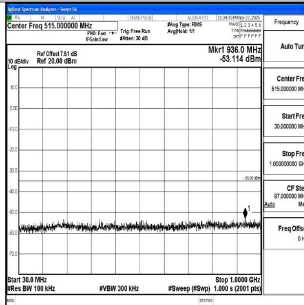
Band7_20MHz_16QAM_21350_1RB#0_30~1000_30~1000
