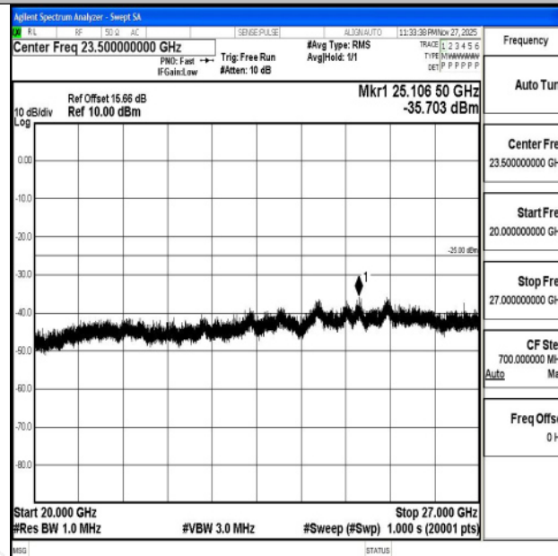
Band7_20MHz_16QAM_21100_1RB#0_20000~27000_20000~27000
