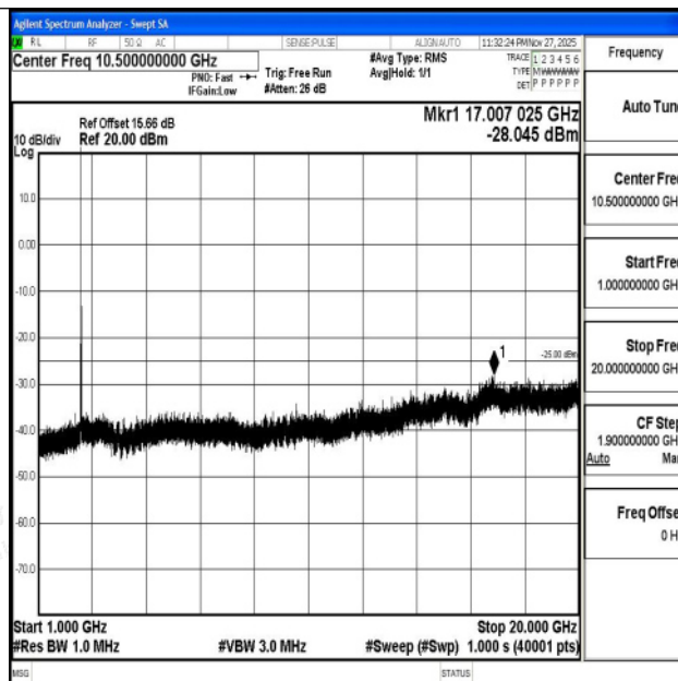
Band7_20MHz_16QAM_20850_1RB#0_1000~20000_1000~20000
