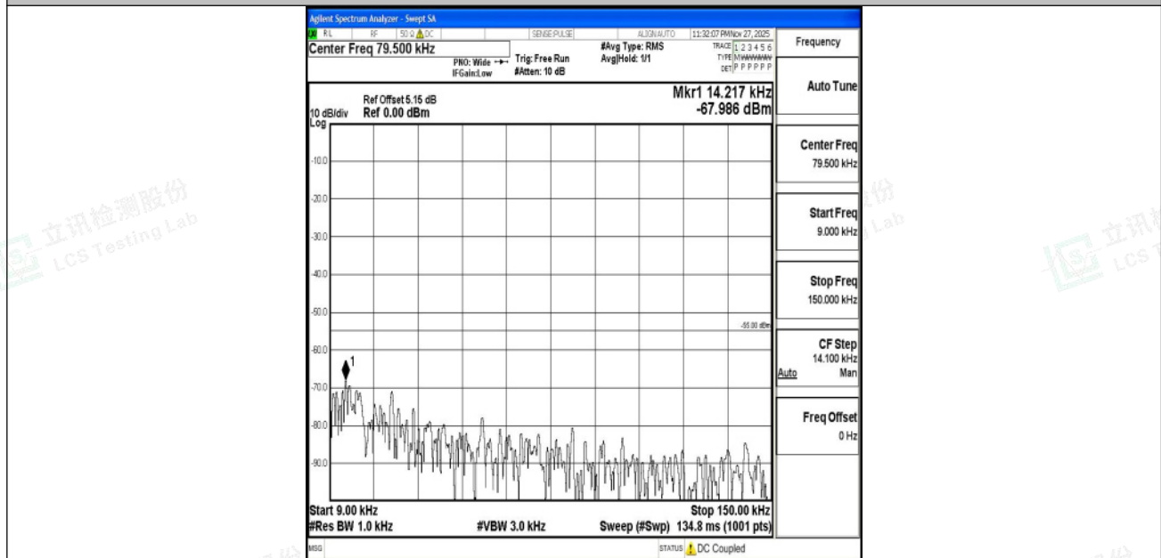
Band7_20MHz_16QAM_20850_1RB#0_0.009~0.15_0.009~0.15
