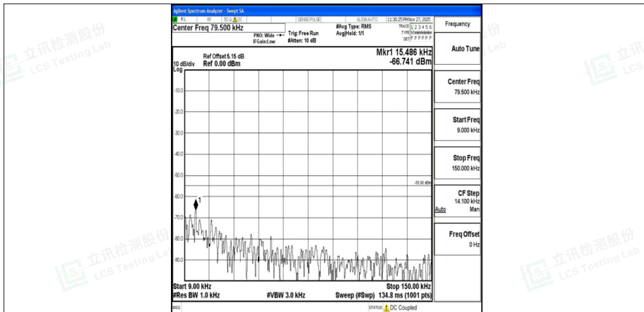
Band7_15MHz_QPSK_21375_1RB#0_0.009~0.15_0.009~0.15
