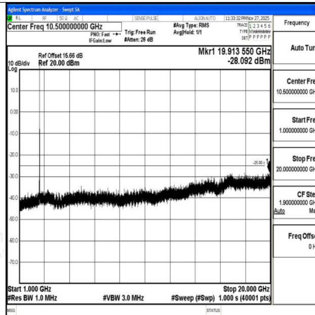
Band7_20MHz_16QAM_21100_1RB#0_1000~20000_1000~20000
