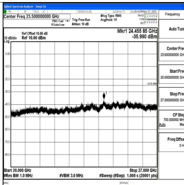
Band7_15MHz_QPSK_21100_1RB#0_20000~27000_20000~27000
