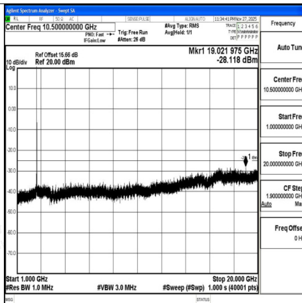
Band7_20MHz_16QAM_21350_1RB#0_1000~20000_1000~20000
