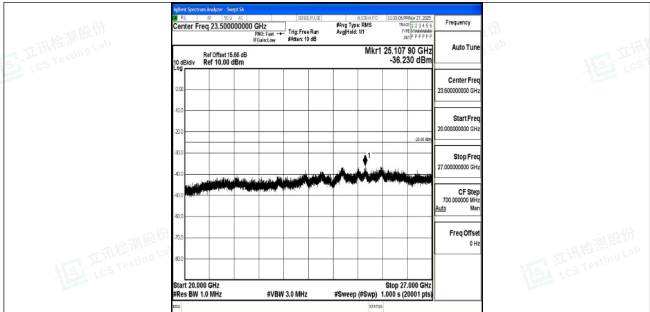
Band7_20MHz_QPSK_21100_1RB#0_20000~27000_20000~27000
