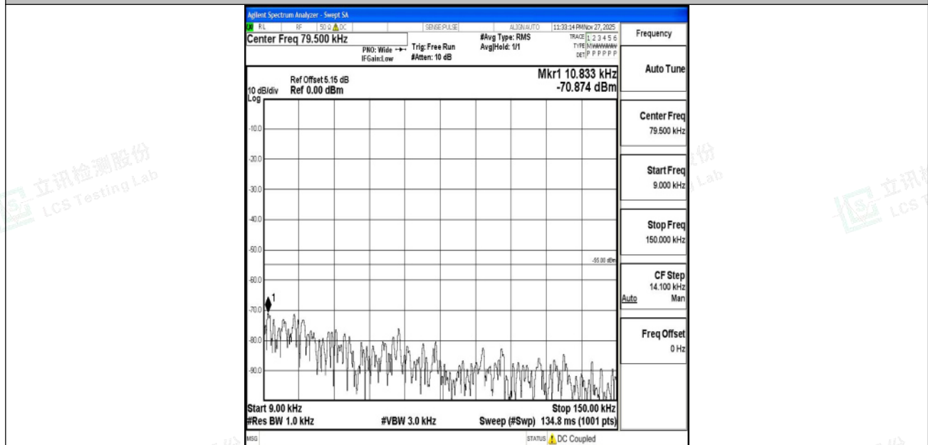
Band7_20MHz_16QAM_21100_1RB#0_0.009~0.15_0.009~0.15
