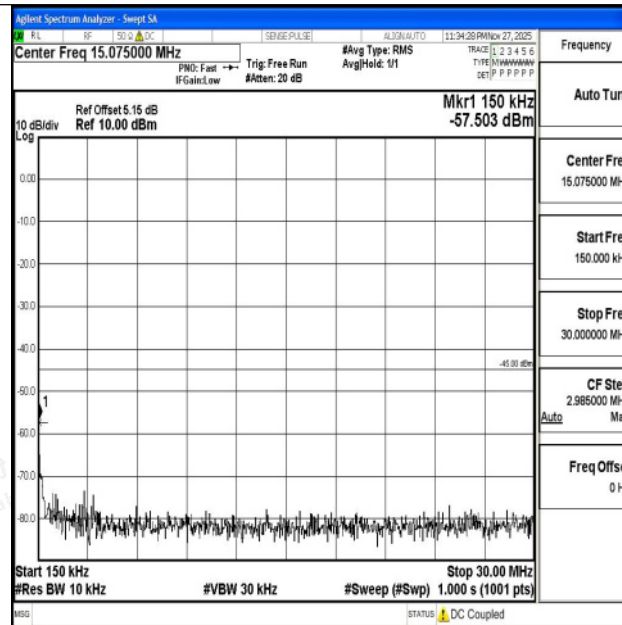
Band7_20MHz_16QAM_21350_1RB#0_0.15~30_0.15~30
