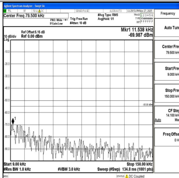
Band7_15MHz_16QAM_21100_1RB#0_0.009~0.15_0.009~0.15
