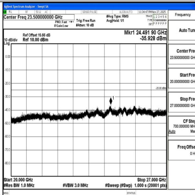
Band7_20MHz_16QAM_21350_1RB#0_20000~27000_20000~27000
