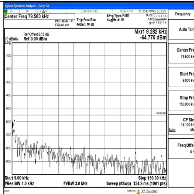
Band7_20MHz_QPSK_21100_1RB#0_0.009~0.15_0.009~0.15
