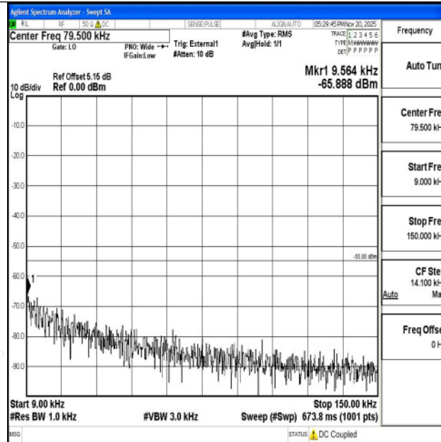
Band38_15MHz_QPSK_38000_1RB#0_0.009~0.15_0.009~0.15
