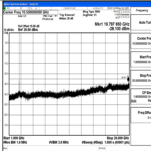
Band38_5MHz_16QAM_38225_1RB#0_1000~20000_1000~20000
