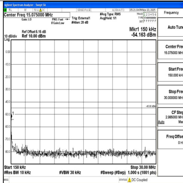
Band38_10MHz_16QAM_38200_1RB#0_0.15~30_0.15~30
