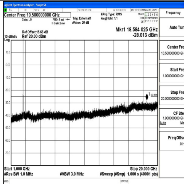
Band38_10MHz_QPSK_37800_1RB#0_1000~20000_1000~20000
