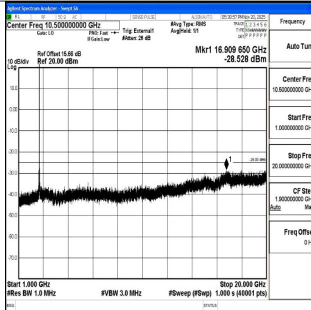
Band38_15MHz_QPSK_38000_1RB#0_1000~20000_1000~20000
