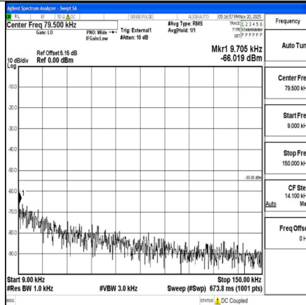
Band38_10MHz_16QAM_38000_1RB#0_0.009~0.15_0.009~0.15
