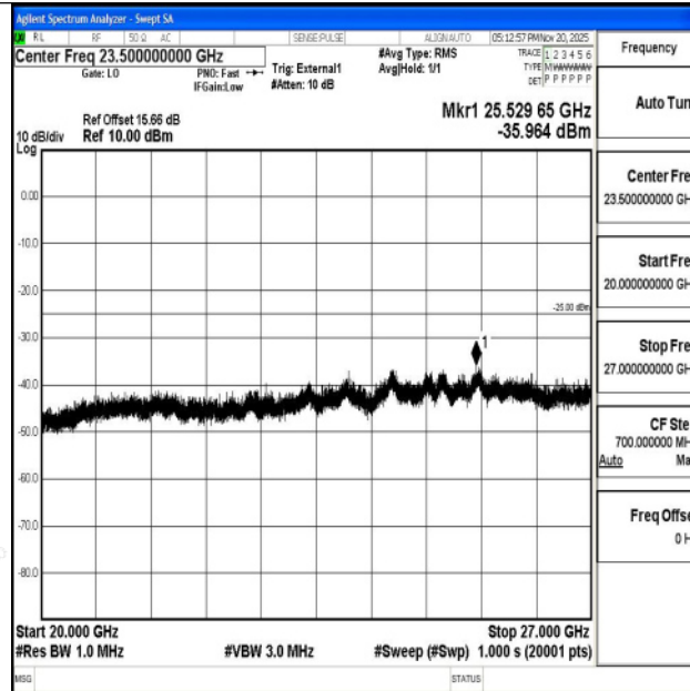
Band38_10MHz_QPSK_37800_1RB#0_20000~27000_20000~27000
