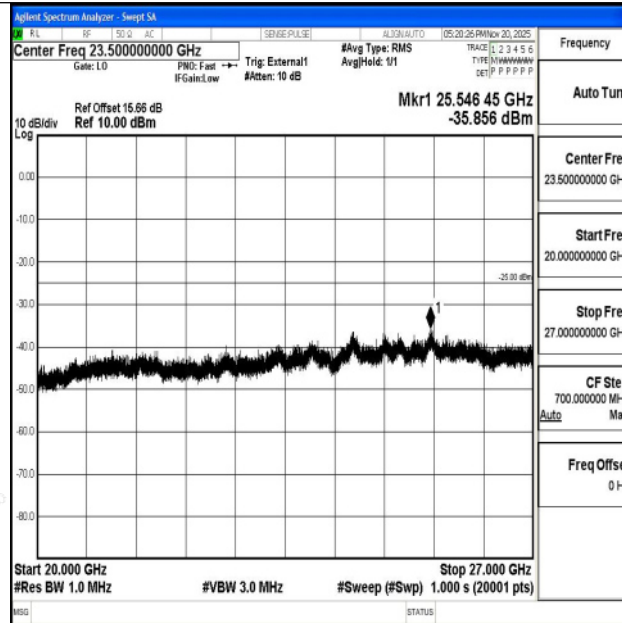
Band38_10MHz_QPSK_38200_1RB#0_20000~27000_20000~27000
