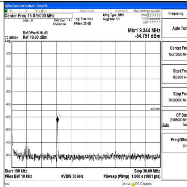
Band38_10MHz_16QAM_37800_1RB#0_0.15~30_0.15~30
