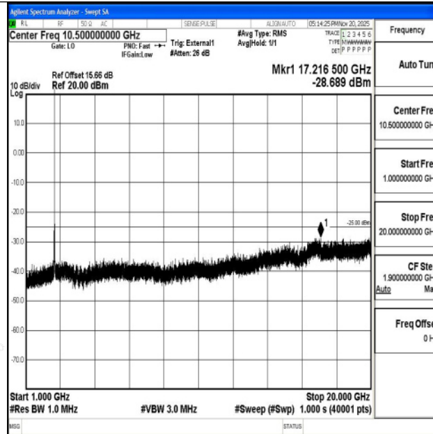
Band38_10MHz_16QAM_37800_1RB#0_1000~20000_1000~20000
