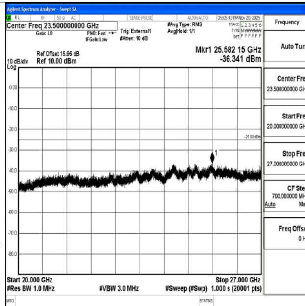
Band38_5MHz_QPSK_38225_1RB#0_20000~27000_20000~27000
