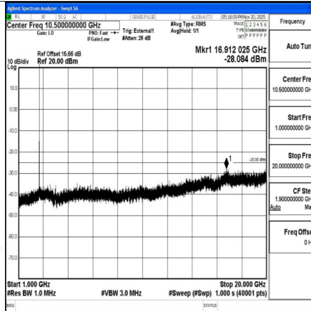
Band38_10MHz_16QAM_38000_1RB#0_1000~20000_1000~20000
