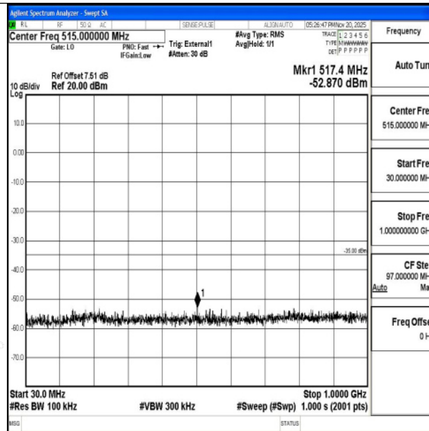
Band38_15MHz_QPSK_37825_1RB#0_30~1000_30~1000
