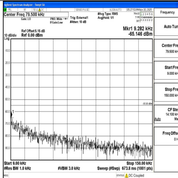
Band38_15MHz_16QAM_37825_1RB#0_0.009~0.15_0.009~0.15
