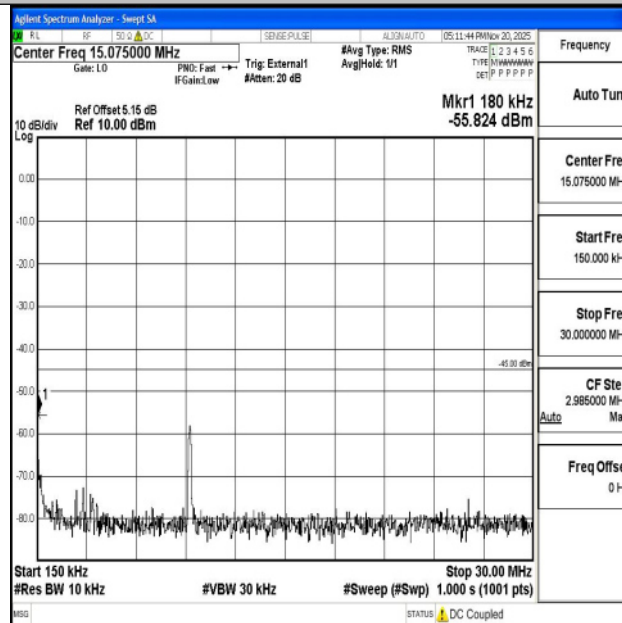
Band38_10MHz_QPSK_37800_1RB#0_0.15~30_0.15~30
