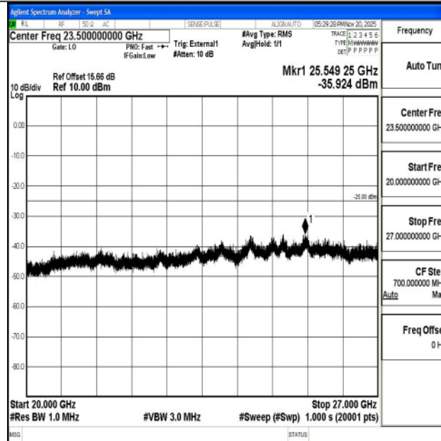
Band38_15MHz_16QAM_37825_1RB#0_20000~27000_20000~27000
