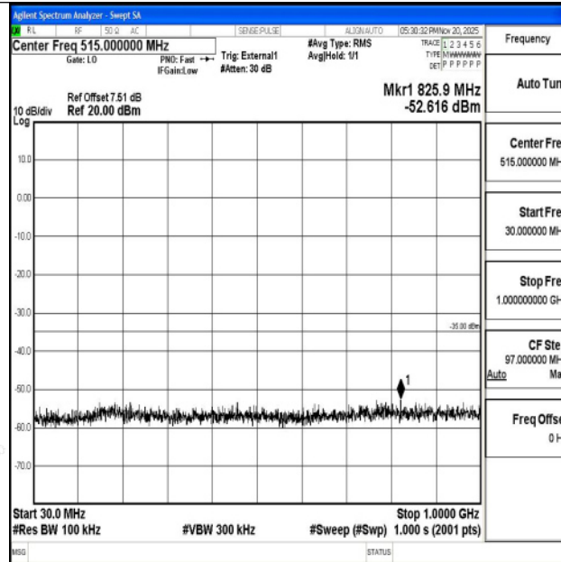
Band38_15MHz_QPSK_38000_1RB#0_30~1000_30~1000
