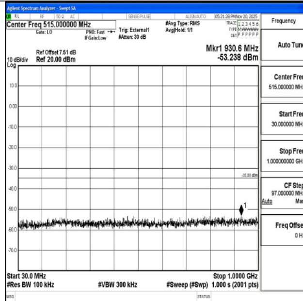
Band38_10MHz_16QAM_38200_1RB#0_30~1000_30~1000
