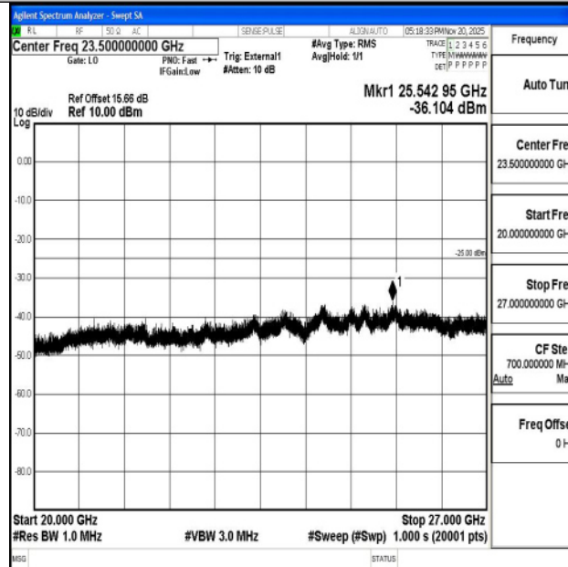
Band38_10MHz_16QAM_38000_1RB#0_20000~27000_20000~27000
