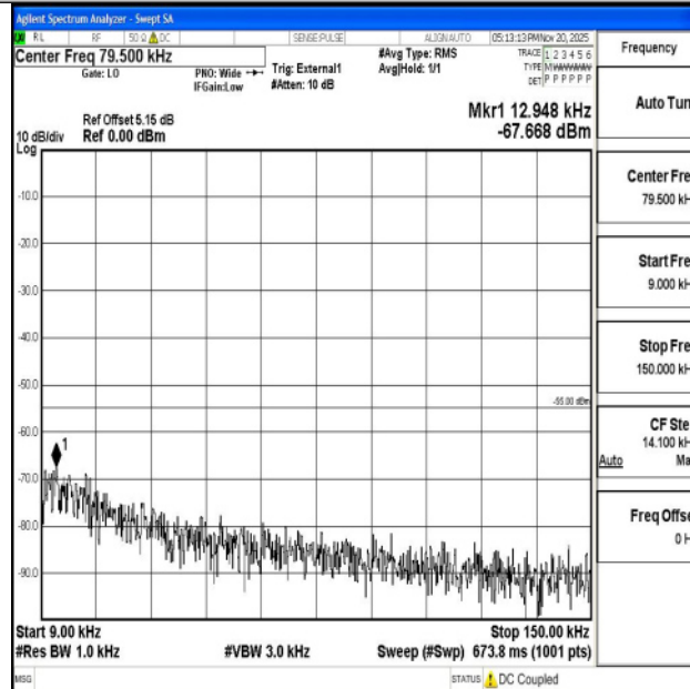
Band38_10MHz_16QAM_37800_1RB#0_0.009~0.15_0.009~0.15
