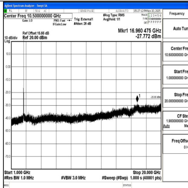
Band38_15MHz_QPSK_37825_1RB#0_1000~20000_1000~20000
