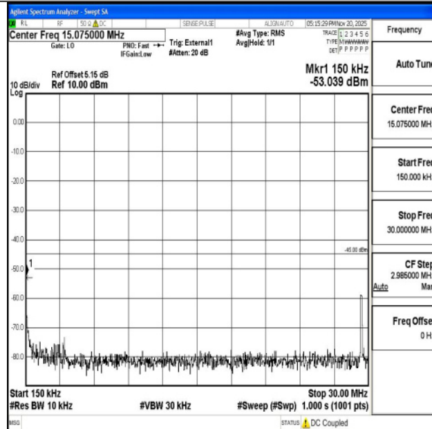
Band38_10MHz_QPSK_38000_1RB#0_0.15~30_0.15~30
