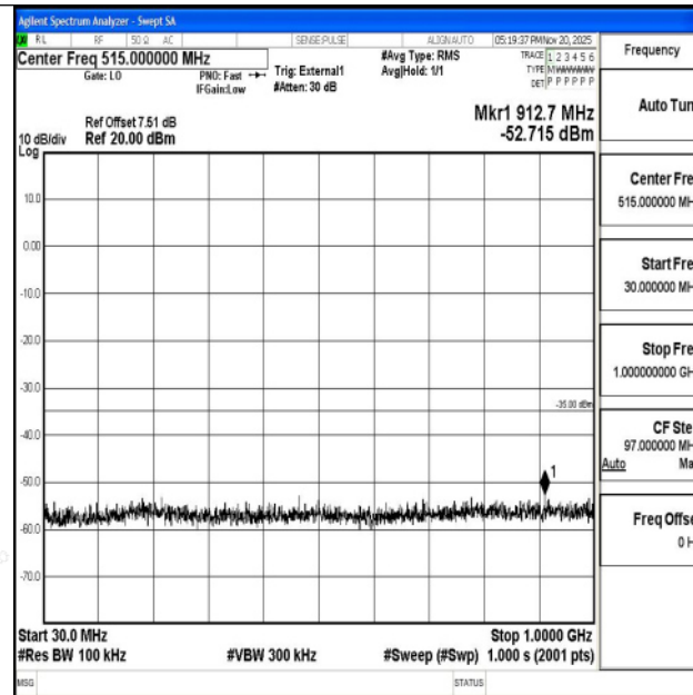
Band38_10MHz_QPSK_38200_1RB#0_30~1000_30~1000
