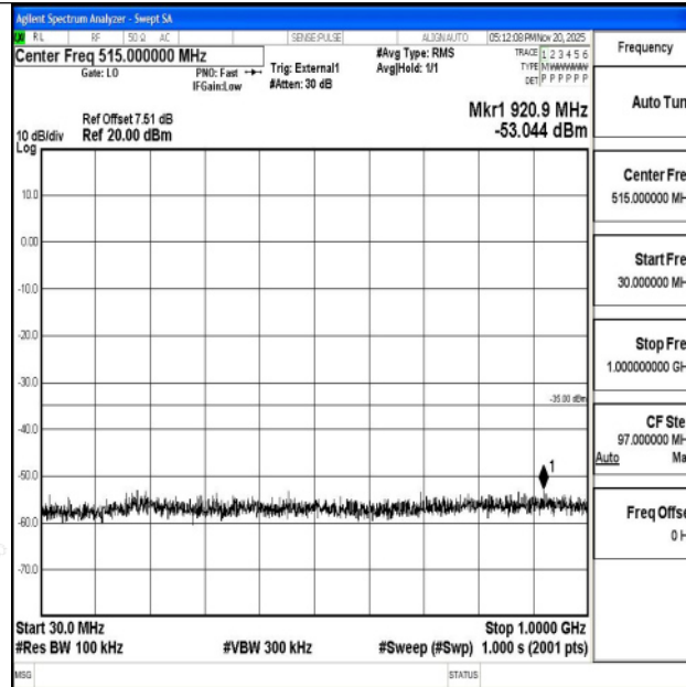
Band38_10MHz_QPSK_37800_1RB#0_30~1000_30~1000
