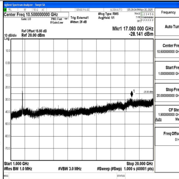
Band38_15MHz_16QAM_37825_1RB#0_1000~20000_1000~20000
