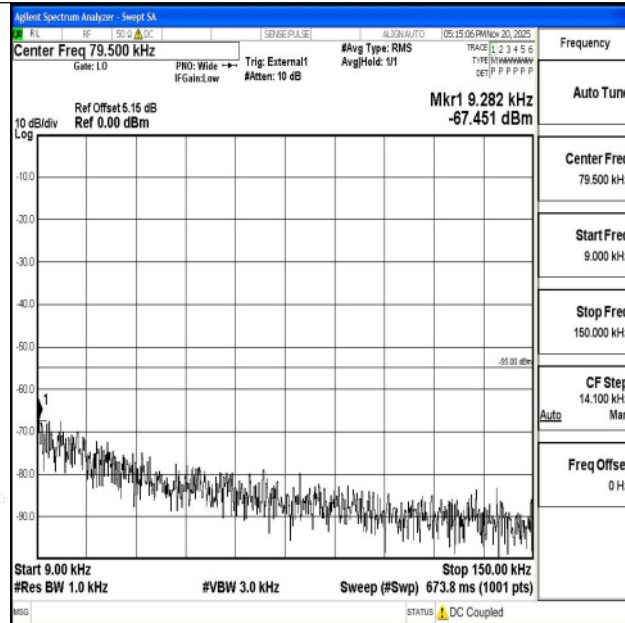
Band38_10MHz_QPSK_38000_1RB#0_0.009~0.15_0.009~0.15
