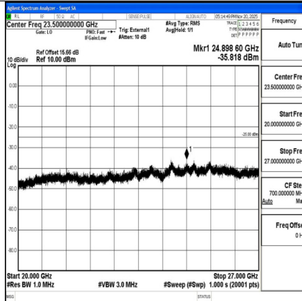
Band38_10MHz_16QAM_37800_1RB#0_20000~27000_20000~27000
