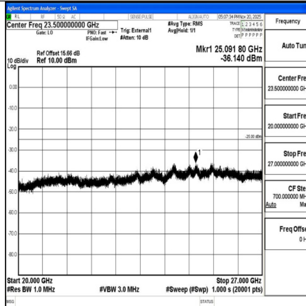
Band38_5MHz_16QAM_38225_1RB#0_20000~27000_20000~27000
