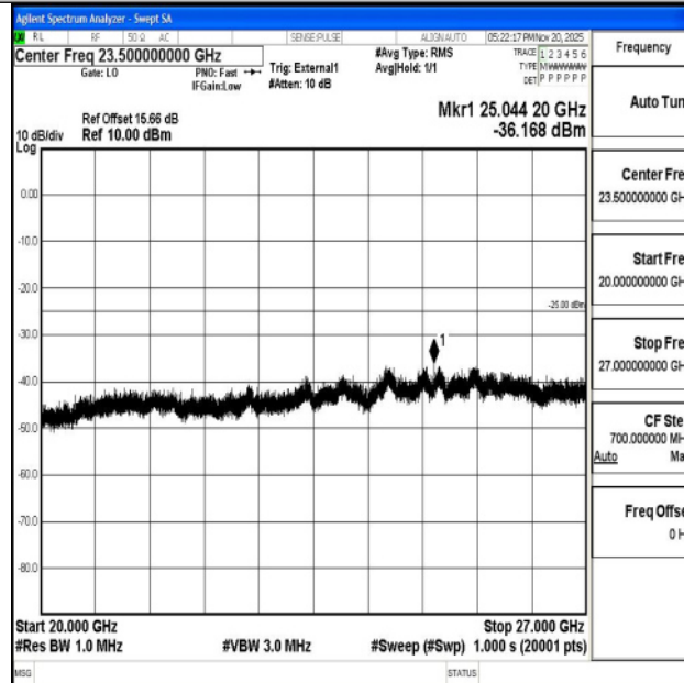
Band38_10MHz_16QAM_38200_1RB#0_20000~27000_20000~27000
