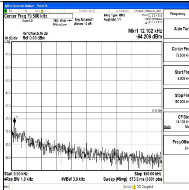
Band38_15MHz_QPSK_37825_1RB#0_0.009~0.15_0.009~0.15
