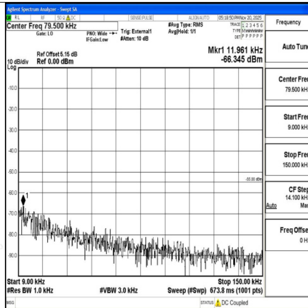
Band38_10MHz_QPSK_38200_1RB#0_0.009~0.15_0.009~0.15
