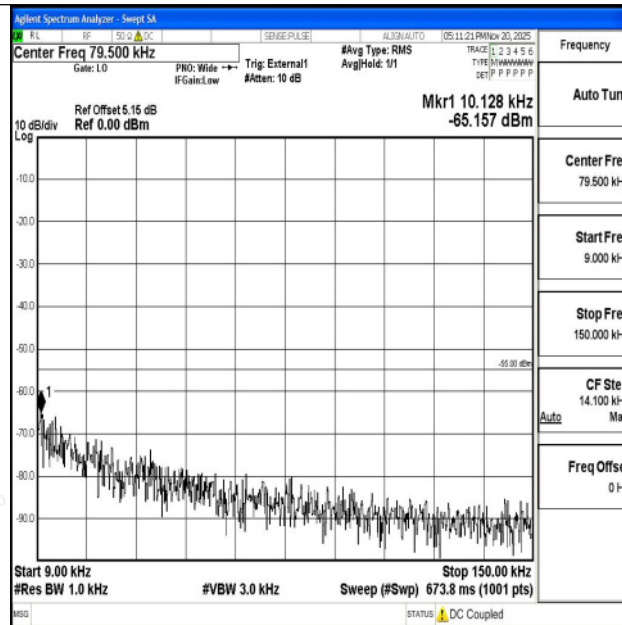
Band38_10MHz_QPSK_37800_1RB#0_0.009~0.15_0.009~0.15
