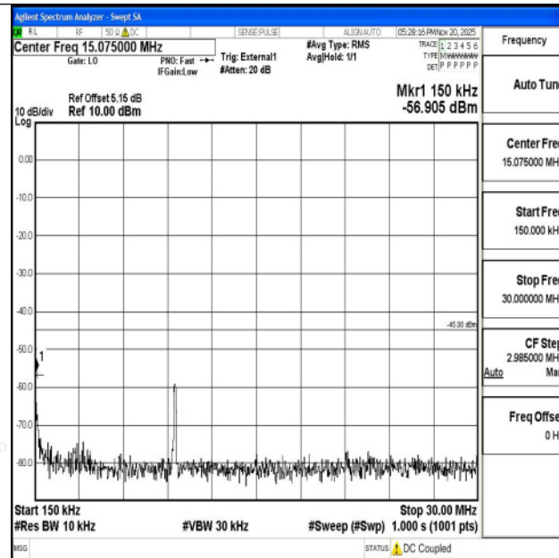
Band38_15MHz_16QAM_37825_1RB#0_0.15~30_0.15~30
