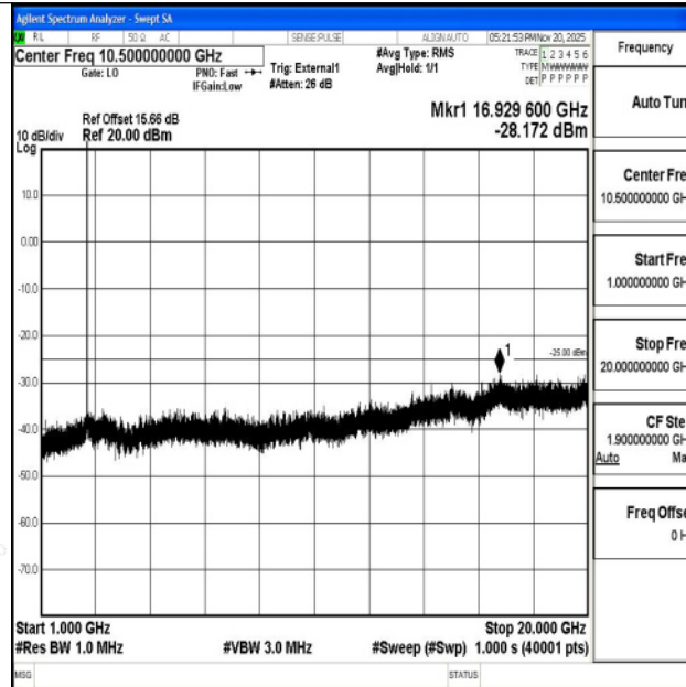
Band38_10MHz_16QAM_38200_1RB#0_1000~20000_1000~20000
