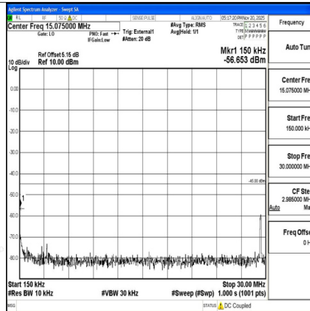
Band38_10MHz_16QAM_38000_1RB#0_0.15~30_0.15~30
