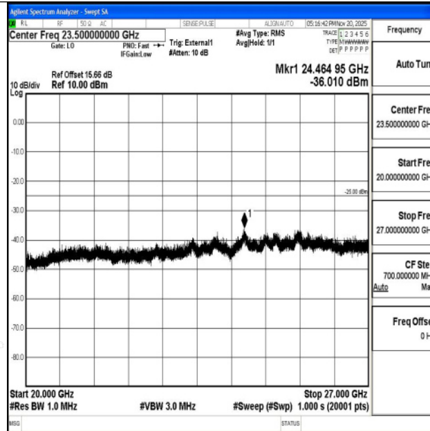
Band38_10MHz_QPSK_38000_1RB#0_20000~27000_20000~27000
