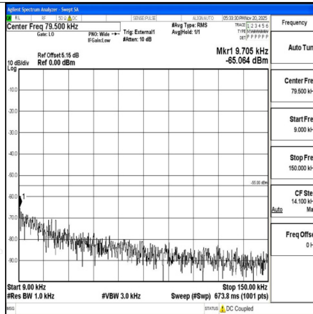
Band38_15MHz_QPSK_38175_1RB#0_0.009~0.15_0.009~0.15
