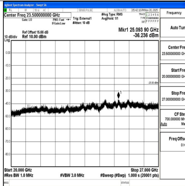
Band38_20MHz_QPSK_37850_1RB#0_20000~27000_20000~27000
