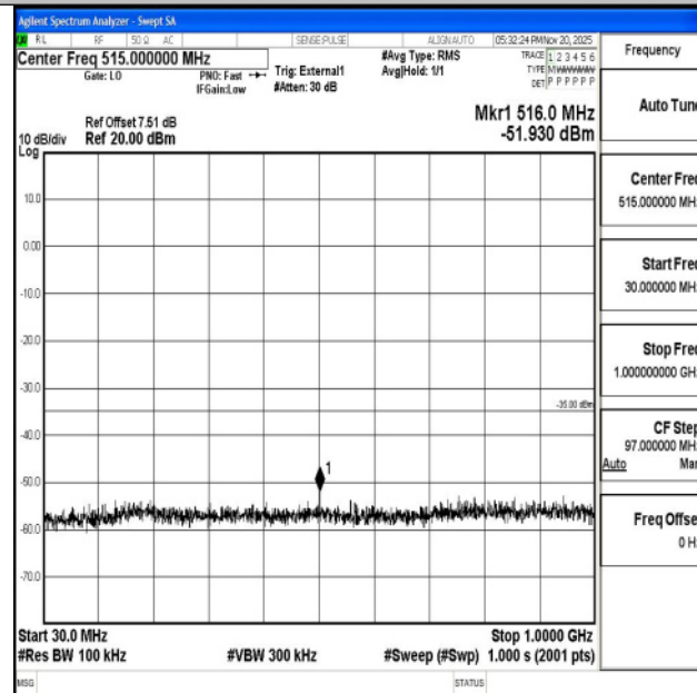
Band38_15MHz_16QAM_38000_1RB#0_30~1000_30~1000
