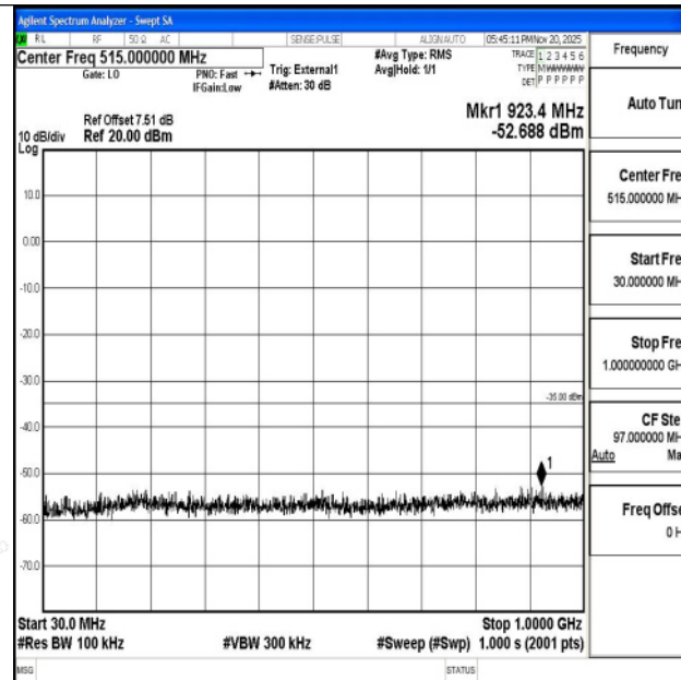
Band38_20MHz_QPSK_38000_1RB#0_30~1000_30~1000
