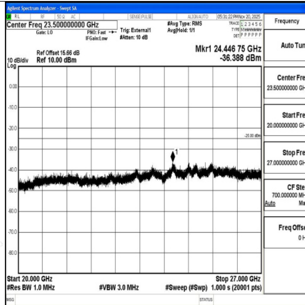
Band38_15MHz_QPSK_38000_1RB#0_20000~27000_20000~27000
