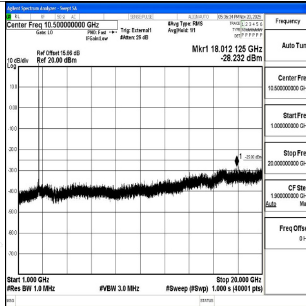
Band38_15MHz_16QAM_38175_1RB#0_1000~20000_1000~20000
