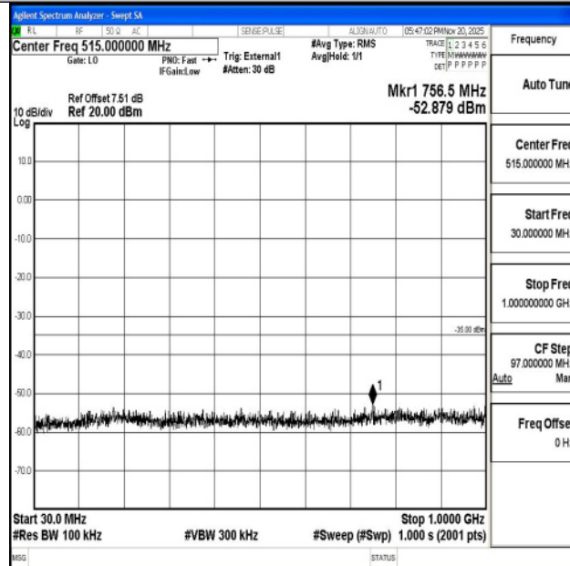
Band38_20MHz_16QAM_38000_1RB#0_30~1000_30~1000
