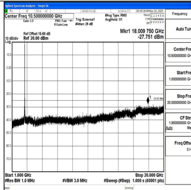
Band38_20MHz_QPSK_38000_1RB#0_1000~20000_1000~20000
