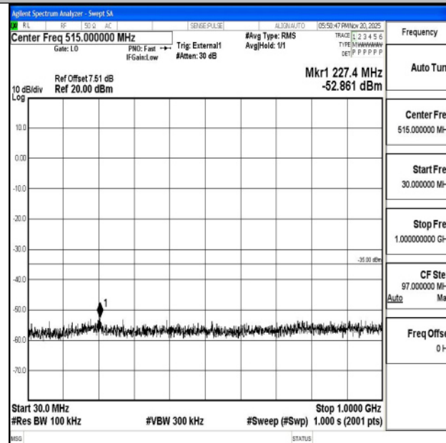
Band38_20MHz_16QAM_38150_1RB#0_30~1000_30~1000
