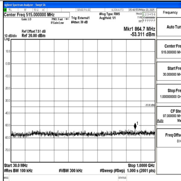
Band38_20MHz_QPSK_38150_1RB#0_30~1000_30~1000
