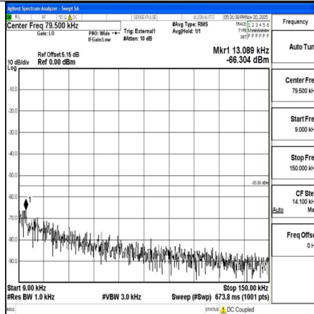
Band38_15MHz_16QAM_38000_1RB#0_0.009~0.15_0.009~0.15
