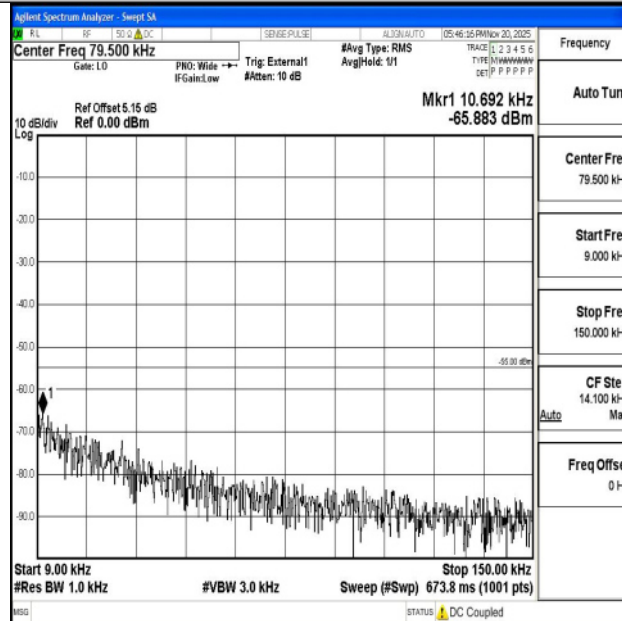
Band38_20MHz_16QAM_38000_1RB#0_0.009~0.15_0.009~0.15
