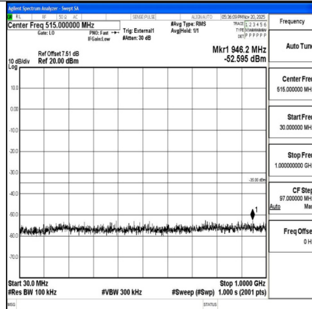
Band38_15MHz_16QAM_38175_1RB#0_30~1000_30~1000
