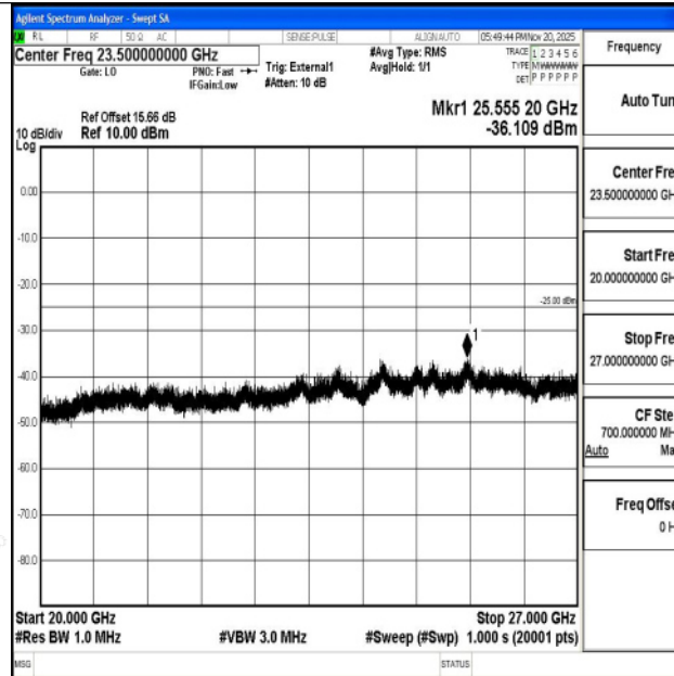
Band38_20MHz_QPSK_38150_1RB#0_20000~27000_20000~27000
