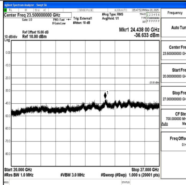
Band38_20MHz_16QAM_38000_1RB#0_20000~27000_20000~27000
