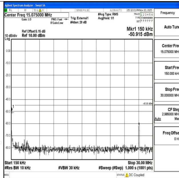
Band38_15MHz_16QAM_38000_1RB#0_0.15~30_0.15~30
