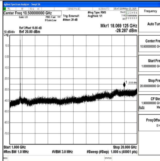
Band38_20MHz_16QAM_38000_1RB#0_1000~20000_1000~20000
