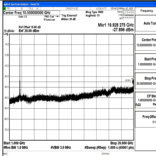
Band38_20MHz_QPSK_38150_1RB#0_1000~20000_1000~20000
