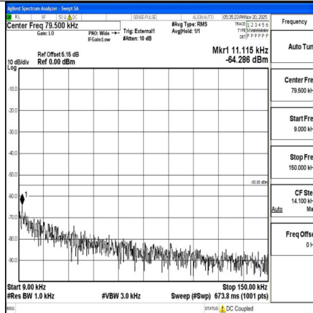
Band38_15MHz_16QAM_38175_1RB#0_0.009~0.15_0.009~0.15
