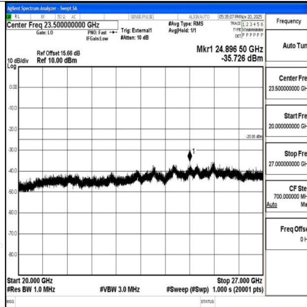
Band38_15MHz_QPSK_38175_1RB#0_20000~27000_20000~27000
