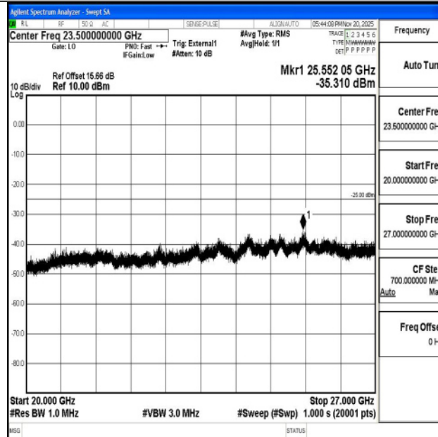
Band38_20MHz_16QAM_37850_1RB#0_20000~27000_20000~27000
