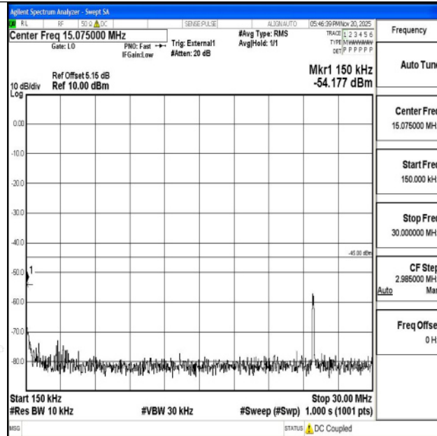
Band38_20MHz_16QAM_38000_1RB#0_0.15~30_0.15~30
