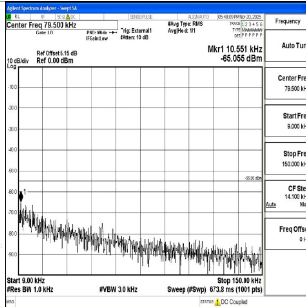
Band38_20MHz_QPSK_38150_1RB#0_0.009~0.15_0.009~0.15
