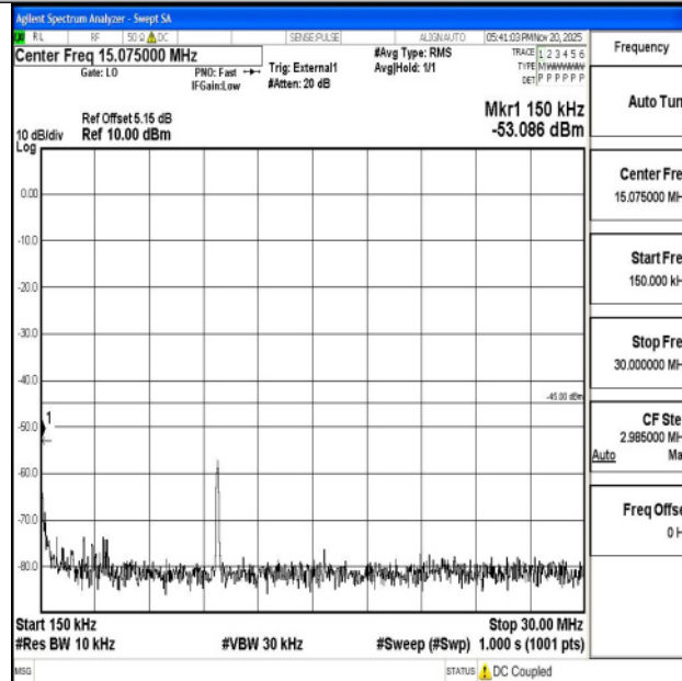
Band38_20MHz_QPSK_37850_1RB#0_0.15~30_0.15~30
