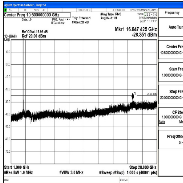
Band38_15MHz_16QAM_38000_1RB#0_1000~20000_1000~20000
