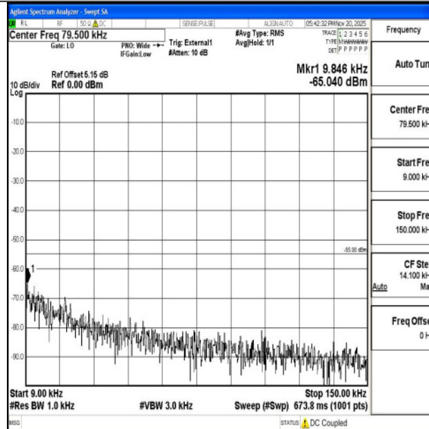
Band38_20MHz_16QAM_37850_1RB#0_0.009~0.15_0.009~0.15
