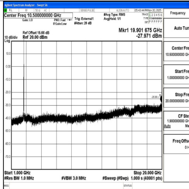
Band38_20MHz_16QAM_37850_1RB#0_1000~20000_1000~20000
