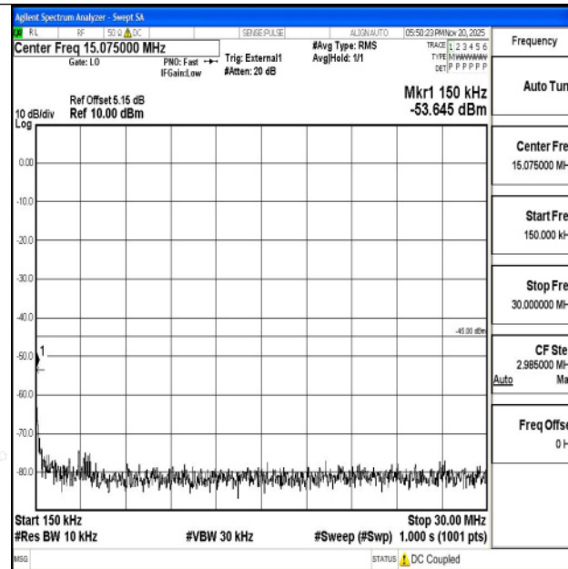
Band38_20MHz_16QAM_38150_1RB#0_0.15~30_0.15~30
