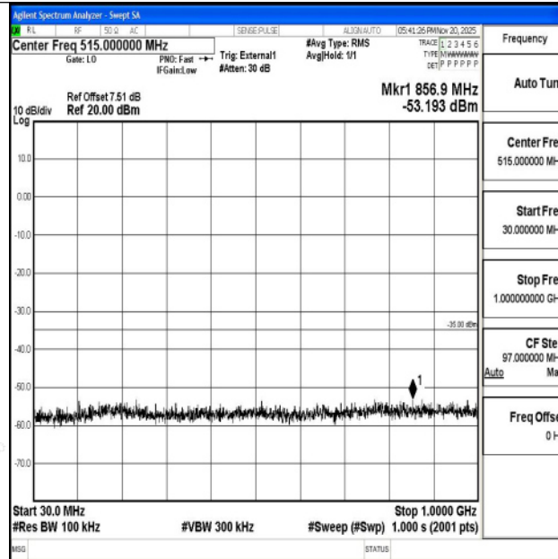
Band38_20MHz_QPSK_37850_1RB#0_30~1000_30~1000
