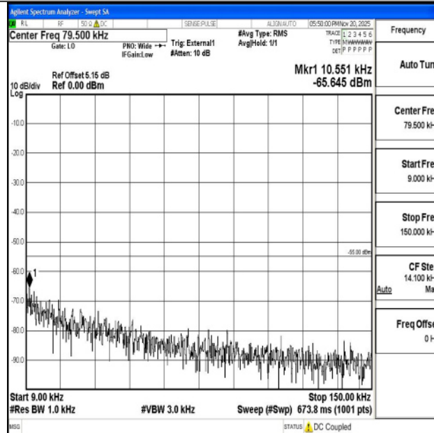
Band38_20MHz_16QAM_38150_1RB#0_0.009~0.15_0.009~0.15
