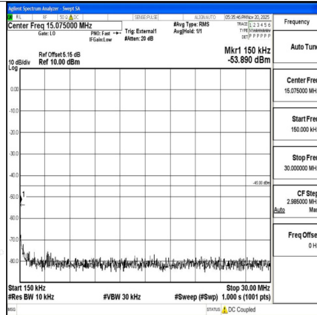
Band38_15MHz_16QAM_38175_1RB#0_0.15~30_0.15~30
