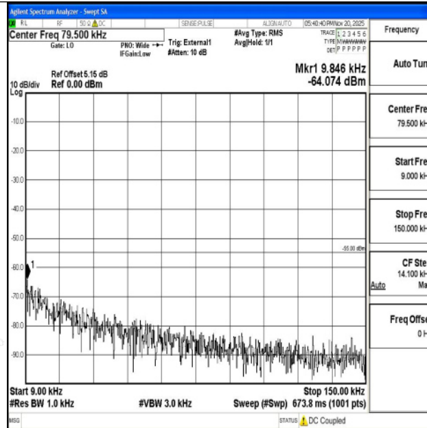
Band38_20MHz_QPSK_37850_1RB#0_0.009~0.15_0.009~0.15
