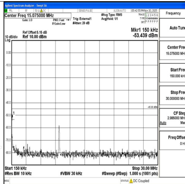
Band38_20MHz_16QAM_37850_1RB#0_0.15~30_0.15~30
