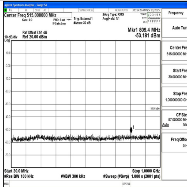
Band38_15MHz_QPSK_38175_1RB#0_30~1000_30~1000
