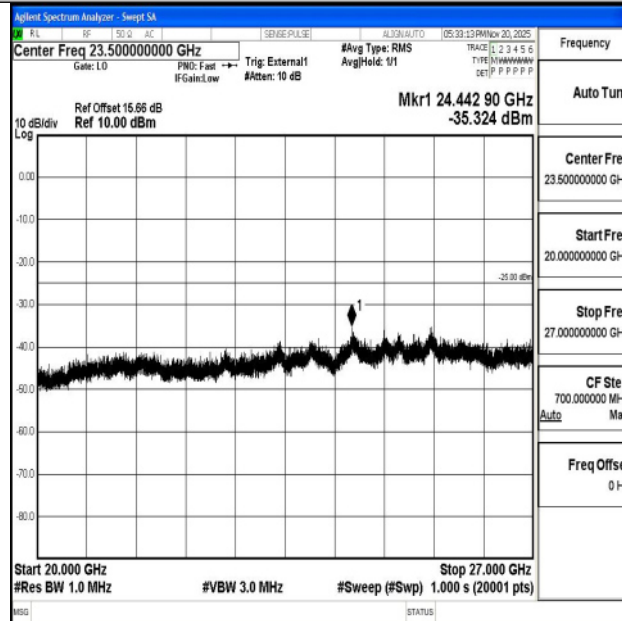
Band38_15MHz_16QAM_38000_1RB#0_20000~27000_20000~27000
