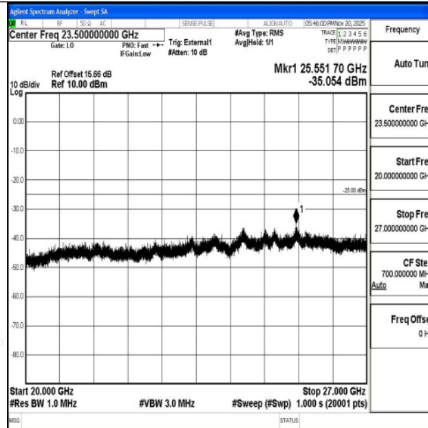
Band38_20MHz_QPSK_38000_1RB#0_20000~27000_20000~27000
