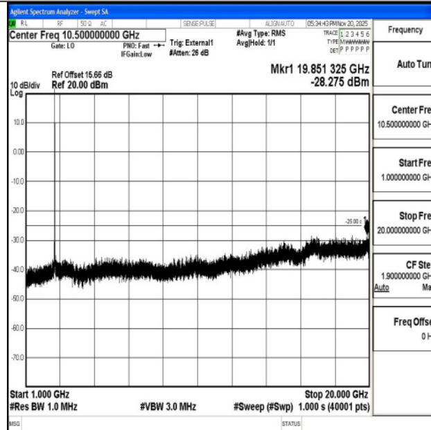
Band38_15MHz_QPSK_38175_1RB#0_1000~20000_1000~20000
