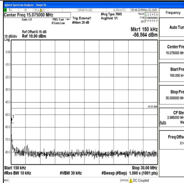
Band38_20MHz_QPSK_38150_1RB#0_0.15~30_0.15~30
