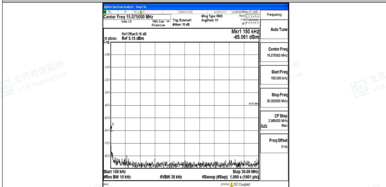
Band41_5MHz_QPSK_41565_1RB#0_0.15~30_0.15~30
