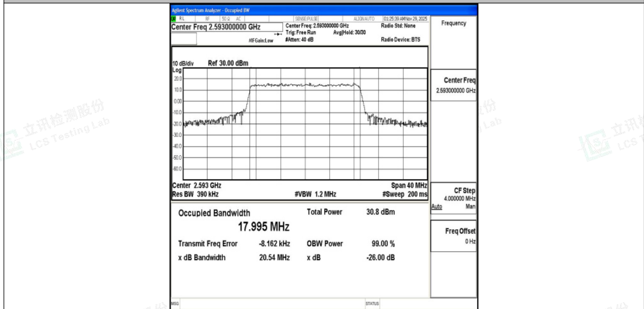
Band41-20MHz-16QAM-40620-100RB#0-PASS
