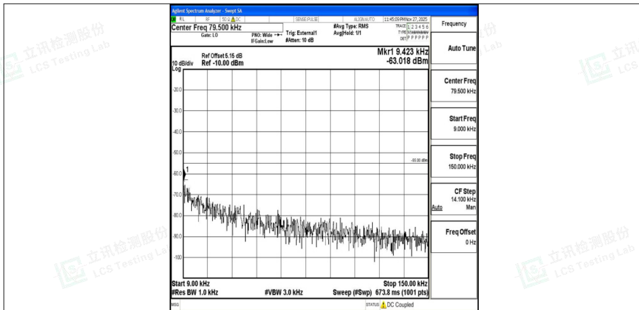
Band41_5MHz_QPSK_41565_1RB#0_0.009~0.15_0.009~0.15
