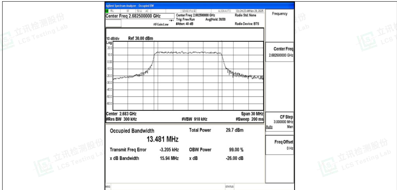
Band41-15MHz-QPSK-41515-75RB#0-PASS
