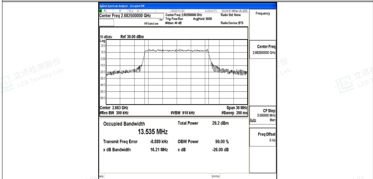
Band41-15MHz-16QAM-41515-75RB#0-PASS
