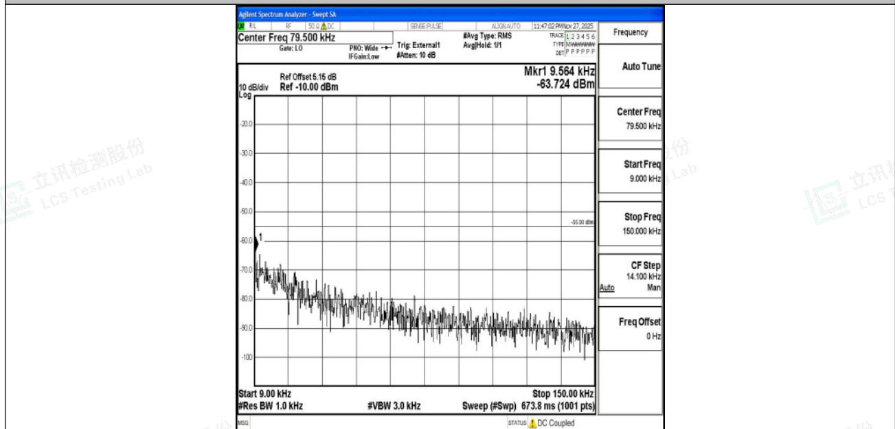
Band41_5MHz_16QAM_41565_1RB#0_0.009~0.15_0.009~0.15
