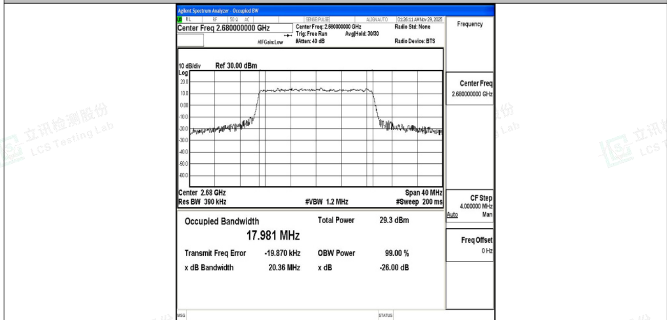
Band41-20MHz-16QAM-41490-100RB#0-PASS
