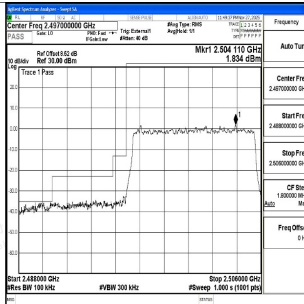
Band41_10MHz_16QAM_39700_50RB#0
