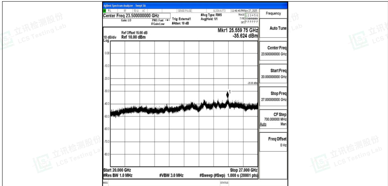
Band41_5MHz_QPSK_41565_1RB#0_20000~27000_20000~27000
