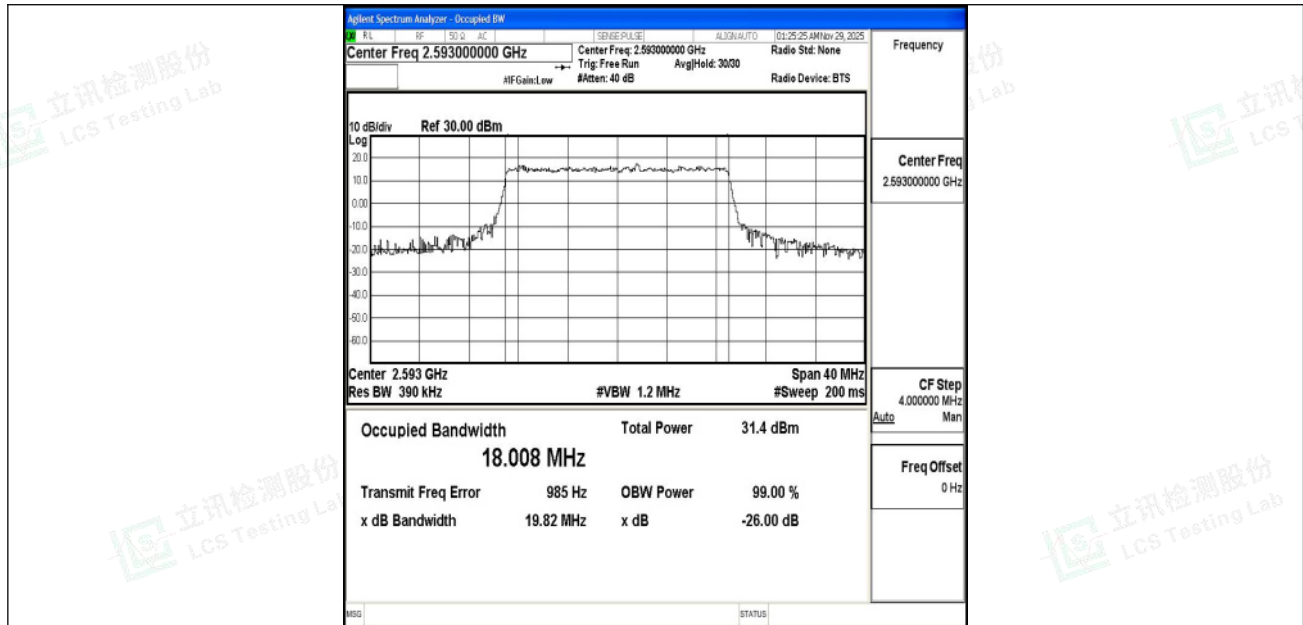
Band41-20MHz-QPSK-40620-100RB#0-PASS
