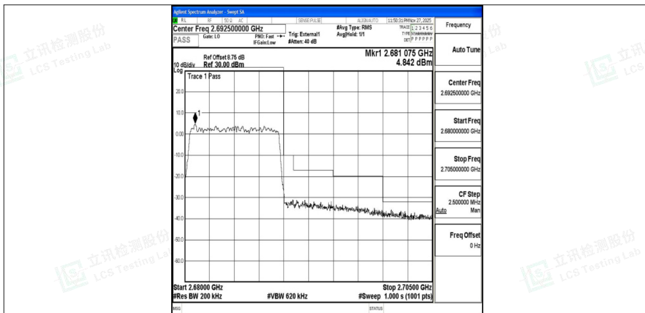
Band41_10MHz_16QAM_41540_50RB#0
