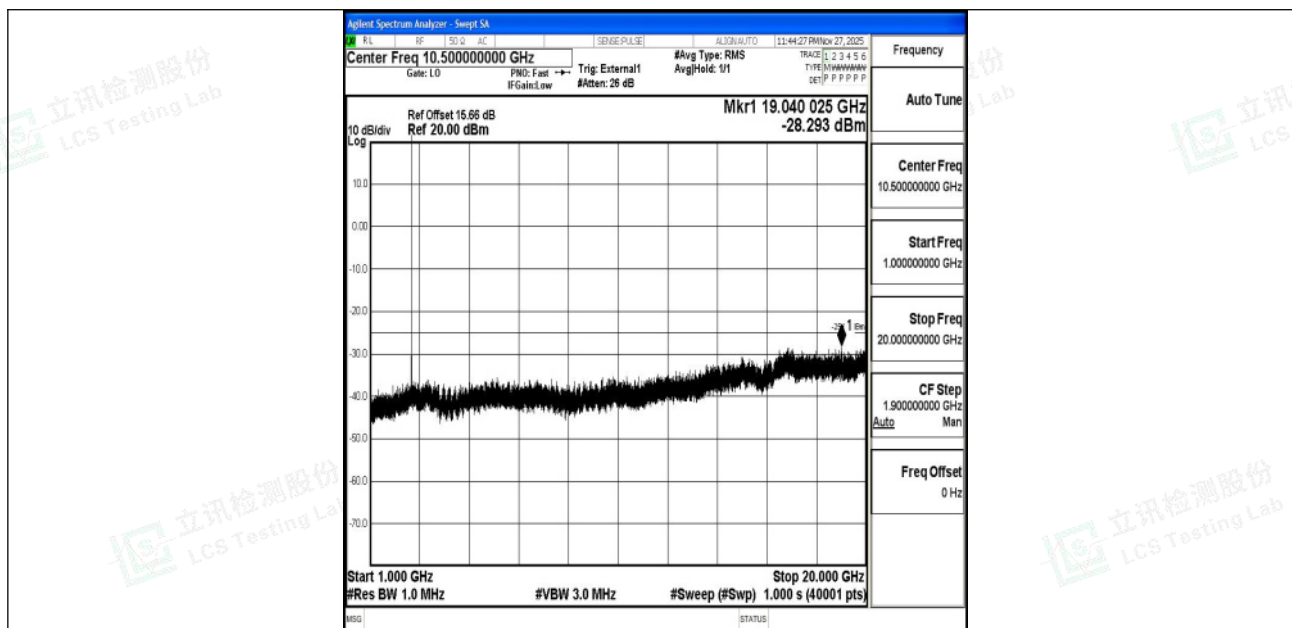
Band41_5MHz_16QAM_40620_1RB#0_1000~20000_1000~20000
