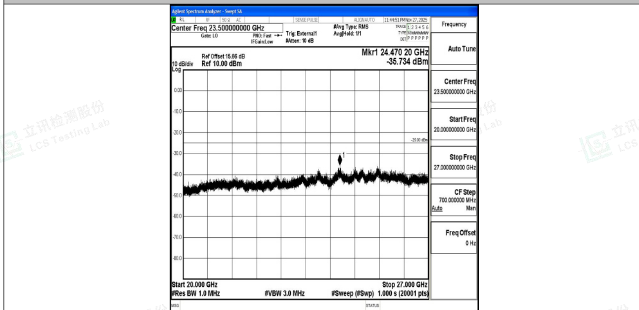
Band41_5MHz_16QAM_40620_1RB#0_20000~27000_20000~27000
