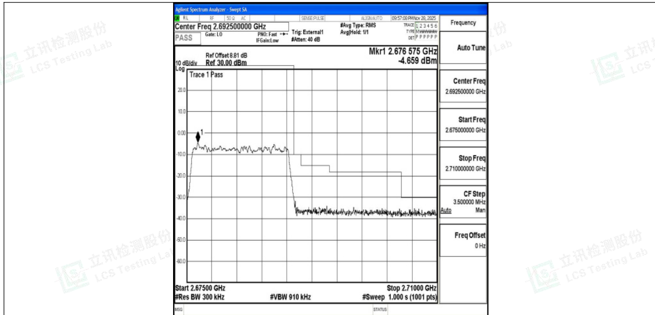
Band41_15MHz_16QAM_41515_75RB#0
