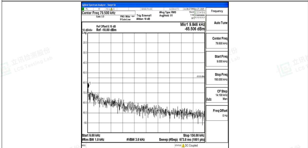
Band41_5MHz_16QAM_39675_1RB#0_0.009~0.15_0.009~0.15
