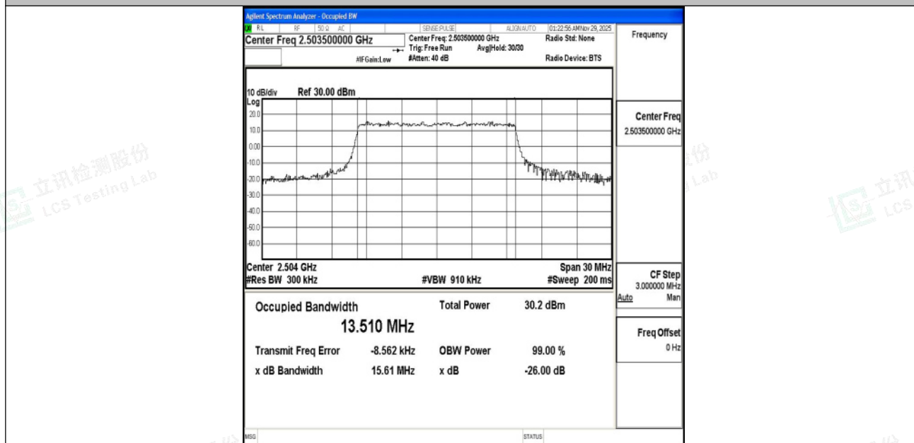
Band41-15MHz-16QAM-39725-75RB#0-PASS
