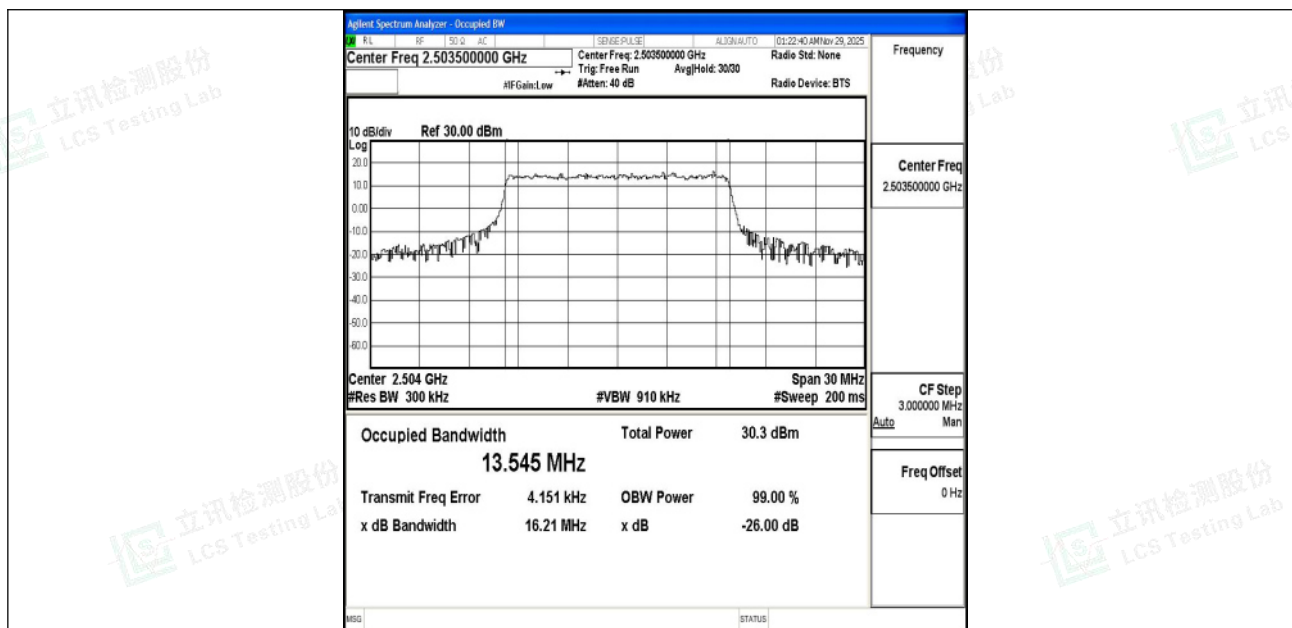
Band41-15MHz-QPSK-39725-75RB#0-PASS
