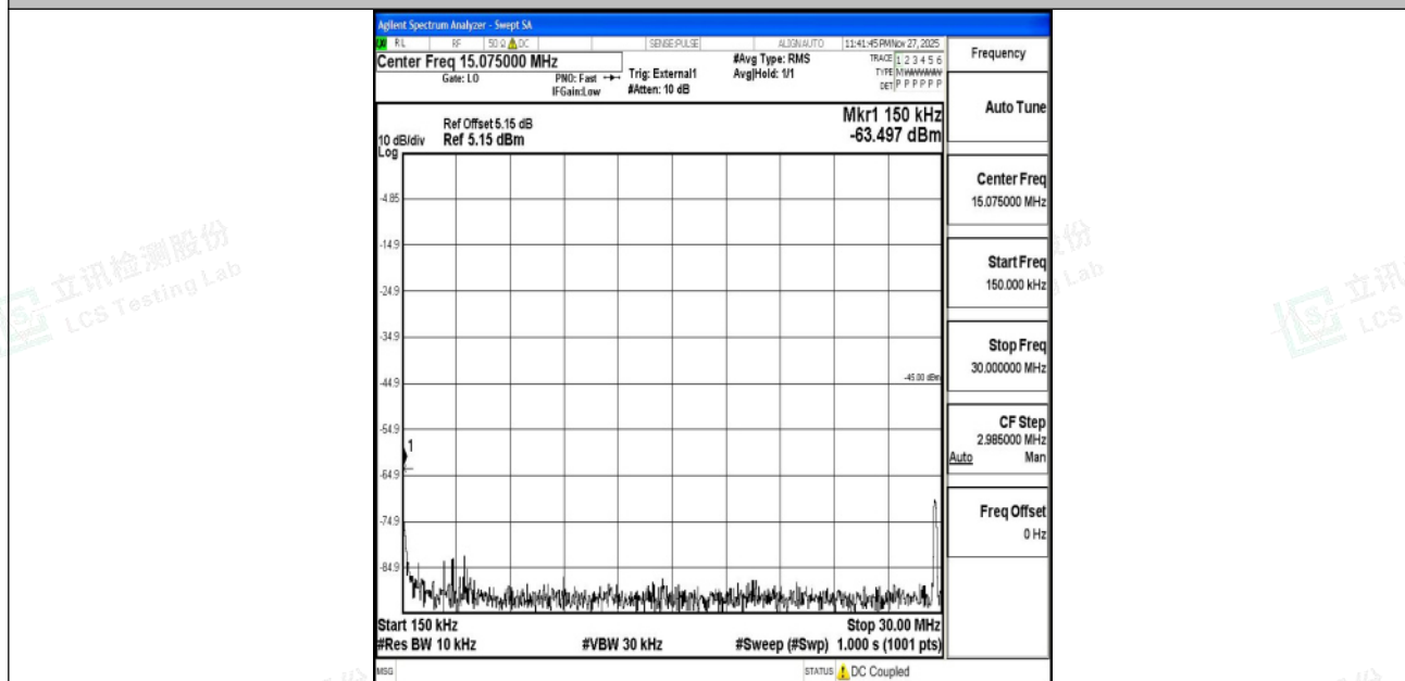
Band41_5MHz_QPSK_40620_1RB#0_0.15~30_0.15~30
