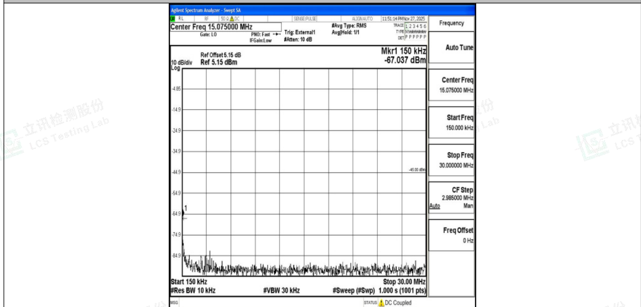
Band41_10MHz_QPSK_39700_1RB#0_0.15~30_0.15~30
