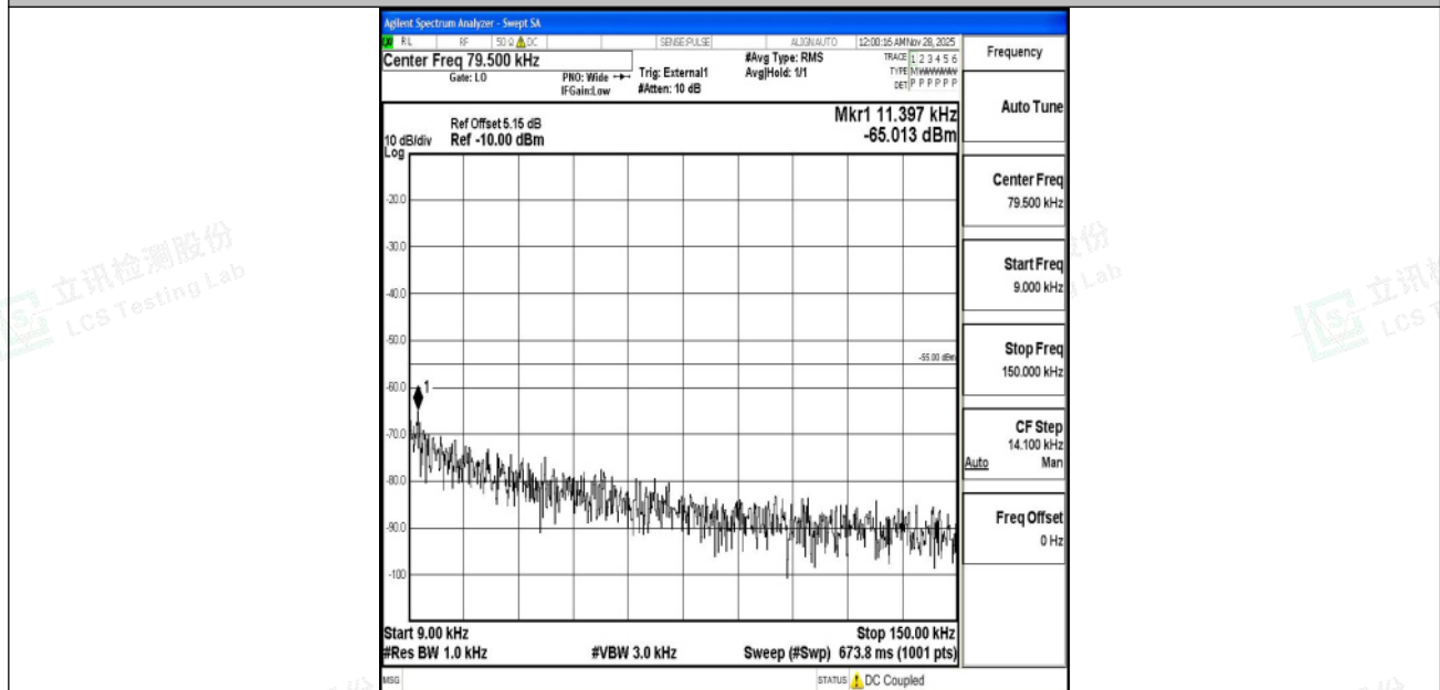
Band41_10MHz_16QAM_41540_1RB#0_0.009~0.15_0.009~0.15
