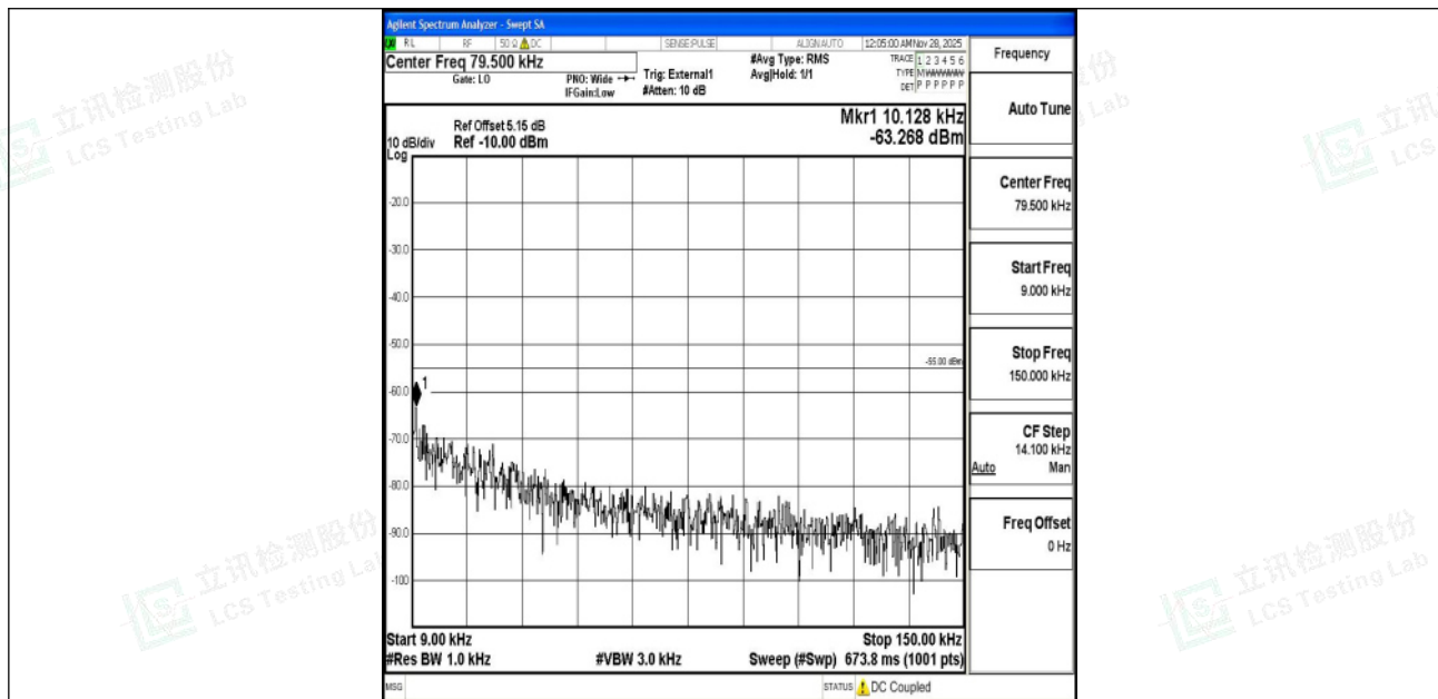
Band41_15MHz_QPSK_39725_1RB#0_0.009~0.15_0.009~0.15
