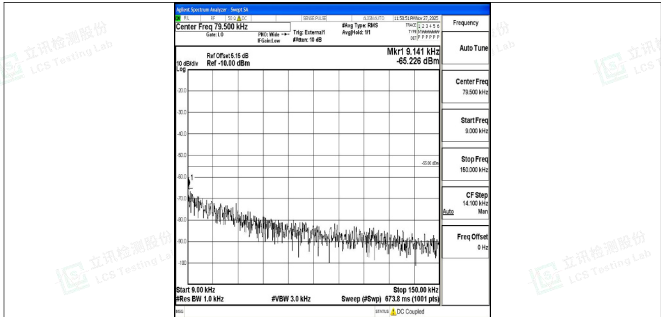
Band41_10MHz_QPSK_39700_1RB#0_0.009~0.15_0.009~0.15
