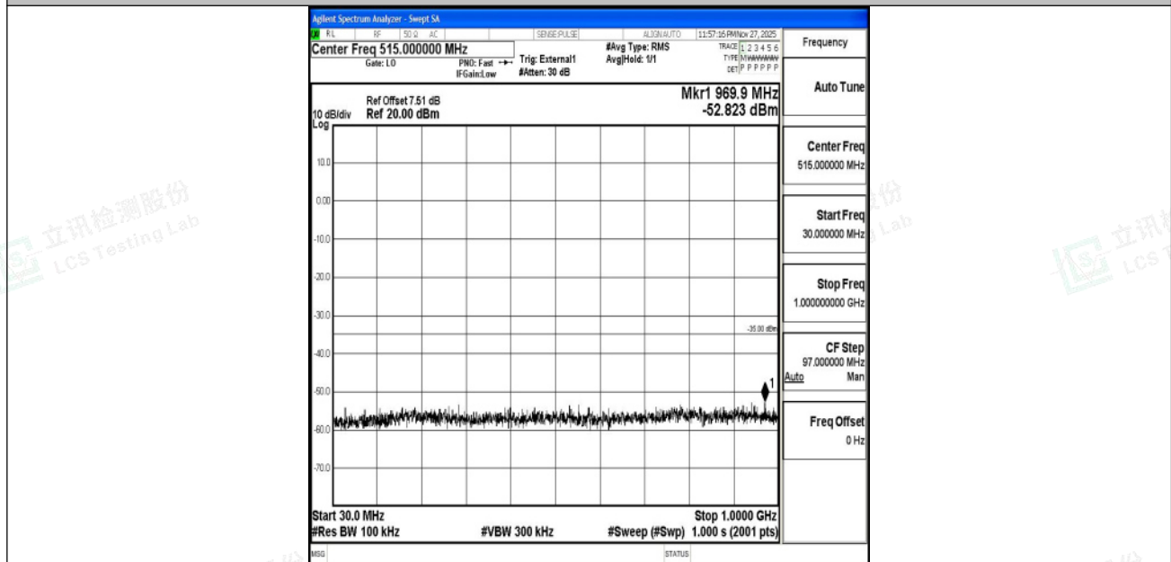
Band41_10MHz_16QAM_40620_1RB#0_30~1000_30~1000
