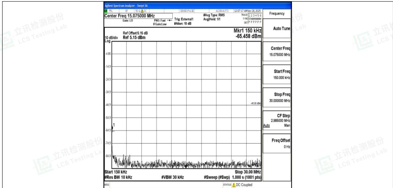
Band41_15MHz_16QAM_39725_1RB#0_0.15~30_0.15~30
