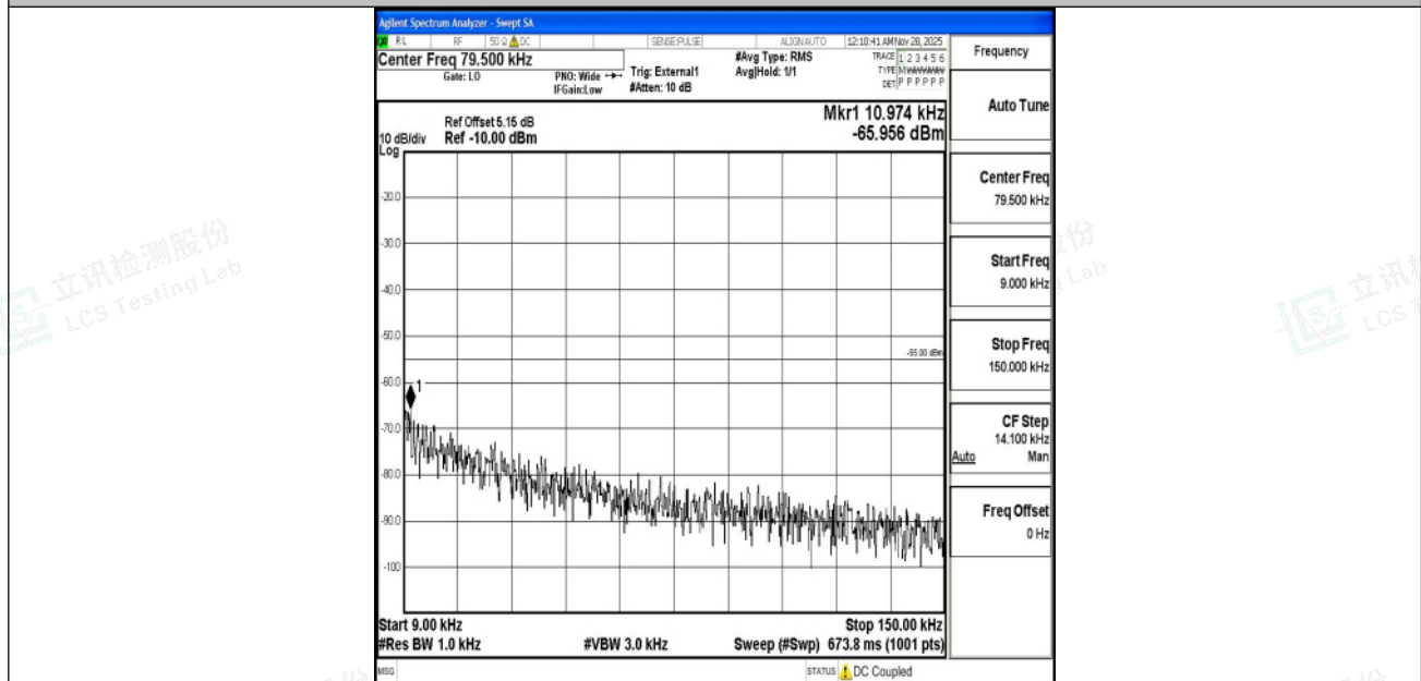
Band41_15MHz_16QAM_40620_1RB#0_0.009~0.15_0.009~0.15
