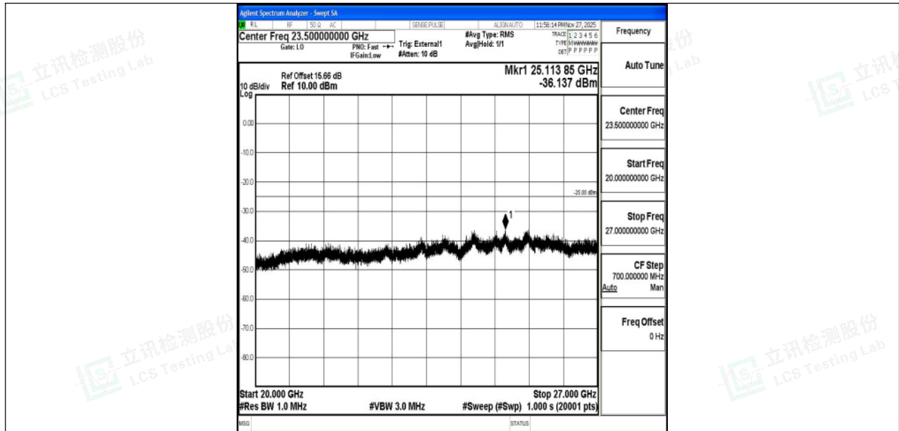
Band41_10MHz_QPSK_40620_1RB#0_20000~27000_20000~27000
