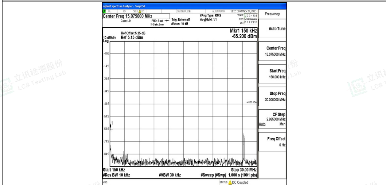
Band41_10MHz_QPSK_40620_1RB#0_0.15~30_0.15~30
