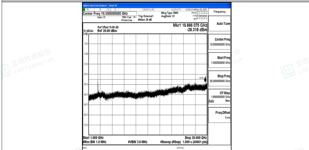
Band41_15MHz_QPSK_39725_1RB#0_1000~20000_1000~20000
