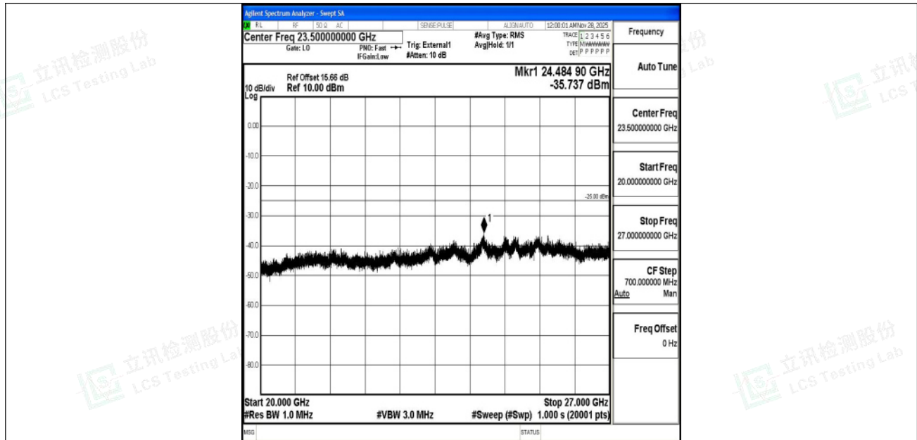
Band41_10MHz_QPSK_41540_1RB#0_20000~27000_20000~27000
