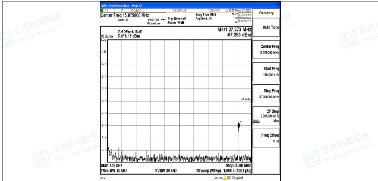
Band41_10MHz_16QAM_40620_1RB#0_0.15~30_0.15~30
