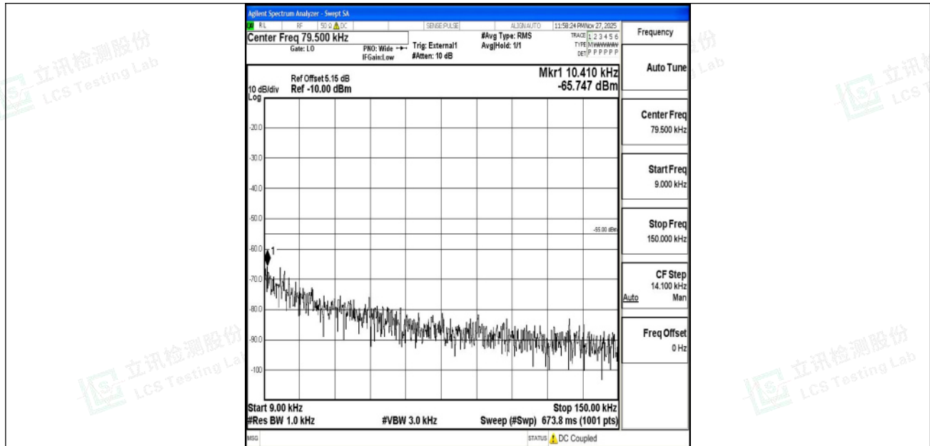
Band41_10MHz_QPSK_41540_1RB#0_0.009~0.15_0.009~0.15
