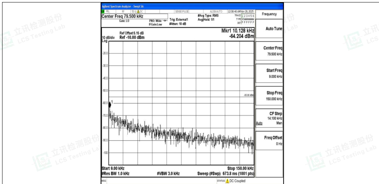
Band41_15MHz_QPSK_40620_1RB#0_0.009~0.15_0.009~0.15
