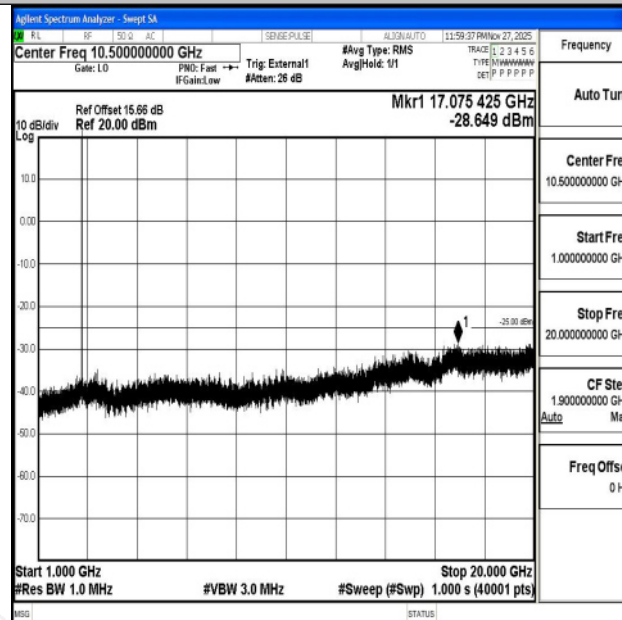
Band41_10MHz_QPSK_41540_1RB#0_1000~20000_1000~20000
