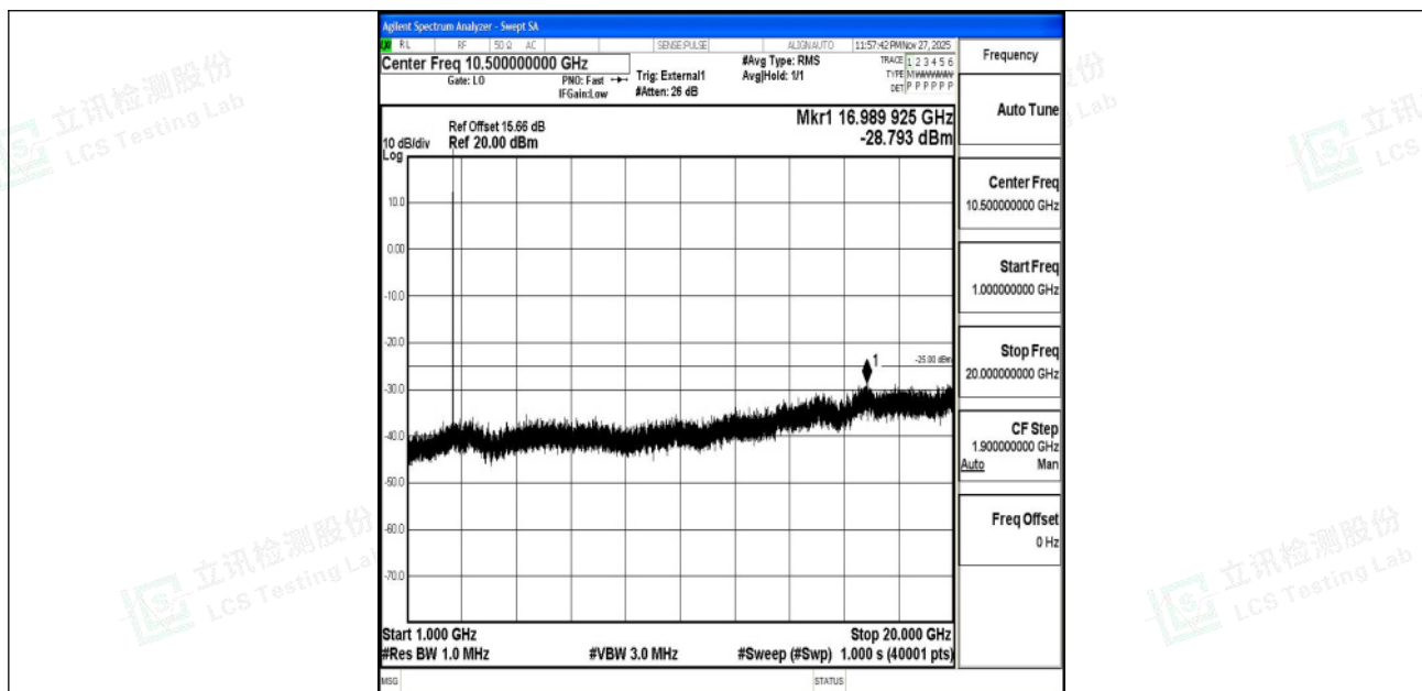
Band41_10MHz_16QAM_40620_1RB#0_1000~20000_1000~20000
