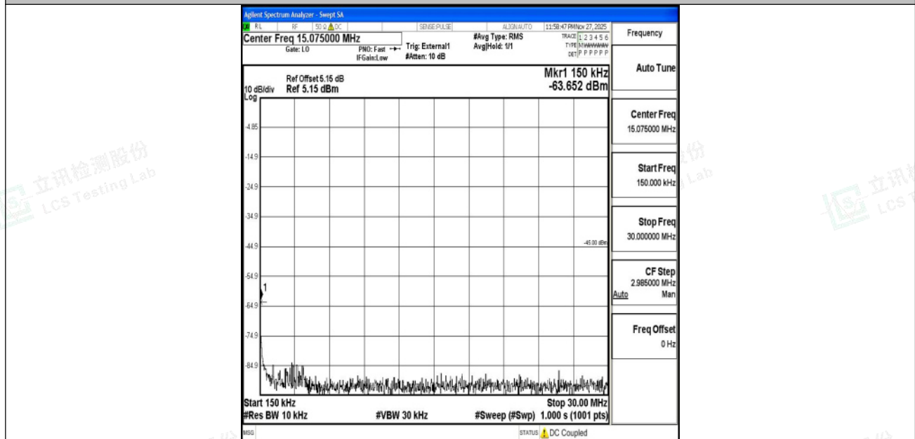
Band41_10MHz_QPSK_41540_1RB#0_0.15~30_0.15~30
