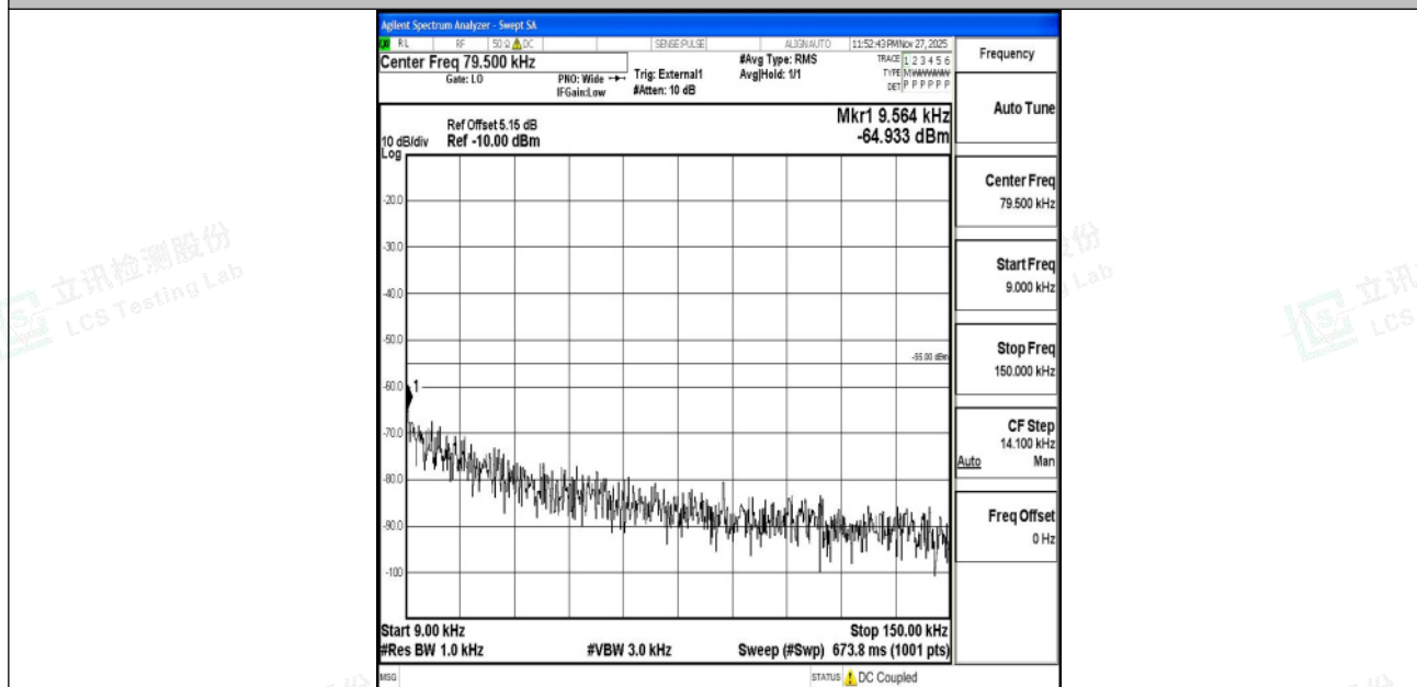
Band41_10MHz_16QAM_39700_1RB#0_0.009~0.15_0.009~0.15
