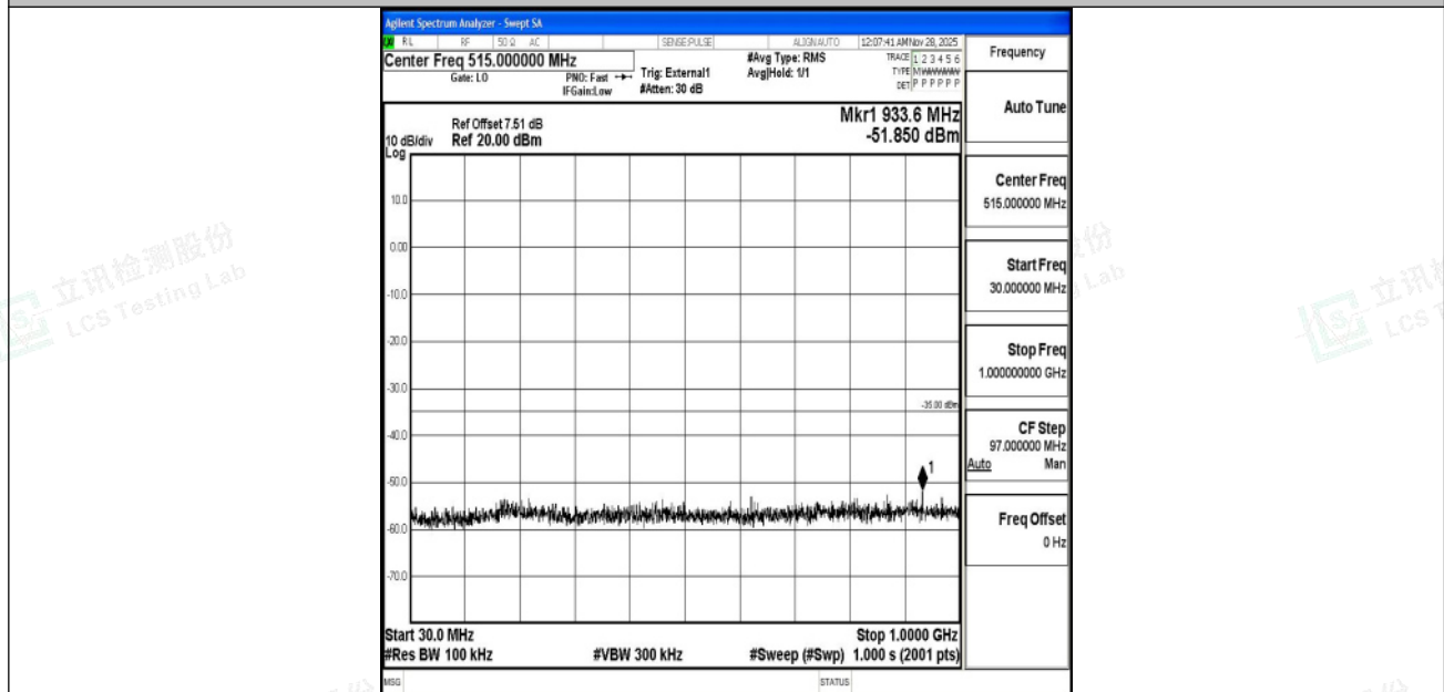
Band41_15MHz_16QAM_39725_1RB#0_30~1000_30~1000
