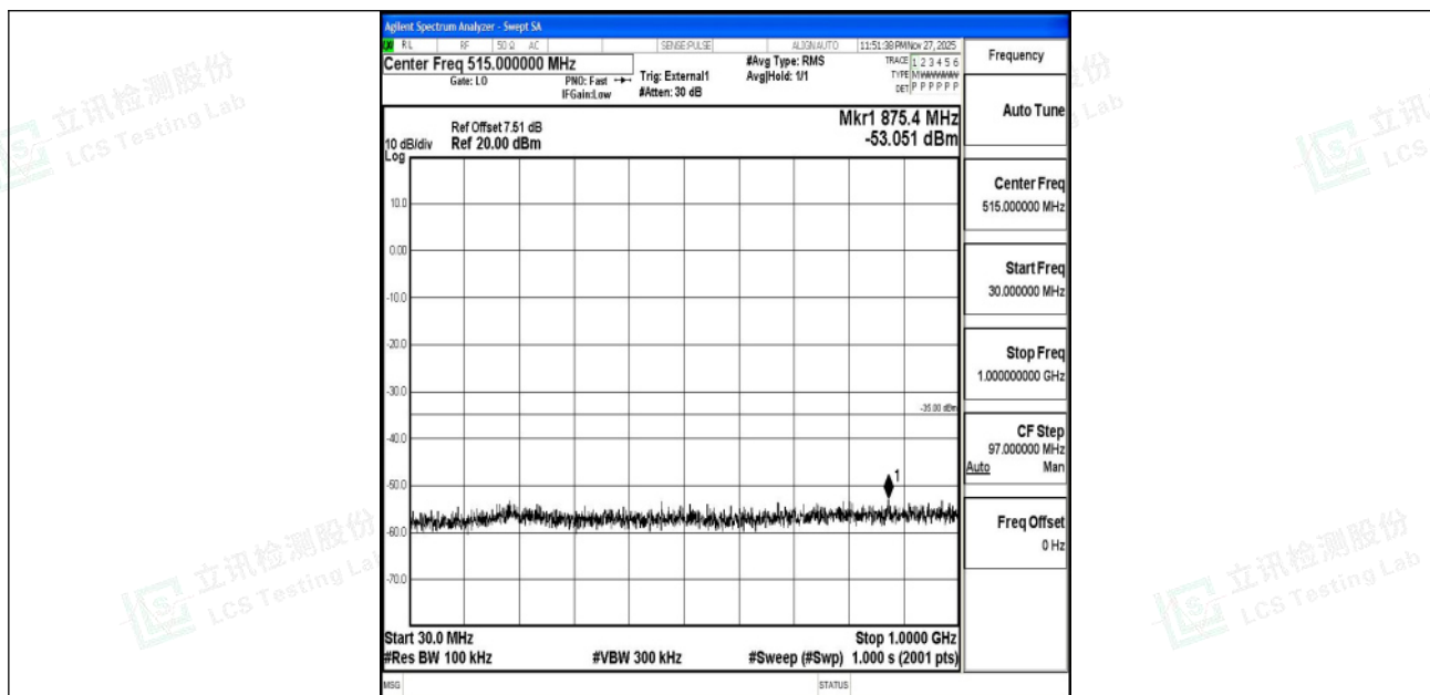
Band41_10MHz_QPSK_39700_1RB#0_30~1000_30~1000
