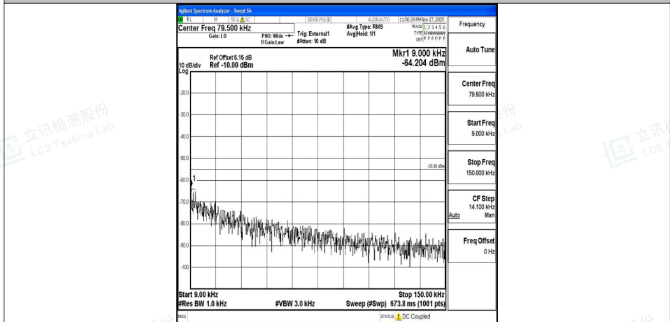
Band41_10MHz_16QAM_40620_1RB#0_0.009~0.15_0.009~0.15
