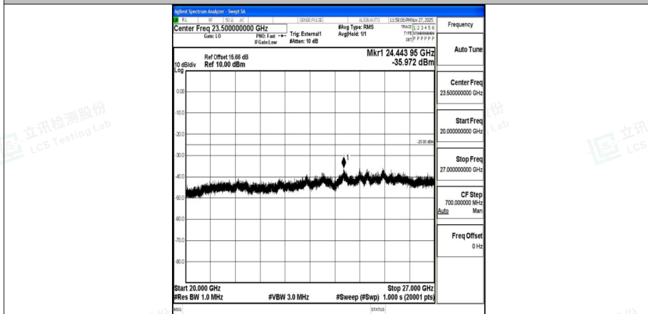
Band41_10MHz_16QAM_40620_1RB#0_20000~27000_20000~27000
