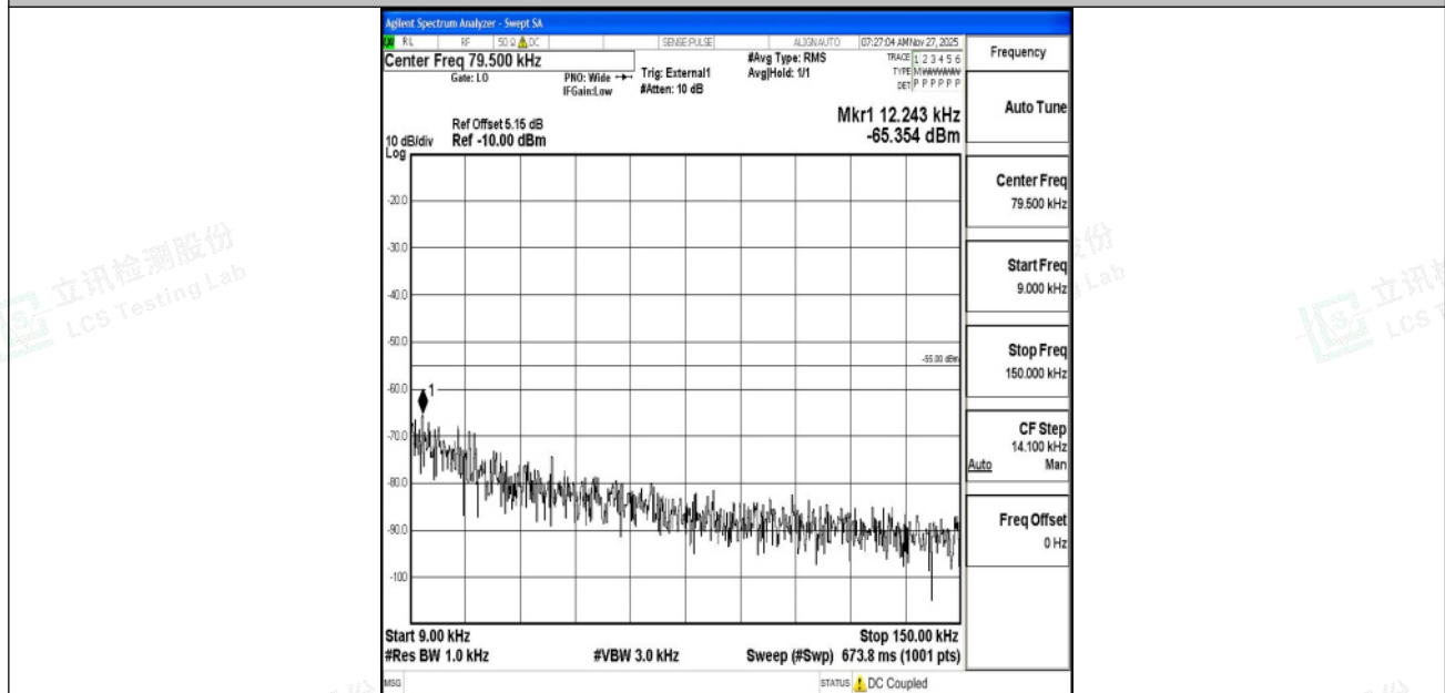
Band41_20MHz_16QAM_40620_1RB#0_0.009~0.15_0.009~0.15
