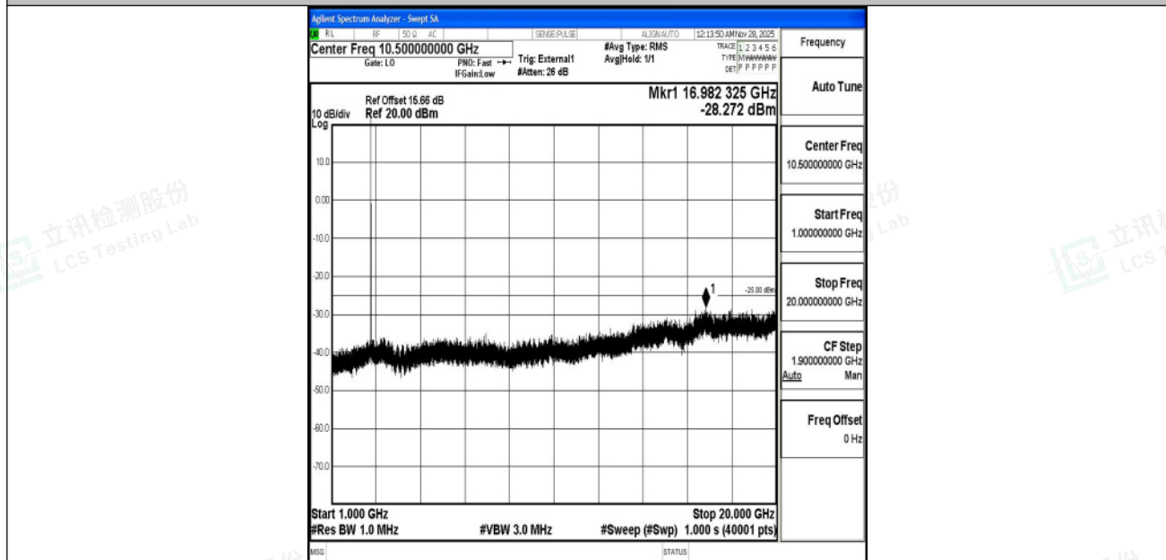
Band41_15MHz_QPSK_41515_1RB#0_1000~20000_1000~20000
