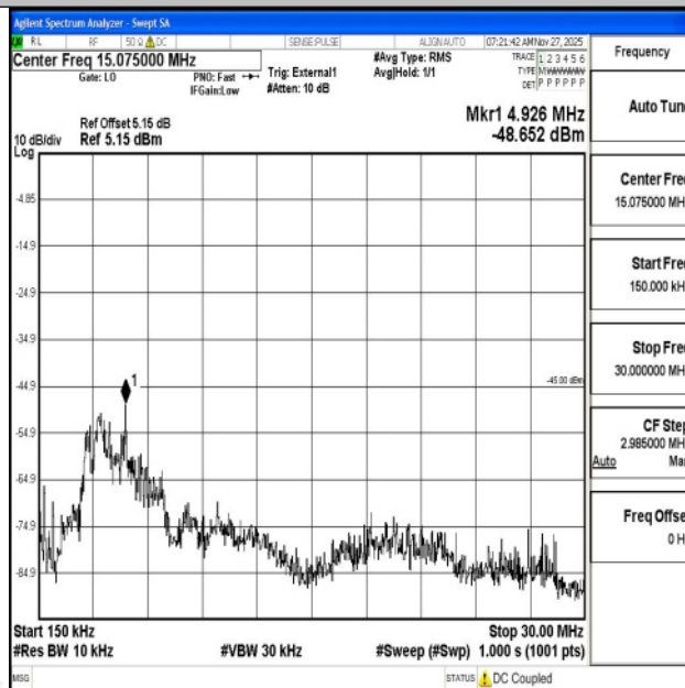
Band41_20MHz_QPSK_39750_1RB#0_0.15~30_0.15~30
