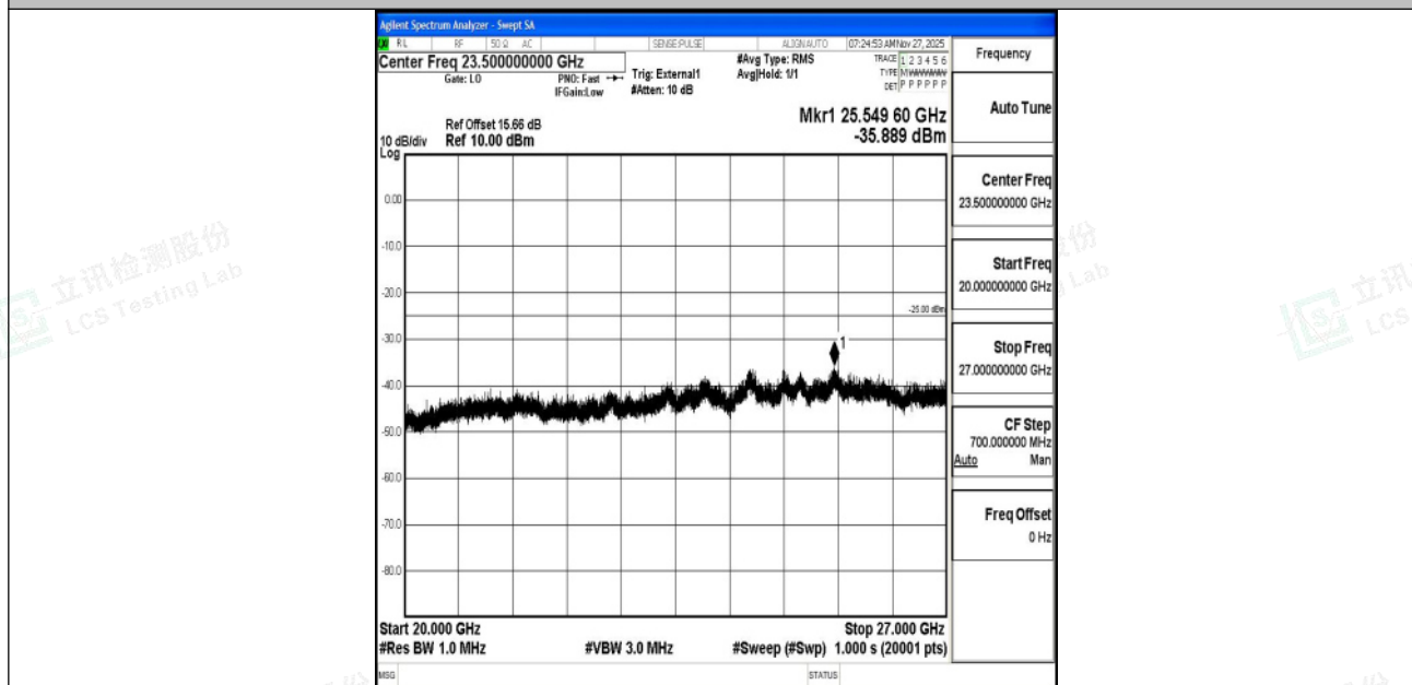
Band41_20MHz_16QAM_39750_1RB#0_20000~27000_20000~27000
