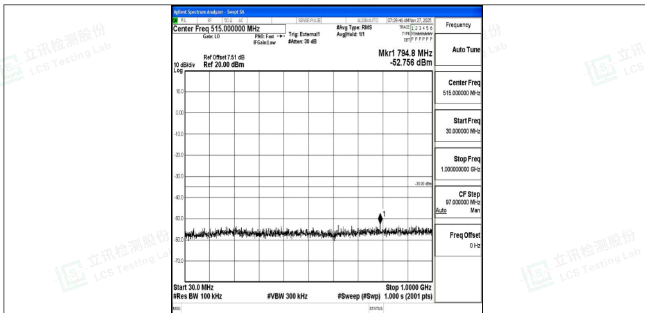
Band41_20MHz_QPSK_41490_1RB#0_30~1000_30~1000
