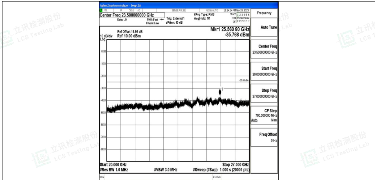
Band41_15MHz_QPSK_41515_1RB#0_20000~27000_20000~27000
