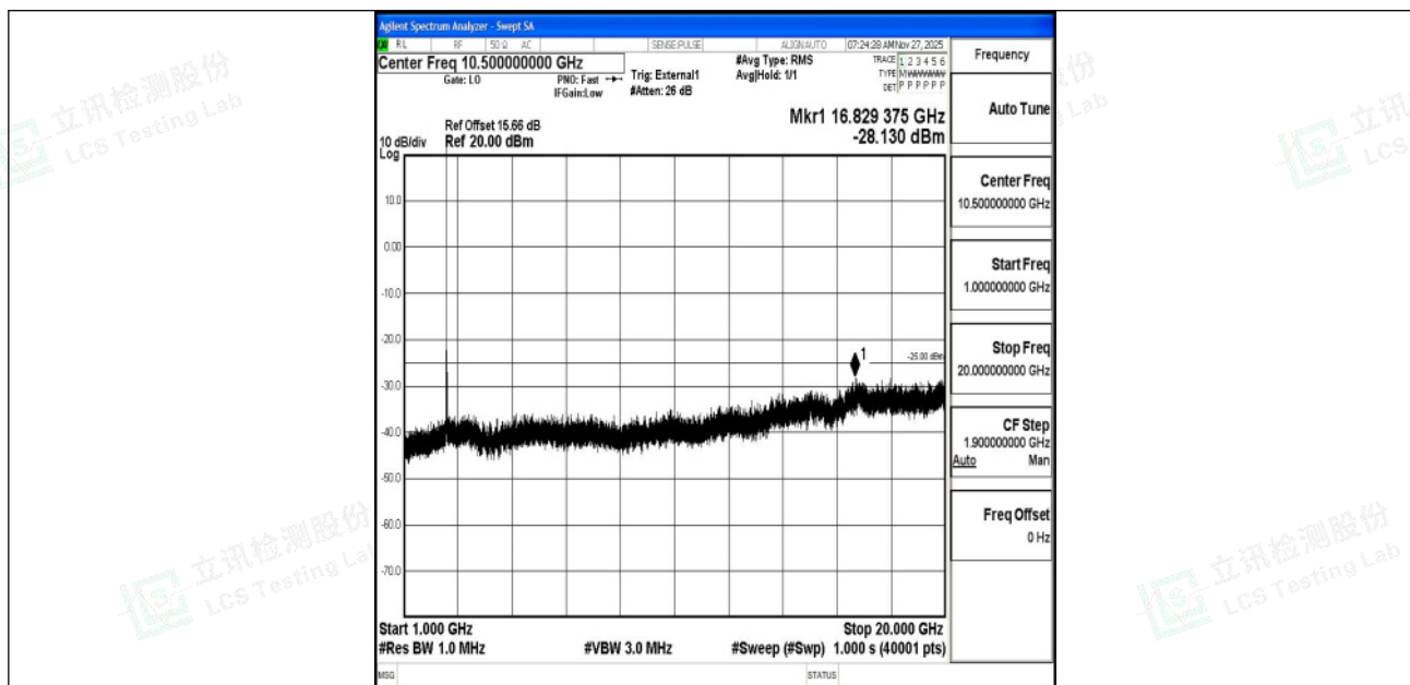
Band41_20MHz_16QAM_39750_1RB#0_1000~20000_1000~20000
