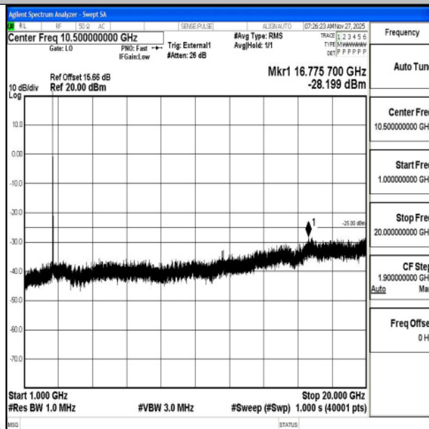
Band41_20MHz_QPSK_40620_1RB#0_1000~20000_1000~20000
