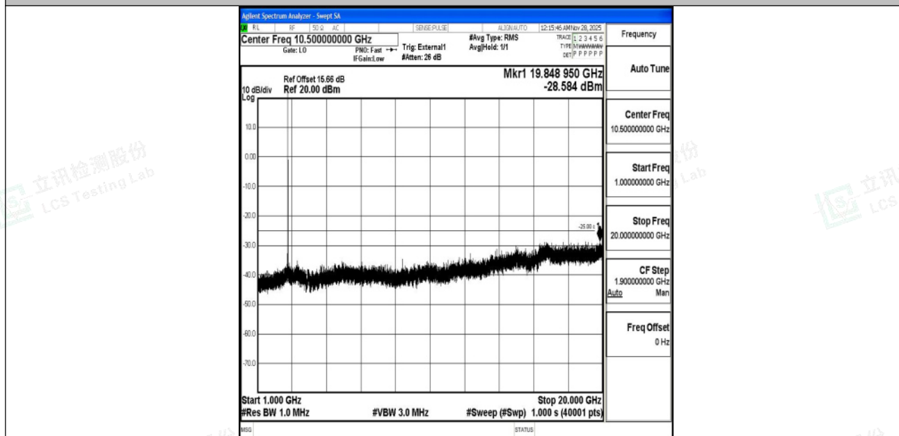
Band41_15MHz_16QAM_41515_1RB#0_1000~20000_1000~20000
