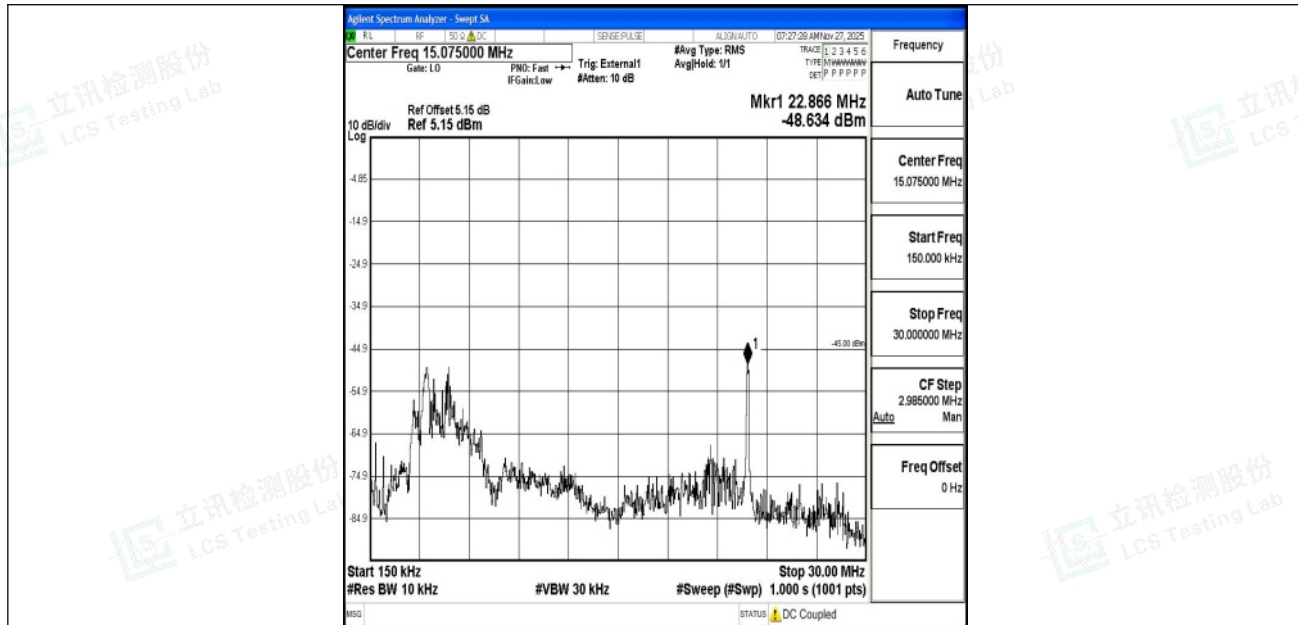
Band41_20MHz_16QAM_40620_1RB#0_0.15~30_0.15~30
