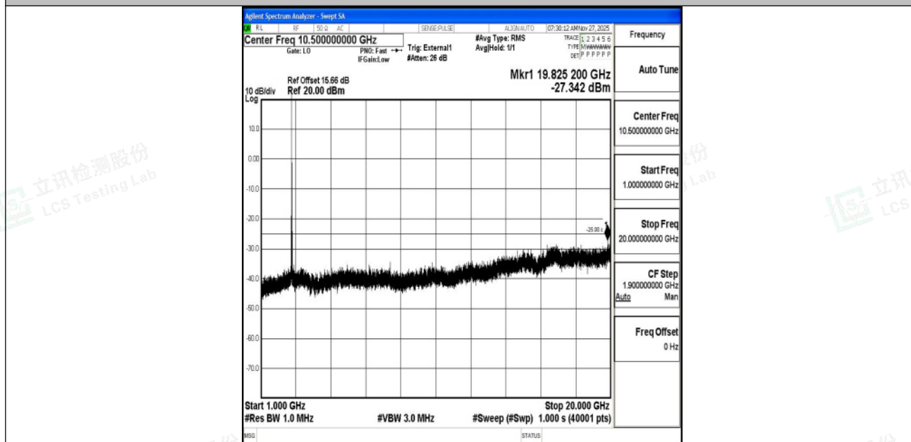
Band41_20MHz_QPSK_41490_1RB#0_1000~20000_1000~20000
