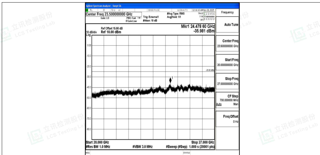
Band41_15MHz_16QAM_41515_1RB#0_20000~27000_20000~27000
