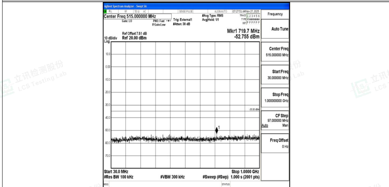
Band41_20MHz_16QAM_40620_1RB#0_30~1000_30~1000
