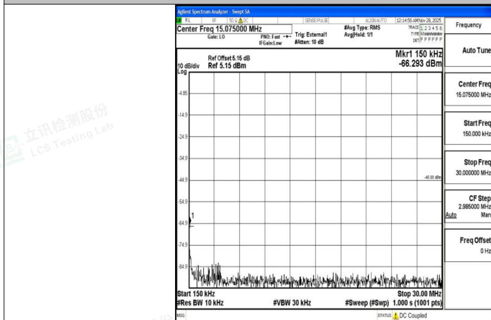
Band41_15MHz_16QAM_41515_1RB#0_0.15~30_0.15~30
