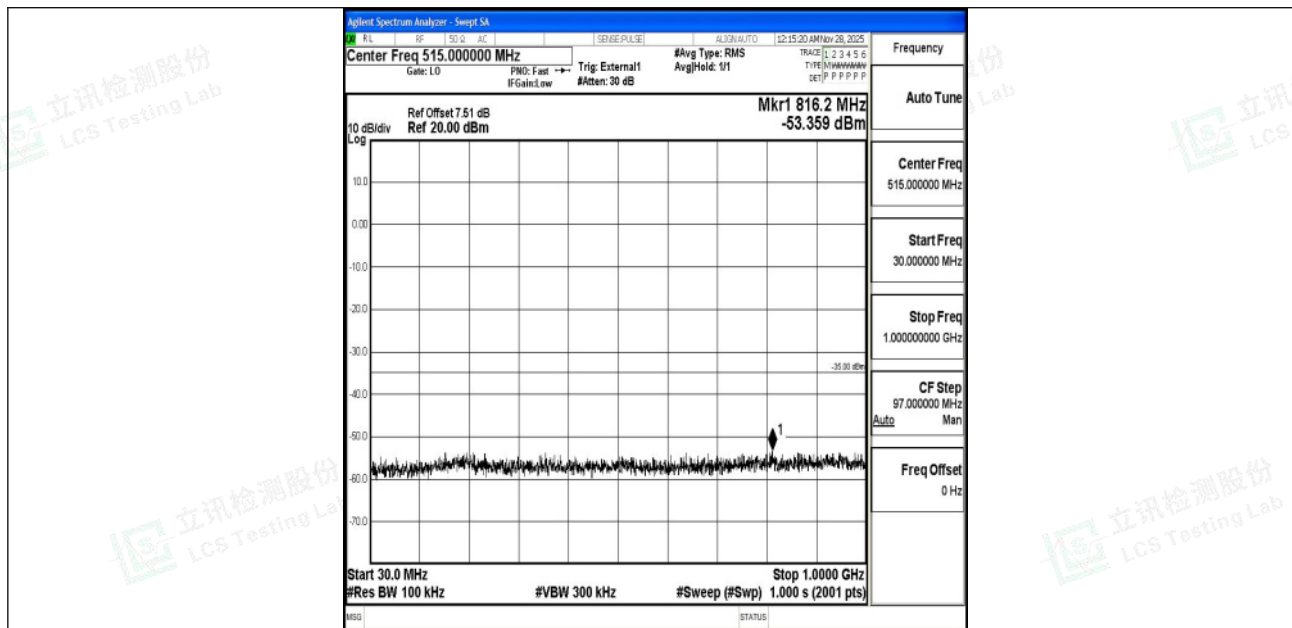
Band41_15MHz_16QAM_41515_1RB#0_30~1000_30~1000
