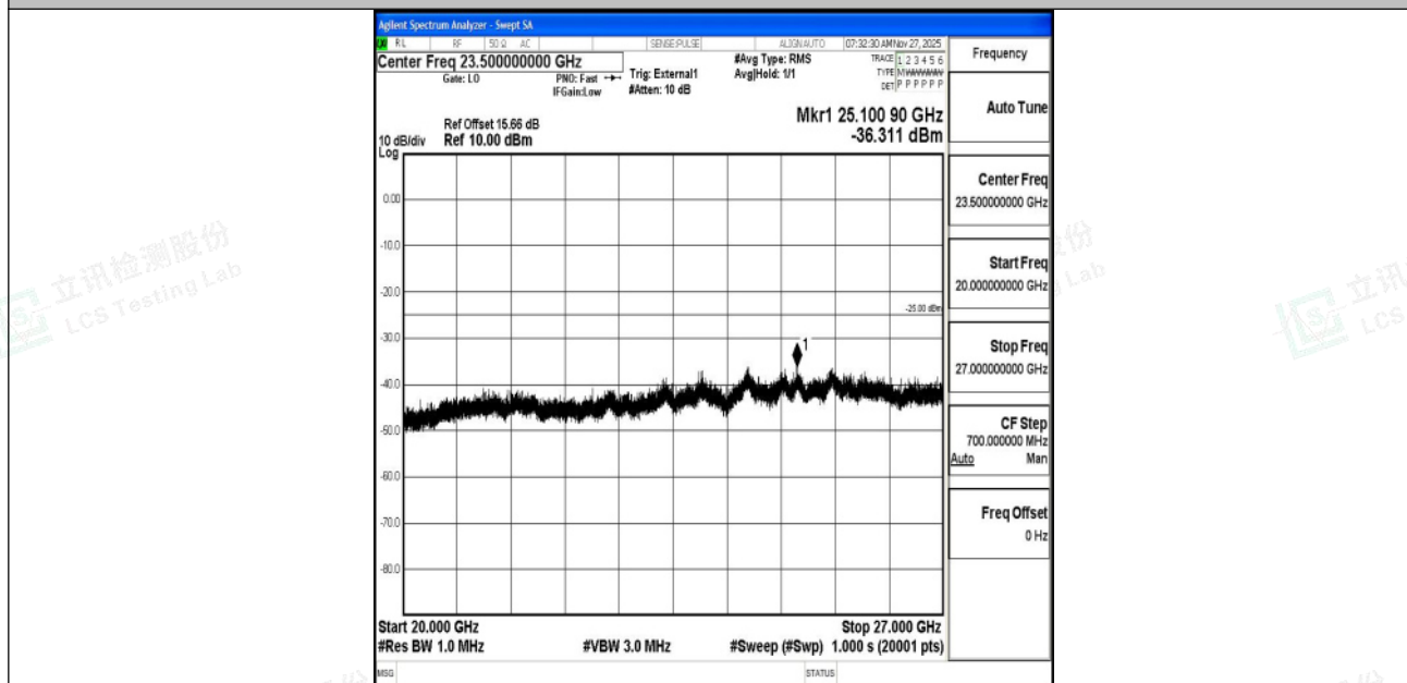
Band41_20MHz_16QAM_41490_1RB#0_20000~27000_20000~27000
