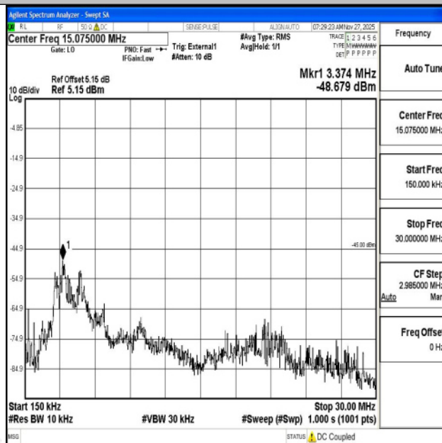
Band41_20MHz_QPSK_41490_1RB#0_0.15~30_0.15~30
