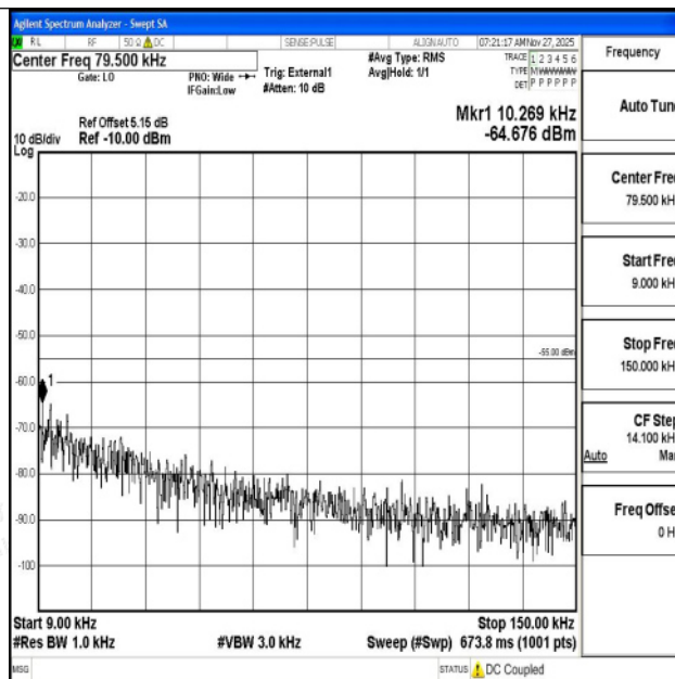
Band41_20MHz_QPSK_39750_1RB#0_0.009~0.15_0.009~0.15
