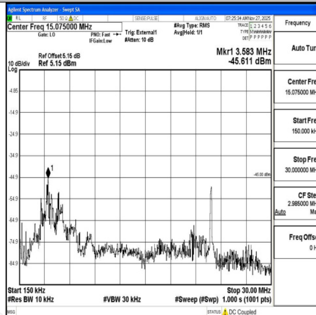
Band41_20MHz_QPSK_40620_1RB#0_0.15~30_0.15~30
