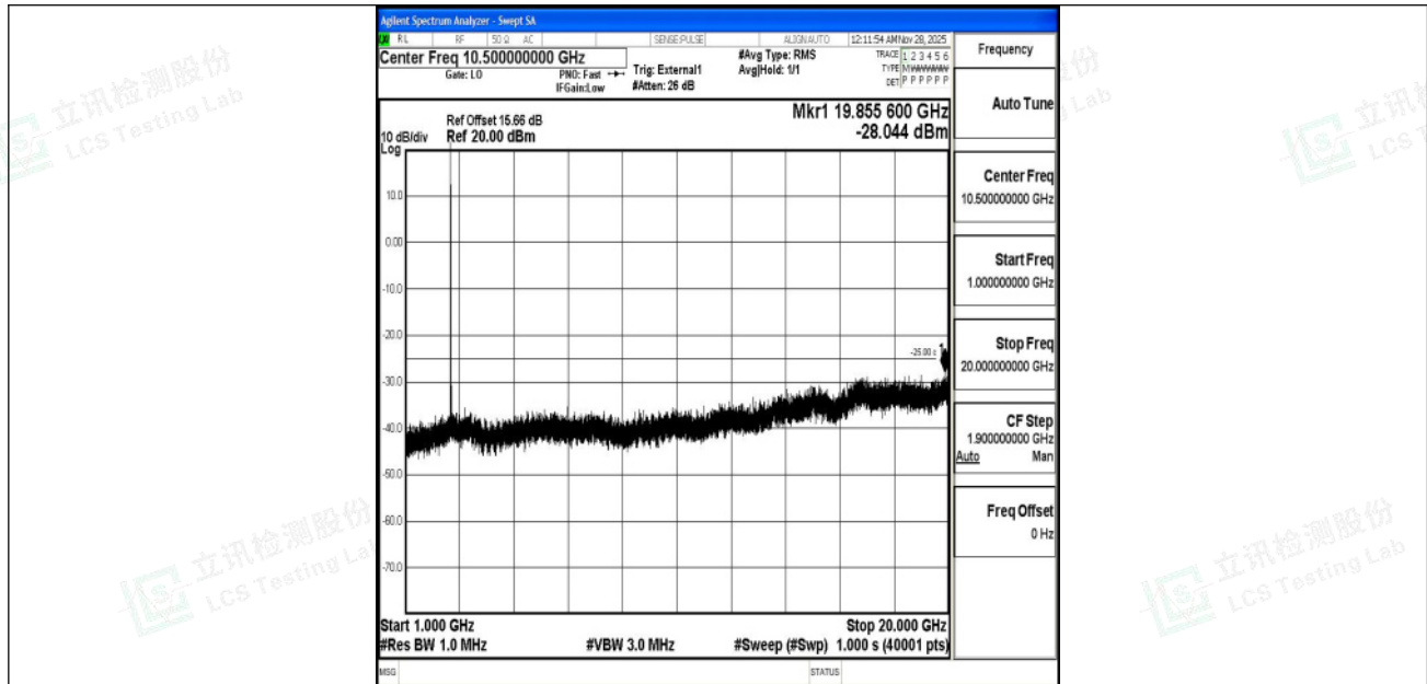
Band41_15MHz_16QAM_40620_1RB#0_1000~20000_1000~20000
