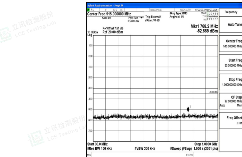
Band41_20MHz_QPSK_39750_1RB#0_30~1000_30~1000
