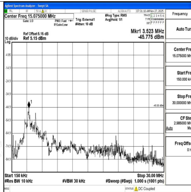
Band41_20MHz_16QAM_41490_1RB#0_0.15~30_0.15~30
