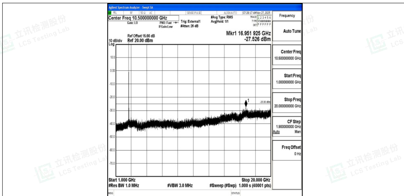
Band41_20MHz_16QAM_40620_1RB#0_1000~20000_1000~20000
