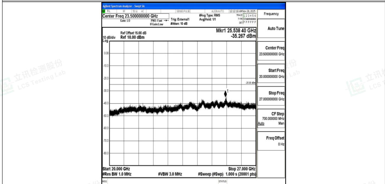
Band41_15MHz_16QAM_40620_1RB#0_20000~27000_20000~27000
