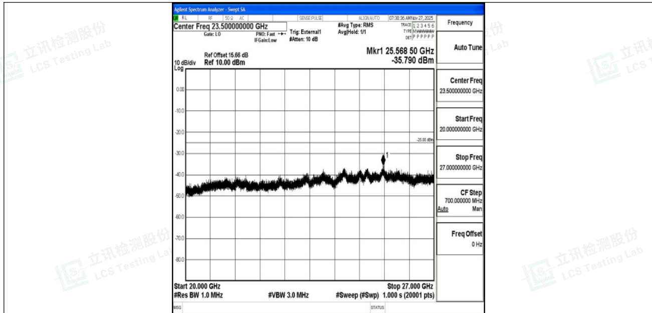
Band41_20MHz_QPSK_41490_1RB#0_20000~27000_20000~27000
