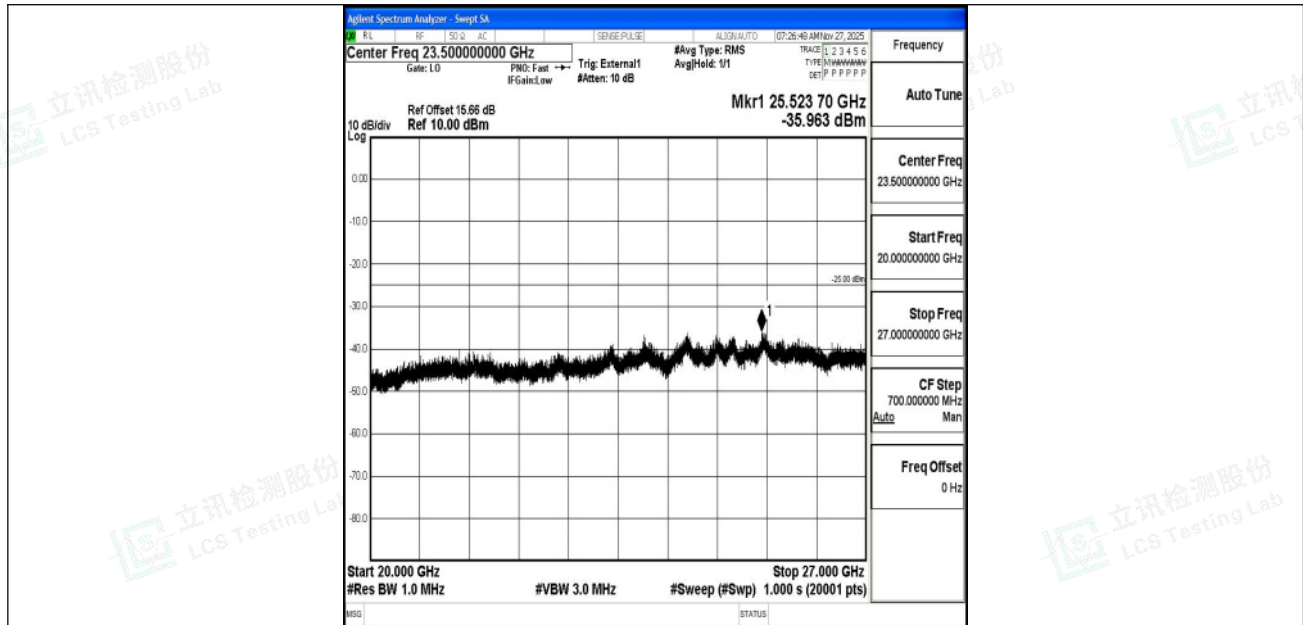
Band41_20MHz_QPSK_40620_1RB#0_20000~27000_20000~27000
