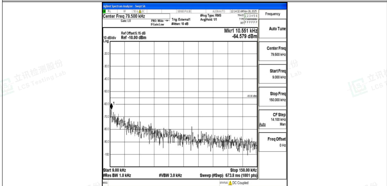
Band41_15MHz_16QAM_41515_1RB#0_0.009~0.15_0.009~0.15
