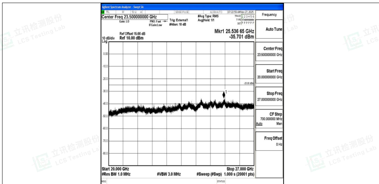
Band41_20MHz_QPSK_39750_1RB#0_20000~27000_20000~27000
