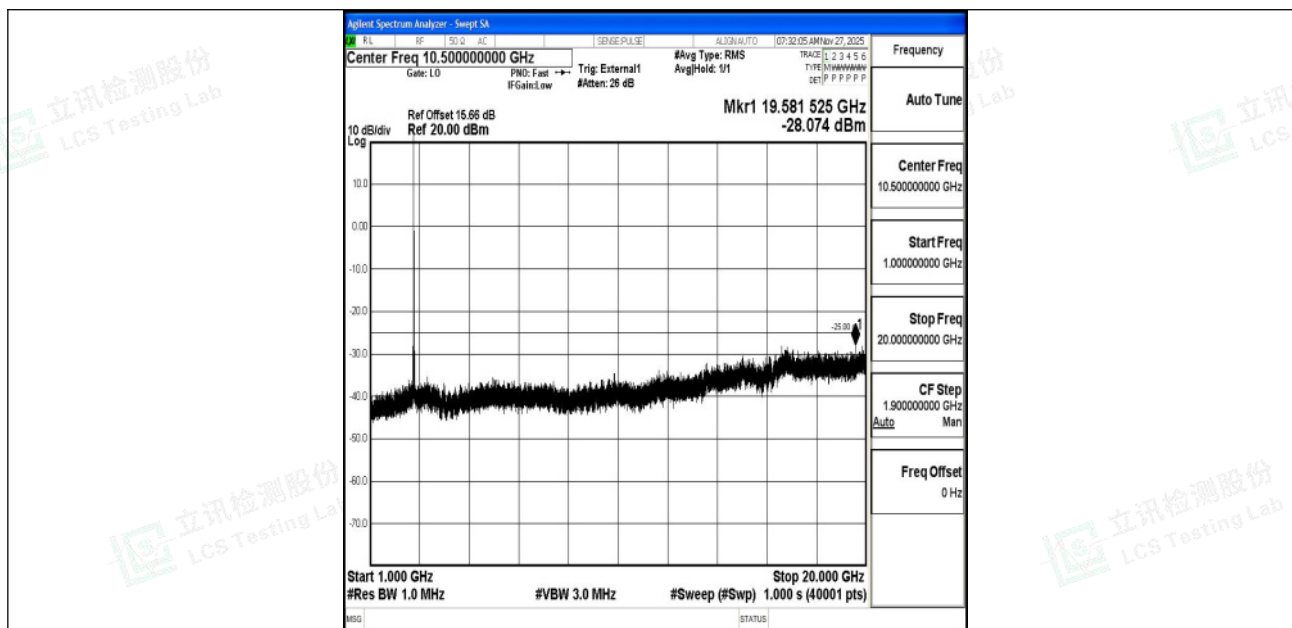
Band41_20MHz_16QAM_41490_1RB#0_1000~20000_1000~20000
