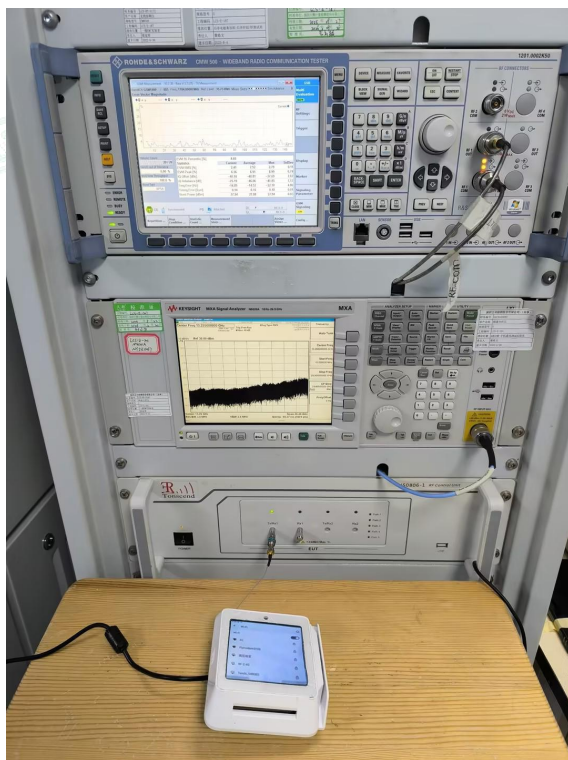
Test Setup Photo(s) of RF Conducted Measurement
