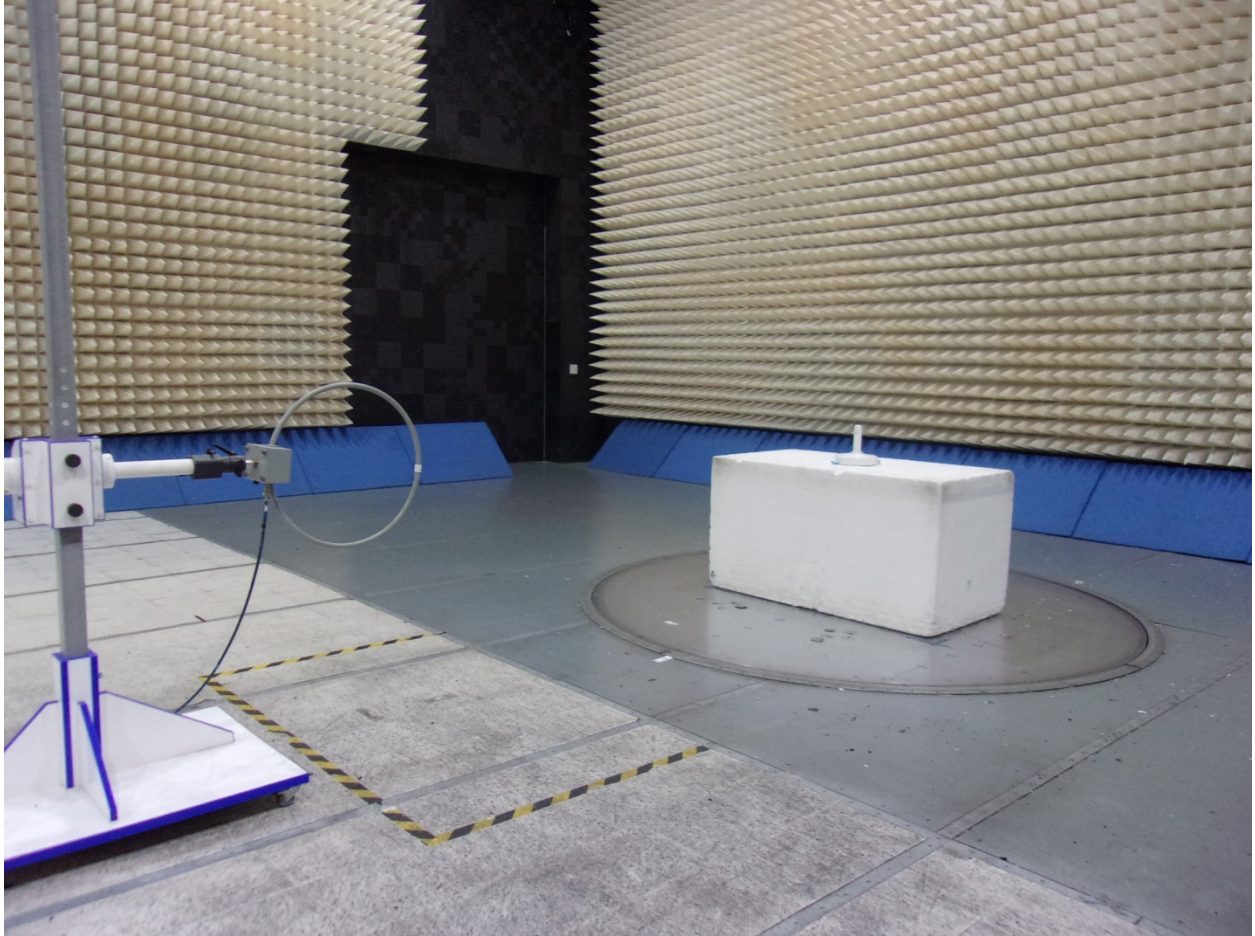
Unintentional and Radiated Spurious Emissions, 10kHz – 30MHz
