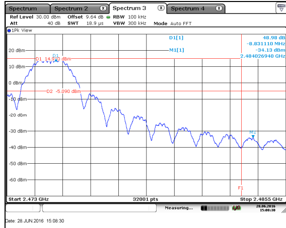
Figure 7.5.1.2-6: Upper Band-Edge – CH 25
