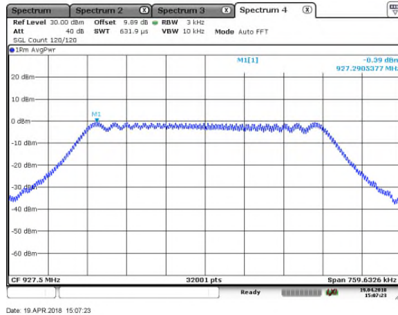
Figure 7.6.2-3: PSD – HCH, SF=7
