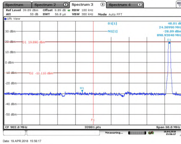
Figure 7.5.1.2-9: Lower Band-edge, SF=12
