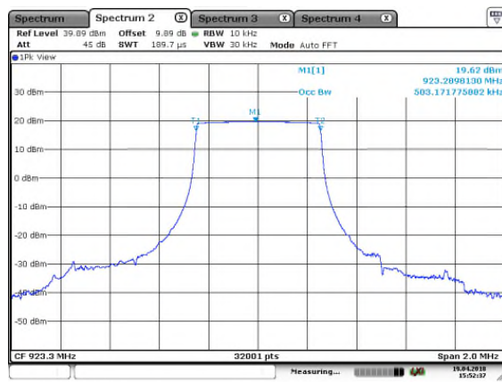
Figure 7.3.2-10: 99% OBW – LCH , SF=12
