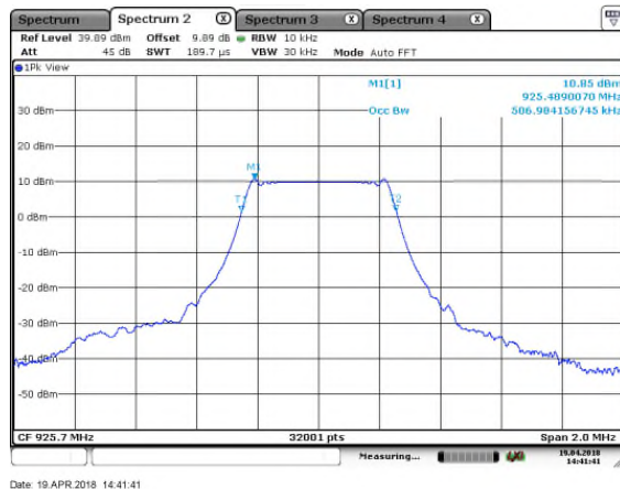
Figure 7.3.2-5: 99% OBW - MCH , SF=7
