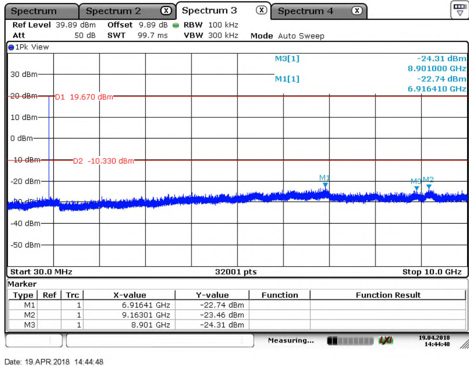
Figure 7.5.1.2-2: RF Conducted Emissions – MCH, SF=7
