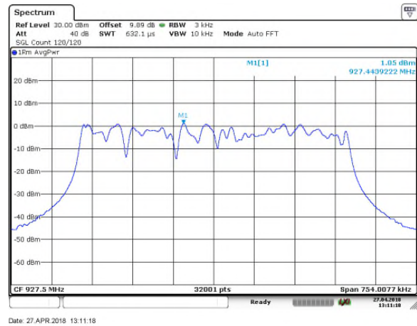
Figure 7.6.2-6: PSD – HCH, SF=12
