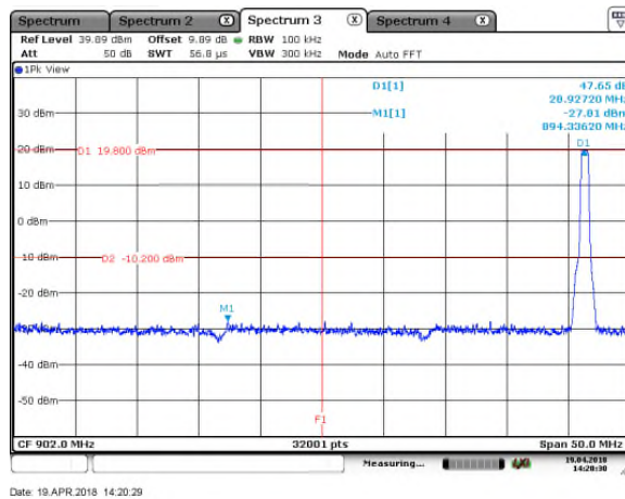
Figure 7.5.1.2-7: Lower Band-edge, SF=7
