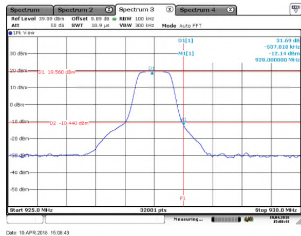
Figure 7.5.1.2-8: Upper Band-edge, SF=7
