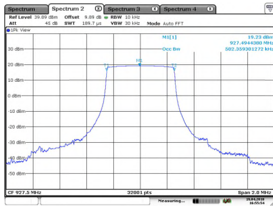
Figure 7.3.2-12: 99% OBW – HCH , SF=12
