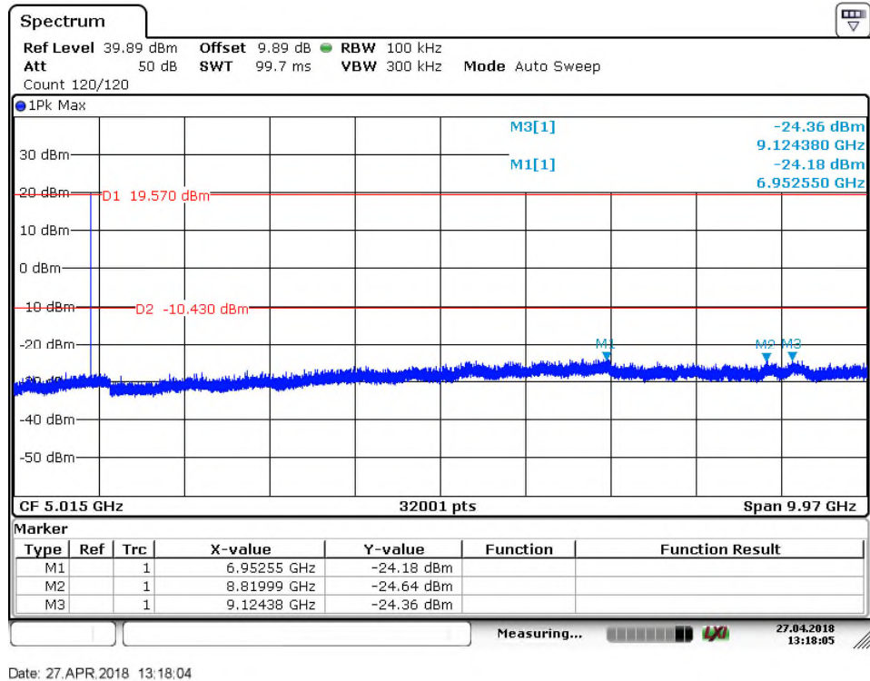
Figure 7.5.1.2-6: RF Conducted Emissions – HCH, SF=12
