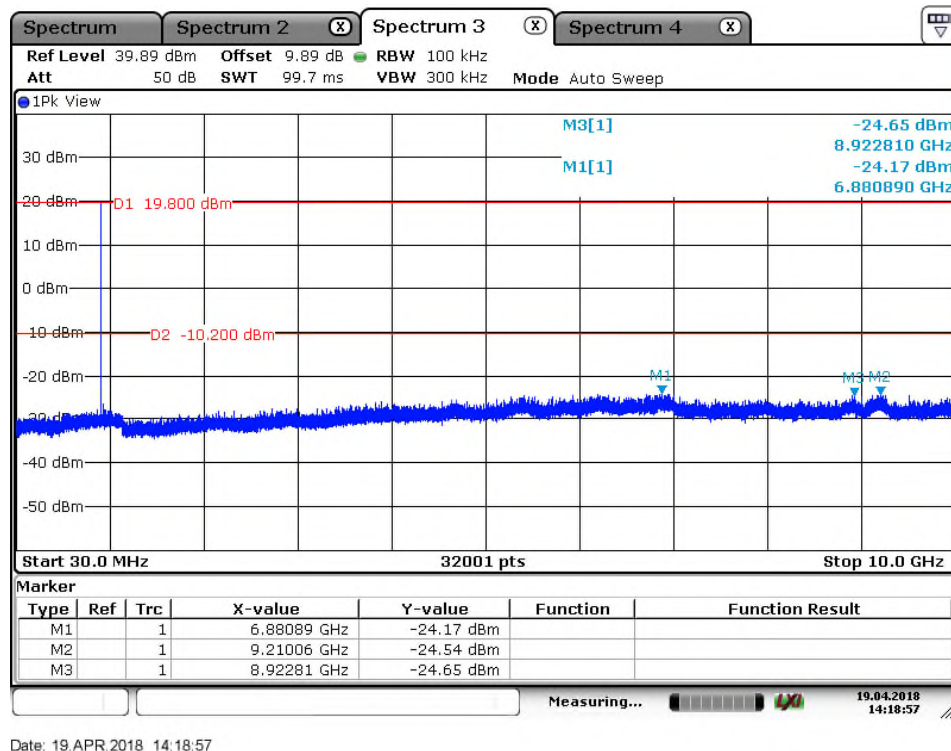
Figure 7.5.1.2-1: RF Conducted Emissions – LCH, SF=7
