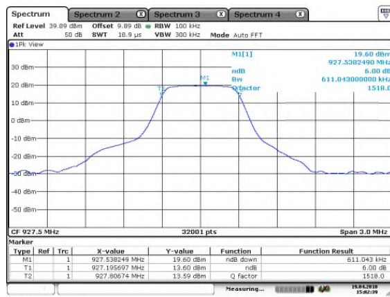
Figure 7.3.2-9: 6dB BW – HCH , SF=12
