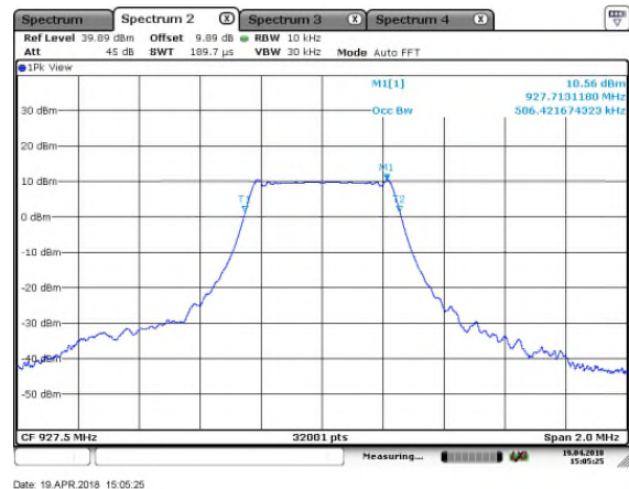
Figure 7.3.2-6: 99% OBW - HCH , SF=7
