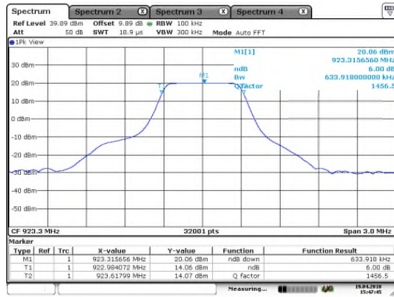
Figure 7.3.2-7: 6dB BW – LCH , SF=12
