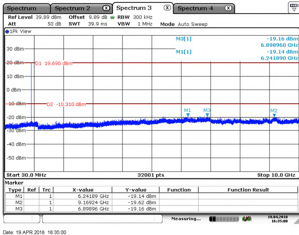
Figure 7.5.1.2-5: RF Conducted Emissions – MCH, SF=12
