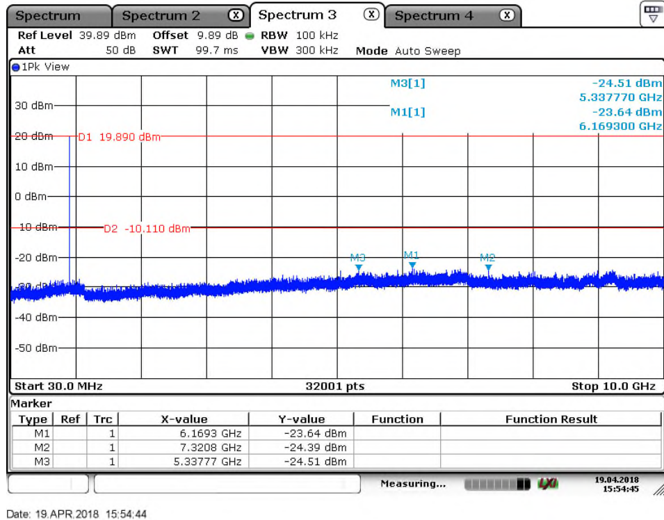
Figure 7.5.1.2-4: RF Conducted Emissions – LCH, SF=12
