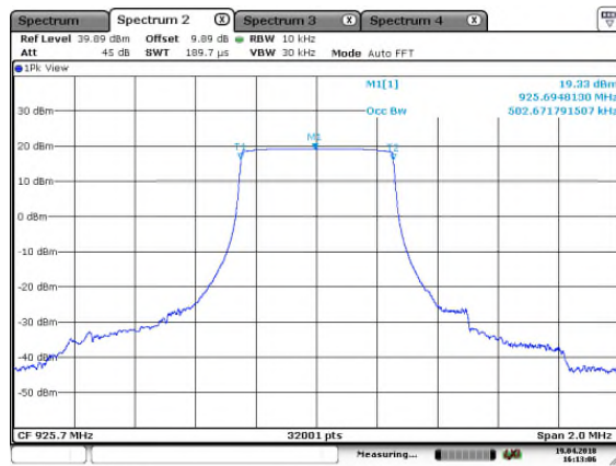
Figure 7.3.2-11: 99% OBW – MCH , SF=12
