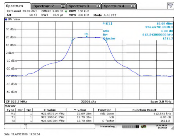
Figure 7.3.2-2: 6dB BW - MCH , SF=7
