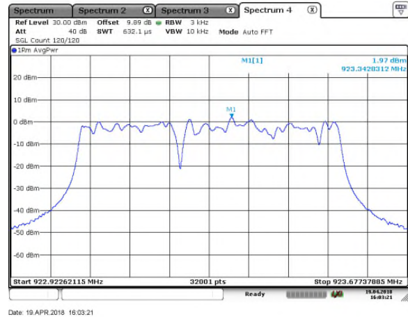
Figure 7.6.2-4: PSD – LCH, SF=12
