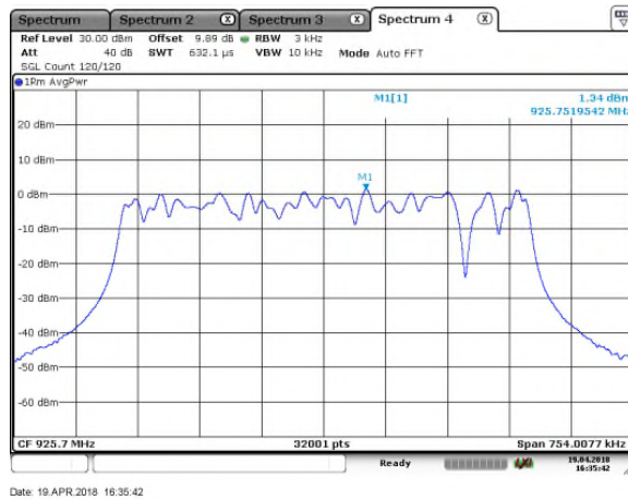
Figure 7.6.2-5: PSD – MCH, SF=12
