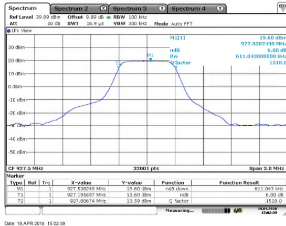
Figure 7.3.2-3: 6dB BW - HCH , SF=7
