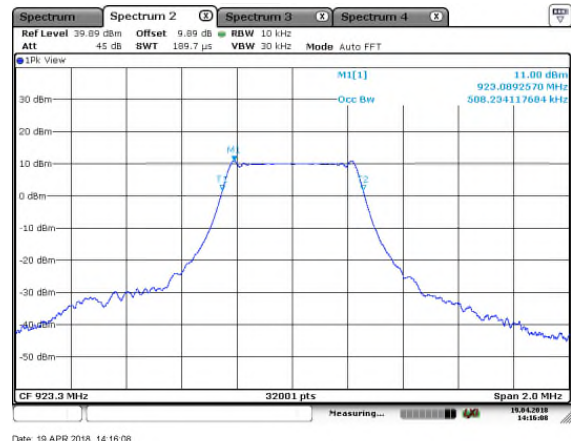
Figure 7.3.2-4: 99% OBW - LCH , SF=7
