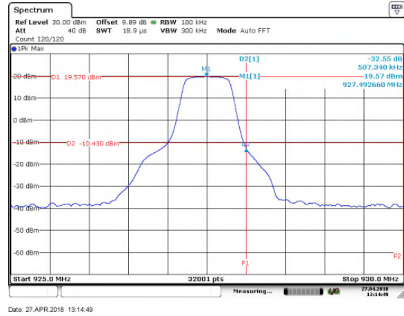
Figure 7.5.1.2-10: Upper Band-edge, SF=12
