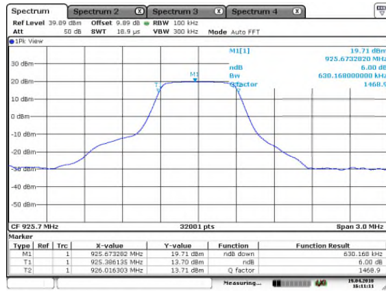
Figure 7.3.2-8: 6dB BW – MCH , SF=12
