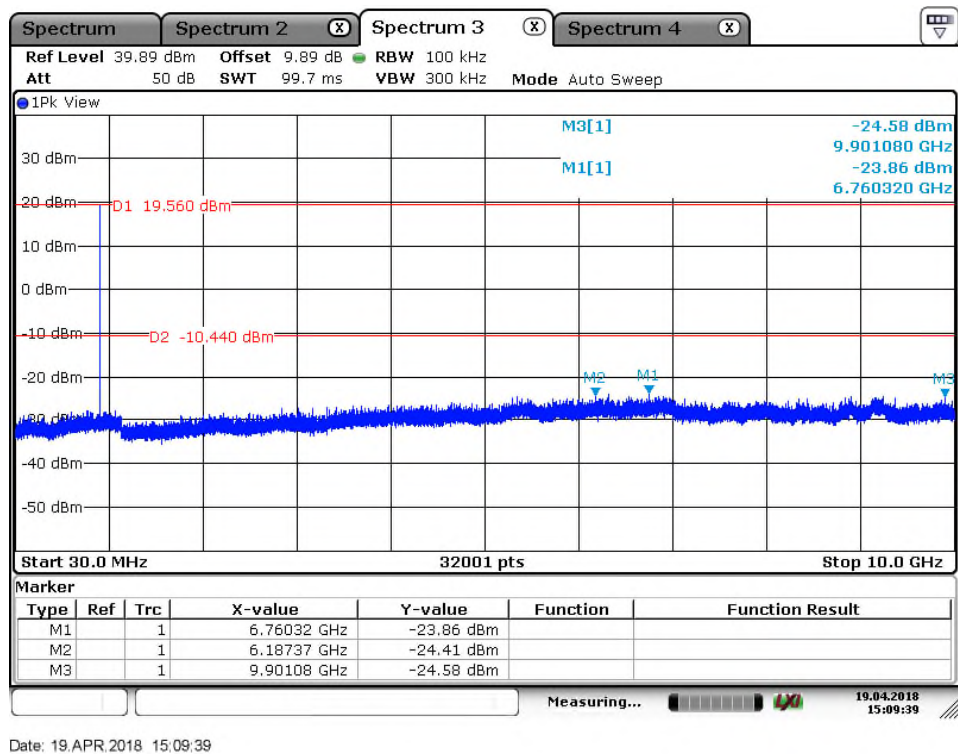
Figure 7.5.1.2-3: RF Conducted Emissions – HCH, SF=7
