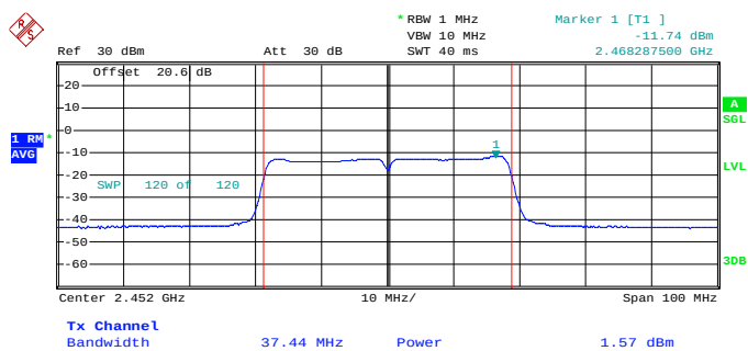
Figure 7.3.2-5: RF Output Power - Middle Channel – 802.11n 40 MHz – Antenna Port 2
