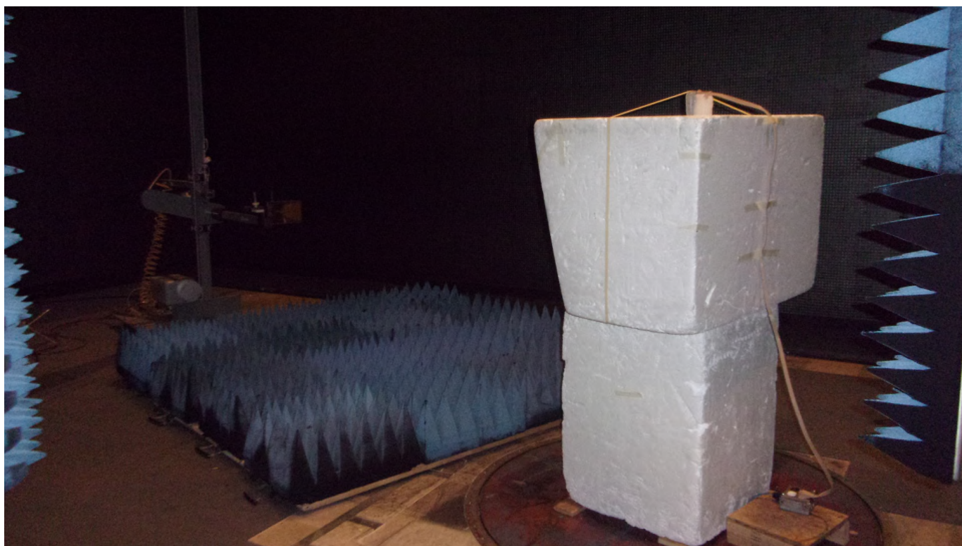
Figure 4: Radiated Emissions – 1GHz – 10GHz
