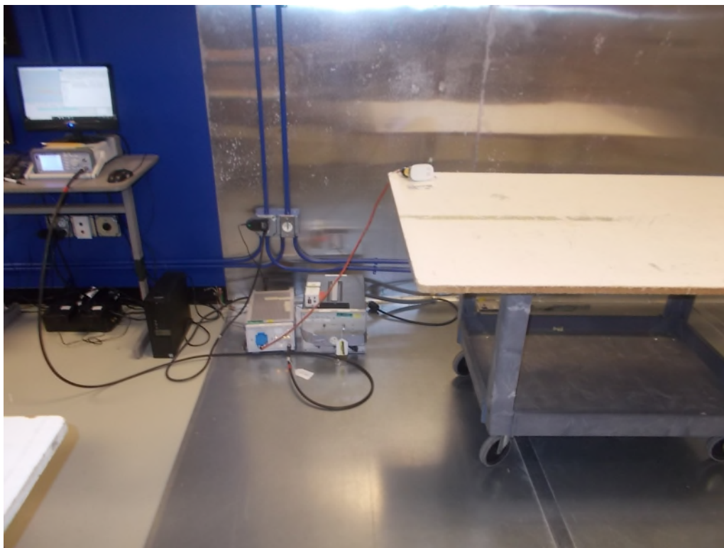
Figure 8: AC Power Line Conducted Emissions
