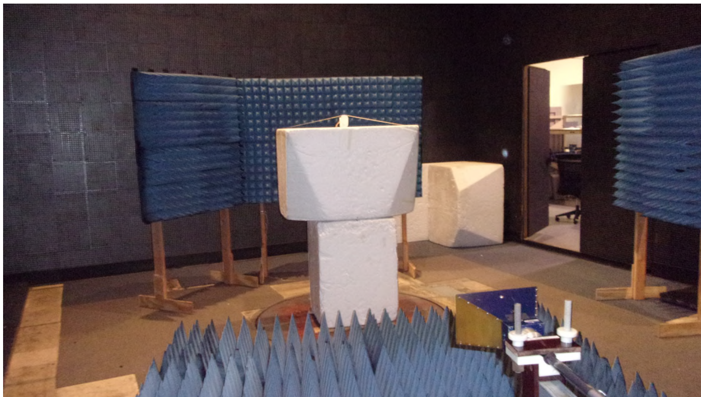
Figure 3: Radiated Emissions – 1GHz – 10GHz
