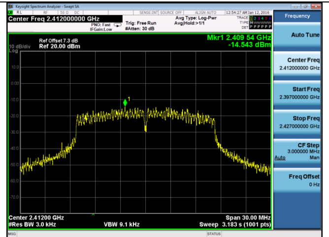
PSD-2.4G-802.11g 2412MHz
