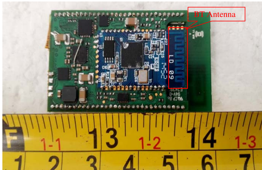
EUT – Main Board-1 Rear View
