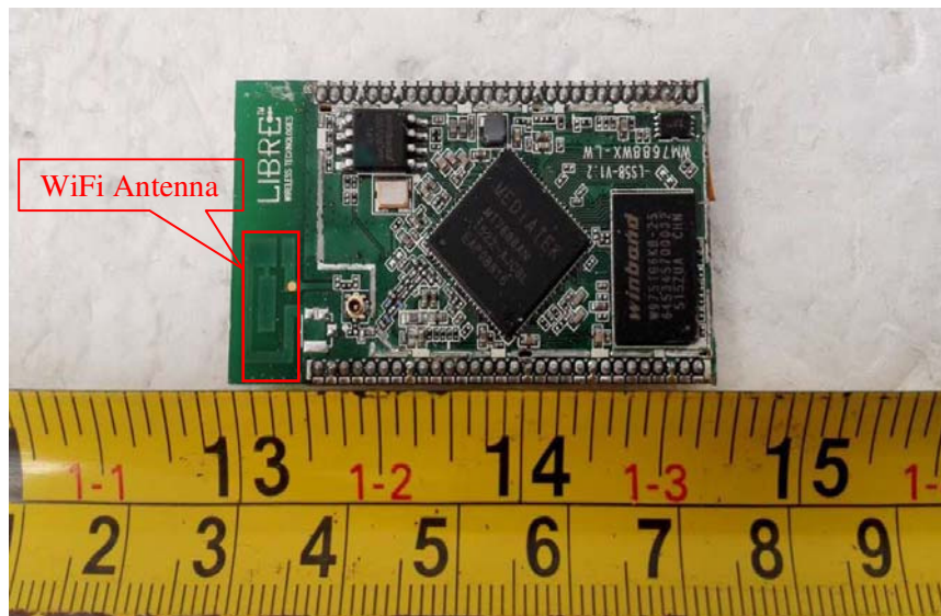
EUT – Main Board-1 Rear View
