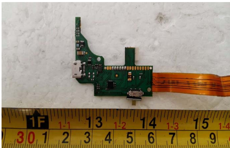
EUT – Main Board-2 Front View
