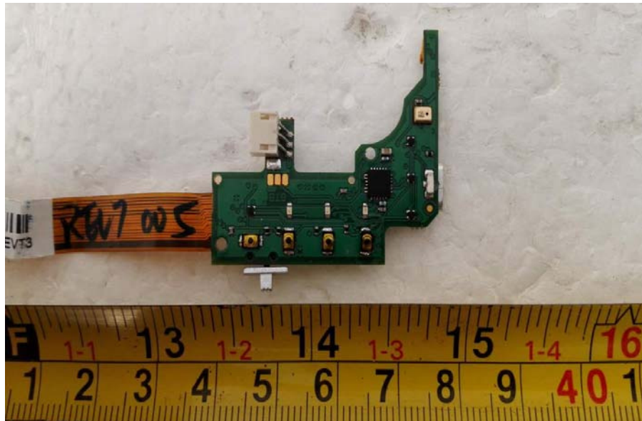
EUT – Main Board-2 Rear View
