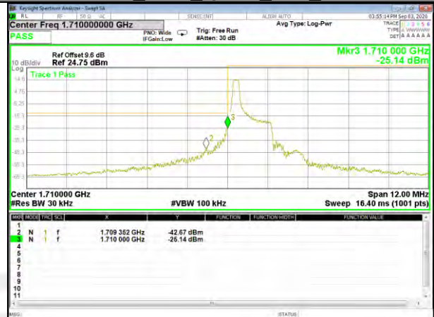
Band4_1.4M_QPSK_Low_Full-RB
