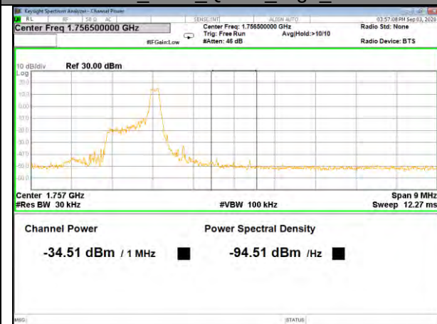
Band4_1.4M_QPSK_High_1-RB
