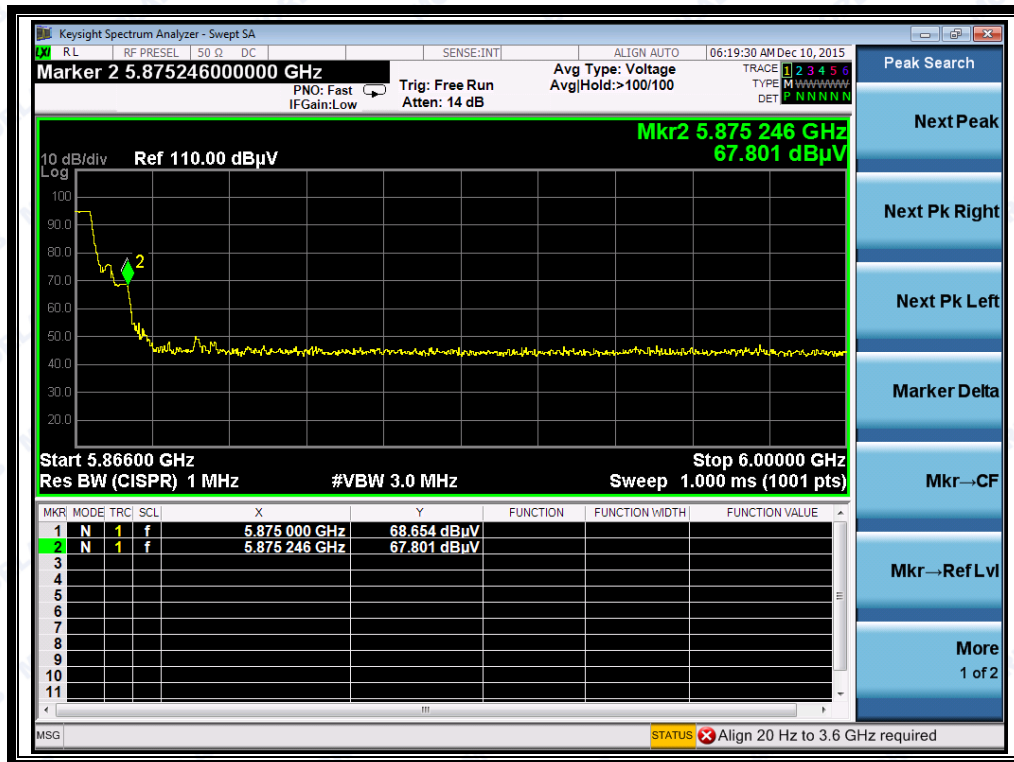
(Plot 5PK@ Highest Channel : 5866 MHz)
