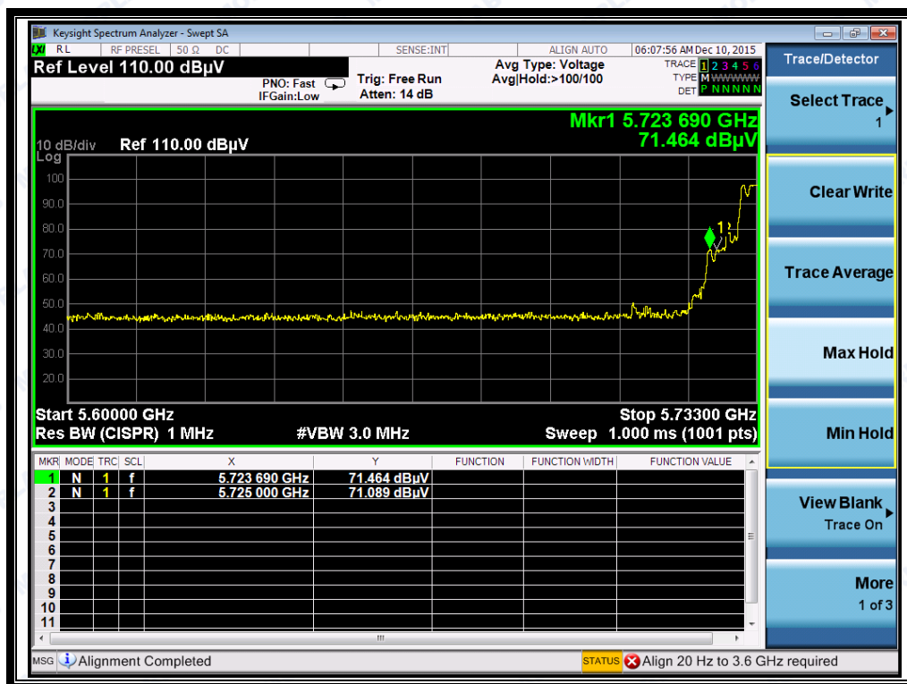
(Plot 1 PK @ Lowest Channel : 5733 MHz)
