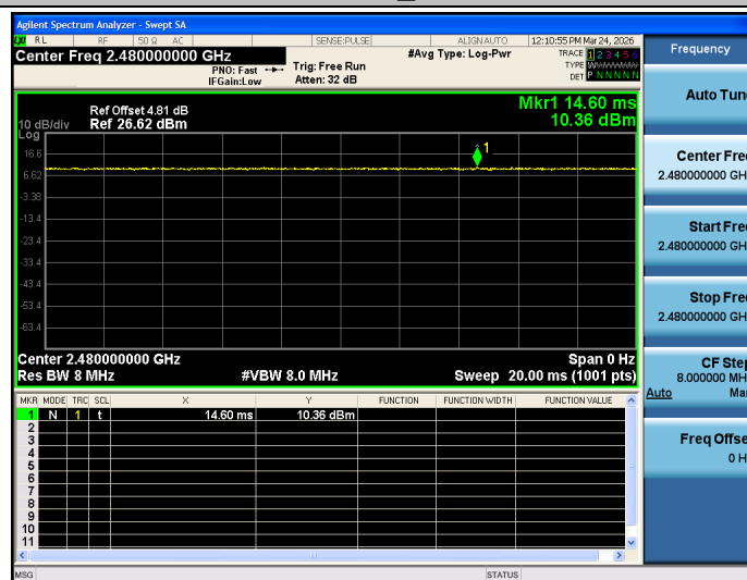
8-DPSK_2480
