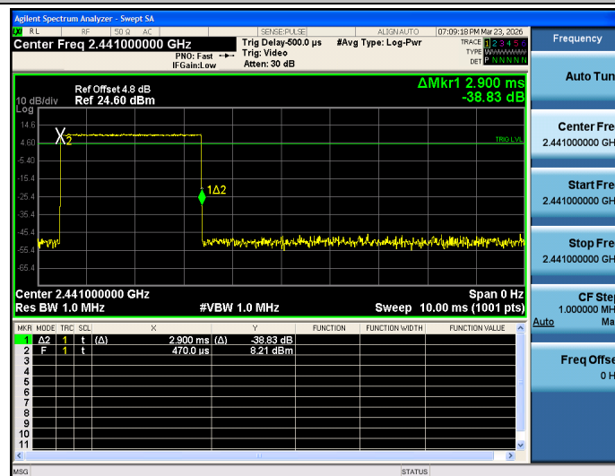
8-DPSK_3DH1_2441
