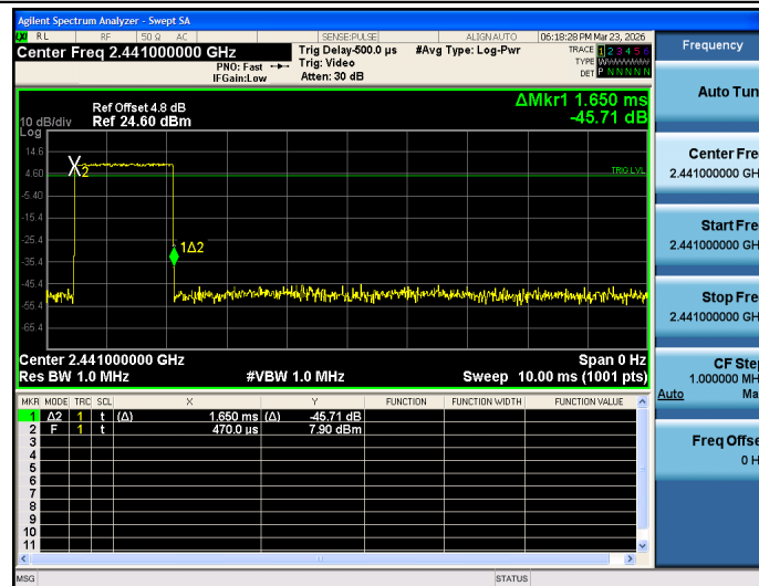
\pi/4 -DQPSK_2DH5_2441
