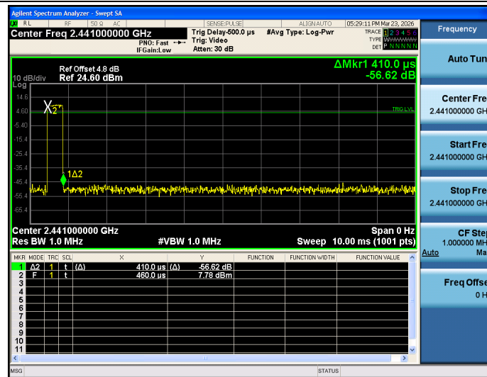
\pi/4 -DQPSK_2DH3_2441
