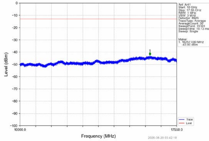
Band4_10MHz_16QAM_LCH_1715MHz_RB_50_0_NTNV
