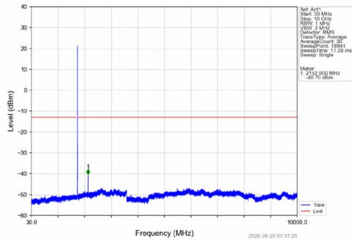
Band4_5MHz_16QAM_HCH_1752.5MHz_RB_1_0_NTNV
