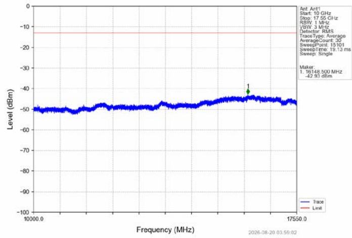
Band4_15MHz_16QAM_HCH_1747.5MHz_RB_1_0_NTNV
