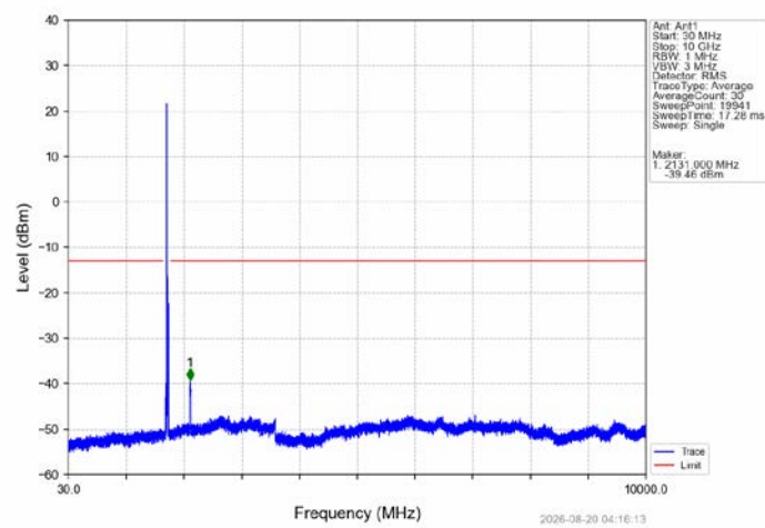
Band4_20MHz_16QAM_MCH_1732.5MHz_RB_1_0_NTNV
