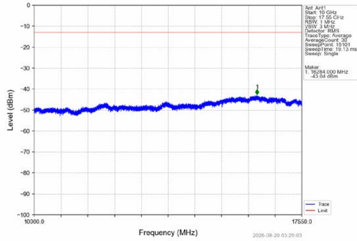
Band4_5MHz_16QAM_LCH_1712.5MHz_RB_25_0_NTNV
