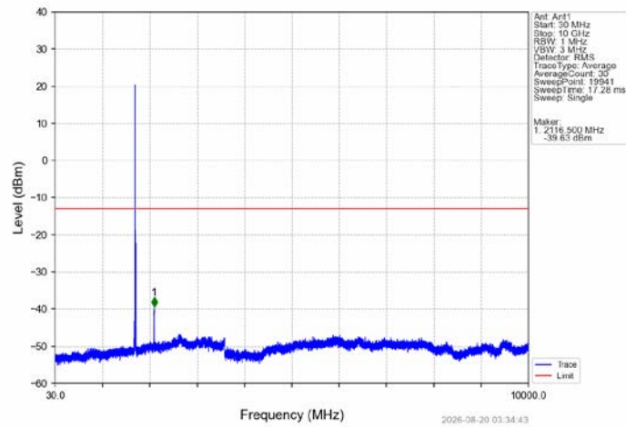
Band4_10MHz_QPSK_LCH_1715MHz_RB_1_0_NTNV
