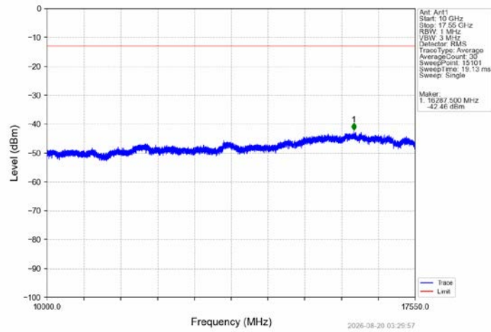
Band4_5MHz_16QAM_HCH_1752.5MHz_RB_1_0_NTNV
