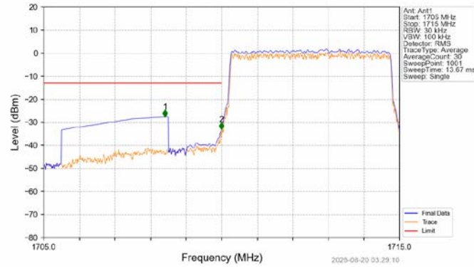
Band4_5MHz_16QAM_LCH_1712.5MHz_RB_25_0_NTNV
