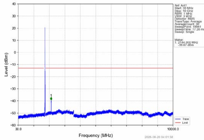
Band4_15MHz_16QAM_HCH_1747.5MHz_RB_1_0_NTNV
