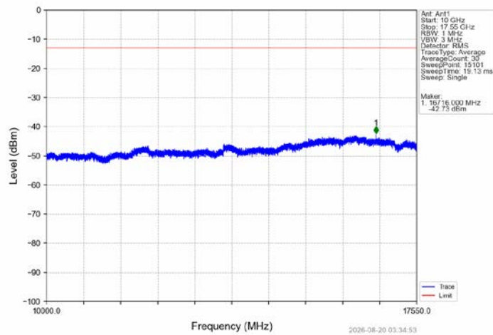
Band4_10MHz_QPSK_LCH_1715MHz_RB_1_0_NTNV
