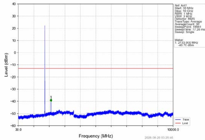
Band4_5MHz_16QAM_MCH_1732.5MHz_RB_1_0_NTNV
