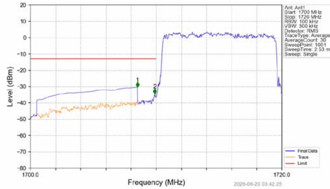
Band4_10MHz_16QAM_LCH_1715MHz_RB_50_0_NTNV
