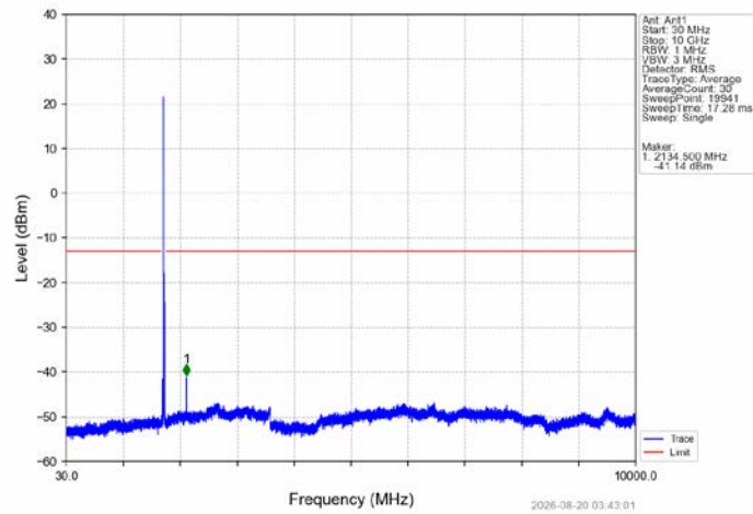
Band4_10MHz_16QAM_MCH_1732.5MHz_RB_1_0_NTNV
