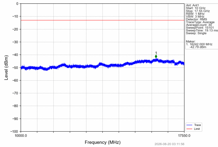
Band4_1.4MHz_16QAM_HCH_1754.3MHz_RB_1_0_NTNV
