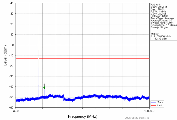
Band4_1.4MHz_16QAM_HCH_1754.3MHz_RB_1_0_NTNV
